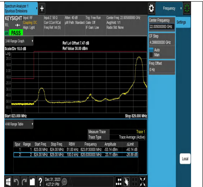
Band26_5MHz_QPSK_26815_1RB#24
