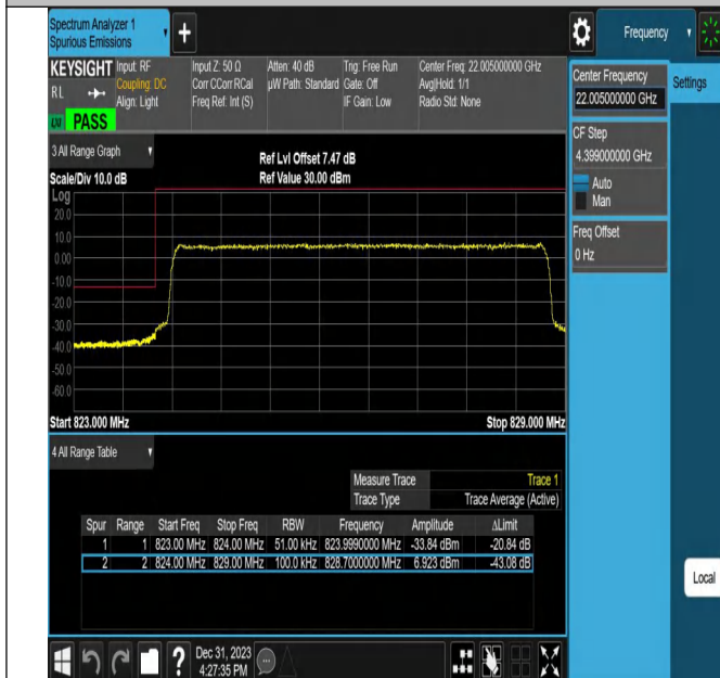
Band26_5MHz_QPSK_26815_25RB#0
