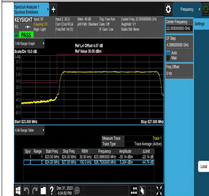
Band26_3MHz_QPSK_26805_15RB#0
