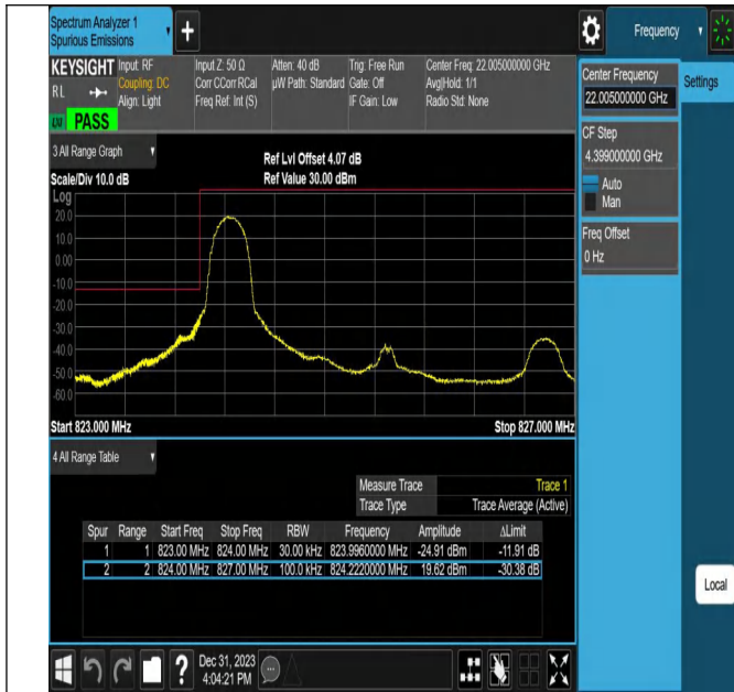
Band26_3MHz_QPSK_26805_1RB#0
