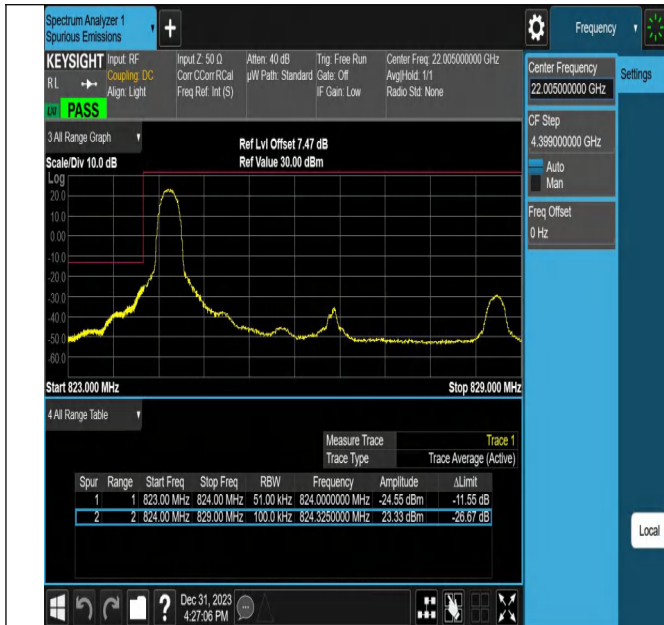
Band26_5MHz_QPSK_26815_1RB#0
