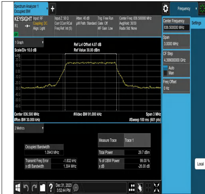
26(824-849)-1.4MHz-16QAM-26915-6RB#0-PASS
