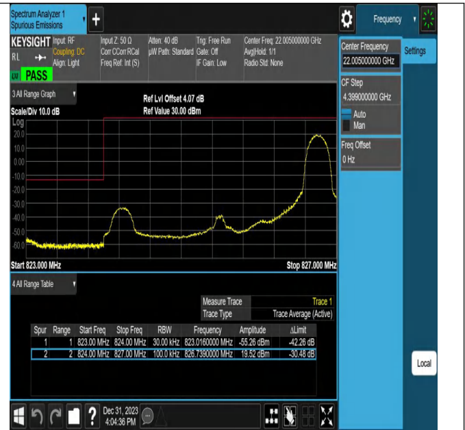
Band26_3MHz_QPSK_26805_1RB#14
