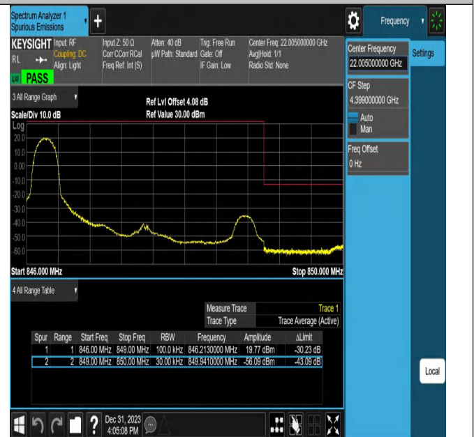
Band26_3MHz_QPSK_27025_1RB#0
