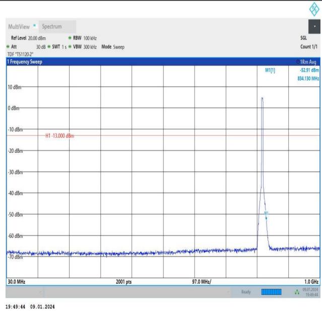
Band26_5MHz_16QAM_26765_25RB#0_30~1000_30~1000
