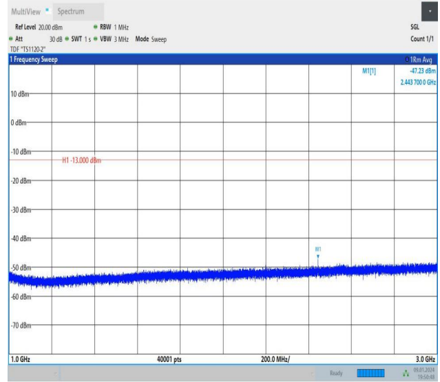
Band26_10MHz_QPSK_26740_1RB#0_1000~3000_1000~300 0
