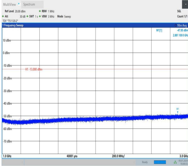
Band26_5MHz_16QAM_26765_25RB#0_1000~3000_1000~3000
