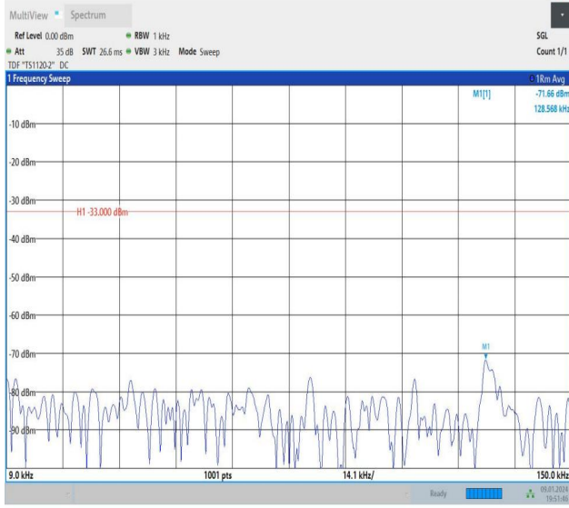
Band26_10MHz_QPSK_26740_1RB#49_0.009~0.15_0.009~0.15
