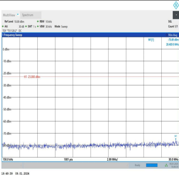
Band26_5MHz_16QAM_26765_25RB#0_0.15~30_0.15~30
