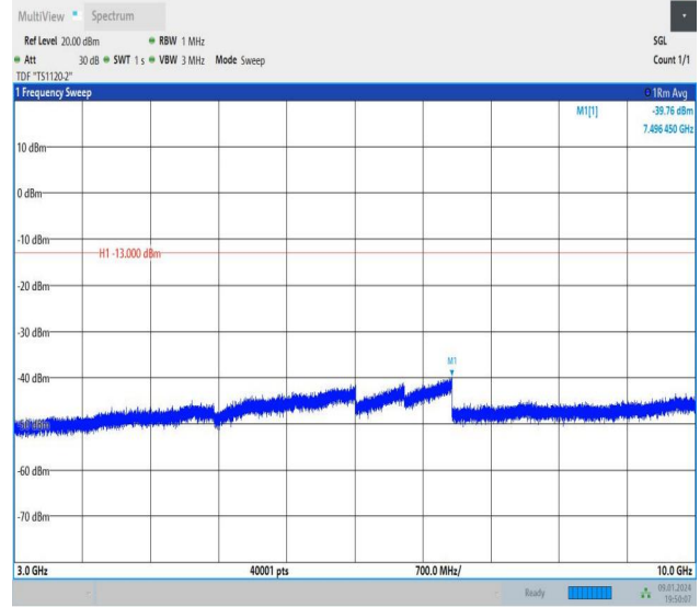
Band26_5MHz_16QAM_26765_25RB#0_3000~10000_3000~10000
