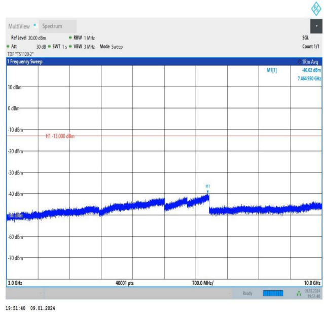
Band26_10MHz_16QAM_26740_1RB#0_3000~10000_3000~10000
