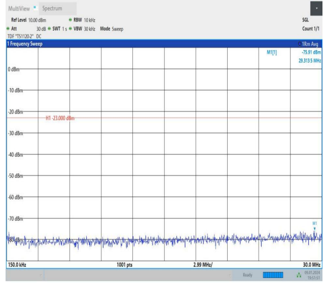
Band26_10MHz_QPSK_26740_1RB#49_0.15~30_0.15~30
