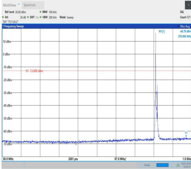
Band26_10MHz_QPSK_26740_1RB#0_30~1000_30~1000
