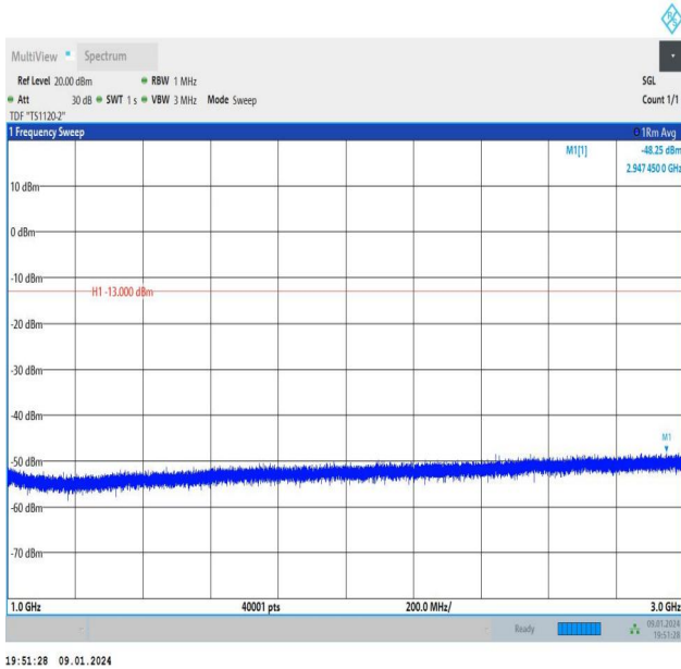
Band26_10MHz_16QAM_26740_1RB#0_1000~3000_1000~3000
