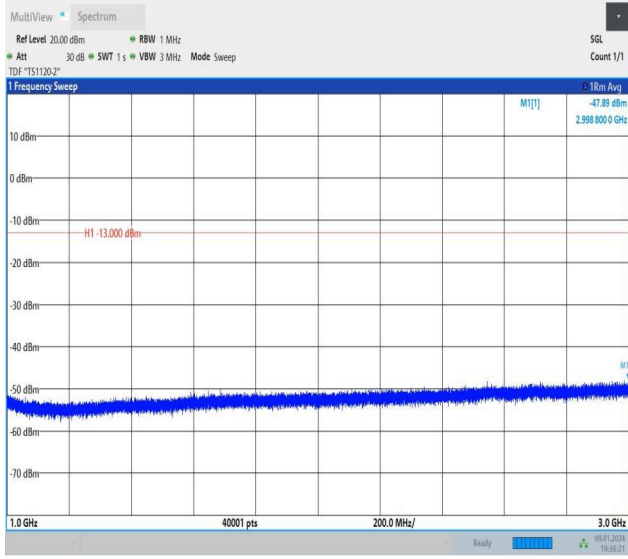
Band26_3MHz_16QAM_26775_1RB#14_1000~3000_1000~3000
