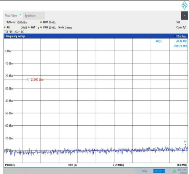
Band26_5MHz_QPSK_26765_1RB#24_0.15~30_0.15~30
