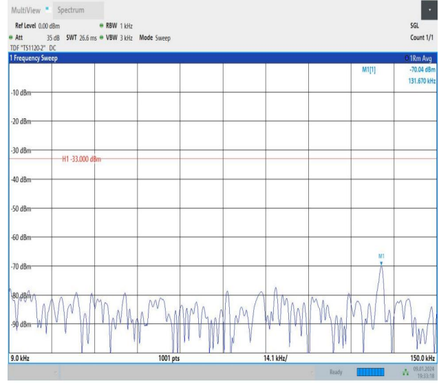
Band26_3MHz_16QAM_26740_15RB#0_0.009~0.15_0.009~0.15
