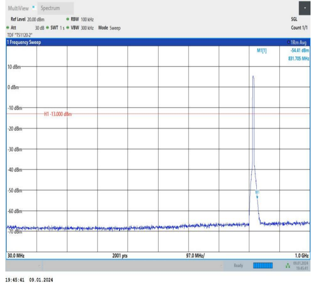
Band26_5MHz_16QAM_26740_25RB#0_30~1000_30~1000
