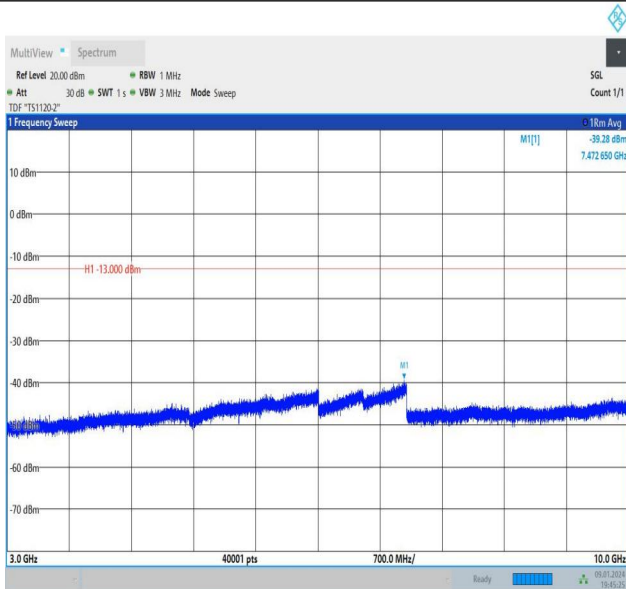
Band26_5MHz_QPSK_26740_25RB#0_3000~10000_3000~1 0000
