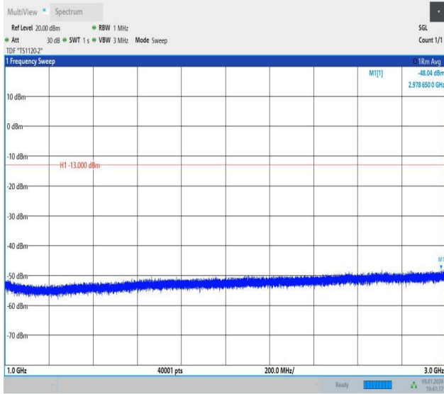
Band26_5MHz_16QAM_26765_1RB#0_1000~3000_1000~30
