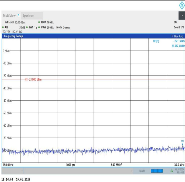
Band26_3MHz_16QAM_26775_1RB#14_0.15~30_0.15~30
