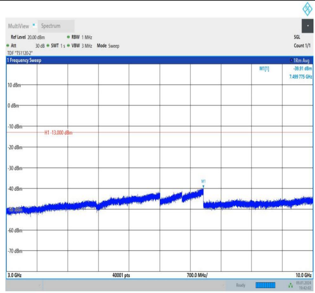
Band26_5MHz_16QAM_26715_25RB#0_3000~10000_3000~10000
