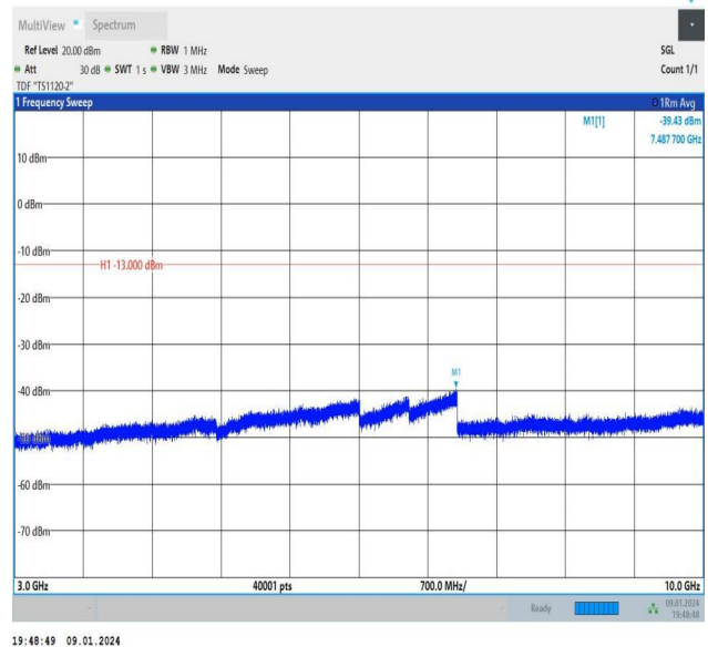
Band26_5MHz_16QAM_26765_1RB#24_3000~10000_3000~10000
