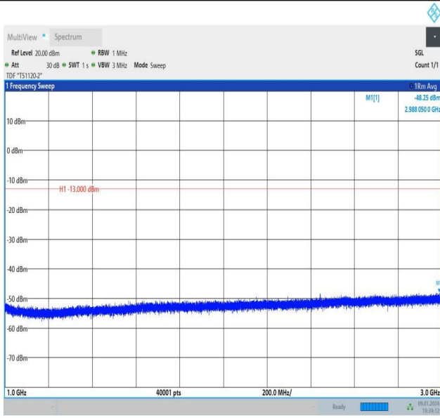
Band26_5MHz_16QAM_26715_1RB#0_1000~3000_1000~3000
