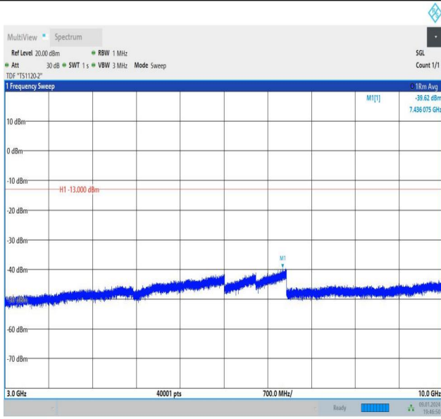
Band26_5MHz_QPSK_26765_1RB#0_3000~10000_3000~10000
