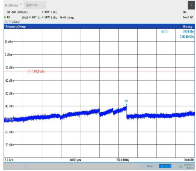
Band26_3MHz_16QAM_26775_1RB#14_3000~10000_3000~10000
