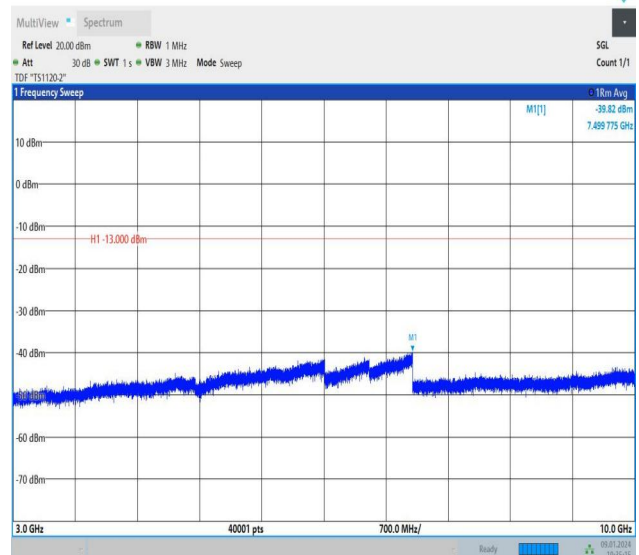
Band26_3MHz_16QAM_26775_1RB#0_3000~10000_3000~10
