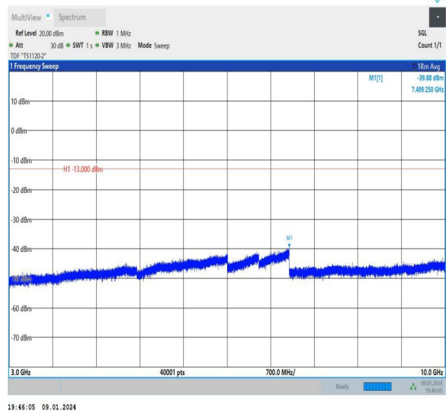
Band26_5MHz_16QAM_26740_25RB#0_3000~10000_3000~10000
