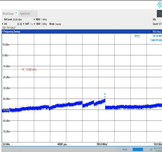
Band26_5MHz_QPSK_26765_1RB#24_3000~10000_3000~1
