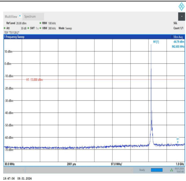
Band26_5MHz_16QAM_26765_1RB#0_30~1000_30~1000
