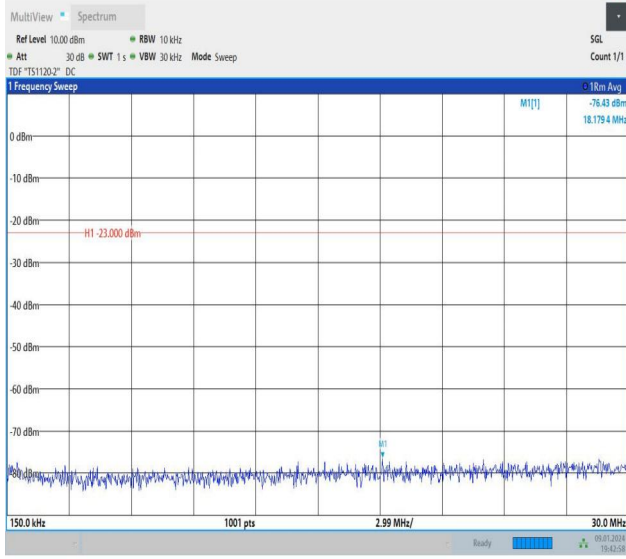
Band26_5MHz_16QAM_26740_1RB#0_0.15~30_0.15~30
