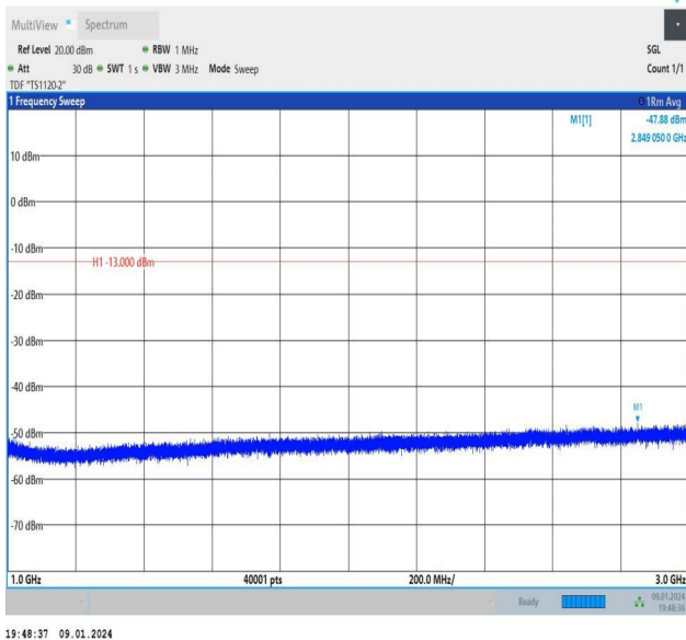
Band26_5MHz_16QAM_26765_1RB#24_1000~3000_1000~3000
