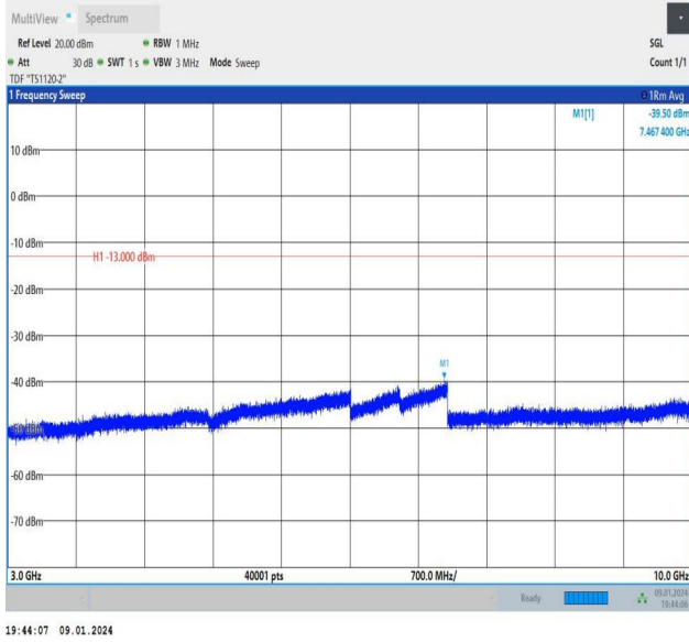
Band26_5MHz_QPSK_26740_1RB#24_3000~10000_3000~10000
