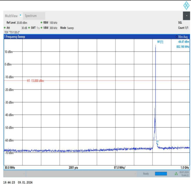
Band26_5MHz_16QAM_26740_1RB#24_30~1000_30~1000
