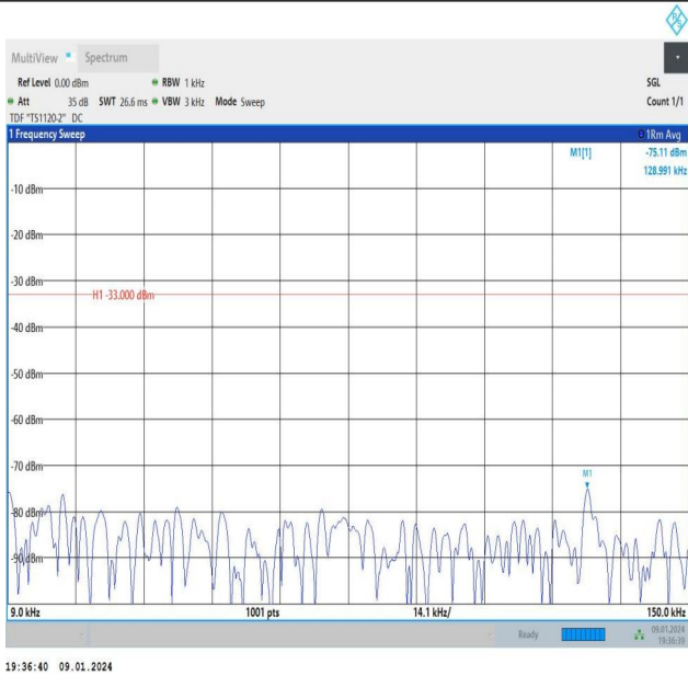
Band26_3MHz_QPSK_26775_15RB#0_0.009~0.15_0.009~0.15
