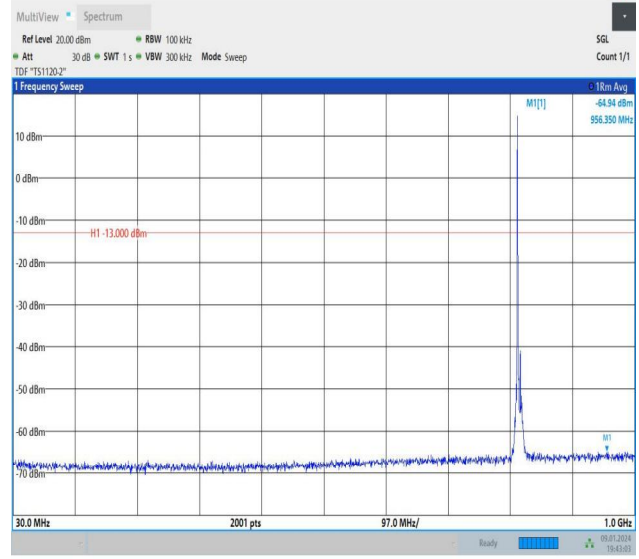
Band26_5MHz_16QAM_26740_1RB#0_30~1000_30~1000
