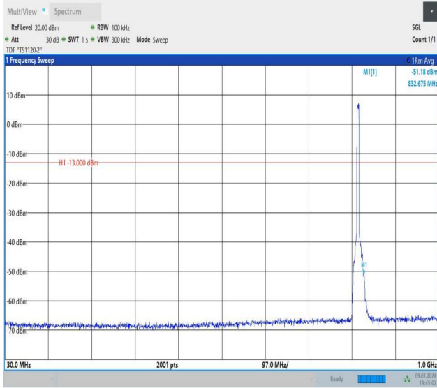
Band26_5MHz_QPSK_26740_25RB#0_30~1000_30~1000
