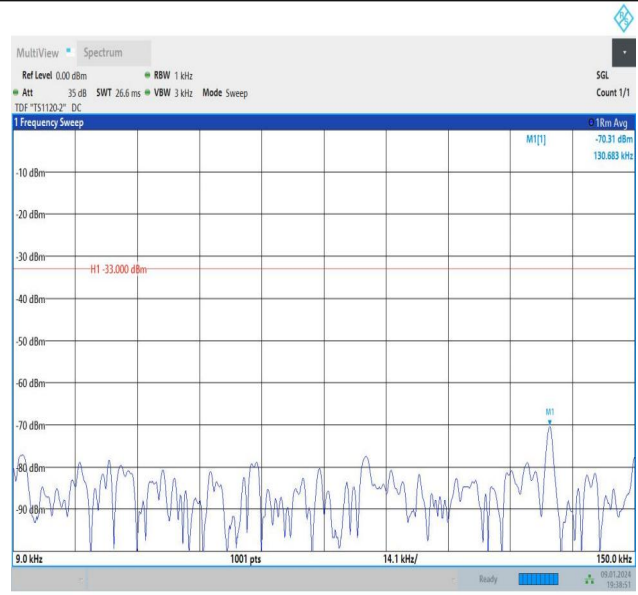
Band26_5MHz_16QAM_26715_1RB#0_0.009~0.15_0.009~0.15
