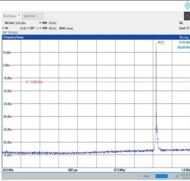
Band26_3MHz_QPSK_26775_1RB#0_30~1000_30~1000
