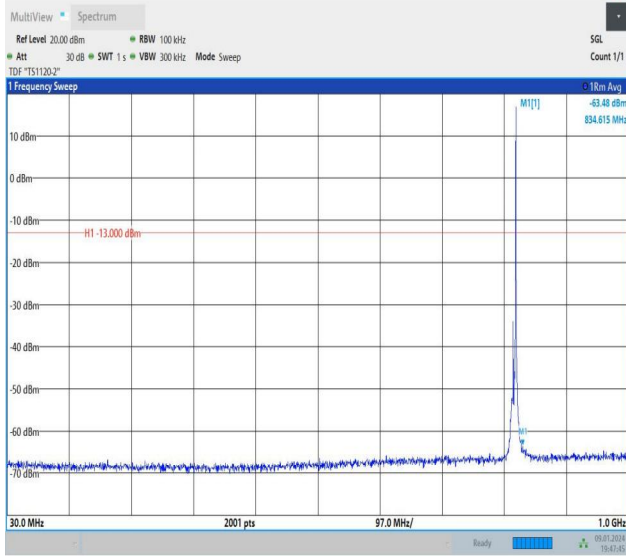
Band26_5MHz_QPSK_26765_1RB#24_30~1000_30~1000
