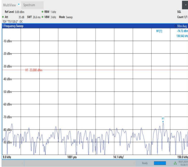
Band26_5MHz_QPSK_26715_1RB#0_0.009~0.15_0.009~0.1
