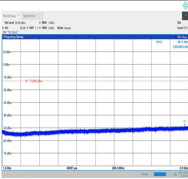
Band26_5MHz_16QAM_26715_25RB#0_1000~3000_1000~3000
