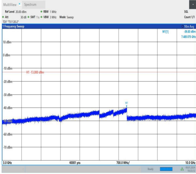
Band26_3MHz_QPSK_26740_15RB#0_3000~10000_3000~10000
