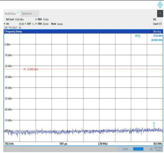
Band26_5MHz_QPSK_26765_1RB#0_0.15~30_0.15~30
