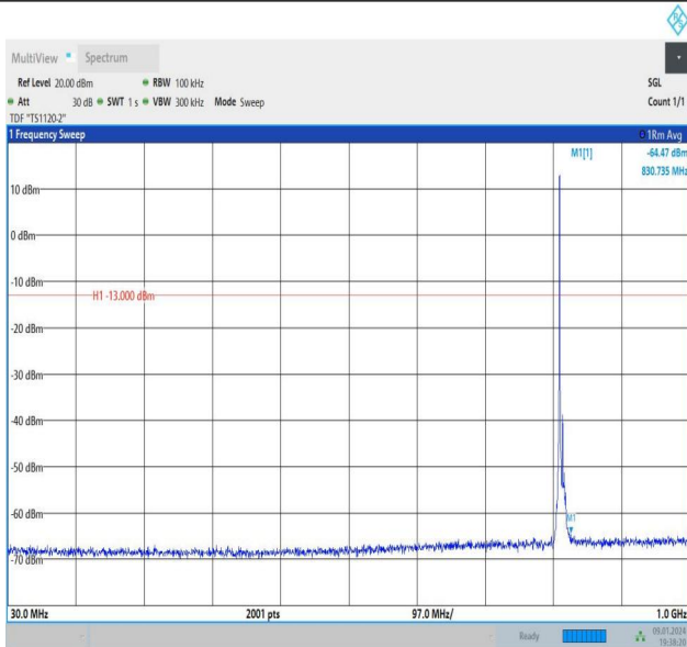
Band26_5MHz_QPSK_26715_1RB#0_30~1000_30~1000
