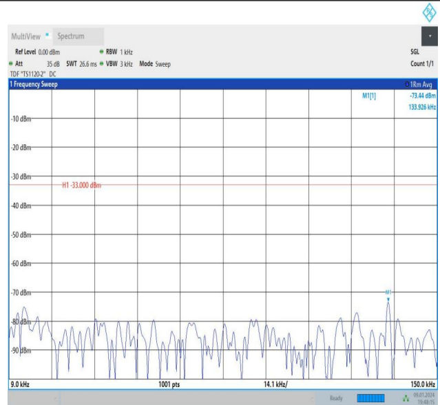
Band26_5MHz_16QAM_26765_1RB#24_0.009~0.15_0.009~0.
