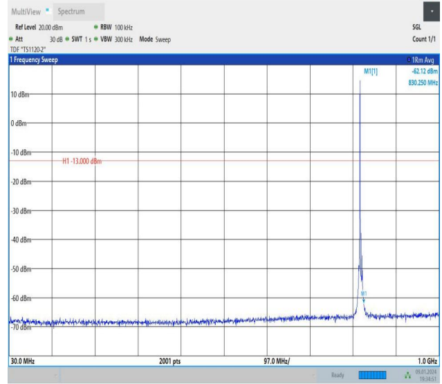
Band26_3MHz_16QAM_26775_1RB#0_30~1000_30~1000
