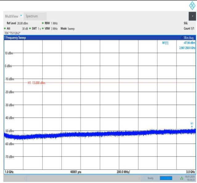
Band26_3MHz_QPSK_26775_1RB#0_1000~3000_1000~3000
