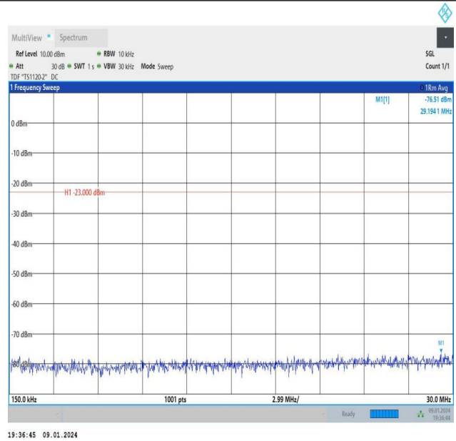
Band26_3MHz_QPSK_26775_15RB#0_0.15~30_0.15~30
