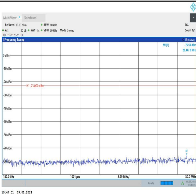
Band26_5MHz_16QAM_26765_1RB#0_0.15~30_0.15~30
