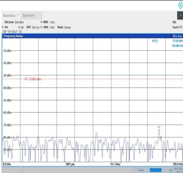
Band26_5MHz_QPSK_26765_1RB#24_0.009~0.15_0.009~0.
