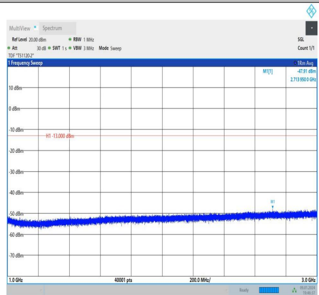
Band26_5MHz_QPSK_26765_1RB#0_1000~3000_1000~3000
