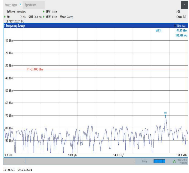
Band26_3MHz_16QAM_26775_1RB#14_0.009~0.15_0.009~0.15
