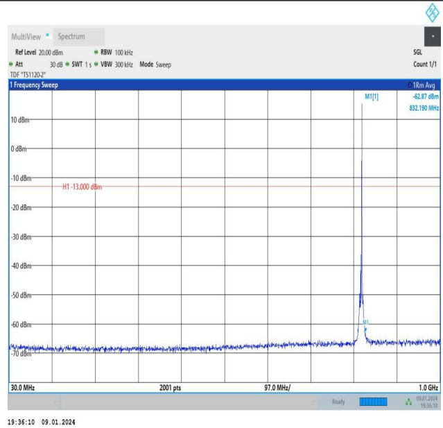
Band26_3MHz_16QAM_26775_1RB#14_30~1000_30~1000
