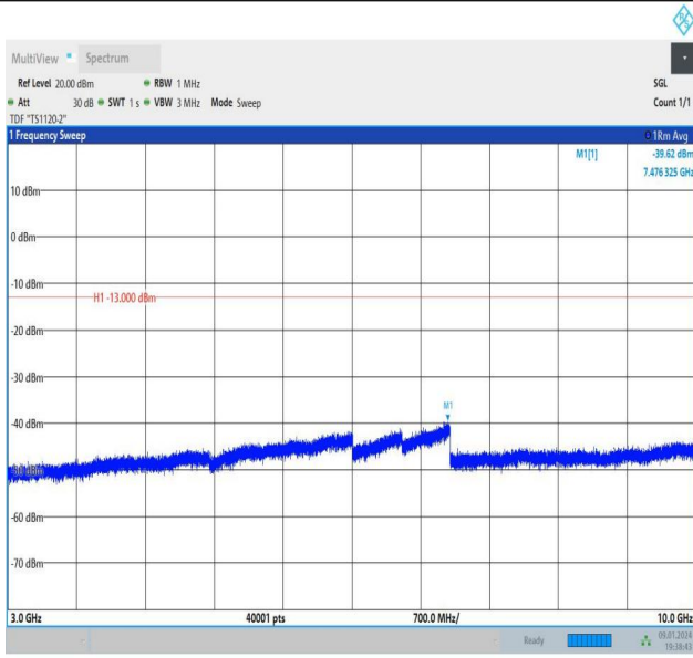
Band26_5MHz_QPSK_26715_1RB#0_3000~10000_3000~10000
