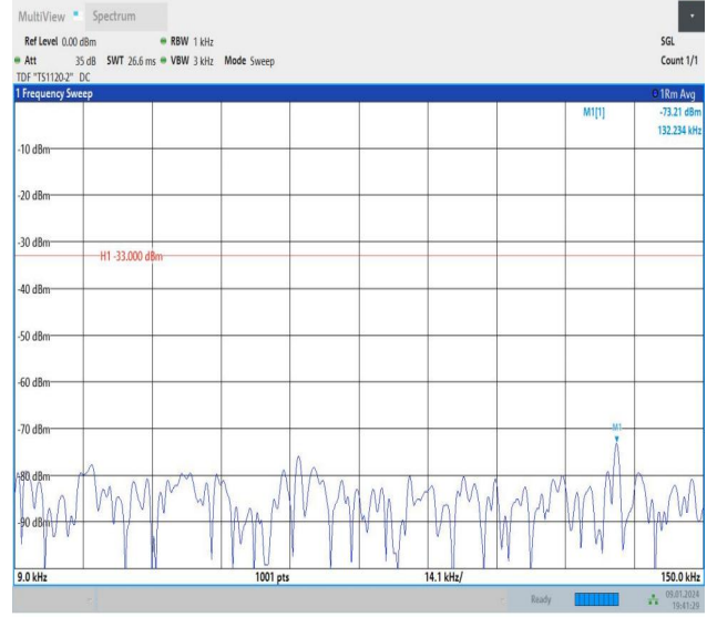
Band26_5MHz_16QAM_26715_25RB#0_0.009~0.15_0.009~0.15
