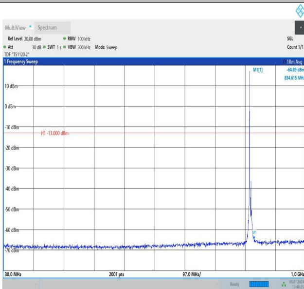
Band26_5MHz_QPSK_26765_1RB#0_30~1000_30~1000
