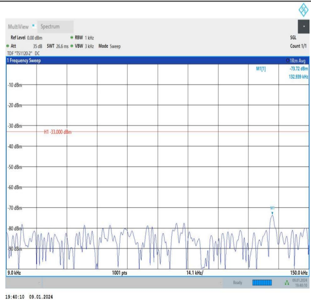
Band26_5MHz_16QAM_26715_1RB#24_0.009~0.15_0.009~0. 15
