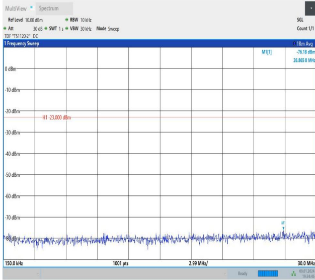
Band26_3MHz_16QAM_26775_1RB#0_0.15~30_0.15~30
