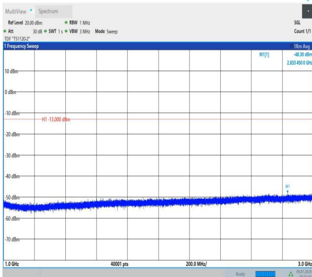
Band26_3MHz_16QAM_26775_1RB#0_1000~3000_1000~30
