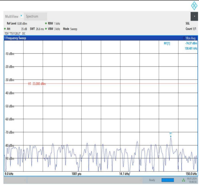
Band26_5MHz_16QAM_26765_1RB#0_0.009~0.15_0.009~0.15
