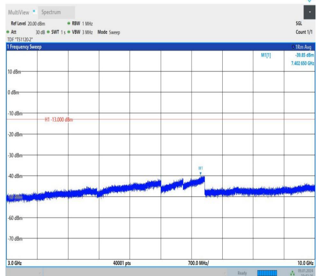
Band26_5MHz_16QAM_26740_1RB#0_3000~10000_3000~10000 000
