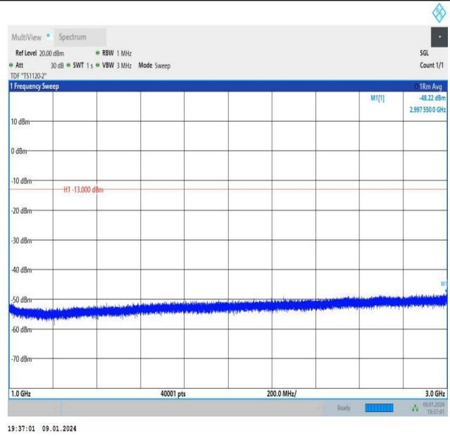
Band26_3MHz_QPSK_26775_15RB#0_1000~3000_1000~300 0
