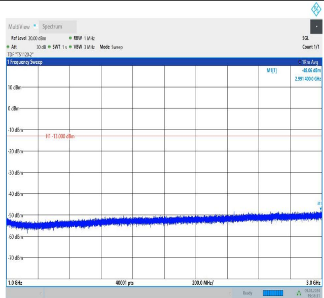
Band26_5MHz_QPSK_26715_1RB#0_1000~3000_1000~3000
