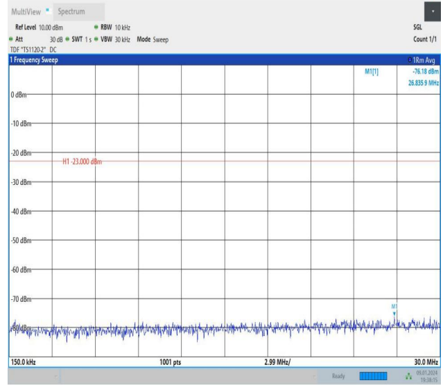
Band26_5MHz_QPSK_26715_1RB#0_0.15~30_0.15~30
