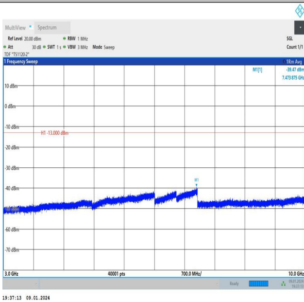
Band26_3MHz_QPSK_26775_15RB#0_3000~10000_3000~1 0000
