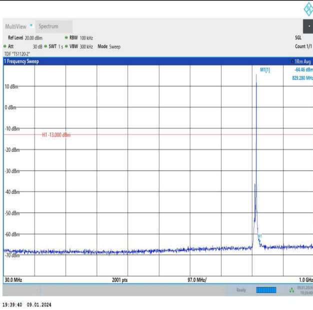
Band26_5MHz_QPSK_26715_1RB#24_30~1000_30~1000
