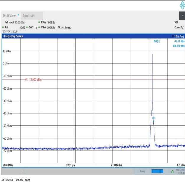
Band26_3MHz_QPSK_26775_15RB#0_30~1000_30~1000
