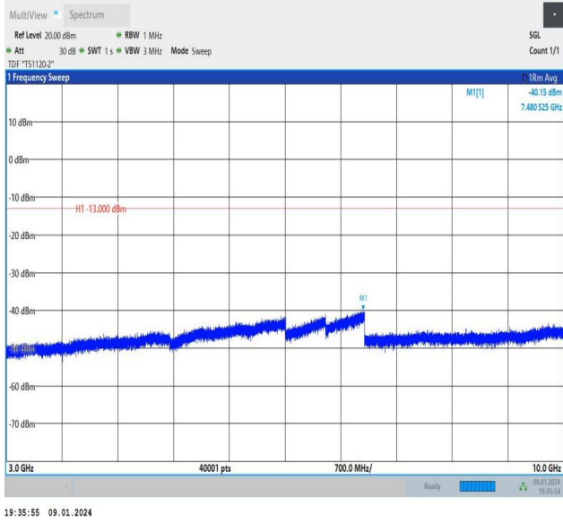
Band26_3MHz_QPSK_26775_1RB#14_3000~10000_3000~10000
