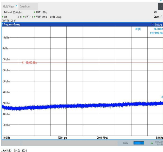
Band26_5MHz_16QAM_26740_25RB#0_1000~3000_1000~3000
