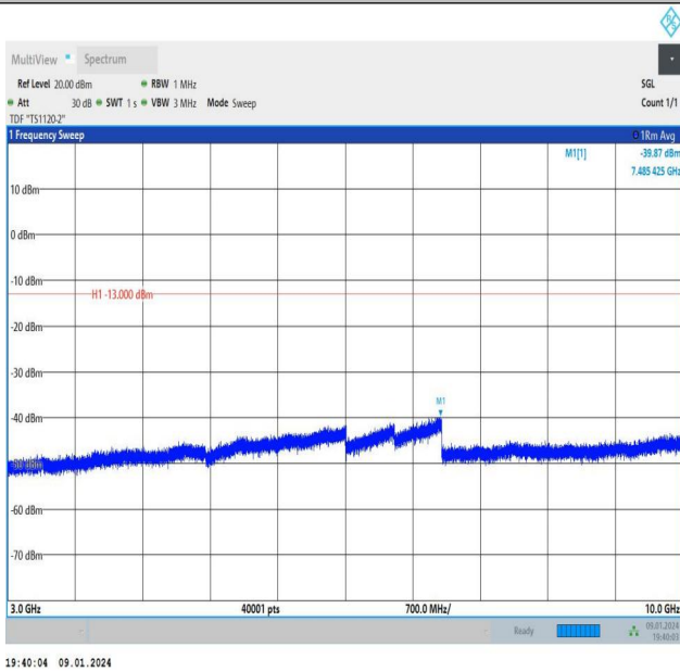
Band26_5MHz_QPSK_26715_1RB#24_3000~10000_3000~1 0000
