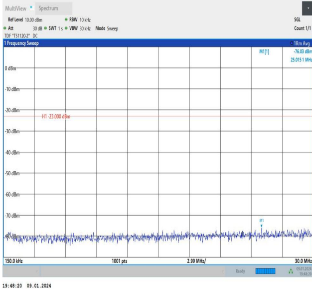
Band26_5MHz_16QAM_26765_1RB#24_0.15~30_0.15~30
