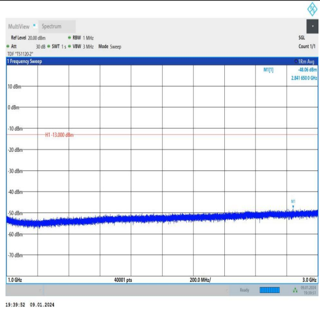
Band26_5MHz_QPSK_26715_1RB#24_1000~3000_1000~300 0
