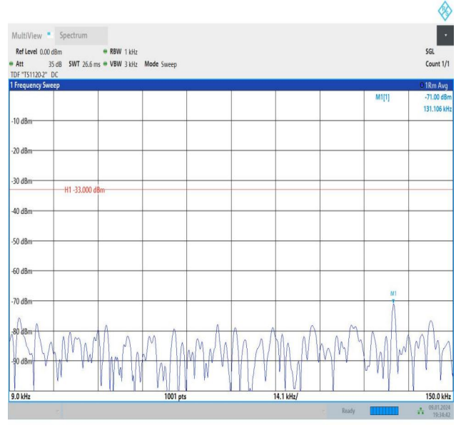
Band26_3MHz_16QAM_26775_1RB#0_0.009~0.15_0.009~0.1
