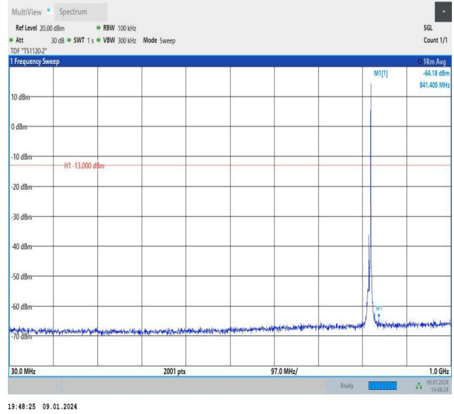
Band26_5MHz_16QAM_26765_1RB#24_30~1000_30~1000
