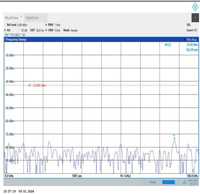
Band26_3MHz_16QAM_26775_15RB#0_0.009~0.15_0.009~0. 15
