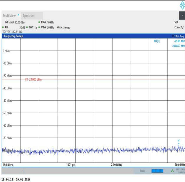
Band26_5MHz_16QAM_26740_1RB#24_0.15~30_0.15~30
