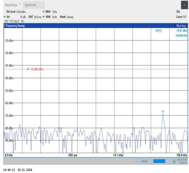
Band26_5MHz_16QAM_26740_1RB#24_0.009~0.15_0.009~0.15
