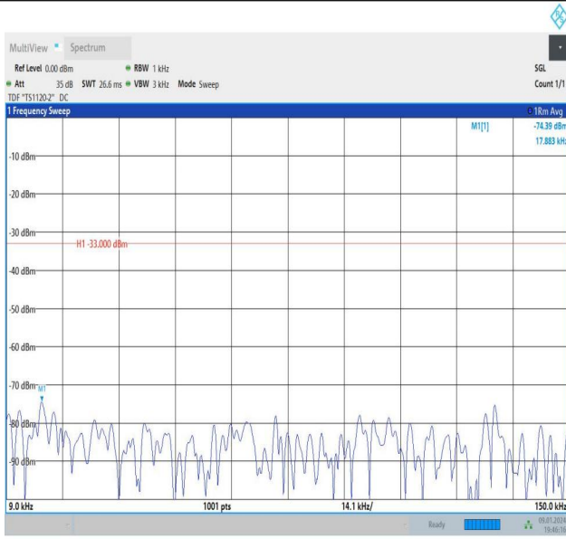
Band26_5MHz_QPSK_26765_1RB#0_0.009~0.15_0.009~0.1
