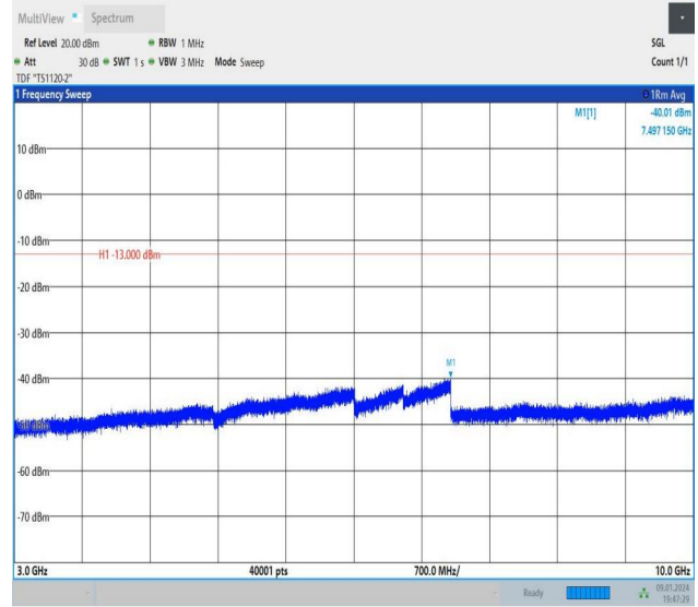
Band26_5MHz_16QAM_26765_1RB#0_3000~10000_3000~10
