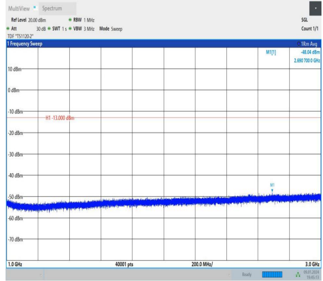
Band26_5MHz_QPSK_26740_25RB#0_1000~3000_1000~300 0
