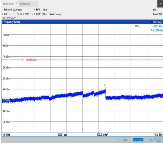
Band26_5MHz_QPSK_26715_25RB#0_3000~10000_3000~10000
