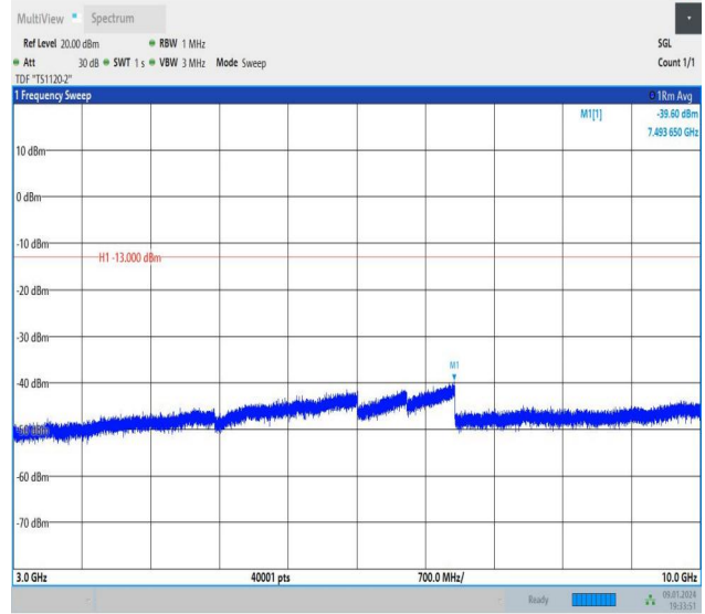
Band26_3MHz_16QAM_26740_15RB#0_3000~10000_3000~10000
