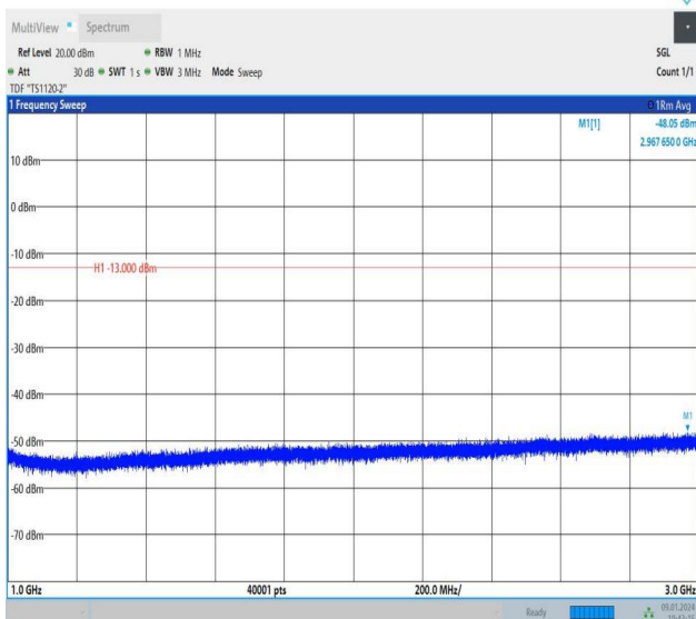
Band26_5MHz_16QAM_26740_1RB#0_1000~3000_1000~3000 00
