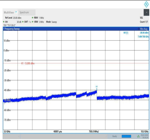
Band26_5MHz_16QAM_26715_1RB#0_3000~10000_3000~10000
