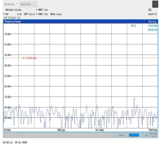
Band26_1.4MHz_16QAM_26783_1RB#0_0.009~0.15_0.009~0.15
