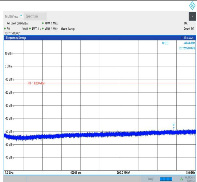
Band26_1.4MHz_QPSK_26783_1RB#0_1000~3000_1000~3000
