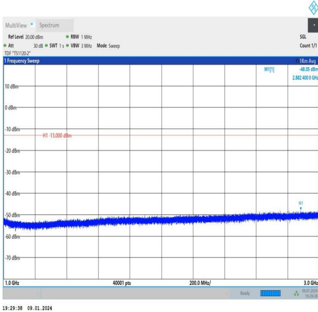
Band26_3MHz_16QAM_26705_15RB#0_1000~3000_1000~3000
