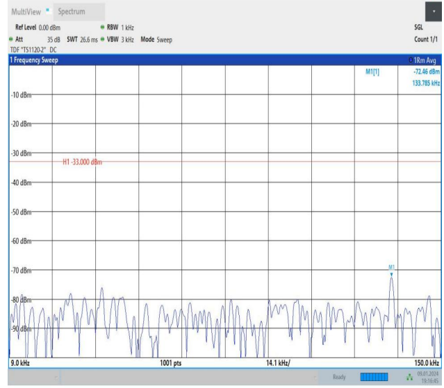
Band26_1.4MHz_16QAM_26697_6RB#0_0.009~0.15_0.009~0.15
