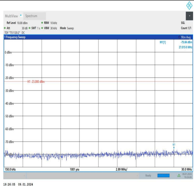
Band26_3MHz_QPSK_26705_1RB#0_0.15~30_0.15~30
