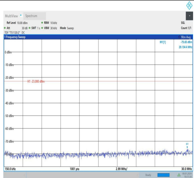
Band26_1.4MHz_16QAM_26697_6RB#0_3000~10000_3000~10000
