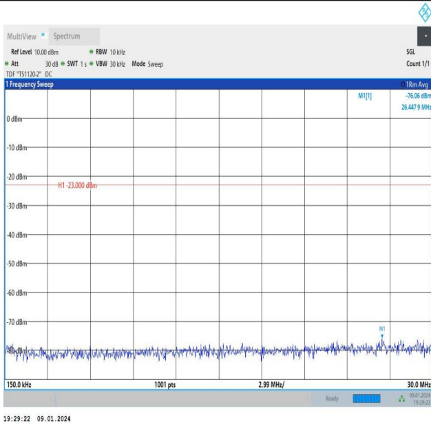
Band26_3MHz_16QAM_26705_15RB#0_0.15~30_0.15~30
