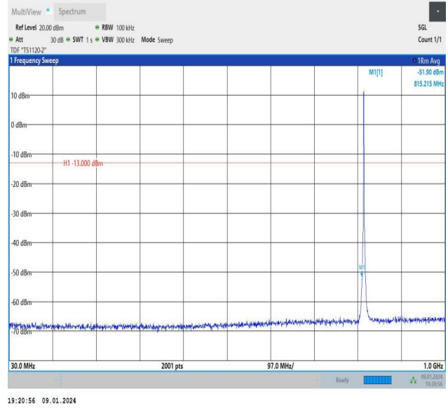
Band26_1.4MHz_16QAM_26740_6RB#0_30~1000_30~1000
