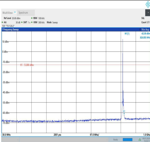
Band26_3MHz_QPSK_26740_1RB#0_30~1000_30~1000
