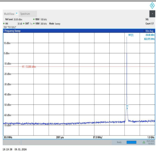
Band26_1.4MHz_16QAM_26740_1RB#5_30~1000_30~1000
