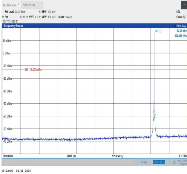
Band26_1.4MHz_QPSK_26783_1RB#5_30~1000_30~1000
