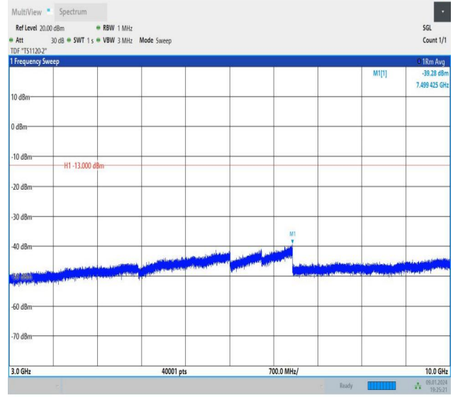
Band26_1.4MHz_16QAM_26783_6RB#0_3000~10000_3000~10000
