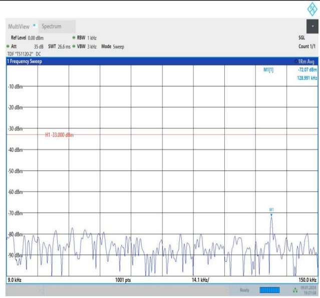
Band26_3MHz_16QAM_26705_1RB#14_0.009~0.15_0.009~0.15
