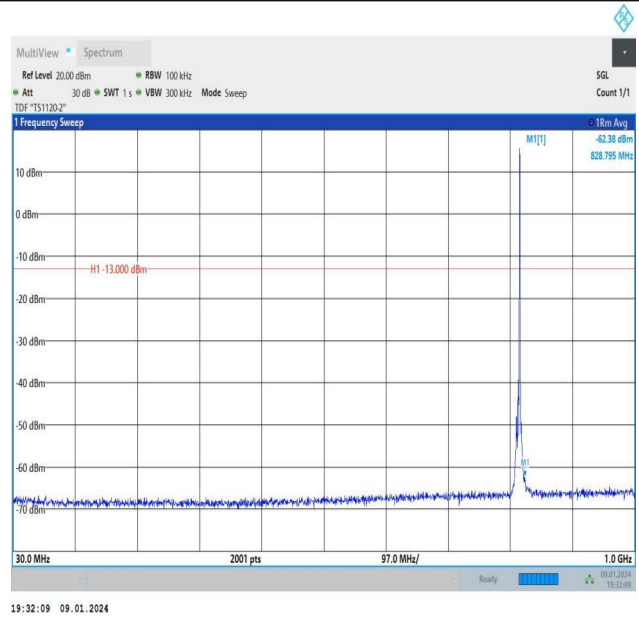
Band26_3MHz_16QAM_26740_1RB#14_30~1000_30~1000
