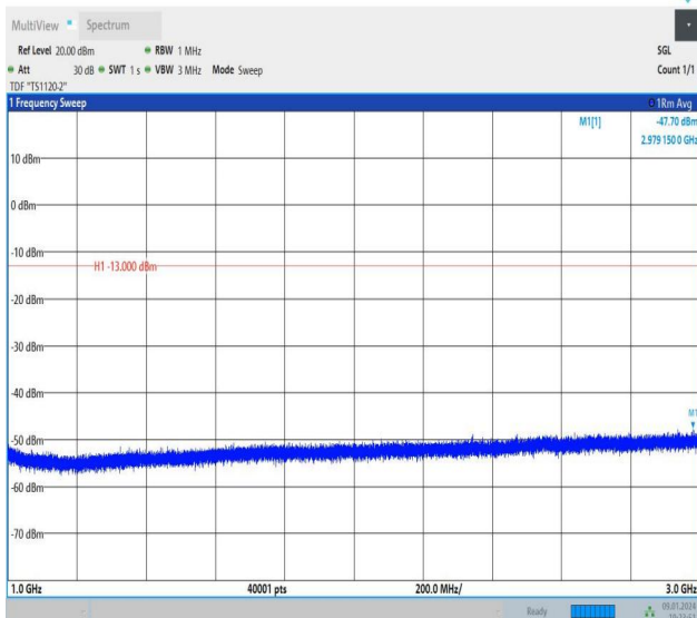
Band26_1.4MHz_16QAM_26783_1RB#5_1000~3000_1000~3000
