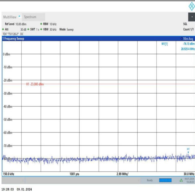
Band26_3MHz_16QAM_26705_1RB#14_0.15~30_0.15~30
