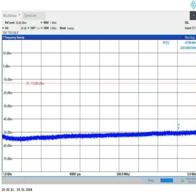
Band26_3MHz_16QAM_26740_1RB#14_1000~3000_1000~3000
