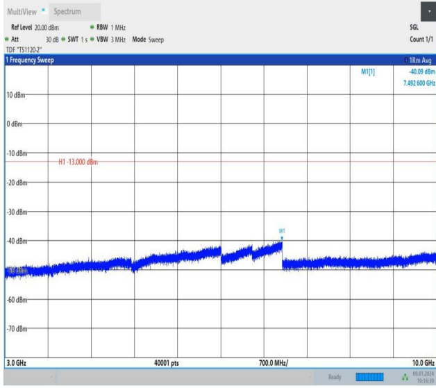
Band26_1.4MHz_QPSK_26697_6RB#0_3000~10000_3000~10000
