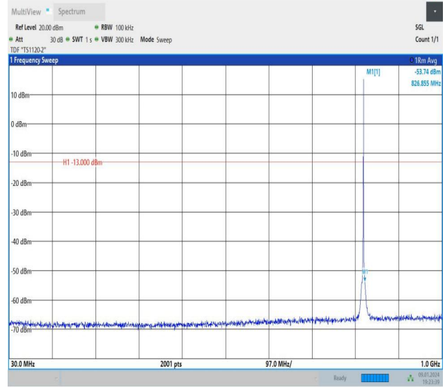
Band26_1.4MHz_16QAM_26783_1RB#5_30~1000_30~1000
