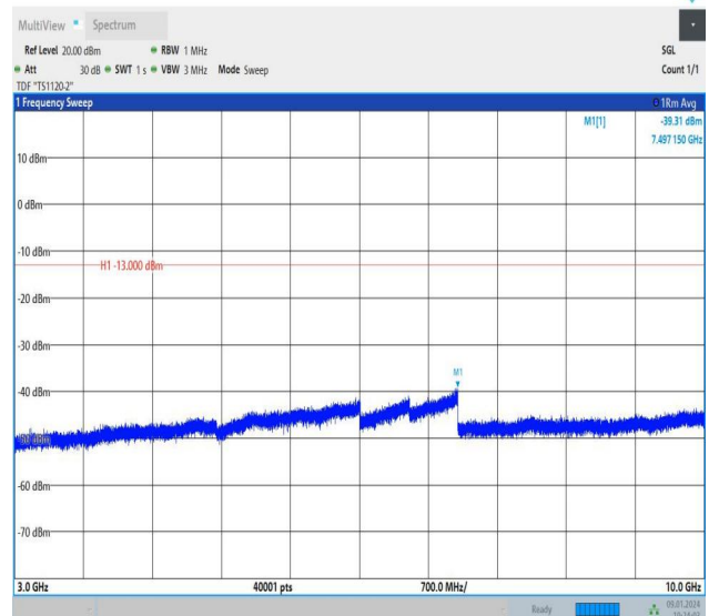
Band26_1.4MHz_16QAM_26783_1RB#5_3000~10000_3000~10000
