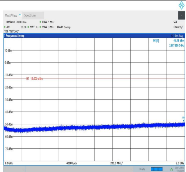
Band26_3MHz_QPSK_26740_1RB#0_1000~3000_1000~3000
