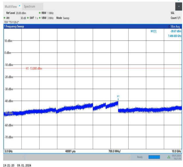
Band26_1.4MHz_16QAM_26740_6RB#0_3000~10000_3000~10000
