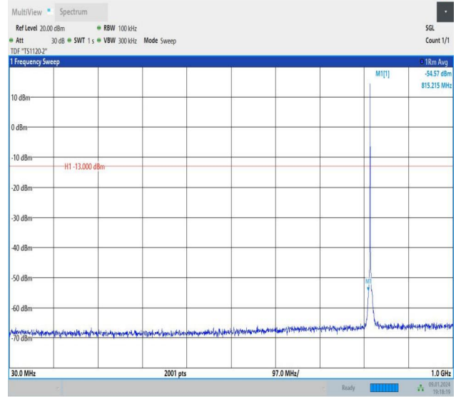
Band26_1.4MHz_16QAM_26740_1RB#0_30~1000_30~1000
