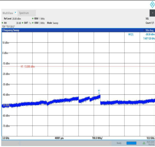
Band26_3MHz_QPSK_26705_1RB#14_3000~10000_3000~10000
