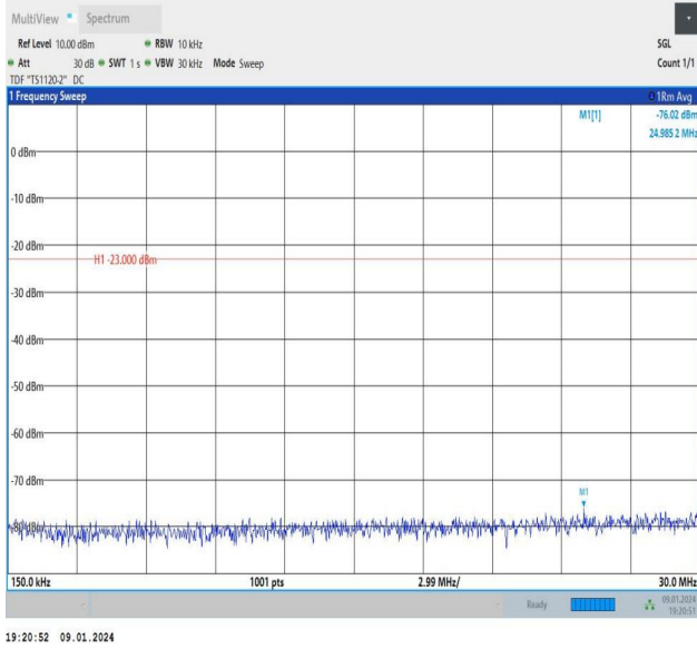
Band26_1.4MHz_16QAM_26740_6RB#0_0.15~30_0.15~30
