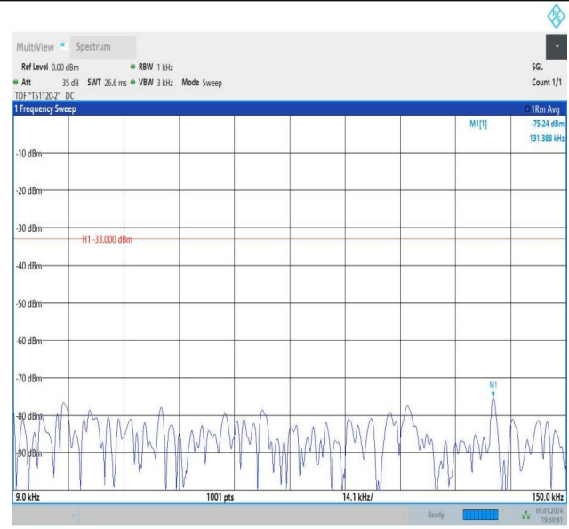
Band26_3MHz_16QAM_26740_1RB#0_0.009~0.15_0.009~0.15
