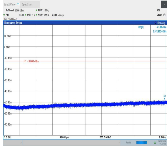
Band26_1.4MHz_QPSK_26740_1RB#0_1000~3000_1000~3000
