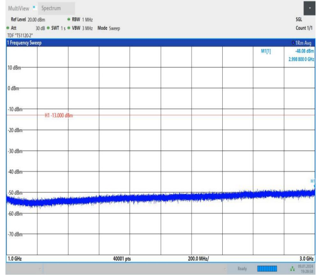
Band26_3MHz_QPSK_26705_15RB#0_1000~3000_1000~300 0
