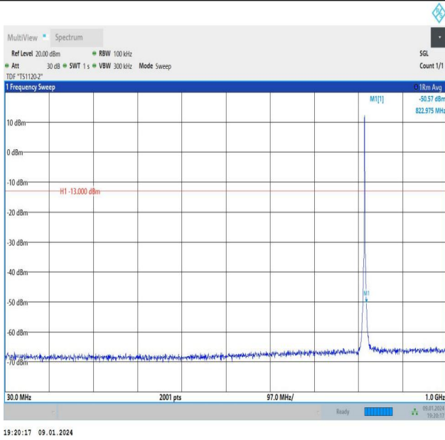
Band26_1.4MHz_QPSK_26740_6RB#0_30~1000_30~1000
