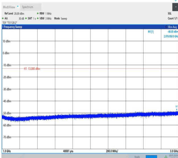
Band26_1.4MHz_16QAM_26740_1RB#0_1000~3000_1000~3000
