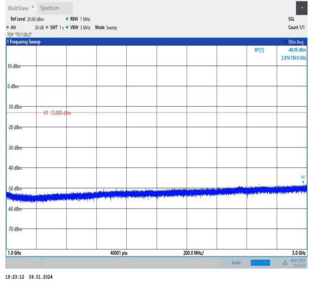
Band26_1.4MHz_QPSK_26783_1RB#5_1000~3000_1000~3000
