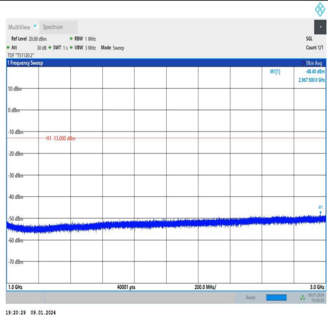
Band26_1.4MHz_QPSK_26740_6RB#0_1000~3000_1000~3000
