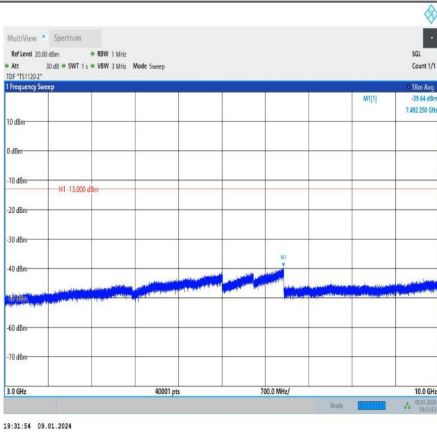
Band26_3MHz_QPSK_26740_1RB#14_3000~10000_3000~1 0000
