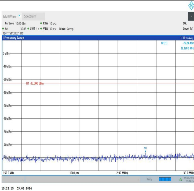
Band26_1.4MHz_16QAM_26783_1RB#0_0.15~30_0.15~30
