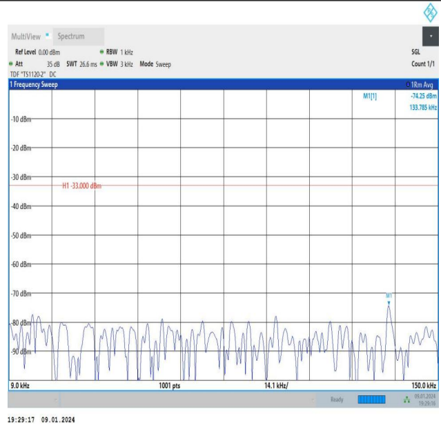
Band26_3MHz_16QAM_26705_15RB#0_0.009~0.15_0.009~0. 15
