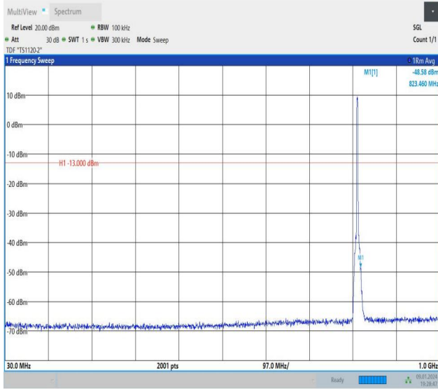
Band26_3MHz_QPSK_26705_15RB#0_30~1000_30~1000
