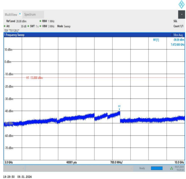
Band26_3MHz_16QAM_26705_15RB#0_3000~10000_3000~10000
