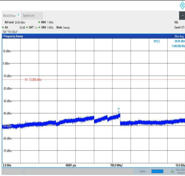
Band26_1.4MHz_QPSK_26740_1RB#5_3000~10000_3000~10000
