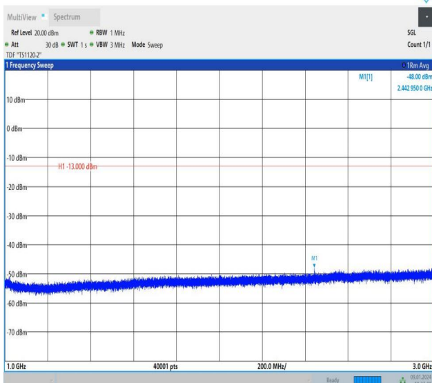
Band26_3MHz_16QAM_26705_1RB#0_1000~3000_1000~3000
