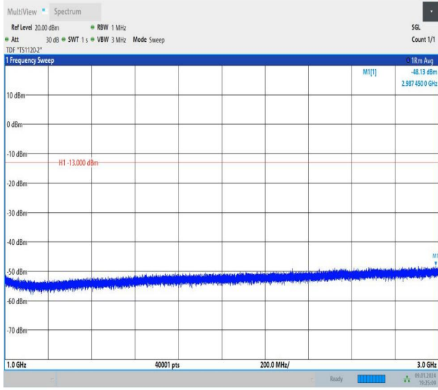
Band26_1.4MHz_16QAM_26783_6RB#0_1000~3000_1000~3000
