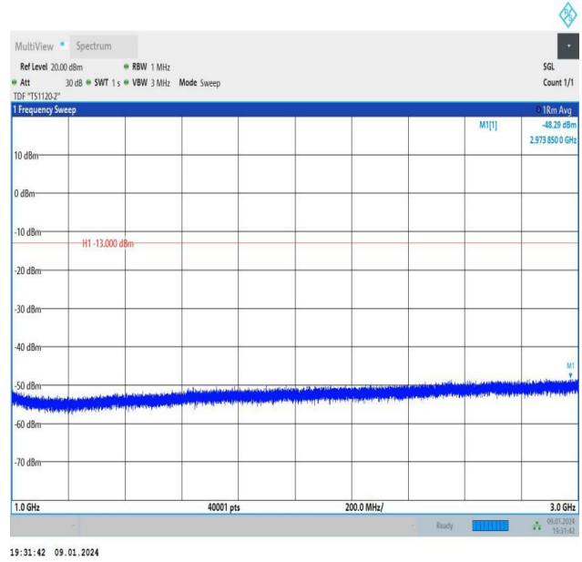
Band26_3MHz_QPSK_26740_1RB#14_1000~3000_1000~300 0
