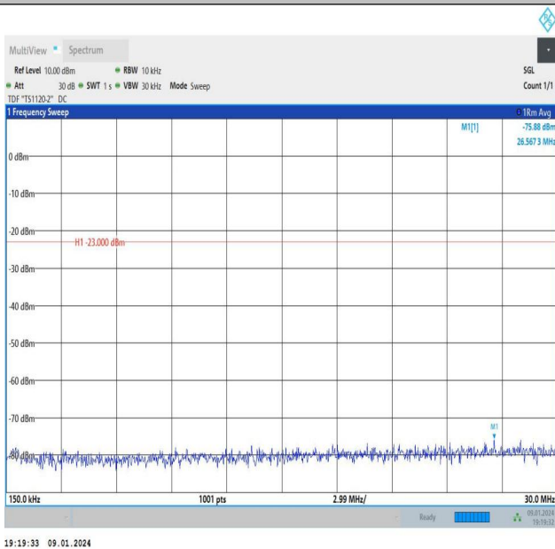
Band26_1.4MHz_16QAM_26740_1RB#5_0.15~30_0.15~30
