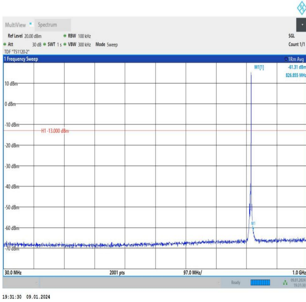
Band26_3MHz_QPSK_26740_1RB#14_30~1000_30~1000
