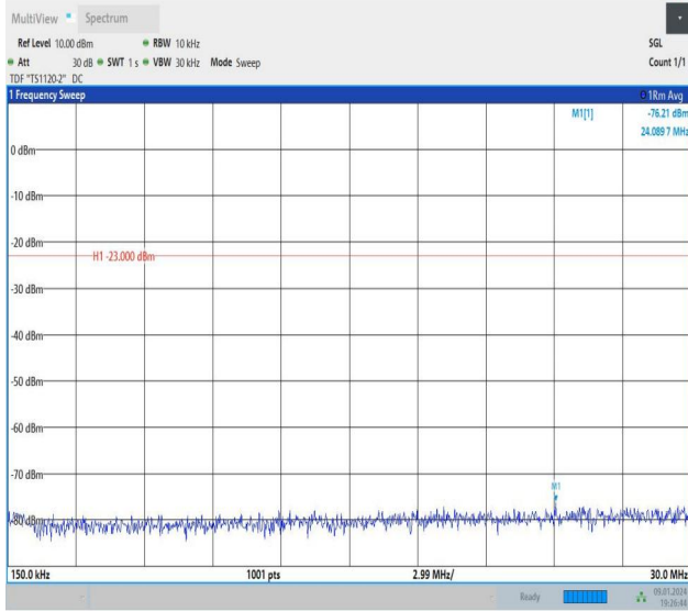
Band26_3MHz_16QAM_26705_1RB#0_0.15~30_0.15~30
