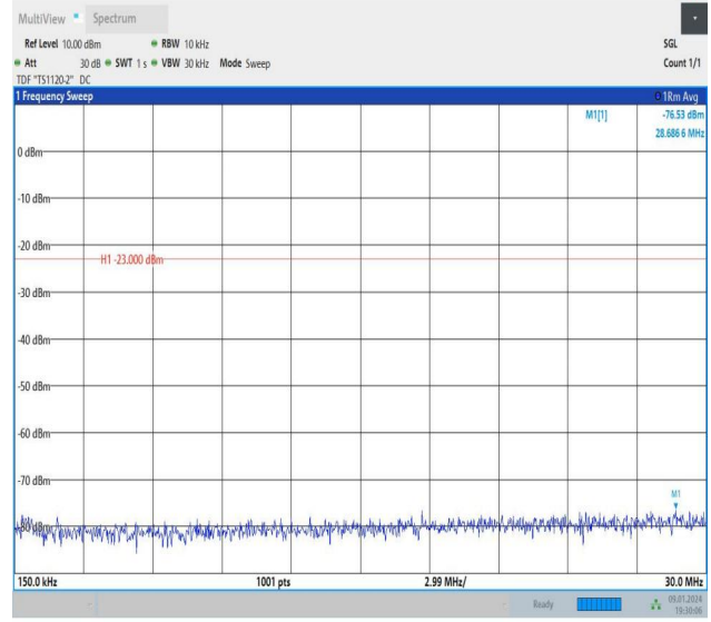
Band26_3MHz_QPSK_26740_1RB#0_0.15~30_0.15~30
