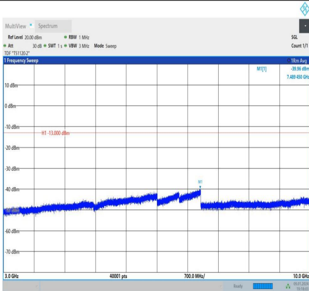
Band26_1.4MHz_QPSK_26740_1RB#0_3000~10000_3000~10000
