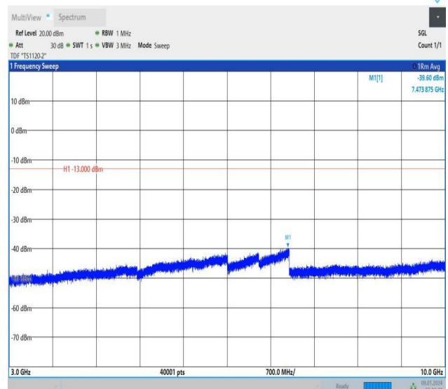
Band26_1.4MHz_16QAM_26740_1RB#0_3000~10000_3000~10000
