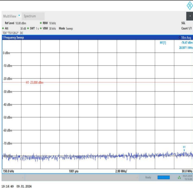
Band26_1.4MHz_16QAM_26697_6RB#0_0.15~30_0.15~30
