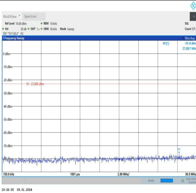
Band26_3MHz_16QAM_26740_1RB#14_0.15~30_0.15~30
