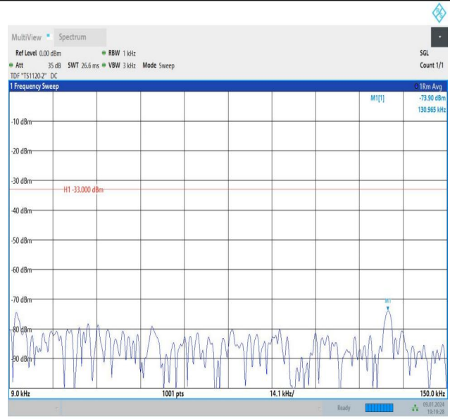
Band26_1.4MHz_16QAM_26740_1RB#5_0.009~0.15_0.009~0.15
