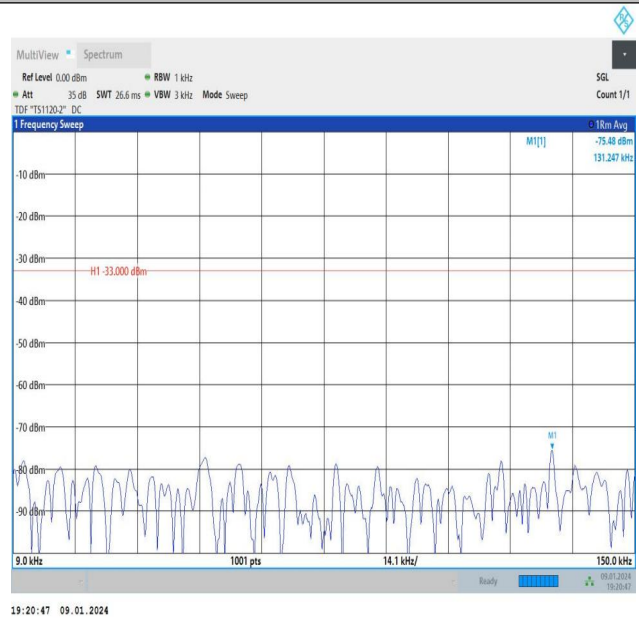
Band26_1.4MHz_16QAM_26740_6RB#0_0.009~0.15_0.009~0.15
