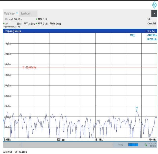
Band26_3MHz_16QAM_26740_1RB#14_0.009~0.15_0.009~0. 15
