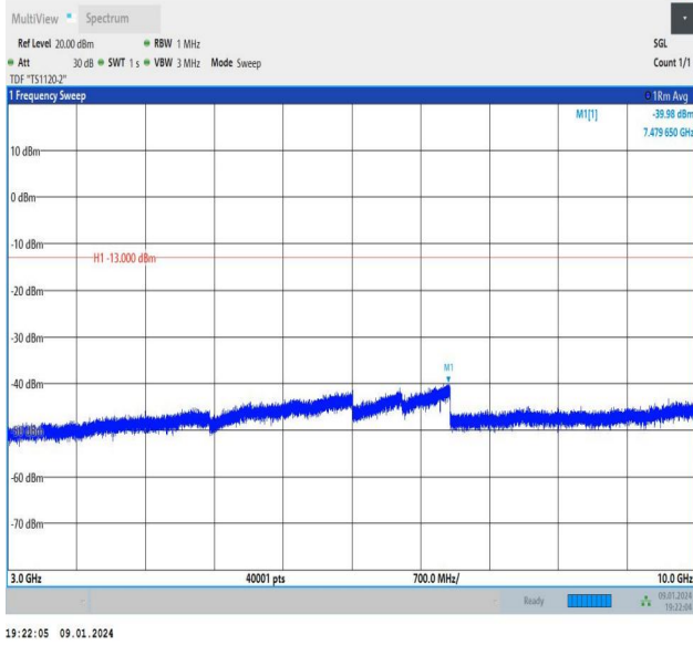
Band26_1.4MHz_QPSK_26783_1RB#0_3000~10000_3000~10000
