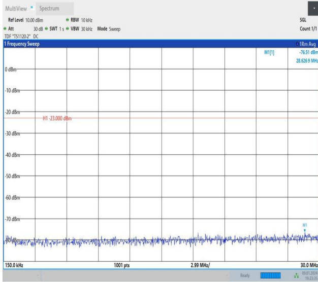
Band26_1.4MHz_16QAM_26783_1RB#5_0.15~30_0.15~30
