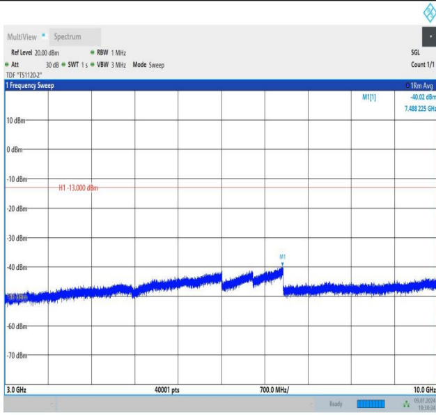
Band26_3MHz_QPSK_26740_1RB#0_3000~10000_3000~10000
