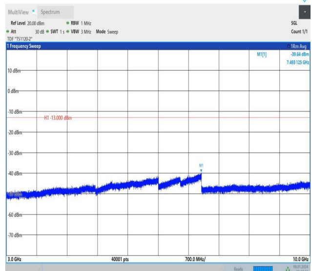
Band26_3MHz_16QAM_26705_1RB#0_3000~10000_3000~10000
