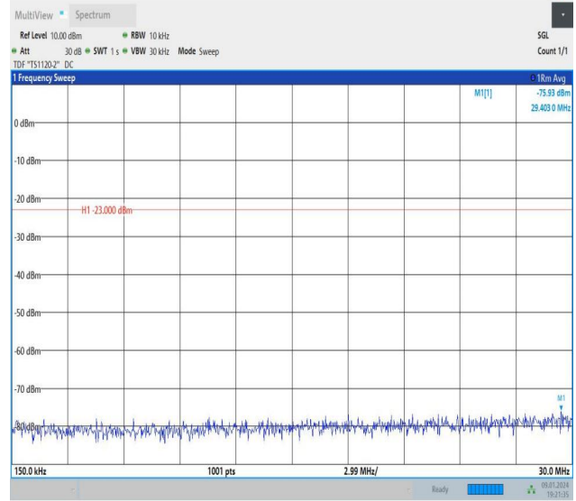
Band26_1.4MHz_QPSK_26783_1RB#0_0.15~30_0.15~30
