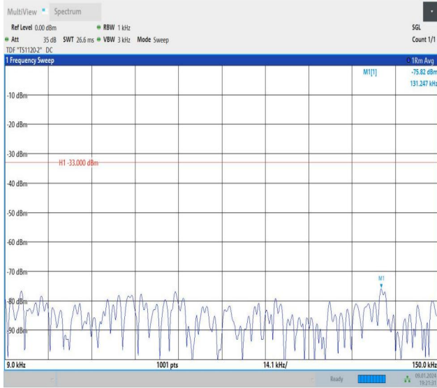
Band26_1.4MHz_QPSK_26783_1RB#0_0.009~0.15_0.009~0.15
