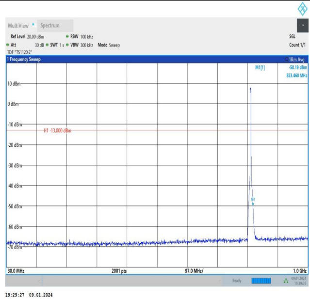
Band26_3MHz_16QAM_26705_15RB#0_30~1000_30~1000
