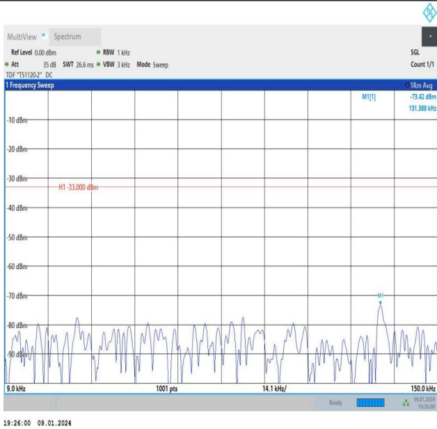
Band26_3MHz_QPSK_26705_1RB#0_0.009~0.15_0.009~0.1 5
