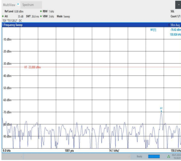
Band26_3MHz_QPSK_26740_1RB#0_0.009~0.15_0.009~0.1
