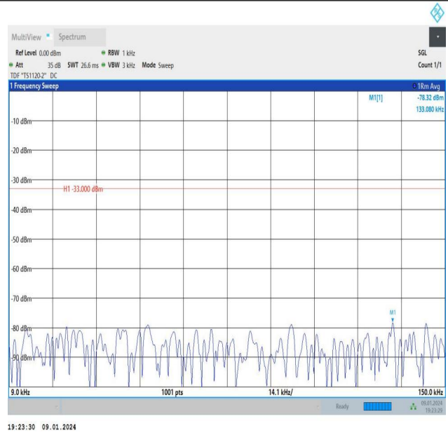
Band26_1.4MHz_16QAM_26783_1RB#5_0.009~0.15_0.009~0.15
