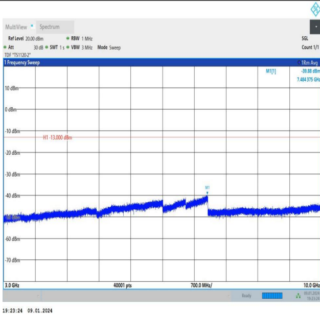
Band26_1.4MHz_QPSK_26783_1RB#5_3000~10000_3000~10000
