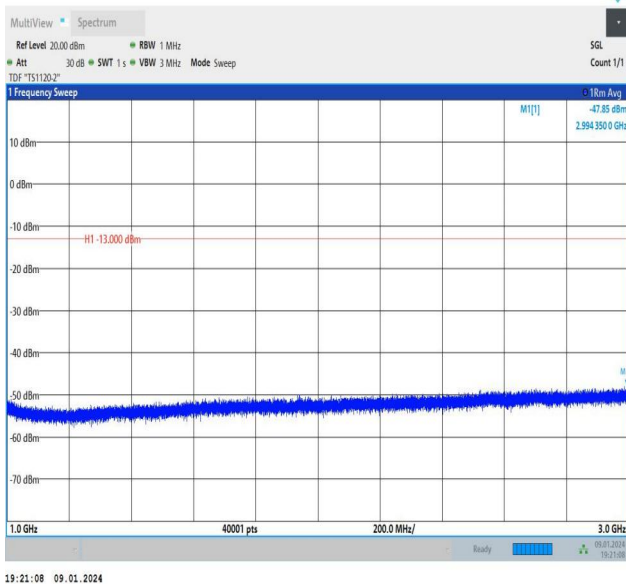
Band26_1.4MHz_16QAM_26740_6RB#0_1000~3000_1000~3000
