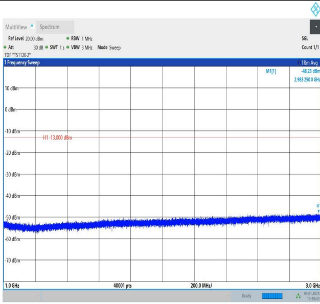
Band26_1.4MHz_16QAM_26740_1RB#5_1000~3000_1000~3000
