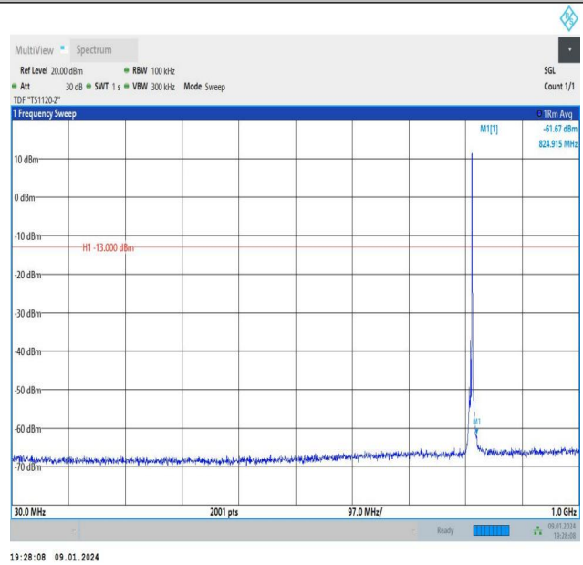
Band26_3MHz_16QAM_26705_1RB#14_30~1000_30~1000
