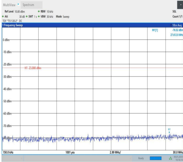
Band26_1.4MHz_16QAM_26740_1RB#0_0.15~30_0.15~30
