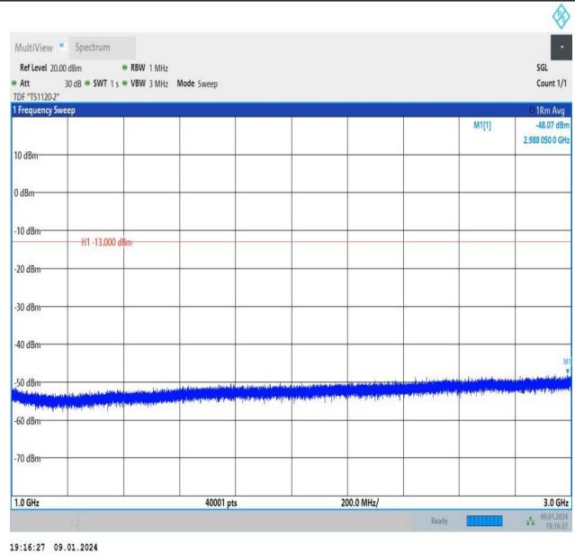
Band26_1.4MHz_QPSK_26697_6RB#0_1000~3000_1000~3000
