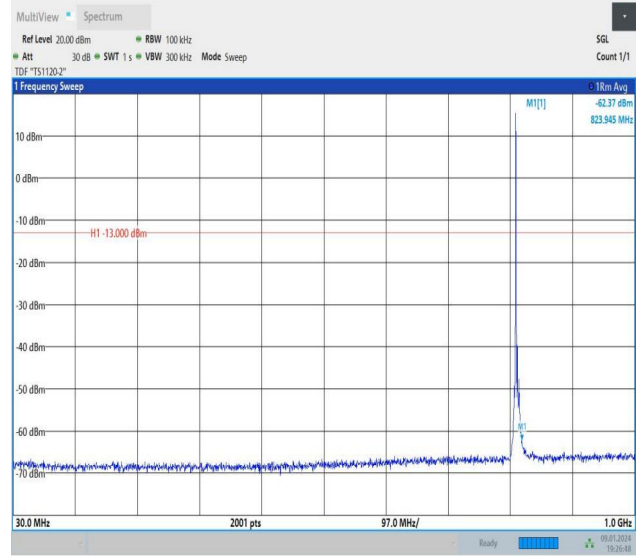
Band26_3MHz_16QAM_26705_1RB#0_30~1000_30~1000
