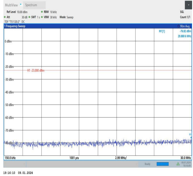
Band26_1.4MHz_QPSK_26697_6RB#0_0.15~30_0.15~30
