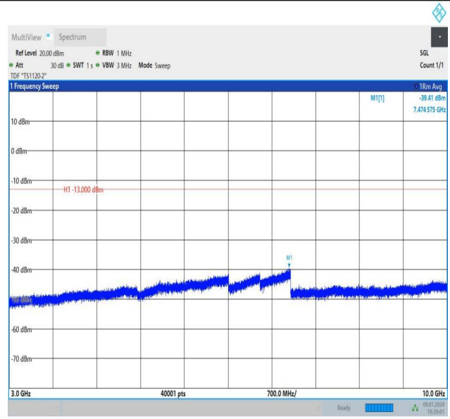
Band26_1.4MHz_16QAM_26740_1RB#5_3000~10000_3000~10000
