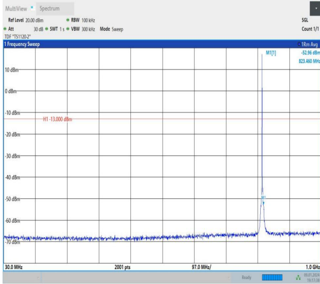
Band26_1.4MHz_QPSK_26740_1RB#0_30~1000_30~1000
