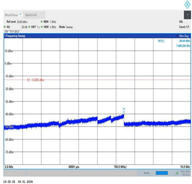
Band26_3MHz_16QAM_26740_1RB#14_3000~10000_3000~10000
