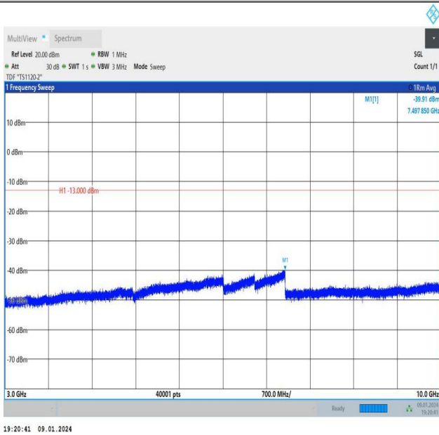
Band26_1.4MHz_QPSK_26740_6RB#0_3000~10000_3000~10000
