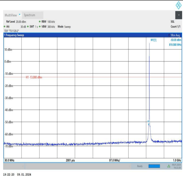
Band26_1.4MHz_16QAM_26783_1RB#0_30~1000_30~1000
