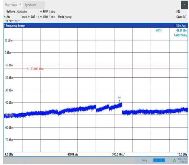
Band26_1.4MHz_16QAM_26697_6RB#0_3000~10000_3000~10000
