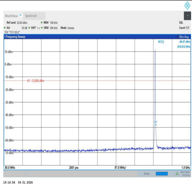
Band26_1.4MHz_16QAM_26697_6RB#0_30~1000_30~1000
