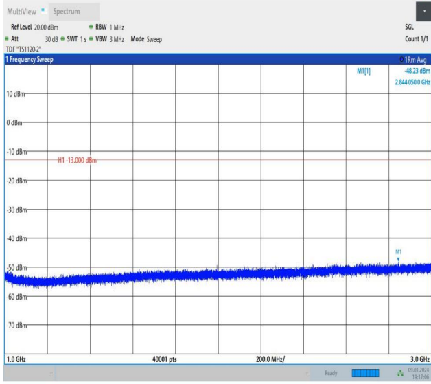
Band26_1.4MHz_16QAM_26697_6RB#0_1000~3000_1000~3000
