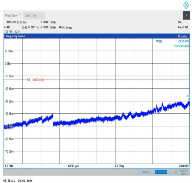
Band25_10MHz_16QAM_26090_1RB#0_3000~20000_3000~20000
