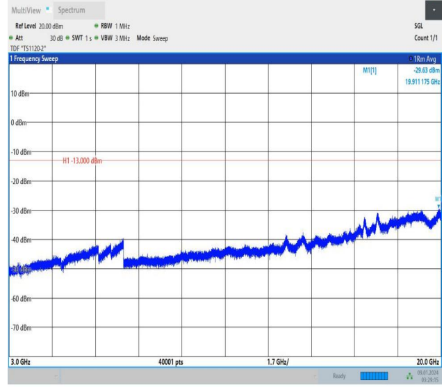
Band25_10MHz_16QAM_26365_1RB#49_3000~20000_3000~20000
