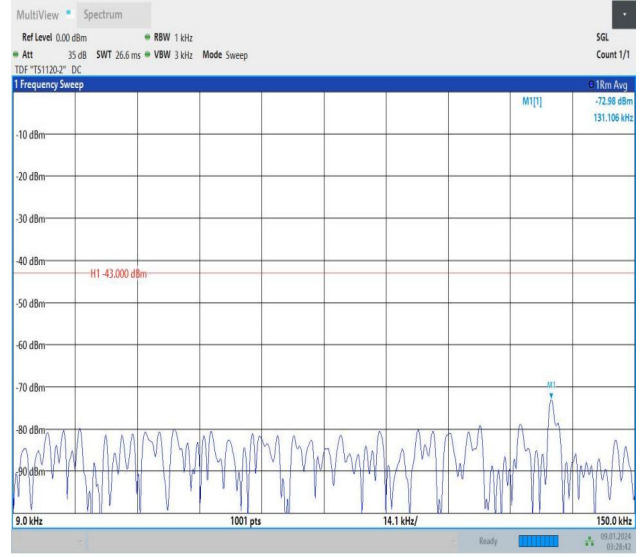
Band25_10MHz_16QAM_26365_1RB#49_0.009~0.15_0.009~0.15
