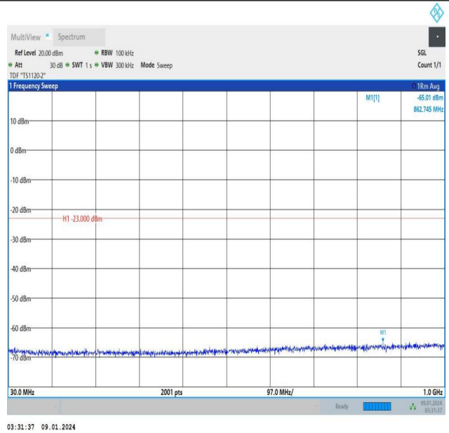
Band25_10MHz_16QAM_26640_1RB#49_30~1000_30~1000
