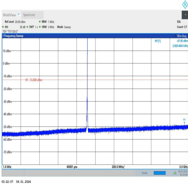
Band25_5MHz_16QAM_26665_1RB#24_1000~3000_1000~3000
