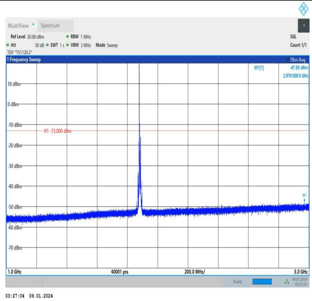
Band25_10MHz_QPSK_26365_1RB#0_1000~3000_1000~3000
