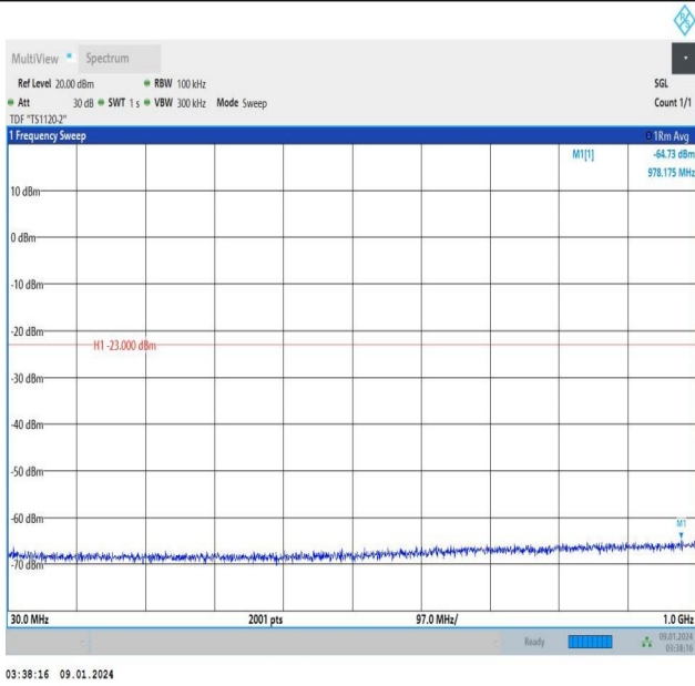
Band25_15MHz_16QAM_26365_1RB#0_30~1000_30~1000
