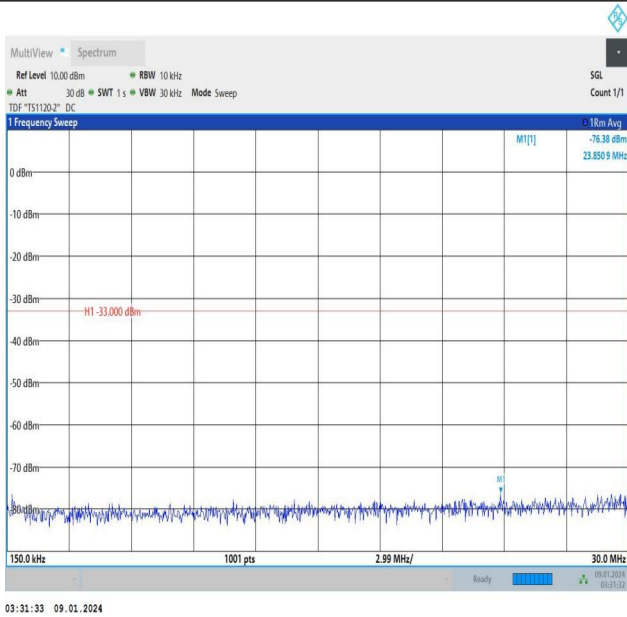
Band25_10MHz_16QAM_26640_1RB#49_0.15~30_0.15~30
