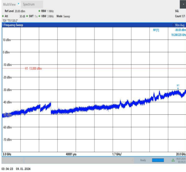
Band25_10MHz_QPSK_26640_50RB#0_3000~20000_3000~20000
