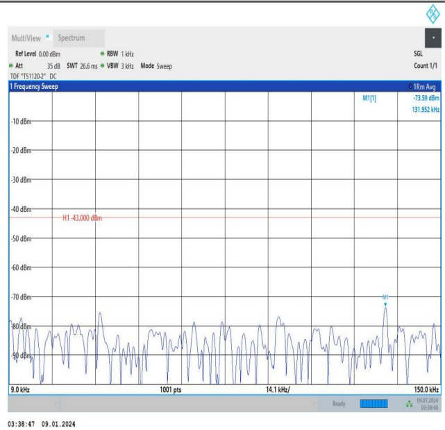
Band25_15MHz_QPSK_26365_1RB#74_0.009~0.15_0.009~0.15
