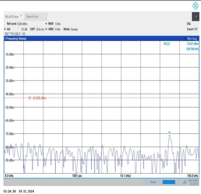
Band25_10MHz_16QAM_26090_1RB#0_0.009~0.15_0.009~0.15
