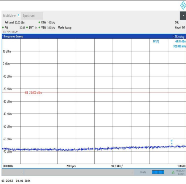
Band25_10MHz_QPSK_26365_1RB#0_30~1000_30~1000
