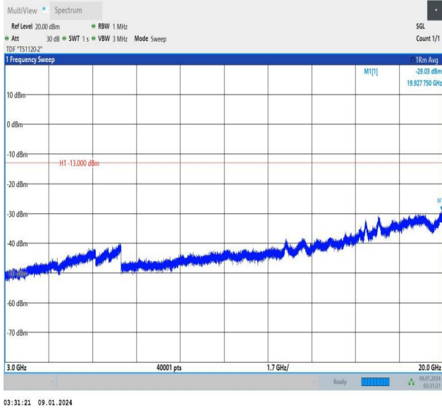
Band25_10MHz_QPSK_26640_1RB#49_3000~20000_3000~20000
