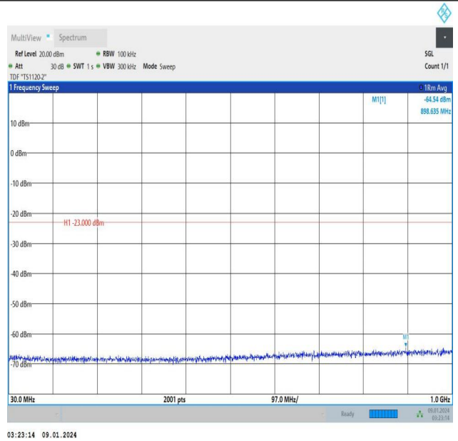
Band25_5MHz_16QAM_26665_25RB#0_30~1000_30~1000
