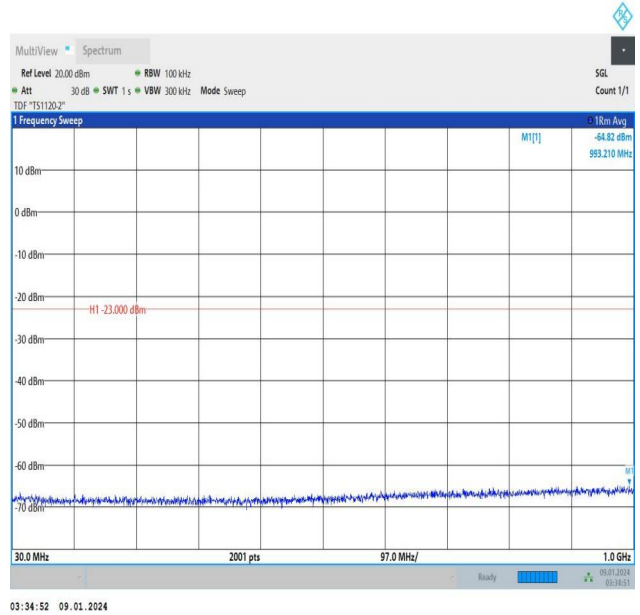
Band25_15MHz_QPSK_26115_1RB#0_30~1000_30~1000
