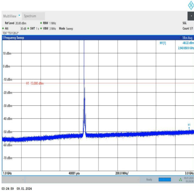
Band25_10MHz_16QAM_26090_1RB#0_1000~3000_1000~3000
