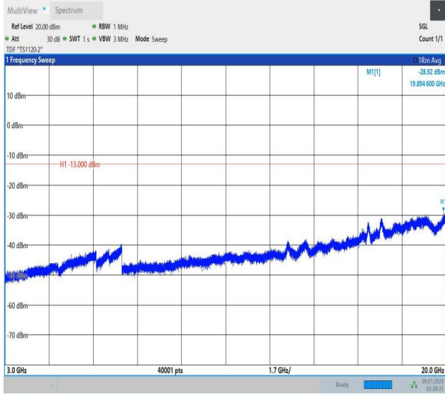
Band25_10MHz_QPSK_26365_1RB#49_3000~20000_3000~20000
