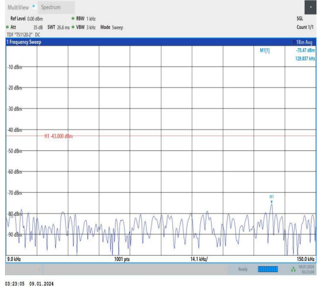
Band25_5MHz_16QAM_26665_25RB#0_0.009~0.15_0.009~0.15
