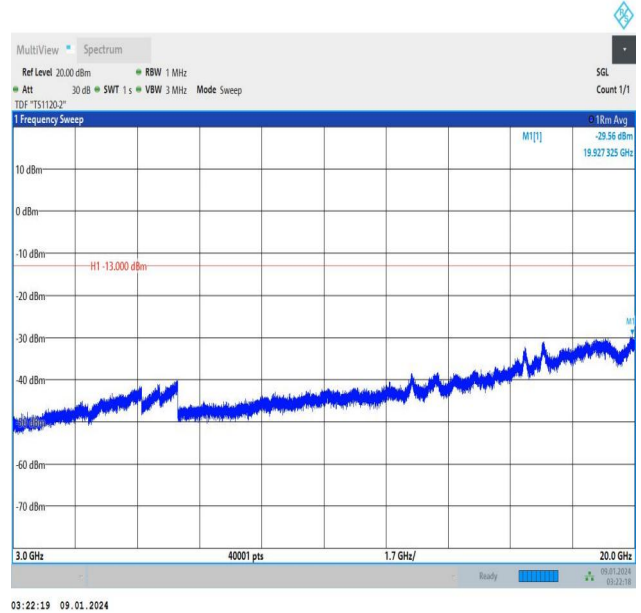
Band25_5MHz_16QAM_26665_1RB#24_3000~20000_3000~20000
