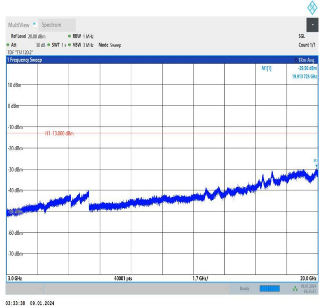
Band25_10MHz_QPSK_26365_50RB#0_3000~20000_3000~20000
