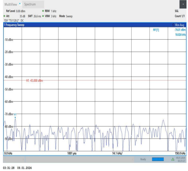
Band25_10MHz_16QAM_26640_1RB#49_0.009~0.15_0.009~0.15
