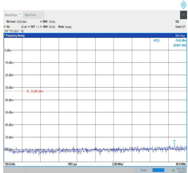
Band25_10MHz_16QAM_26365_1RB#49_3000~20000_3000~20000
