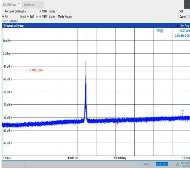
Band25_10MHz_16QAM_26365_1RB#49_1000~3000_1000~3000
