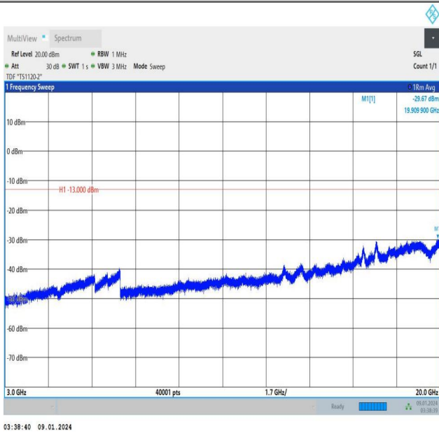
Band25_15MHz_16QAM_26365_1RB#0_3000~20000_3000~20000
