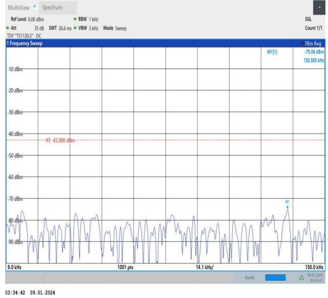
Band25_15MHz_QPSK_26115_1RB#0_0.009~0.15_0.009~0.1 5
