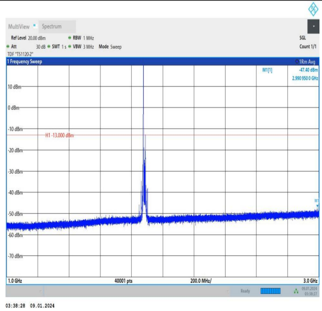
Band25_15MHz_16QAM_26365_1RB#0_1000~3000_1000~3000
