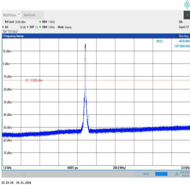
Band25_10MHz_QPSK_26365_50RB#0_1000~3000_1000~3000
