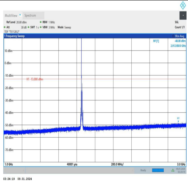
Band25_10MHz_QPSK_26090_1RB#0_1000~3000_1000~3000
