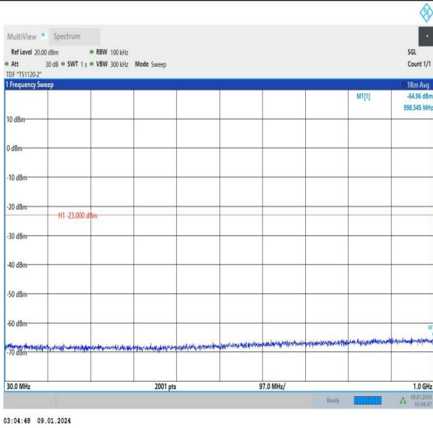
Band25_3MHz_QPSK_26365_1RB#14_30~1000_30~1000
