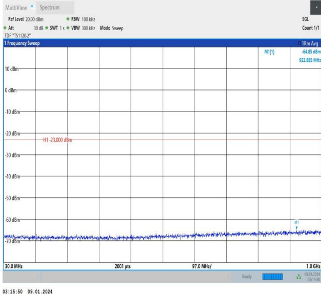
Band25_5MHz_QPSK_26365_1RB#0_30~1000_30~1000
