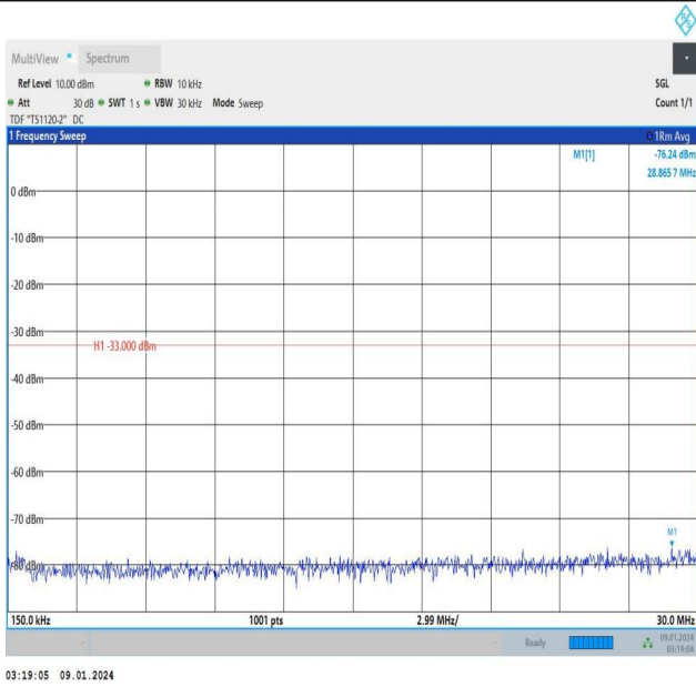
Band25_5MHz_16QAM_26365_25RB#0_0.15~30_0.15~30
