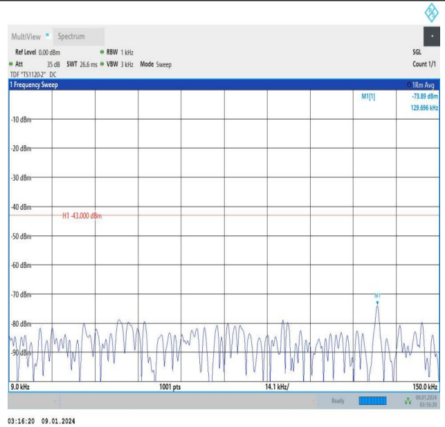
Band25_5MHz_16QAM_26365_1RB#0_0.009~0.15_0.009~0.15 15
