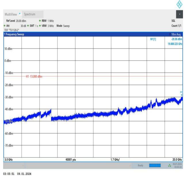
Band25_3MHz_16QAM_26365_1RB#14_3000~20000_3000~20000
