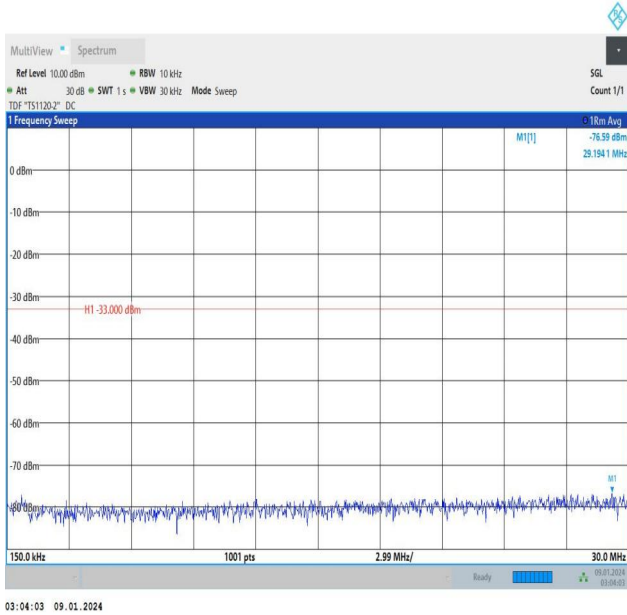
Band25_3MHz_16QAM_26365_1RB#0_0.15~30_0.15~30
