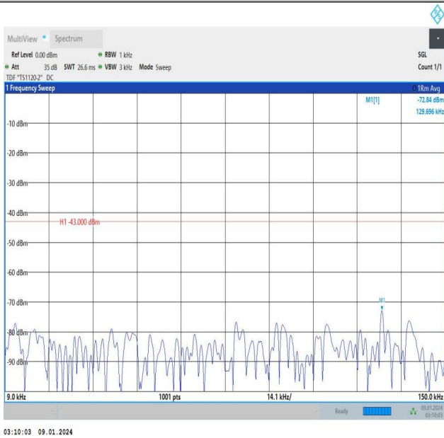
Band25_3MHz_QPSK_26675_15RB#0_0.009~0.15_0.009~0.15
