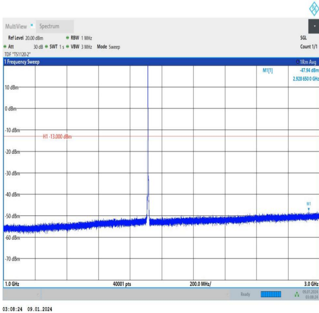
Band25_3MHz_16QAM_26675_1RB#0_1000~3000_1000~3000
