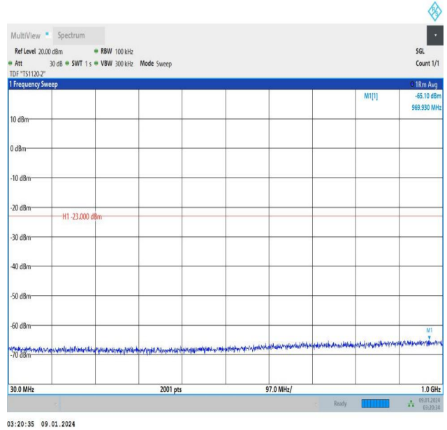
Band25_5MHz_16QAM_26665_1RB#0_30~1000_30~1000
