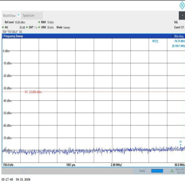
Band25_5MHz_16QAM_26365_1RB#24_0.15~30_0.15~30
