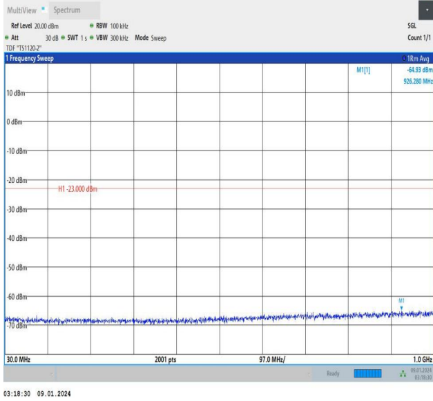
Band25_5MHz_QPSK_26365_25RB#0_30~1000_30~1000
