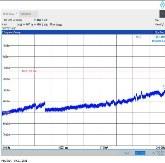
Band25_5MHz_QPSK_26365_1RB#0_3000~20000_3000~20000 000
