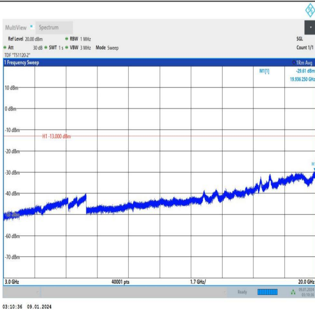
Band25_3MHz_QPSK_26675_15RB#0_3000~20000_3000~2 0000
