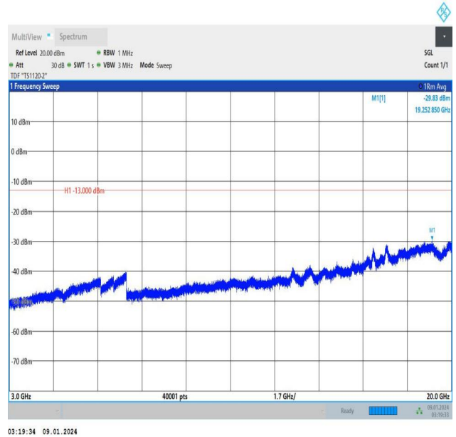
Band25_5MHz_16QAM_26365_25RB#0_3000~20000_3000~20000
