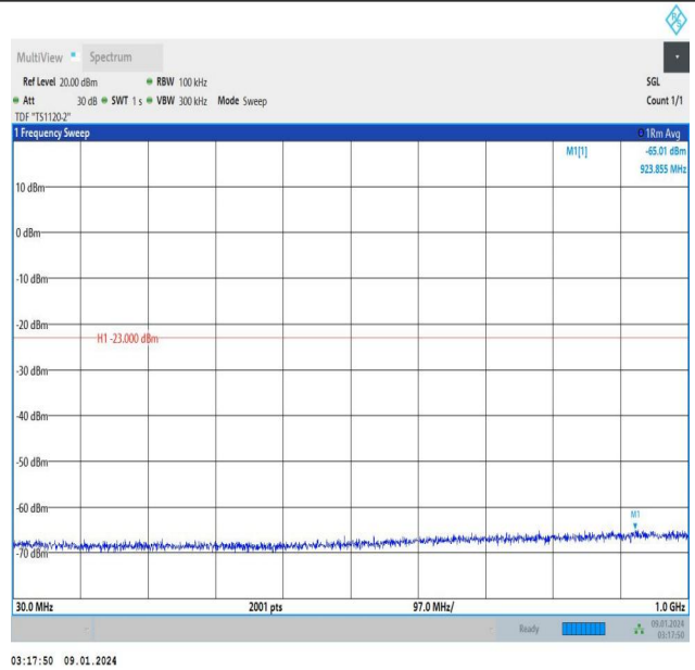
Band25_5MHz_16QAM_26365_1RB#24_30~1000_30~1000
