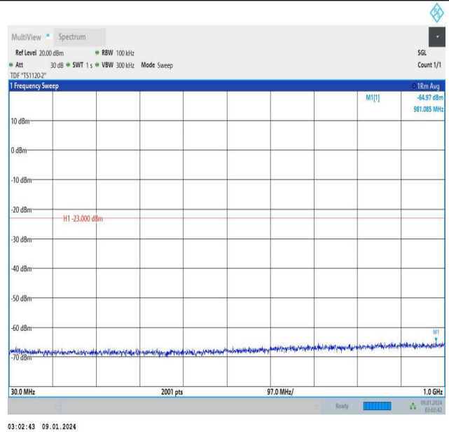
Band25_3MHz_16QAM_26055_15RB#0_30~1000_30~1000
