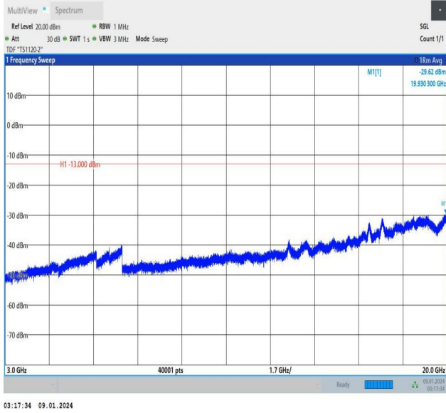
Band25_5MHz_QPSK_26365_1RB#24_3000~20000_3000~20000
