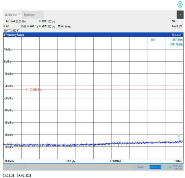
Band25_5MHz_16QAM_26065_1RB#0_30~1000_30~1000
