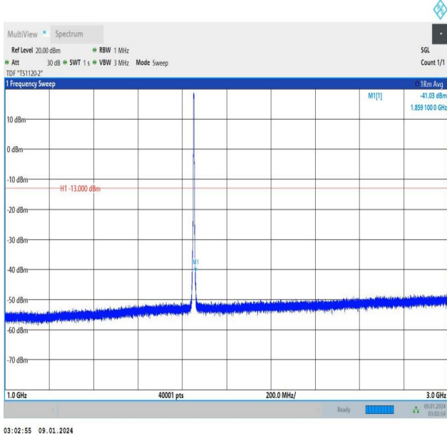
Band25_3MHz_16QAM_26055_15RB#0_1000~3000_1000~3000
