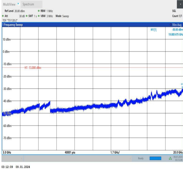
Band25_5MHz_QPSK_26065_1RB#0_3000~20000_3000~20000
