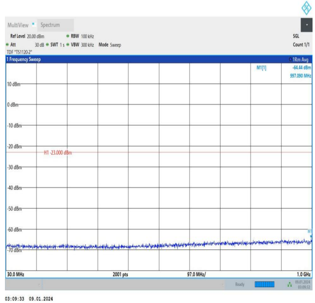
Band25_3MHz_16QAM_26675_1RB#14_30~1000_30~1000
