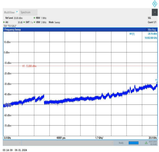
Band25_5MHz_16QAM_26065_1RB#24_3000~20000_3000~20000
