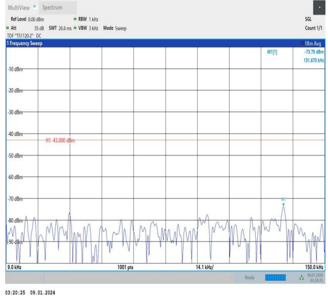
Band25_5MHz_16QAM_26665_1RB#0_0.009~0.15_0.009~0.15
