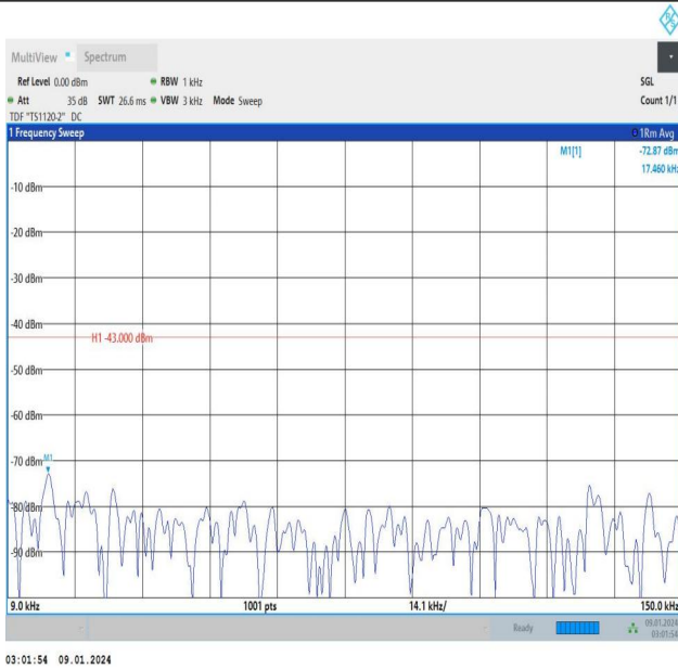
Band25_3MHz_QPSK_26055_15RB#0_0.009~0.15_0.009~0.15
