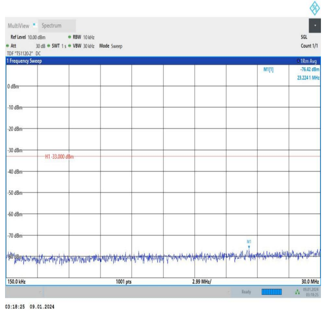
Band25_5MHz_QPSK_26365_25RB#0_0.15~30_0.15~30
