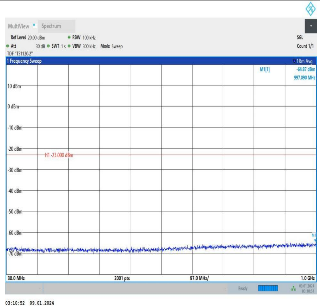
Band25_3MHz_16QAM_26675_15RB#0_30~1000_30~1000
