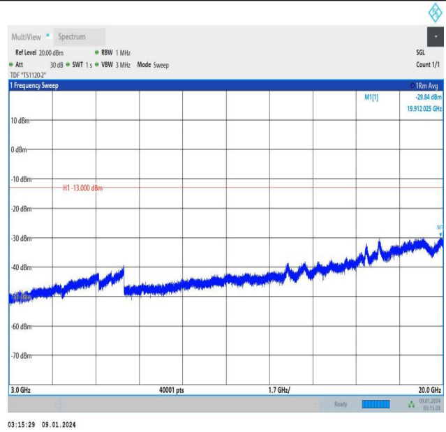
Band25_5MHz_16QAM_26065_25RB#0_3000~20000_3000~20000
