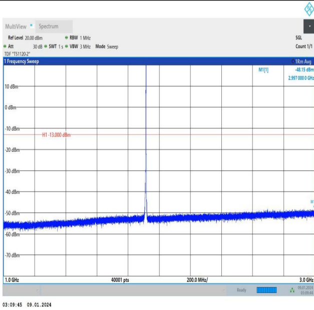
Band25_3MHz_16QAM_26675_1RB#14_1000~3000_1000~3000
