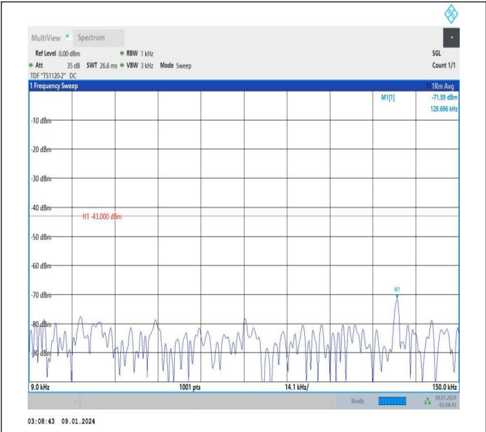
Band25_3MHz_QPSK_26675_1RB#14_0.009~0.15_0.009~0.15
