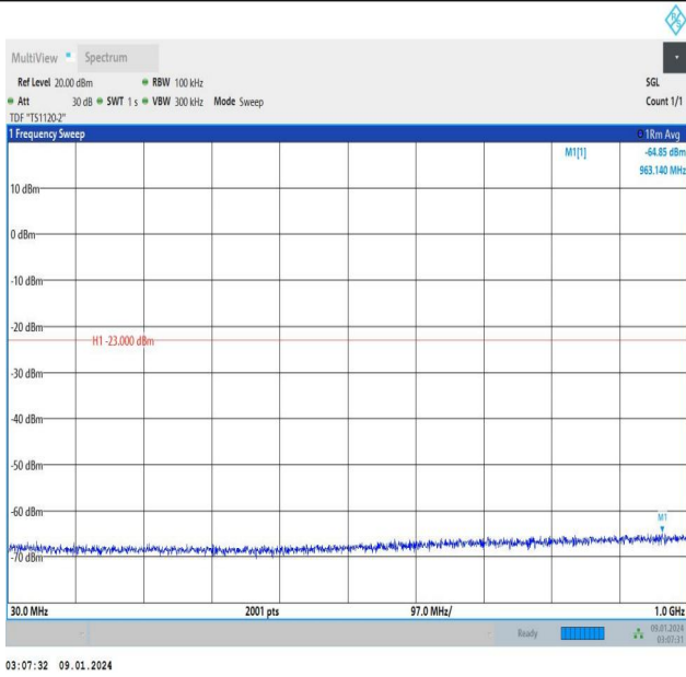
Band25_3MHz_QPSK_26675_1RB#0_30~1000_30~1000
