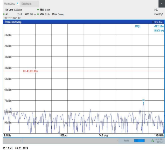
Band25_5MHz_16QAM_26365_1RB#24_0.009~0.15_0.009~0.15
