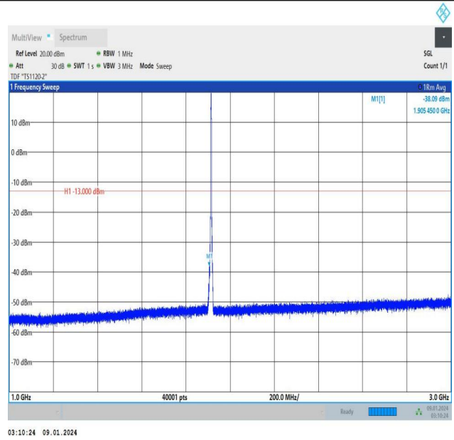
Band25_3MHz_QPSK_26675_15RB#0_1000~3000_1000~30 00
