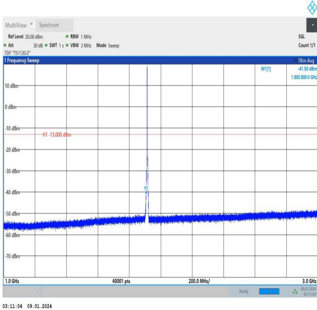
Band25_3MHz_16QAM_26675_15RB#0_1000~3000_1000~3000
