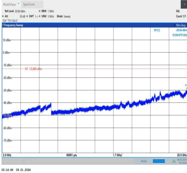
Band25_5MHz_QPSK_26065_25RB#0_3000~20000_3000~20000
