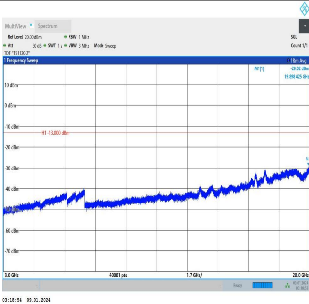
Band25_5MHz_QPSK_26365_25RB#0_3000~20000_3000~2 0000
