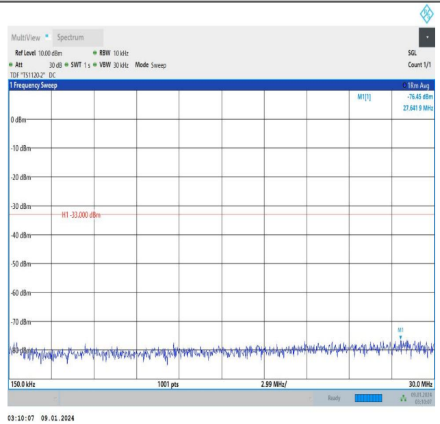
Band25_3MHz_QPSK_26675_15RB#0_0.15~30_0.15~30
