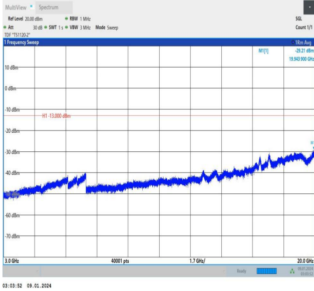
Band25_3MHz_QPSK_26365_1RB#0_3000~20000_3000~20000
