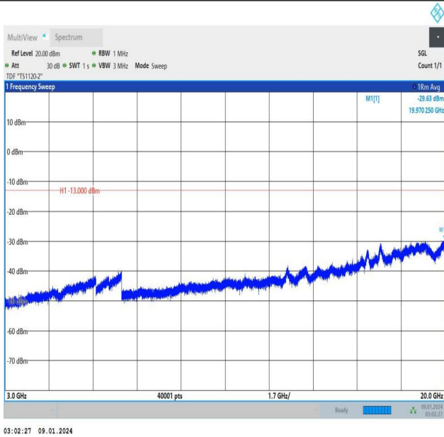
Band25_3MHz_QPSK_26055_15RB#0_3000~20000_3000~20000
