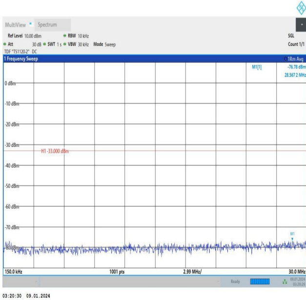
Band25_5MHz_16QAM_26665_1RB#0_0.15~30_0.15~30
