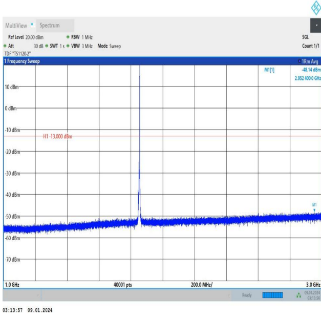
Band25_5MHz_16QAM_26065_1RB#24_1000~3000_1000~3000
