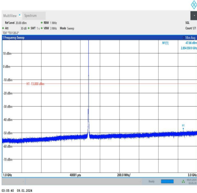
Band25_3MHz_16QAM_26365_1RB#14_1000~3000_1000~3000
