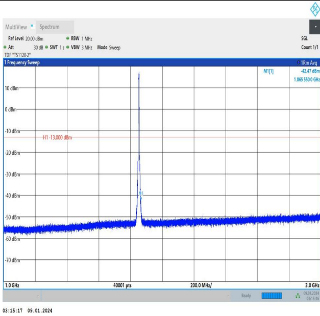
Band25_5MHz_16QAM_26065_25RB#0_1000~3000_1000~3000
