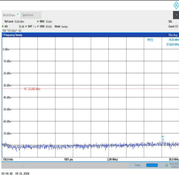
Band25_3MHz_16QAM_26365_15RB#0_0.15~30_0.15~30
