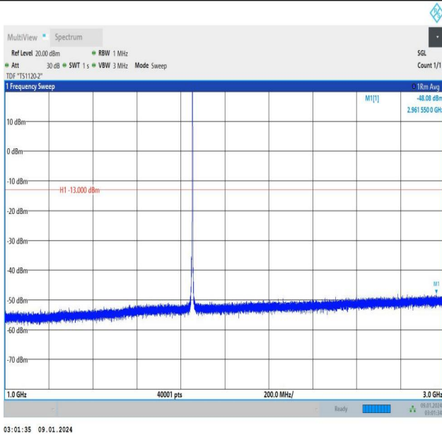
Band25_3MHz_16QAM_26055_1RB#14_1000~3000_1000~3000
