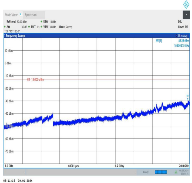
Band25_3MHz_16QAM_26675_15RB#0_3000~20000_3000~20000
