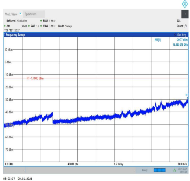
Band25_3MHz_16QAM_26055_15RB#0_3000~20000_3000~20000
