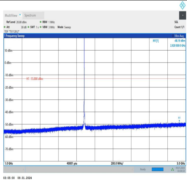
Band25_3MHz_QPSK_26365_1RB#14_1000~3000_1000~3000
