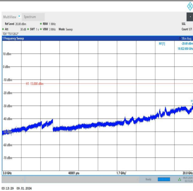
Band25_5MHz_QPSK_26065_1RB#24_3000~20000_3000~2 0000
