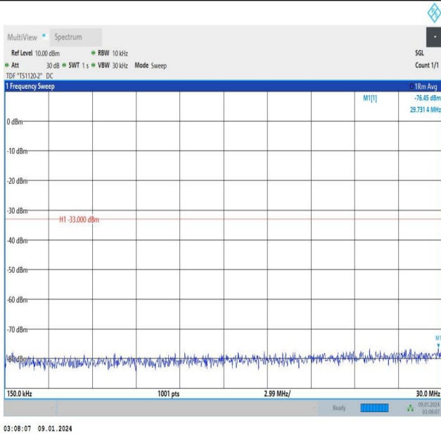
Band25_3MHz_16QAM_26675_1RB#0_0.15~30_0.15~30
