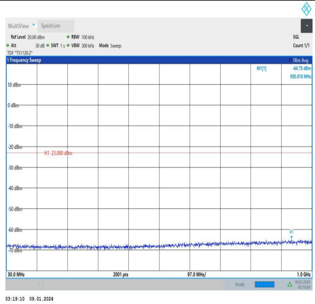
Band25_5MHz_16QAM_26365_25RB#0_30~1000_30~1000
