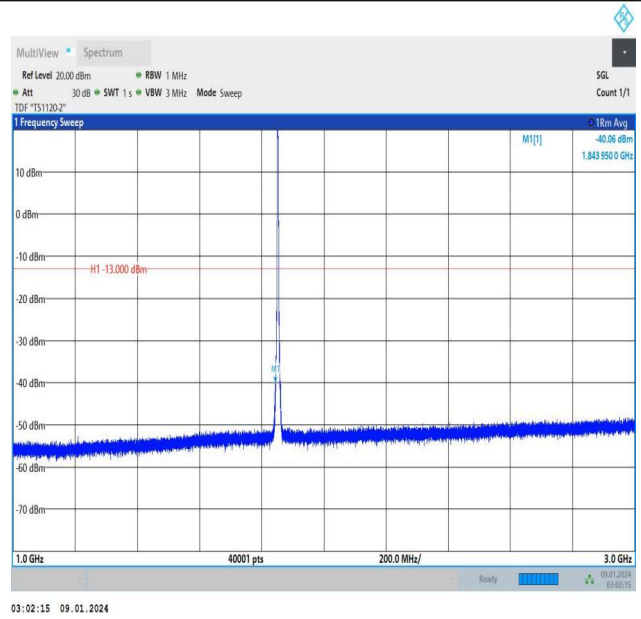
Band25_3MHz_QPSK_26055_15RB#0_1000~3000_1000~3000
