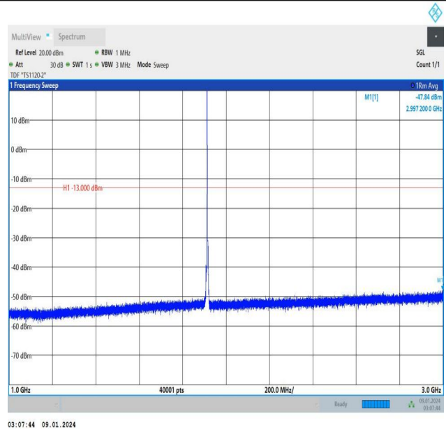
Band25_3MHz_QPSK_26675_1RB#0_1000~3000_1000~300 0
