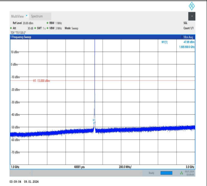
Band25_3MHz_QPSK_26675_1RB#14_1000~3000_1000~30
