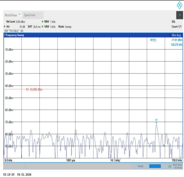
Band25_5MHz_16QAM_26365_25RB#0_0.009~0.15_0.009~0 .15
