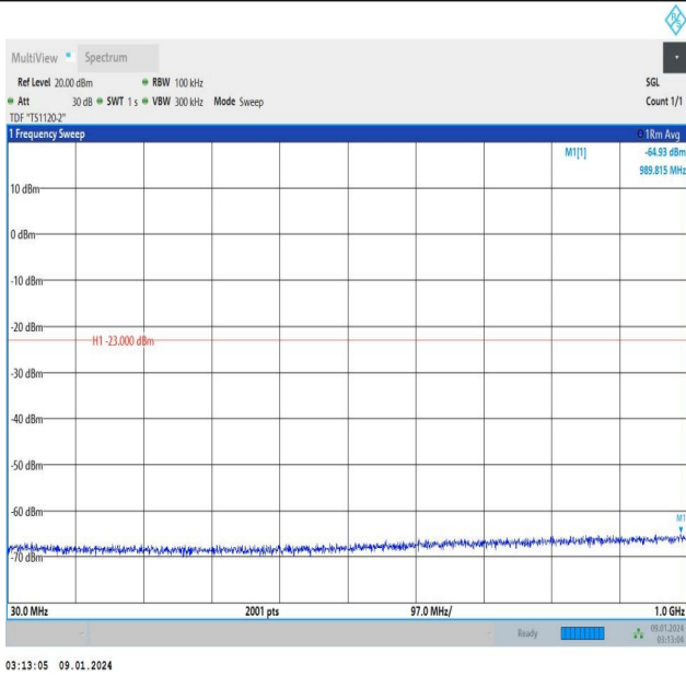
Band25_5MHz_QPSK_26065_1RB#24_30~1000_30~1000
