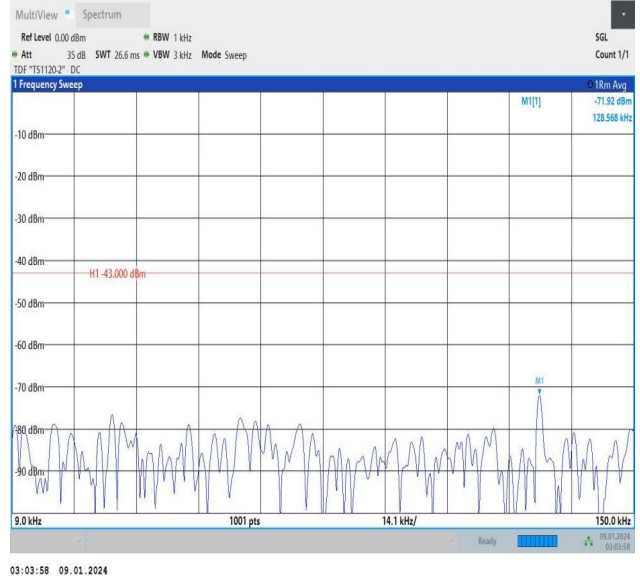
Band25_3MHz_16QAM_26365_1RB#0_0.009~0.15_0.009~0.15
