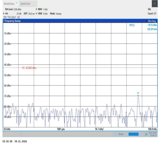
Band25_3MHz_16QAM_26365_15RB#0_0.009~0.15_0.009~0.15
