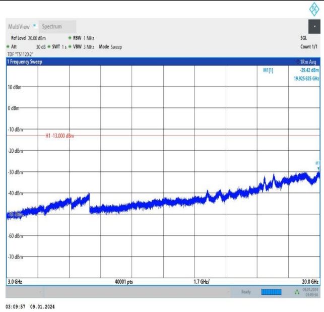
Band25_3MHz_16QAM_26675_1RB#14_3000~20000_3000~20000
