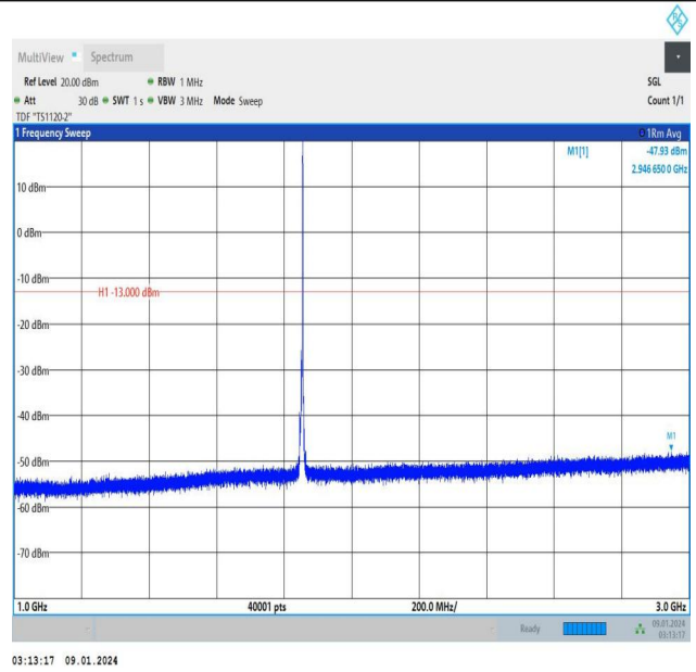
Band25_5MHz_QPSK_26065_1RB#24_1000~3000_1000~30 00
