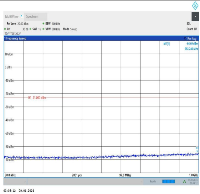
Band25_3MHz_16QAM_26675_1RB#0_30~1000_30~1000
