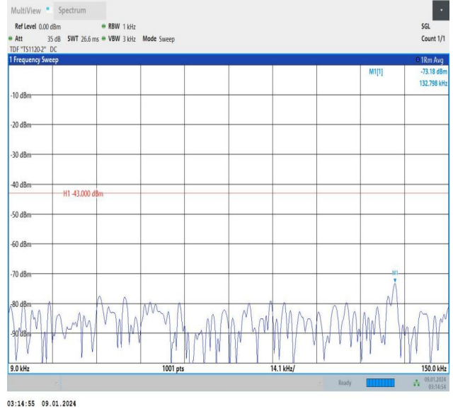
Band25_5MHz_16QAM_26065_25RB#0_0.009~0.15_0.009~0.15
