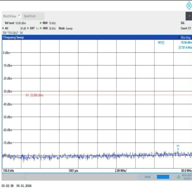
Band25_3MHz_16QAM_26055_15RB#0_0.15~30_0.15~30
