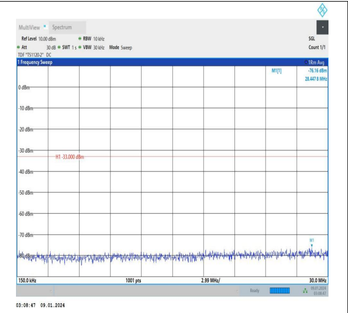
Band25_3MHz_QPSK_26675_1RB#14_0.15~30_0.15~30
