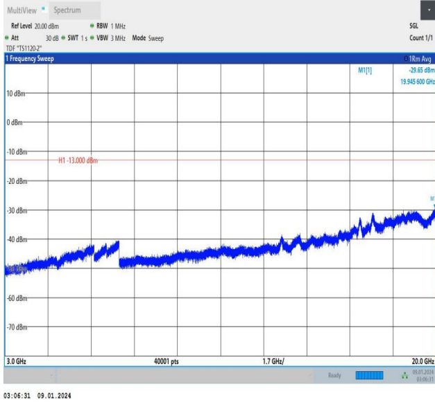
Band25_3MHz_QPSK_26365_15RB#0_3000~20000_3000~20000
