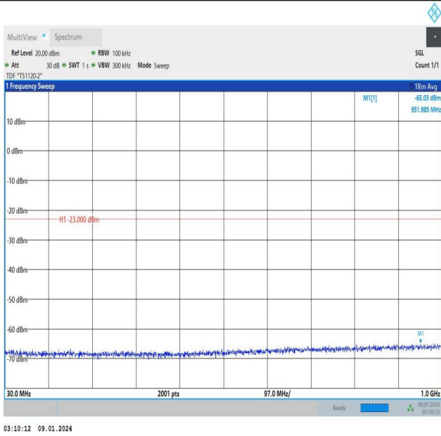
Band25_3MHz_QPSK_26675_15RB#0_30~1000_30~1000
