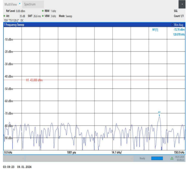
Band25_3MHz_16QAM_26675_1RB#14_0.009~0.15_0.009~0.15
