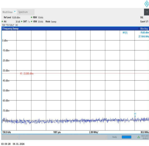
Band25_3MHz_16QAM_26675_1RB#14_0.15~30_0.15~30
