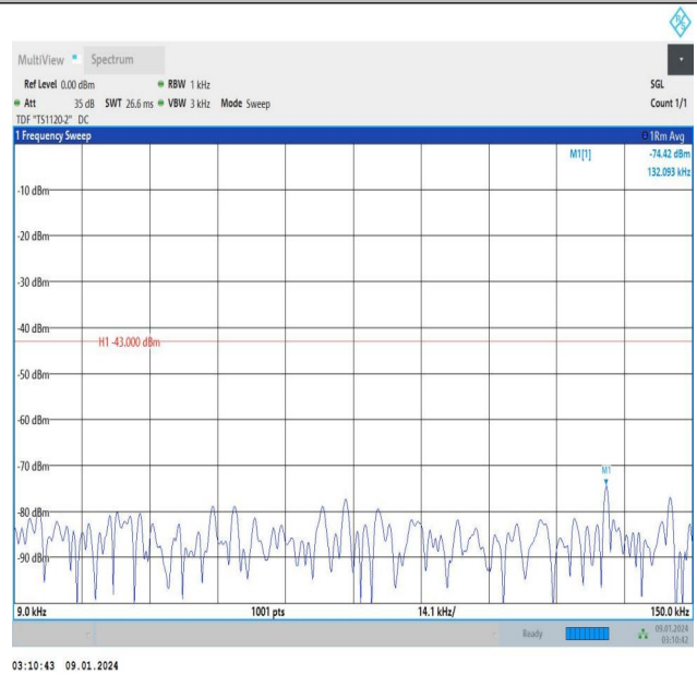
Band25_3MHz_16QAM_26675_15RB#0_0.009~0.15_0.009~0 .15
