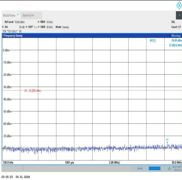
Band25_3MHz_16QAM_26365_1RB#14_0.15~30_0.15~30
