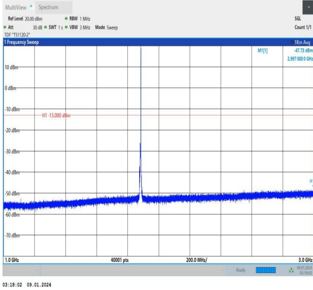
Band25_5MHz_16QAM_26365_1RB#24_1000~3000_1000~3000
