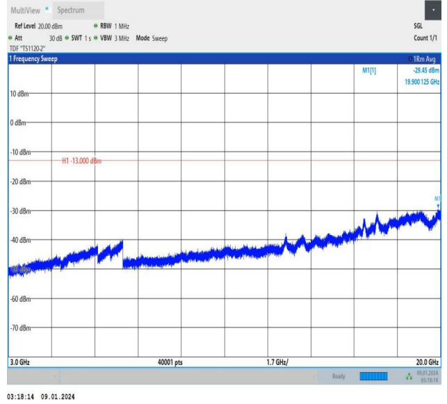
Band25_5MHz_16QAM_26365_1RB#24_3000~20000_3000~20000
