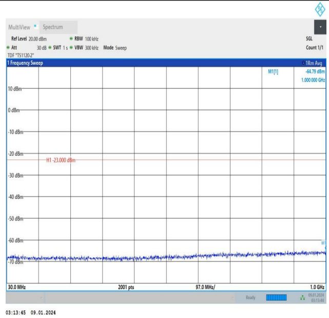
Band25_5MHz_16QAM_26065_1RB#24_30~1000_30~1000
