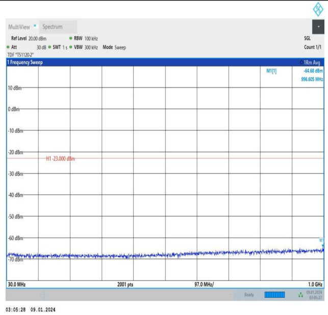
Band25_3MHz_16QAM_26365_1RB#14_30~1000_30~1000
