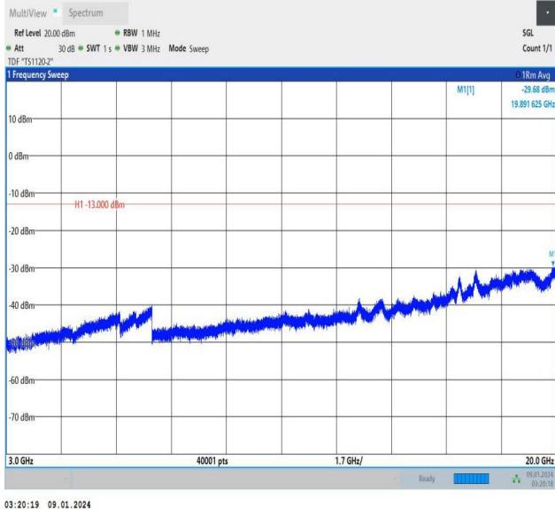
Band25_5MHz_QPSK_26665_1RB#0_3000~20000_3000~20000
