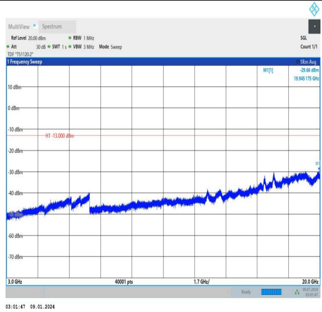
Band25_3MHz_16QAM_26055_1RB#14_3000~20000_3000~20000
