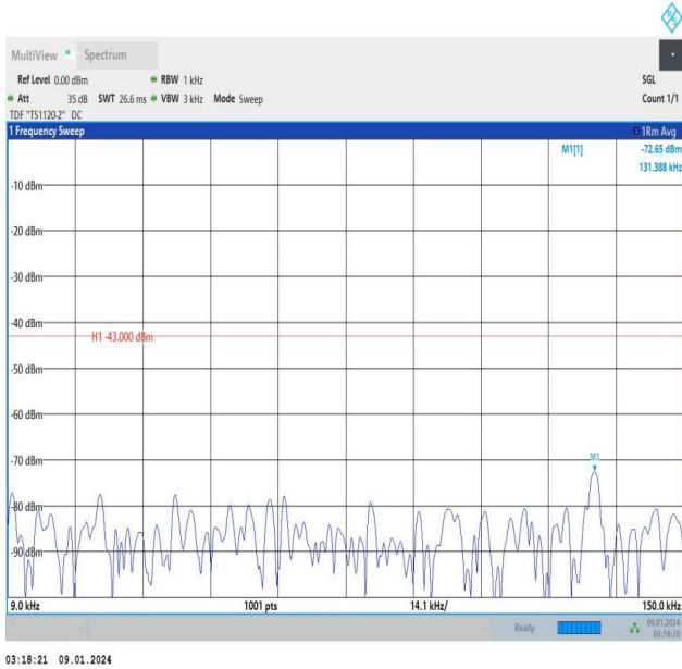
Band25_5MHz_QPSK_26365_25RB#0_0.009~0.15_0.009~0.15
