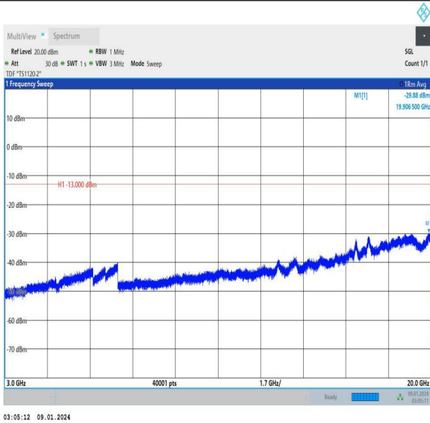
Band25_3MHz_QPSK_26365_1RB#14_3000~20000_3000~20000
