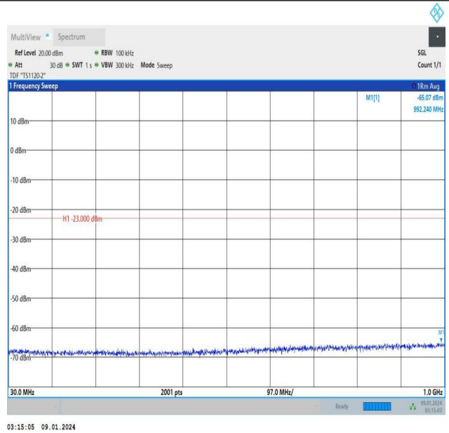
Band25_5MHz_16QAM_26065_25RB#0_30~1000_30~1000
