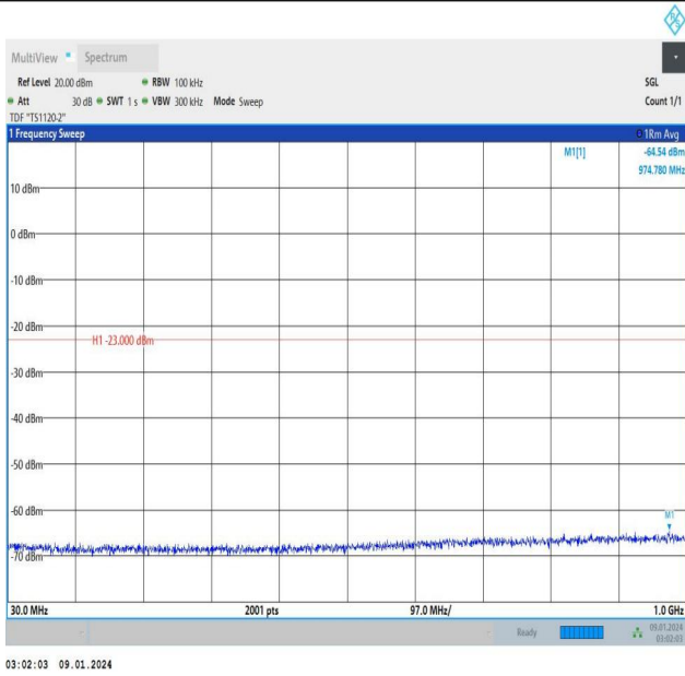
Band25_3MHz_QPSK_26055_15RB#0_30~1000_30~1000
