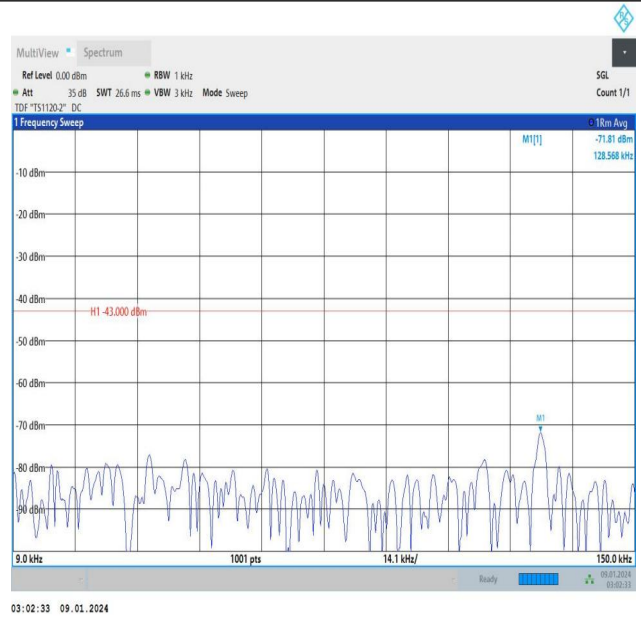
Band25_3MHz_16QAM_26055_15RB#0_0.009~0.15_0.009~0.15
