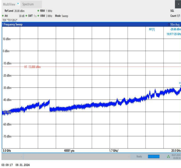
Band25_3MHz_QPSK_26675_1RB#14_3000~20000_3000~20000
