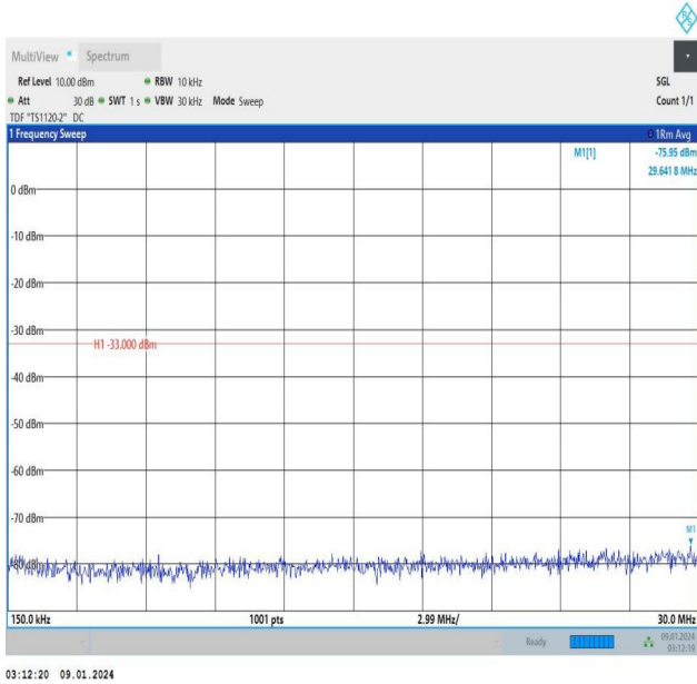
Band25_5MHz_16QAM_26065_1RB#0_0.15~30_0.15~30
