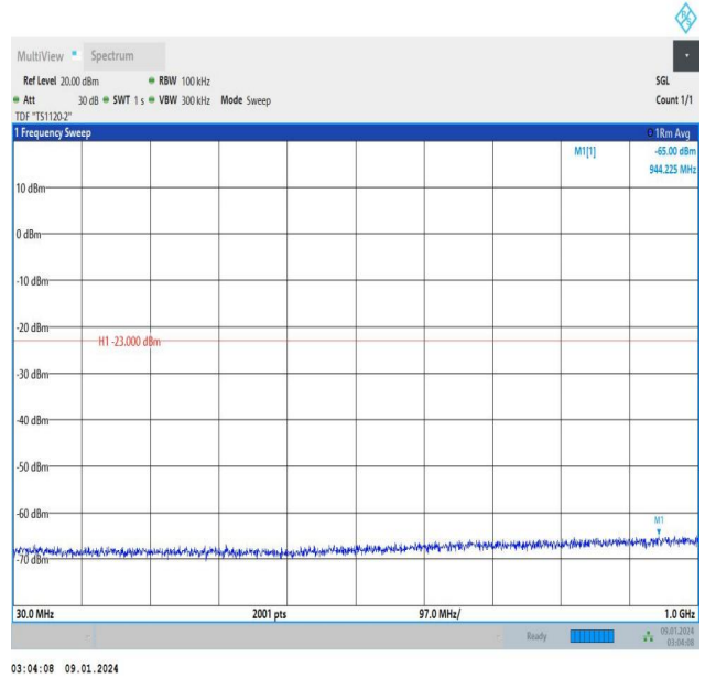
Band25_3MHz_16QAM_26365_1RB#0_30~1000_30~1000
