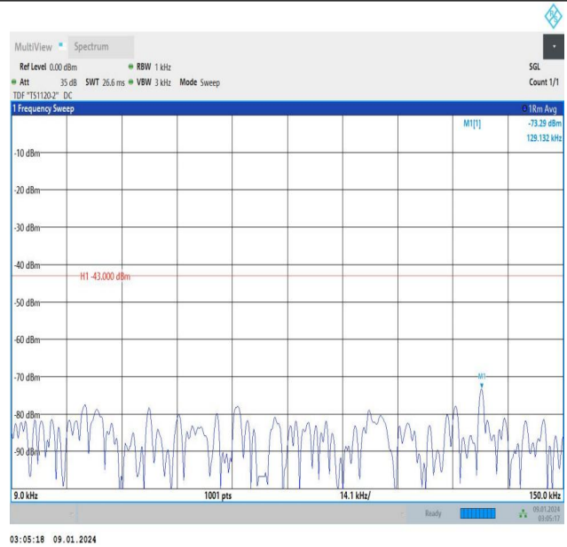
Band25_3MHz_16QAM_26365_1RB#14_0.009~0.15_0.009~0.15
