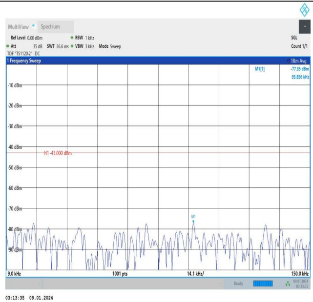
Band25_5MHz_16QAM_26065_1RB#24_0.009~0.15_0.009~0 .15
