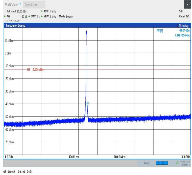
Band25_5MHz_QPSK_26365_25RB#0_1000~3000_1000~30 00
