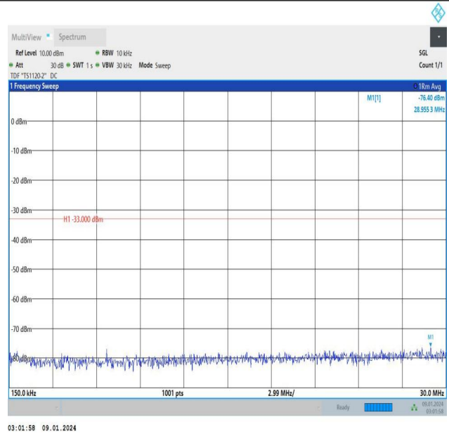
Band25_3MHz_QPSK_26055_15RB#0_0.15~30_0.15~30
