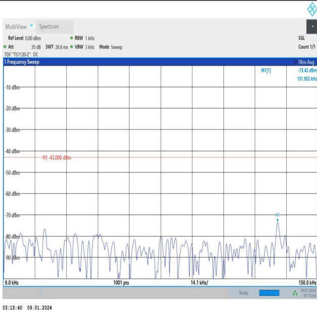
Band25_5MHz_QPSK_26365_1RB#0_0.009~0.15_0.009~0.15
