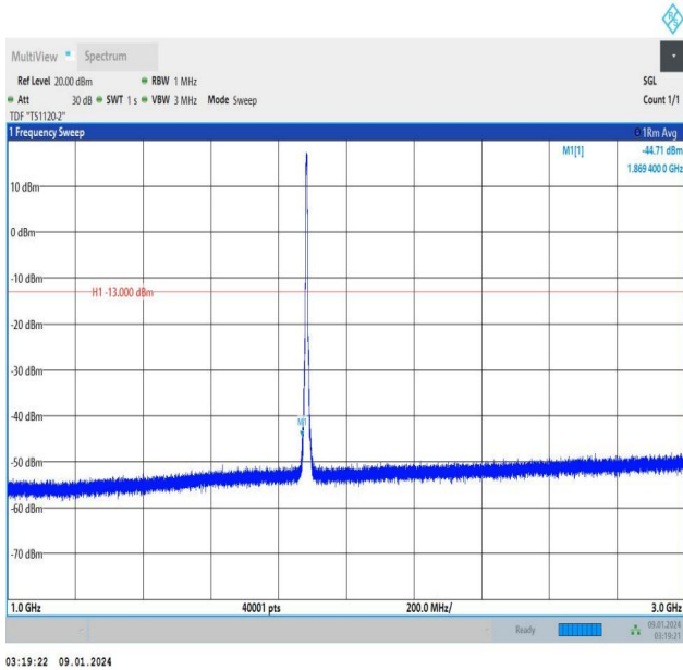
Band25_5MHz_16QAM_26365_25RB#0_1000~3000_1000~3000
