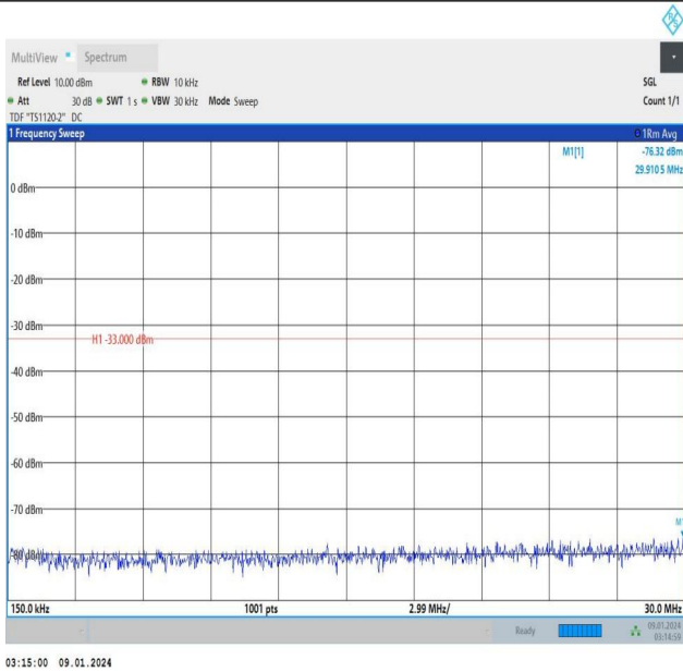
Band25_5MHz_16QAM_26065_25RB#0_0.15~30_0.15~30
