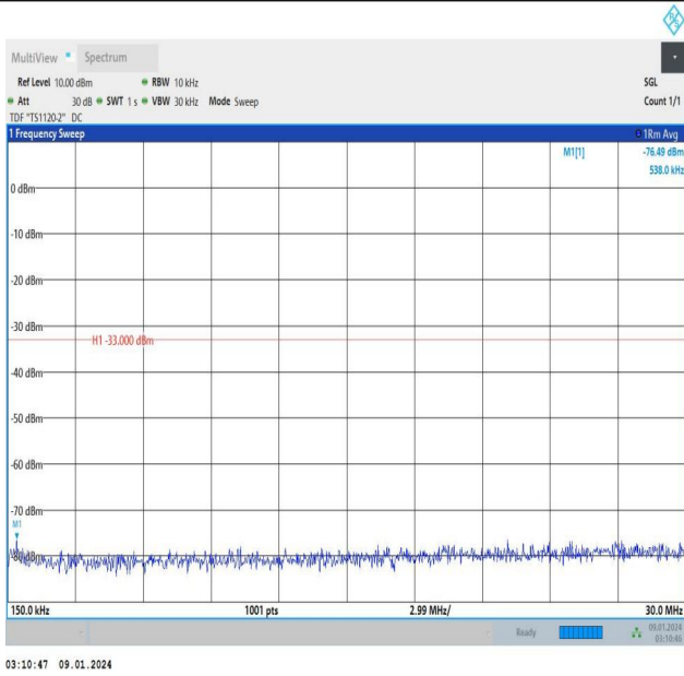
Band25_3MHz_16QAM_26675_15RB#0_0.15~30_0.15~30
