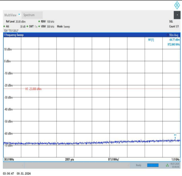
Band25_3MHz_16QAM_26365_15RB#0_30~1000_30~1000
