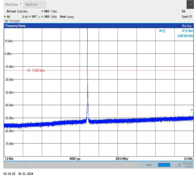
Band25_5MHz_QPSK_26365_1RB#0_1000~3000_1000~300 0
