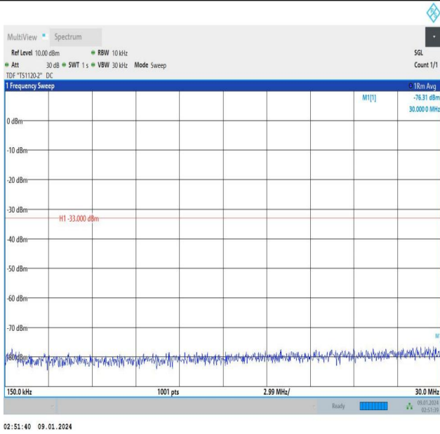
Band25_1.4MHz_16QAM_26365_1RB#0_0.15~30_0.15~30
