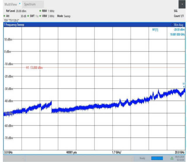
Band25_1.4MHz_16QAM_26047_6RB#0_3000~20000_3000~20000
