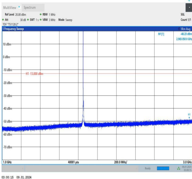
Band25_3MHz_16QAM_26055_1RB#0_1000~3000_1000~3000
