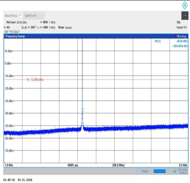
Band25_1.4MHz_QPSK_26047_1RB#5_1000~3000_1000~3000 00
