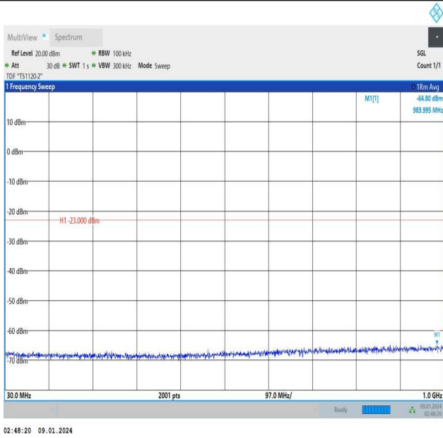
Band25_1.4MHz_QPSK_26047_1RB#5_30~1000_30~1000
