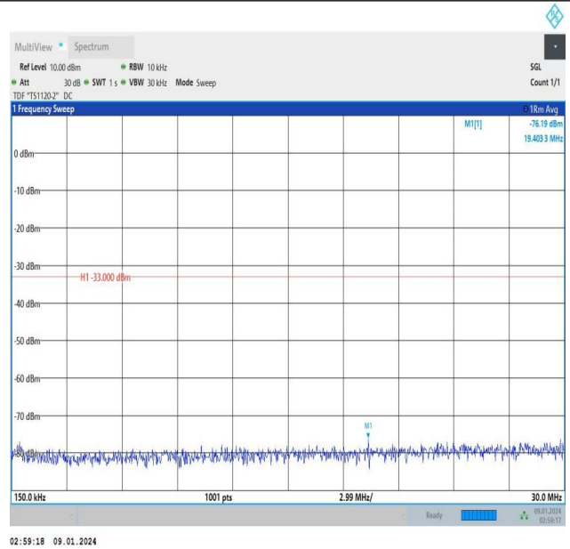
Band25_3MHz_QPSK_26055_1RB#0_0.15~30_0.15~30
