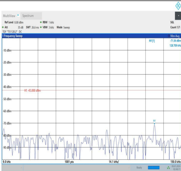
Band25_1.4MHz_16QAM_26047_1RB#0_1000~3000_1000~3000
