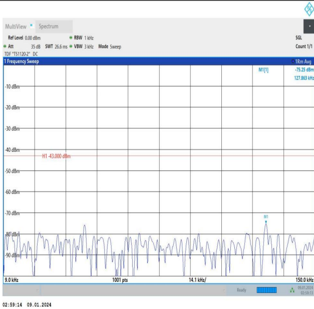
Band25_3MHz_QPSK_26055_1RB#0_0.009~0.15_0.009~0.15
