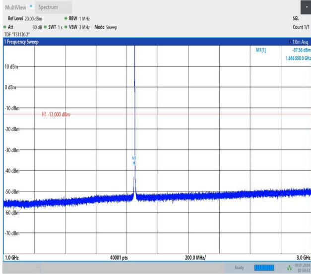
Band25_1.4MHz_16QAM_26047_6RB#0_1000~3000_1000~3000
