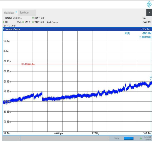
Band25_1.4MHz_16QAM_26047_1RB#0_3000~20000_3000~20000
