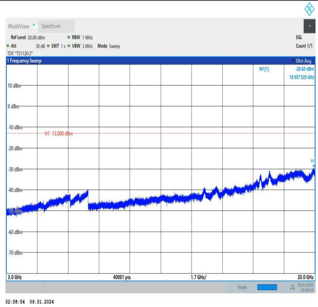
Band25_1.4MHz_16QAM_26683_6RB#0_3000~20000_3000~20000
