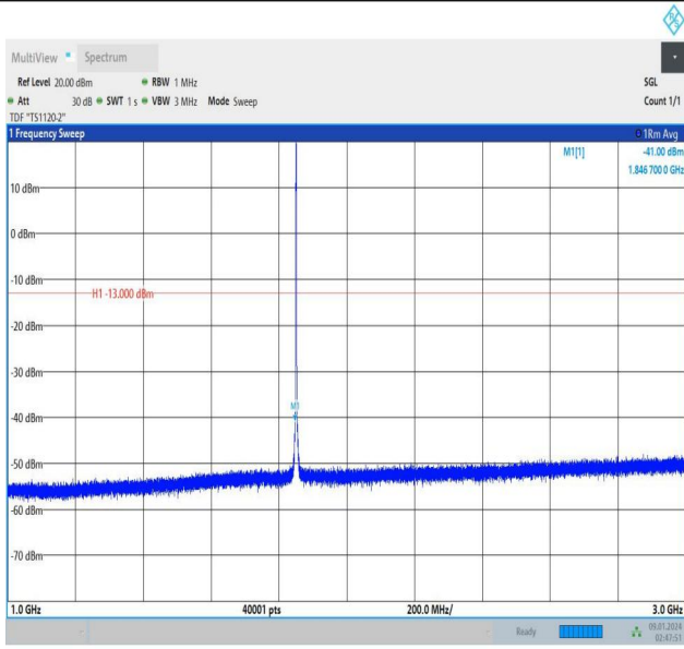
Band25_1.4MHz_16QAM_26047_1RB#0_1000~3000_1000~3000
