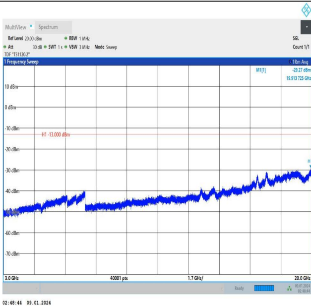
Band25_1.4MHz_QPSK_26047_1RB#5_3000~20000_3000~20000 0000
