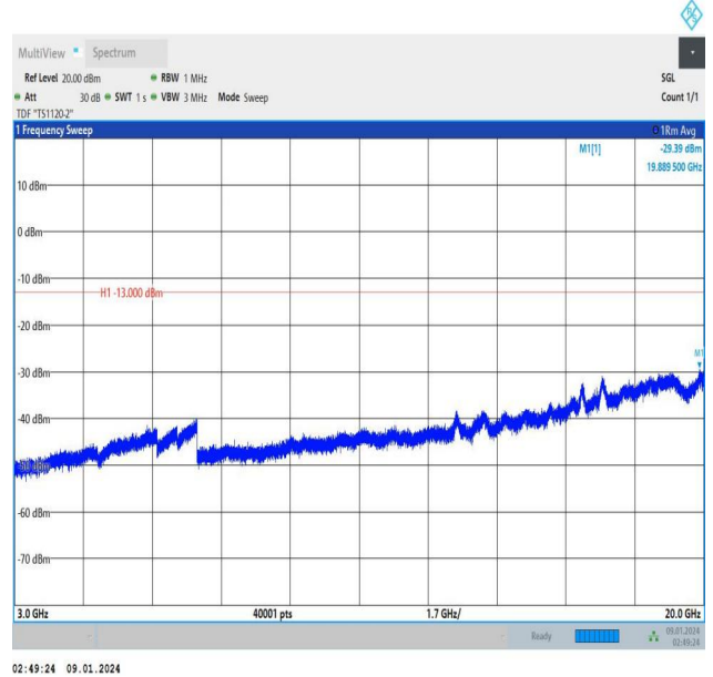
Band25_1.4MHz_16QAM_26047_1RB#5_3000~20000_3000~20000
