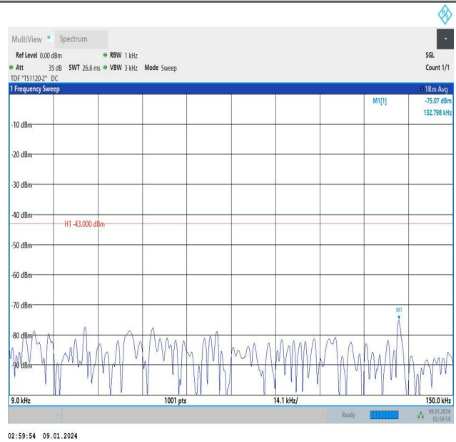
Band25_3MHz_16QAM_26055_1RB#0_0.009~0.15_0.009~0.
