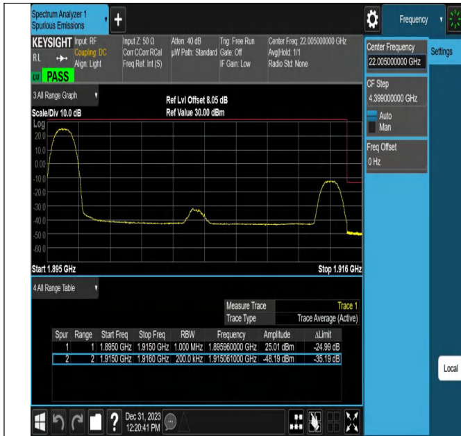
Band25_20MHz_16QAM_26590_1RB#0
