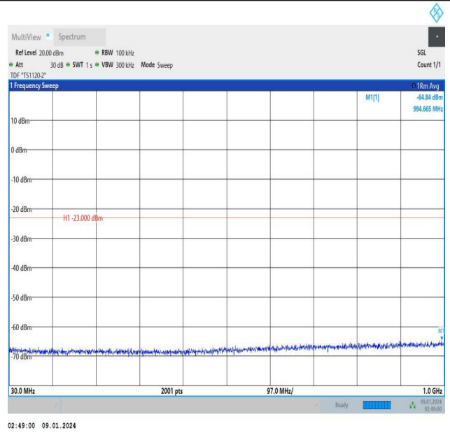
Band25_1.4MHz_16QAM_26047_1RB#5_30~1000_30~1000
