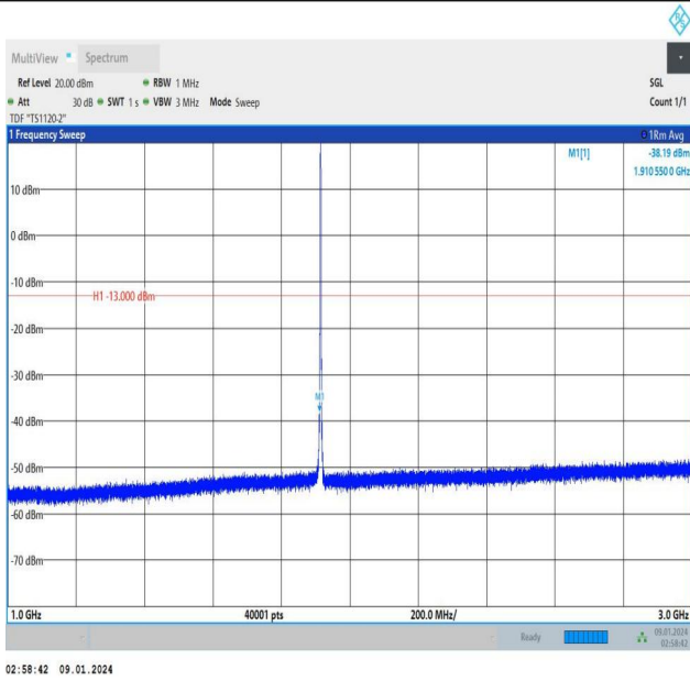
Band25_1.4MHz_16QAM_26683_6RB#0_1000~3000_1000~3000
