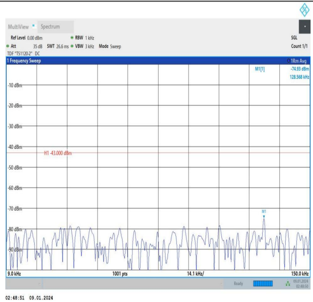
Band25_1.4MHz_16QAM_26047_1RB#5_0.009~0.15_0.009~0.15
