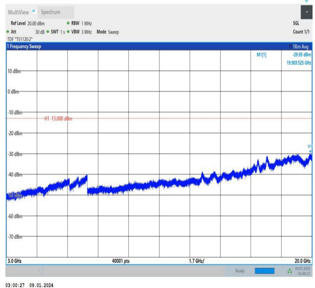
Band25_3MHz_16QAM_26055_1RB#0_3000~20000_3000~20000
