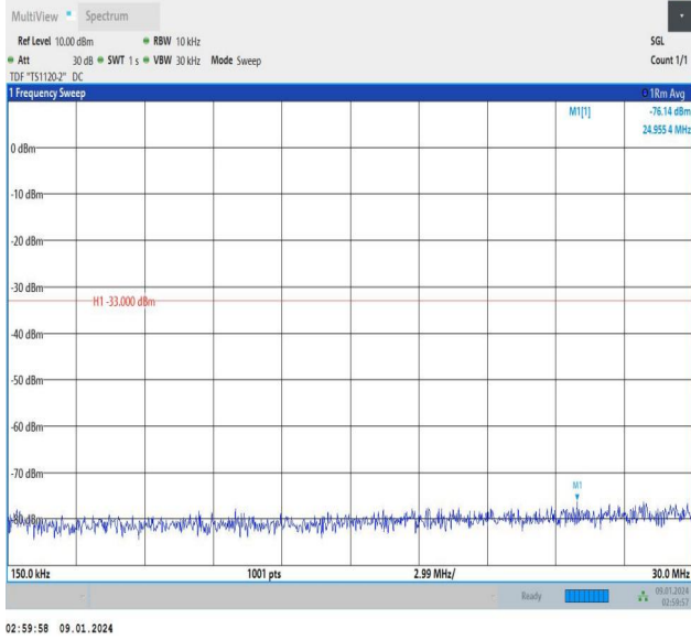
Band25_3MHz_16QAM_26055_1RB#0_0.15~30_0.15~30
