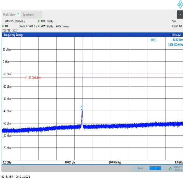
Band25_1.4MHz_16QAM_26365_1RB#0_1000~3000_1000~3000
