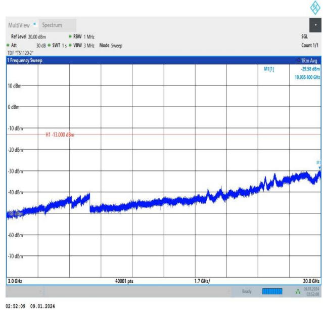
Band25_1.4MHz_16QAM_26365_1RB#0_3000~20000_3000~20000
