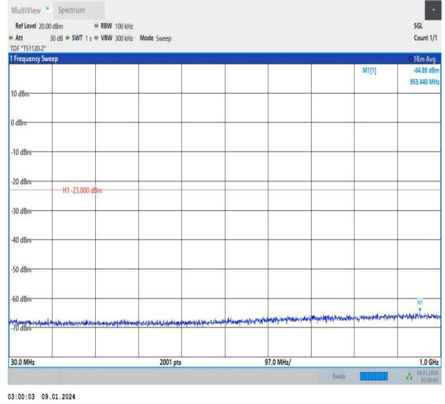
Band25_3MHz_16QAM_26055_1RB#0_30~1000_30~1000
