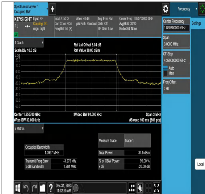
Band25-1.4MHz-QPSK-26047-6RB#0-PASS
