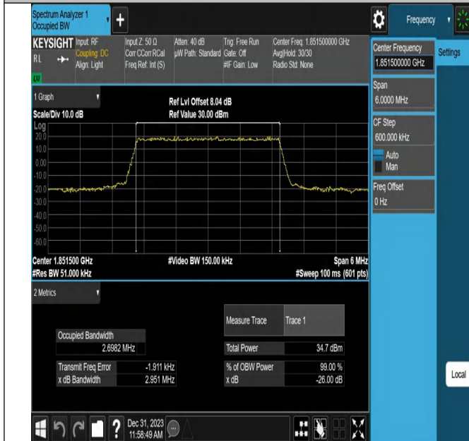
Band25-3MHz-QPSK-26055-15RB#0-PASS
