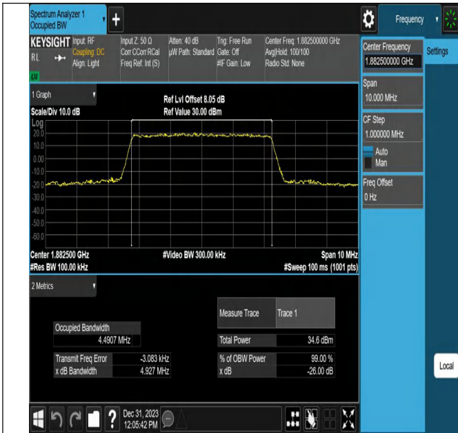
Band25-5MHz-16QAM-26365-25RB#0-PASS
