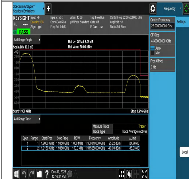
Band25_15MHz_16QAM_26615_1RB#0
