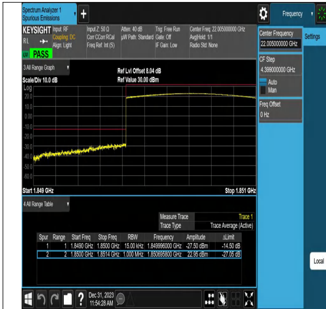
Band25_1.4MHz_16QAM_26047_6RB#0
