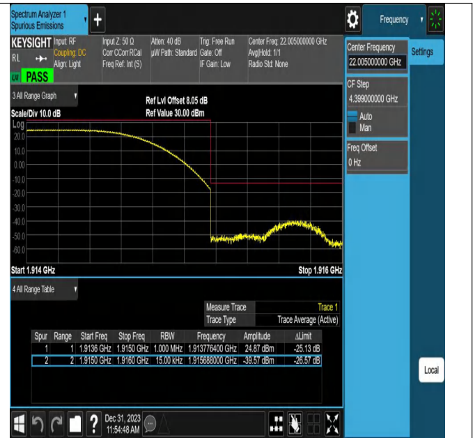
Band25_1.4MHz_16QAM_26683_1RB#0
