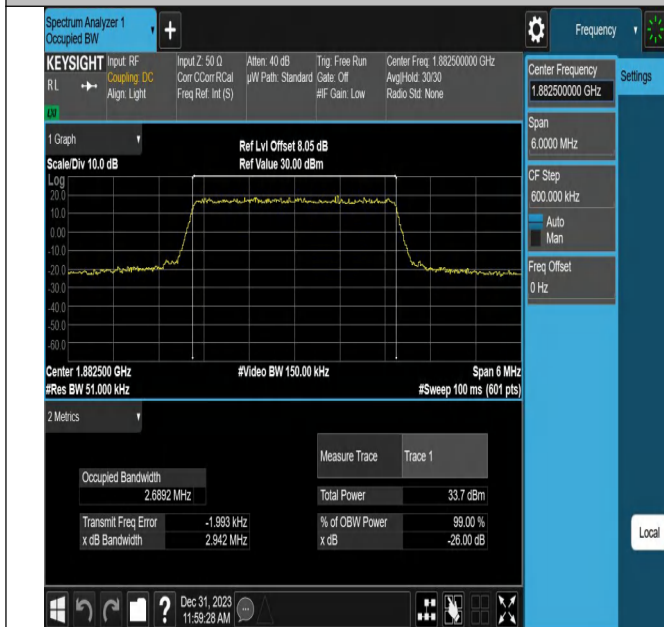
Band25-3MHz-16QAM-26365-15RB#0-PASS
