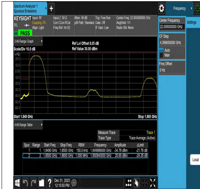
Band25_15MHz_16QAM_26115_1RB#0
