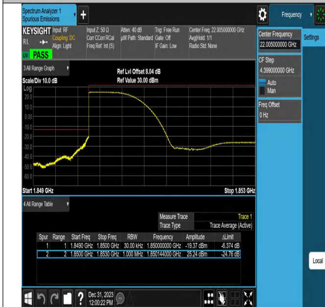
Band25_3MHz_16QAM_26055_1RB#0
