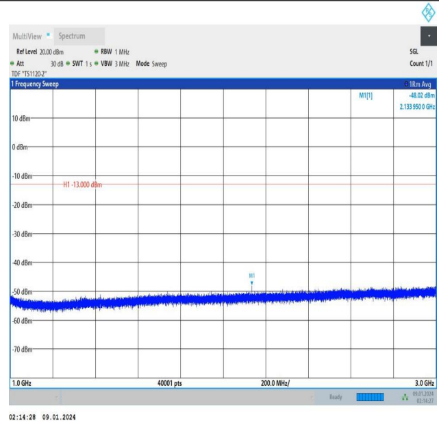
Band12_5MHz_QPSK_23155_1RB#0_1000~3000_1000~3000
