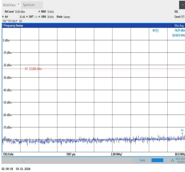
Band12_5MHz_16QAM_23035_1RB#24_0.15~30_0.15~30
