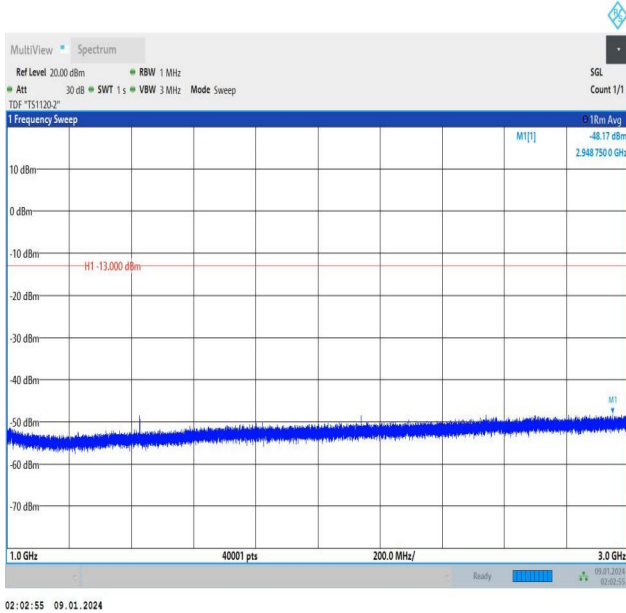
Band12_3MHz_16QAM_23165_1RB#0_1000~3000_1000~30
