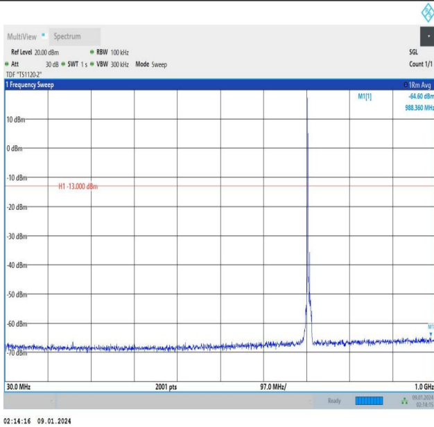
Band12_5MHz_QPSK_23155_1RB#0_30~1000_30~1000
