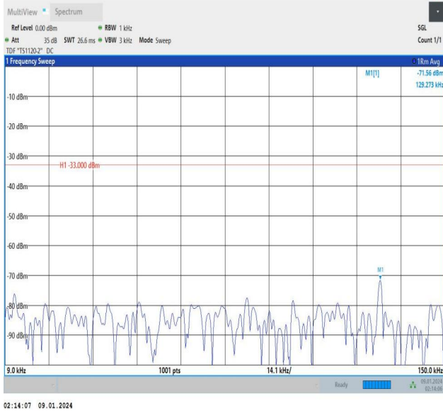
Band12_5MHz_QPSK_23155_1RB#0_0.009~0.15_0.009~0.1
