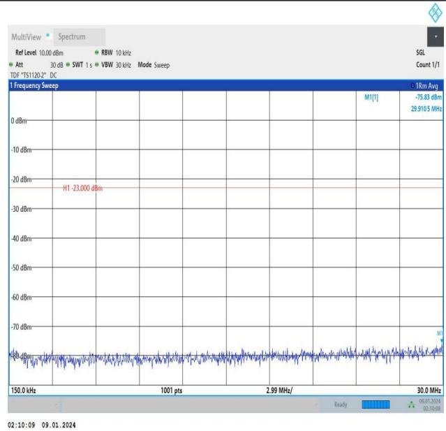
Band12_5MHz_QPSK_23095_1RB#0_0.15~30_0.15~30
