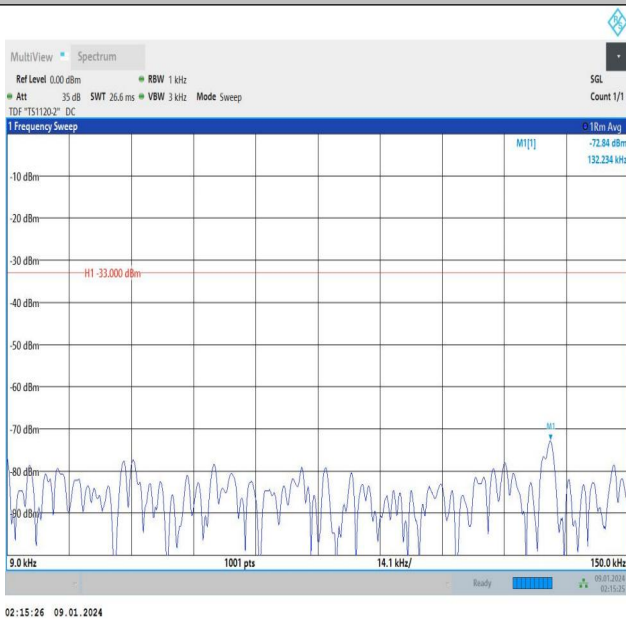
Band12_5MHz_QPSK_23155_1RB#24_0.009~0.15_0.009~0.15
