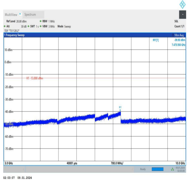
Band12_3MHz_16QAM_23165_1RB#0_3000~10000_3000~10
