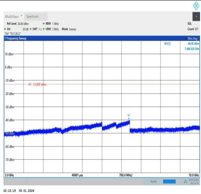
Band12_5MHz_16QAM_23155_1RB#0_3000~10000_3000~10000
