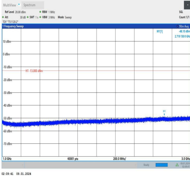
Band12_5MHz_16QAM_23035_25RB#0_1000~3000_1000~3000
