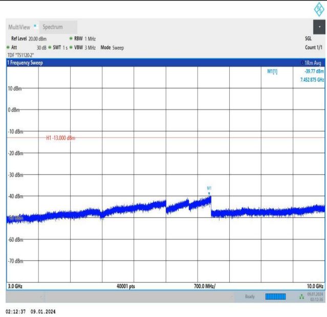
Band12_5MHz_16QAM_23095_1RB#24_3000~10000_3000~10000
