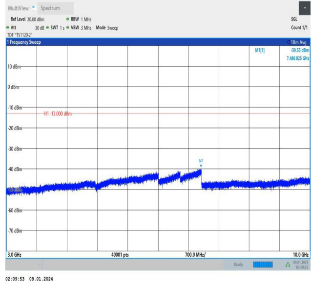
Band12_5MHz_16QAM_23035_25RB#0_3000~10000_3000~10000
