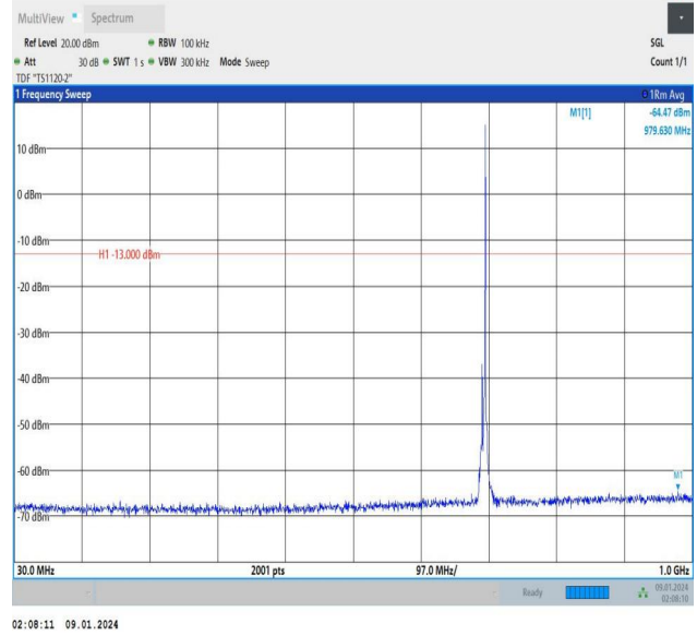
Band12_5MHz_16QAM_23035_1RB#24_30~1000_30~1000
