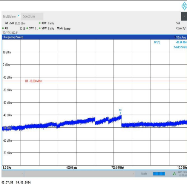
Band12_5MHz_QPSK_23035_1RB#24_3000~10000_3000~1 0000
