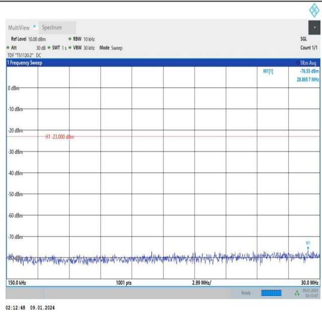
Band12_5MHz_QPSK_23095_25RB#0_0.15~30_0.15~30
