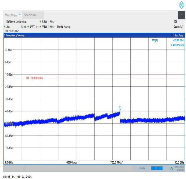
Band12_3MHz_16QAM_23165_15RB#0_3000~10000_3000~10000
