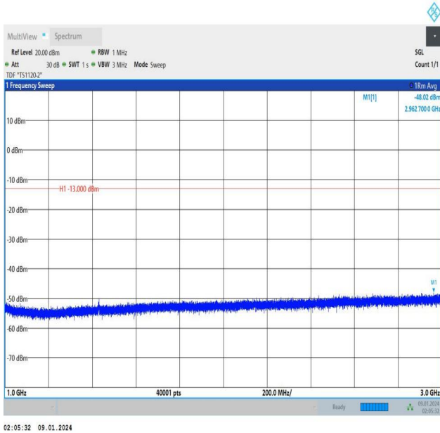
Band12_3MHz_16QAM_23165_15RB#0_1000~3000_1000~3000
