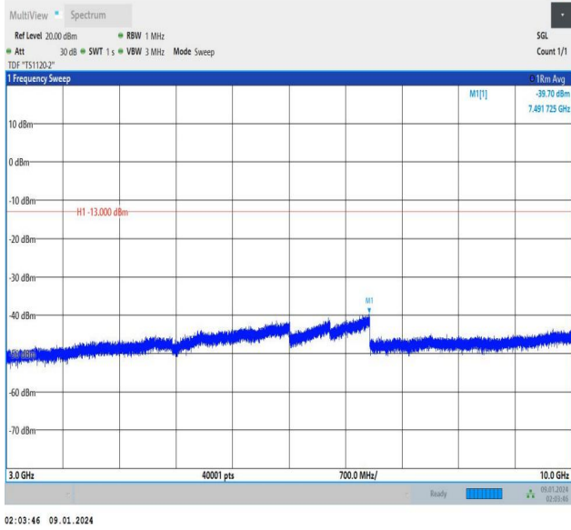
Band12_3MHz_QPSK_23165_1RB#14_3000~10000_3000~10000
