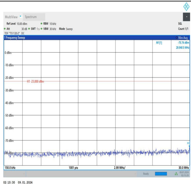
Band12_5MHz_QPSK_23155_1RB#24_0.15~30_0.15~30
