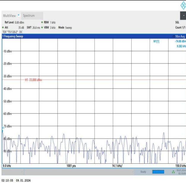
Band12_5MHz_QPSK_23095_1RB#0_0.009~0.15_0.009~0.15
