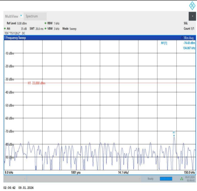
Band12_5MHz_16QAM_23035_1RB#0_0.009~0.15_0.009~0.15
