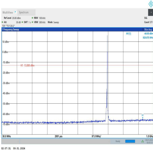
Band12_5MHz_QPSK_23035_1RB#24_30~1000_30~1000
