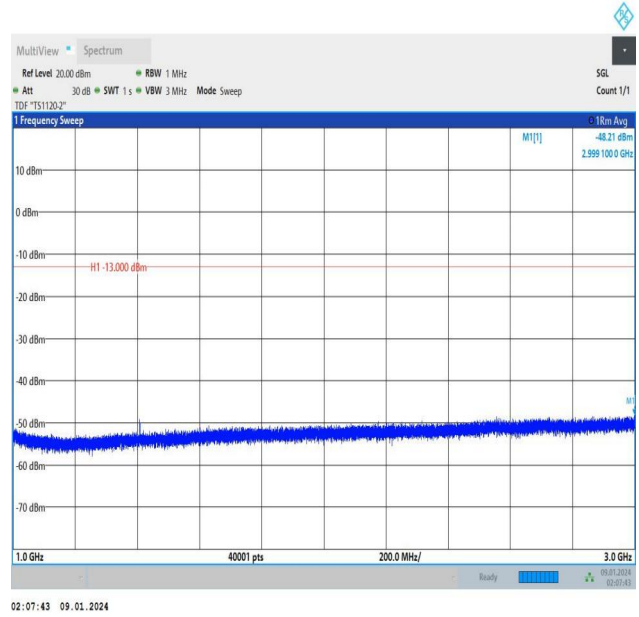
Band12_5MHz_QPSK_23035_1RB#24_1000~3000_1000~300 0
