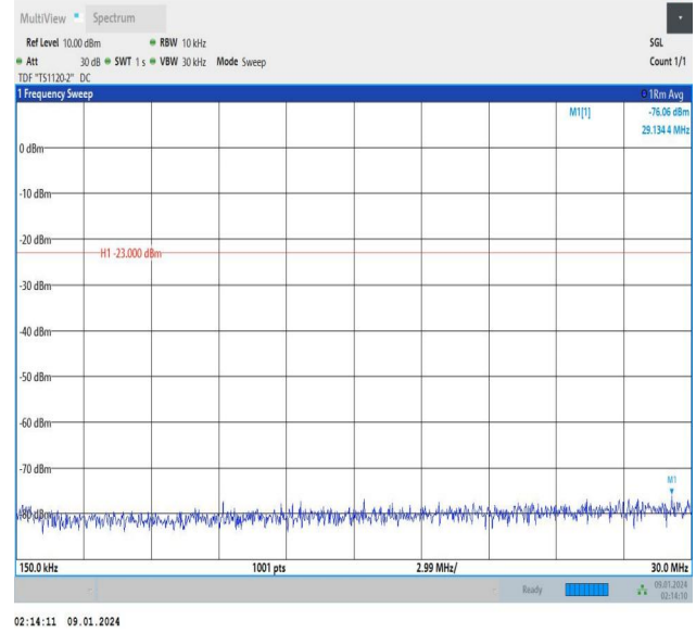
Band12_5MHz_QPSK_23155_1RB#0_0.15~30_0.15~30
