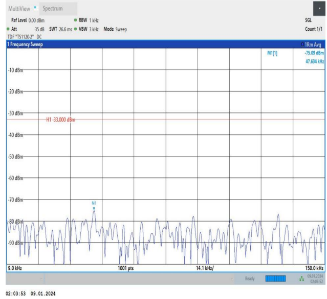
Band12_3MHz_16QAM_23165_1RB#14_0.009~0.15_0.009~0.15
