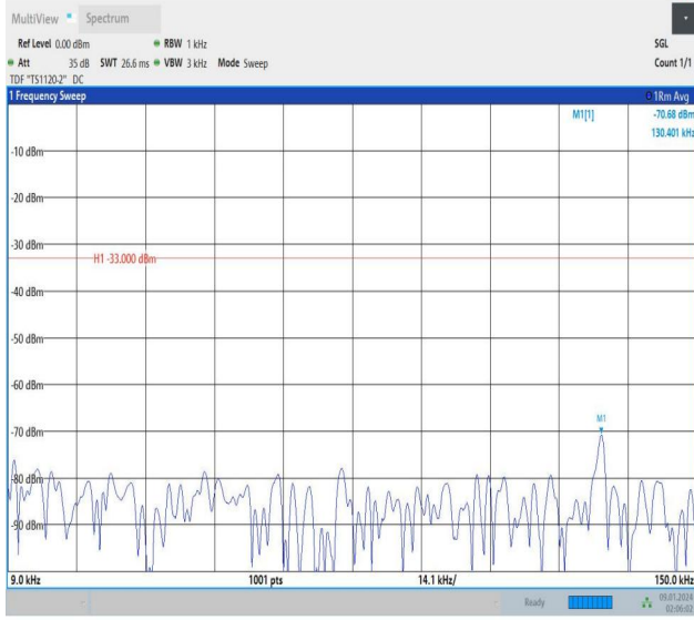
Band12_5MHz_QPSK_23035_1RB#0_0.009~0.15_0.009~0.1
