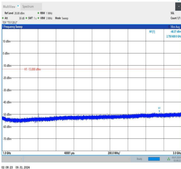
Band12_5MHz_16QAM_23035_1RB#24_1000~3000_1000~3000
