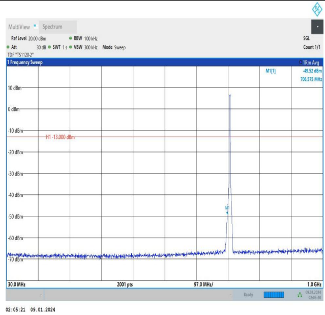
Band12_3MHz_16QAM_23165_15RB#0_30~1000_30~1000
