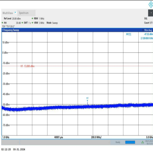
Band12_5MHz_16QAM_23095_1RB#24_1000~3000_1000~3000
