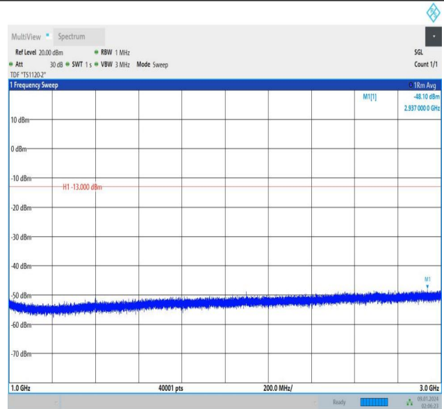
Band12_5MHz_QPSK_23035_1RB#0_1000~3000_1000~3000
