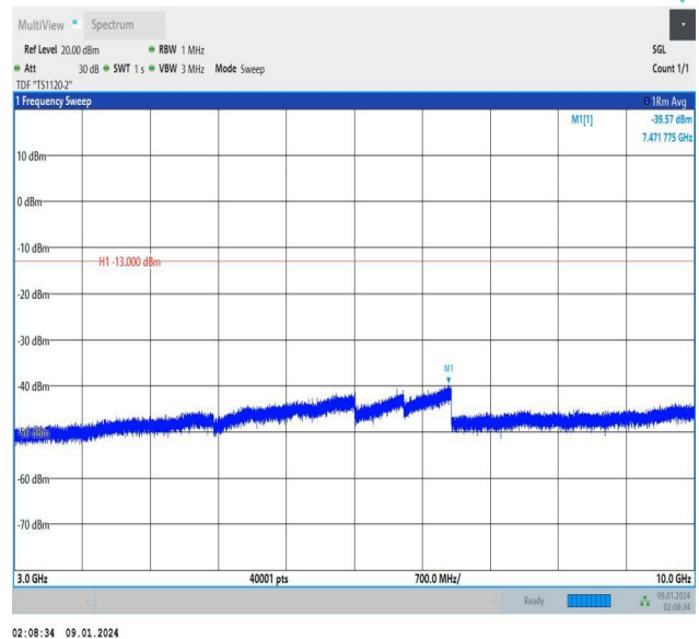
Band12_5MHz_16QAM_23035_1RB#24_3000~10000_3000~10000
