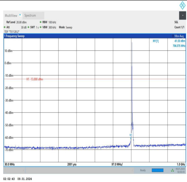
Band12_3MHz_16QAM_23165_1RB#0_30~1000_30~1000
