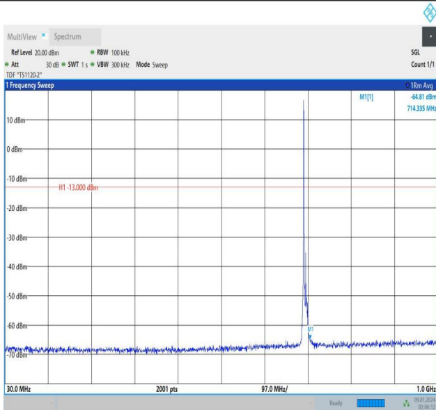
Band12_5MHz_QPSK_23035_1RB#0_30~1000_30~1000
