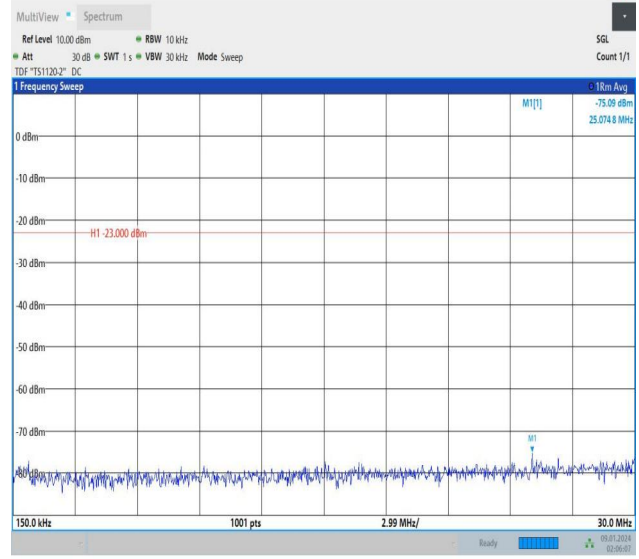
Band12_5MHz_QPSK_23035_1RB#0_0.15~30_0.15~30
