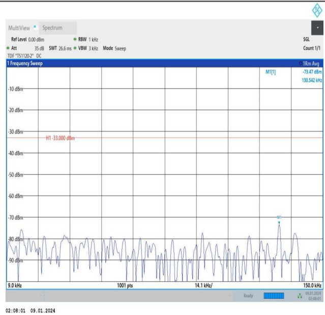
Band12_5MHz_16QAM_23035_1RB#24_0.009~0.15_0.009~0.15 15
