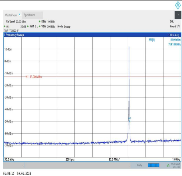
Band12_1.4MHz_16QAM_23173_6RB#0_30~1000_30~1000
