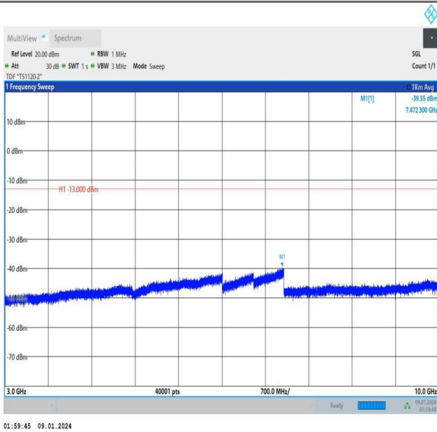
Band12_3MHz_QPSK_23095_1RB#14_3000~10000_3000~1 0000
