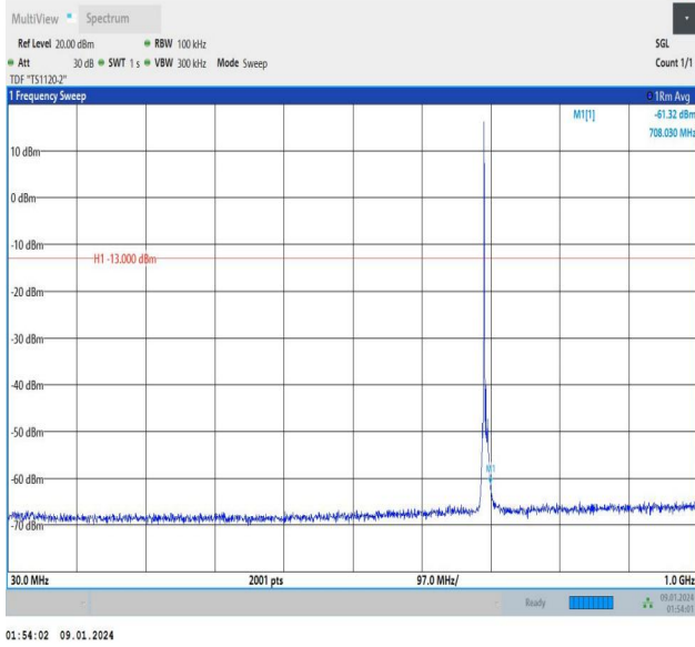
Band12_3MHz_QPSK_23025_1RB#0_30~1000_30~1000
