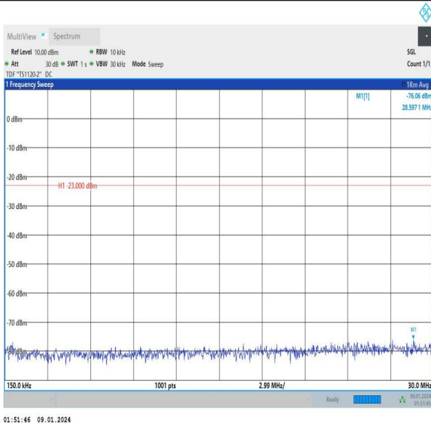
Band12_1.4MHz_16QAM_23173_1RB#5_0.15~30_0.15~30
