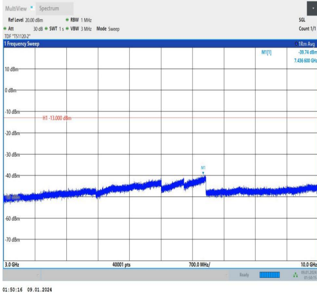
Band12_1.4MHz_QPSK_23173_1RB#0_3000~10000_3000~10000
