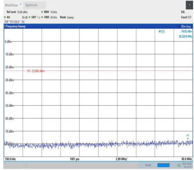
Band12_3MHz_QPSK_23095_1RB#0_0.15~30_0.15~30
