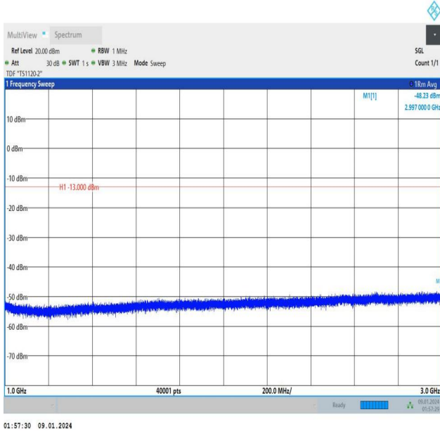
Band12_3MHz_16QAM_23025_15RB#0_1000~3000_1000~3000
