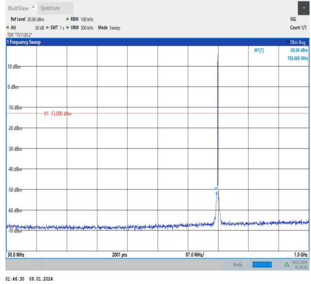
Band12_1.4MHz_16QAM_23095_1RB#0_30~1000_30~1000
