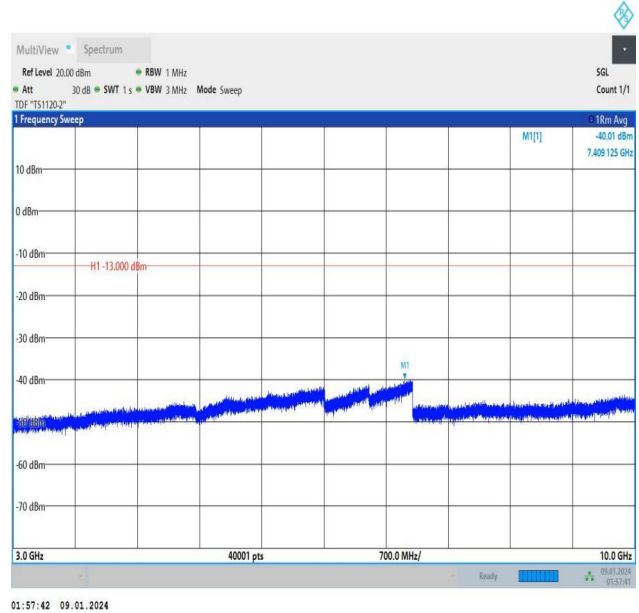
Band12_3MHz_16QAM_23025_15RB#0_3000~10000_3000~10000
