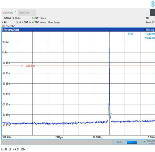
Band12_3MHz_QPSK_23095_1RB#14_30~1000_30~1000
