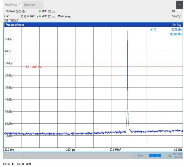
Band12_1.4MHz_16QAM_23017_1RB#5_30~1000_30~1000
