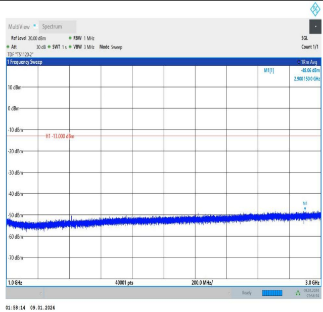
Band12_3MHz_QPSK_23095_1RB#0_1000~3000_1000~3000
