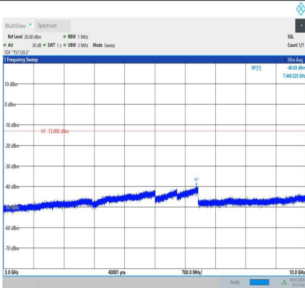
Band12_3MHz_QPSK_23025_15RB#0_3000~10000_3000~1 0000
