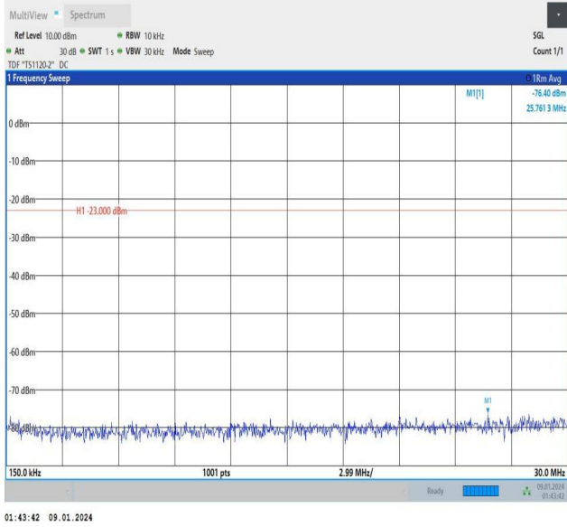
Band12_1.4MHz_16QAM_23017_1RB#5_0.15~30_0.15~30
