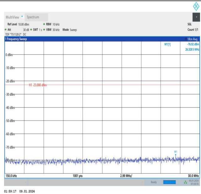
Band12_3MHz_QPSK_23095_1RB#14_0.15~30_0.15~30
