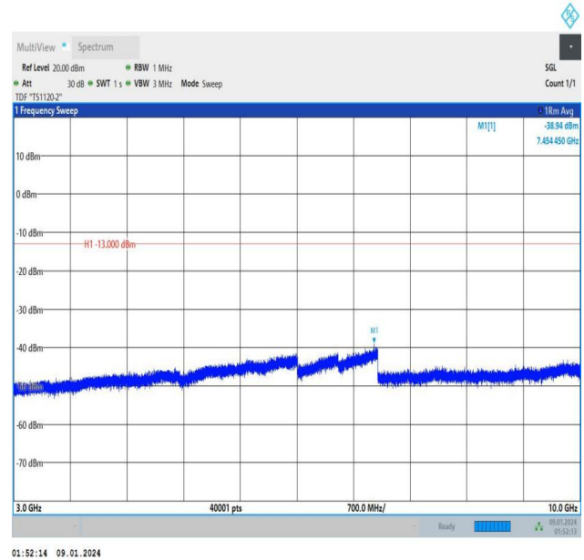
Band12_1.4MHz_16QAM_23173_1RB#5_3000~10000_3000~10000
