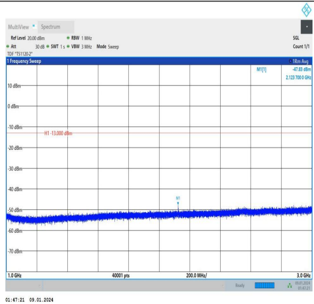
Band12_1.4MHz_QPSK_23095_1RB#5_1000~3000_1000~3000
