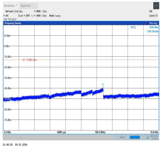
Band12_1.4MHz_16QAM_23095_1RB#0_3000~10000_3000~10000
