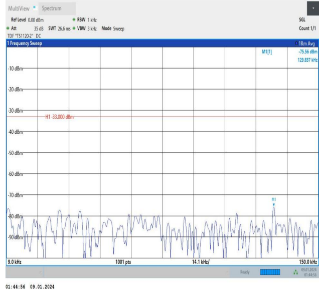
Band12_1.4MHz_16QAM_23017_6RB#0_0.009~0.15_0.009~0.15
