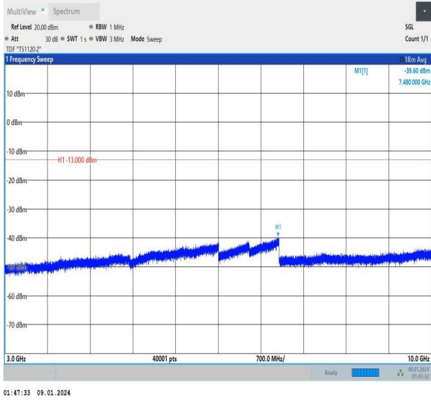
Band12_1.4MHz_QPSK_23095_1RB#5_3000~10000_3000~10000
