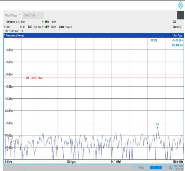
Band12_3MHz_QPSK_23025_15RB#0_1000~3000_1000~300 0
