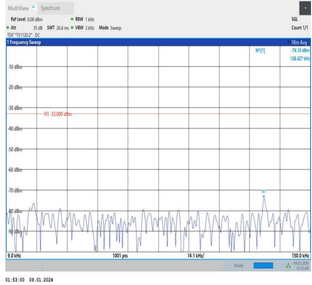
Band12_1.4MHz_16QAM_23173_6RB#0_0.009~0.15_0.009~0.15
