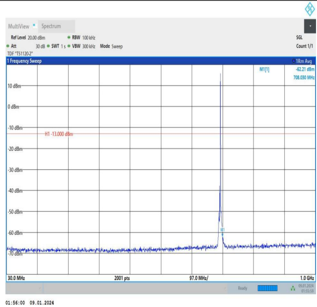
Band12_3MHz_16QAM_23025_1RB#14_30~1000_30~1000
