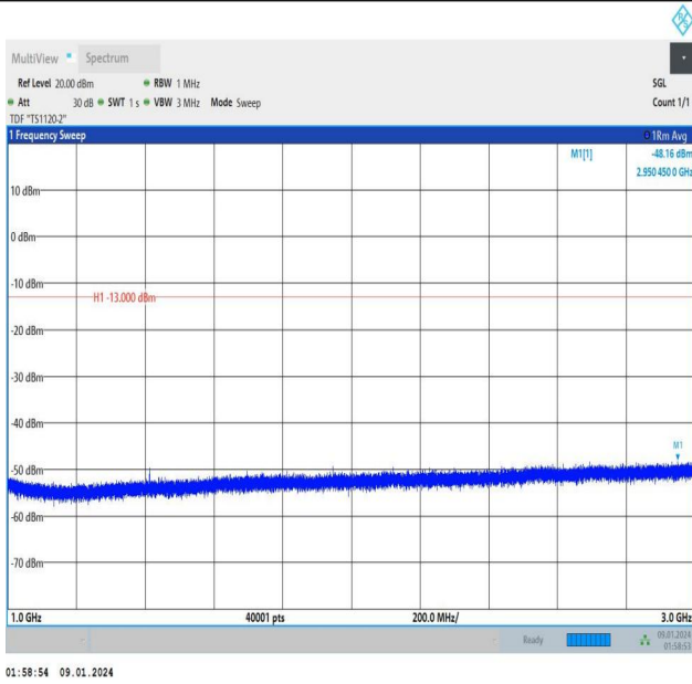
Band12_3MHz_16QAM_23095_1RB#0_1000~3000_1000~3000
