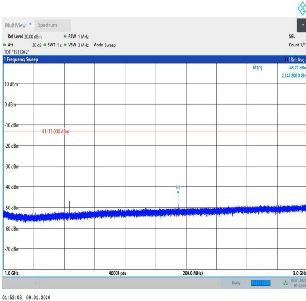
Band12_1.4MHz_16QAM_23173_1RB#5_1000~3000_1000~3000
