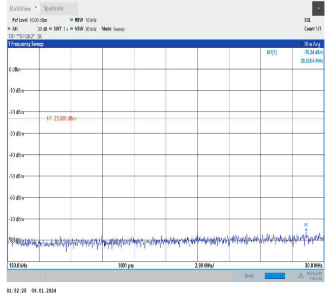
Band12_1.4MHz_QPSK_23173_6RB#0_0.15~30_0.15~30
