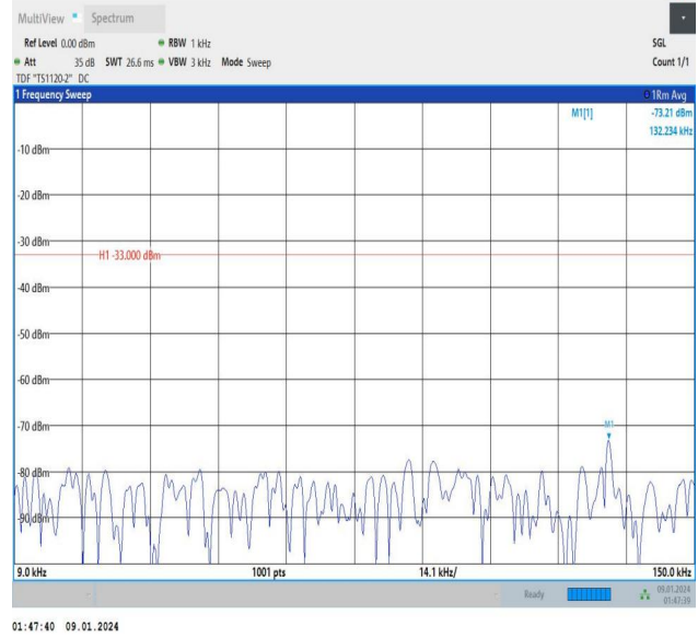
Band12_1.4MHz_16QAM_23095_1RB#5_0.009~0.15_0.009~0.15
