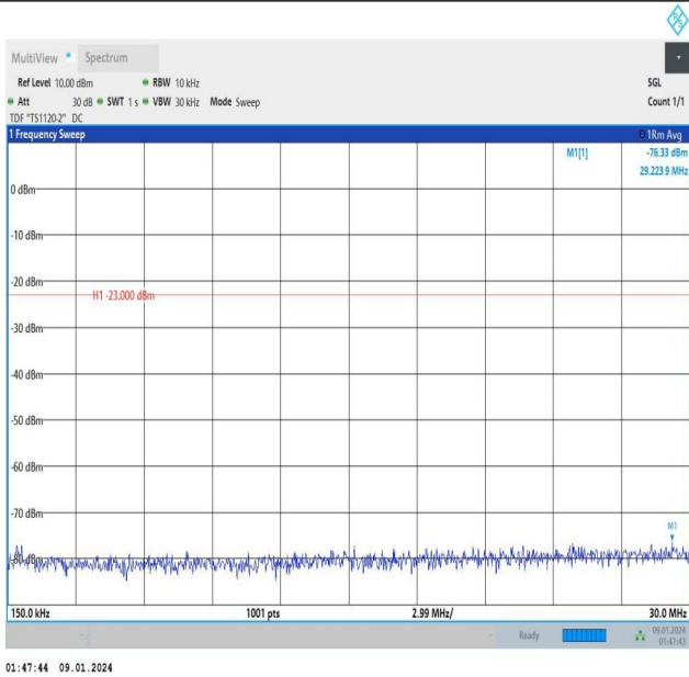
Band12_1.4MHz_16QAM_23095_1RB#5_0.15~30_0.15~30
