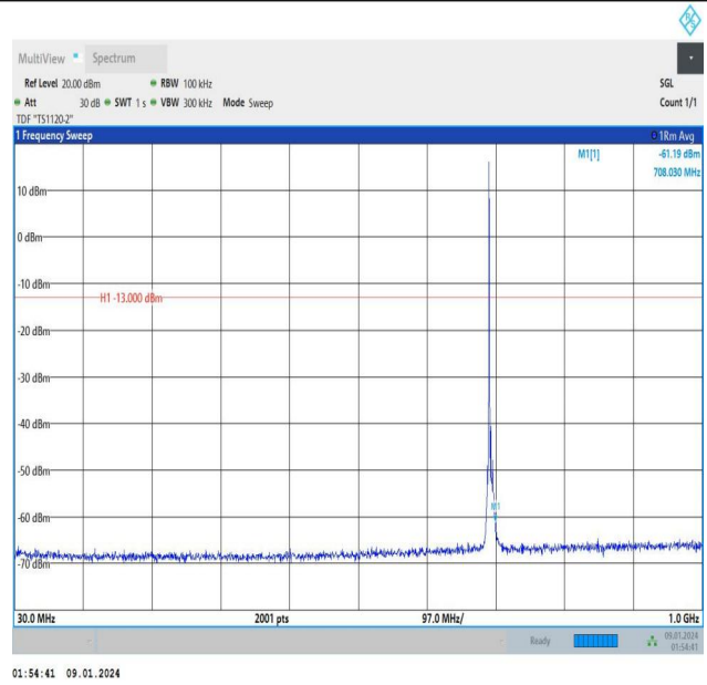
Band12_3MHz_16QAM_23025_1RB#0_30~1000_30~1000
