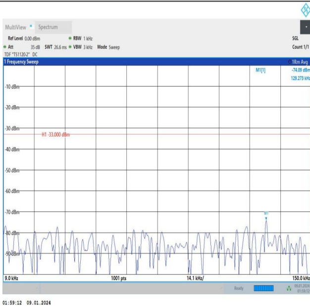
Band12_3MHz_QPSK_23095_1RB#14_0.009~0.15_0.009~0.15
