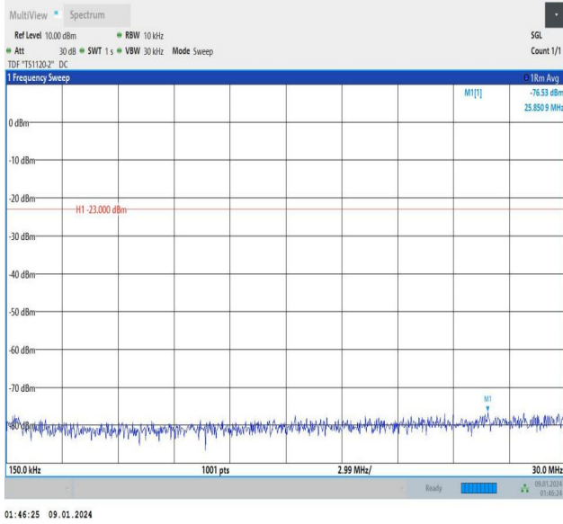
Band12_1.4MHz_16QAM_23095_1RB#0_0.15~30_0.15~30
