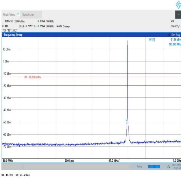
Band12_1.4MHz_QPSK_23095_1RB#0_30~1000_30~1000
