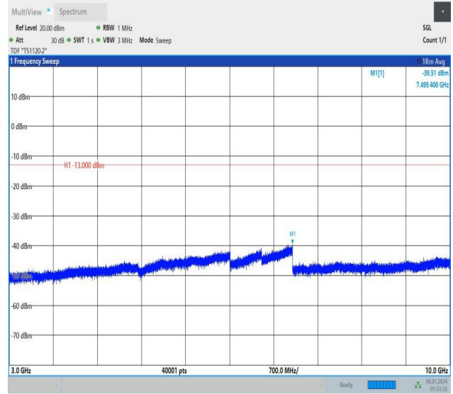
Band12_1.4MHz_16QAM_23173_6RB#0_3000~10000_3000~10000
