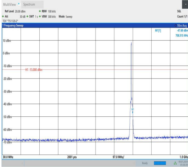
Band12_3MHz_QPSK_23025_15RB#0_30~1000_30~1000
