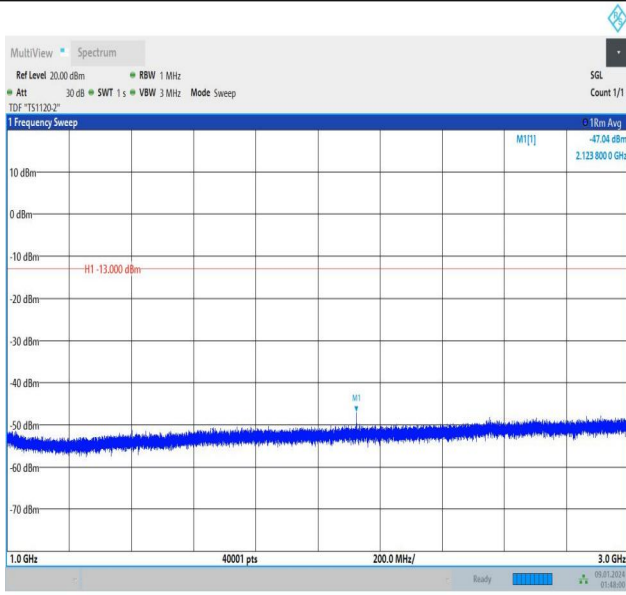
Band12_1.4MHz_16QAM_23095_1RB#5_1000~3000_1000~3000
