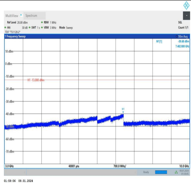
Band12_3MHz_16QAM_23095_1RB#0_3000~10000_3000~10000
