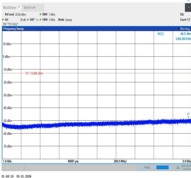
Band12_1.4MHz_16QAM_23095_6RB#0_1000~3000_1000~3000
