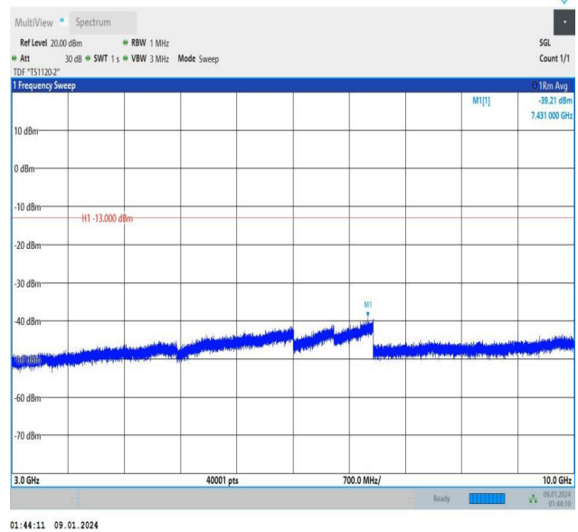
Band12_1.4MHz_16QAM_23017_1RB#5_3000~10000_3000~10000
