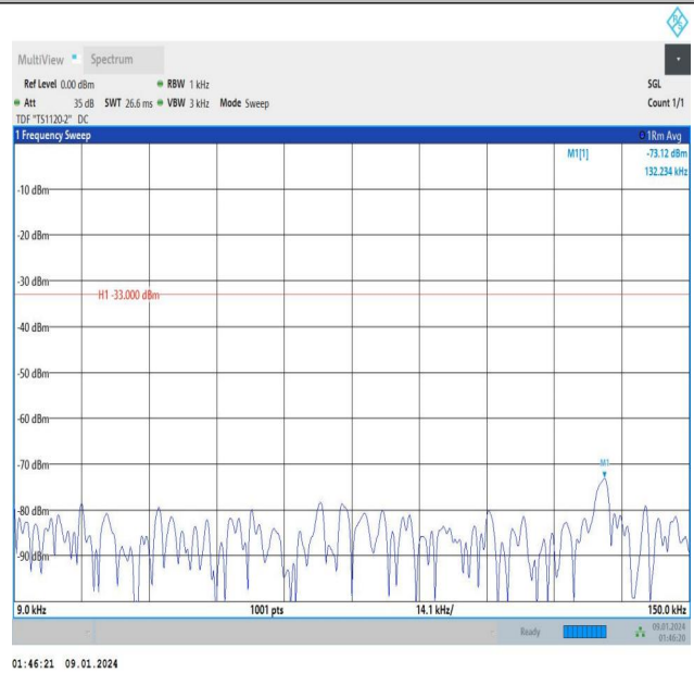
Band12_1.4MHz_16QAM_23095_1RB#0_0.009~0.15_0.009~0.15
