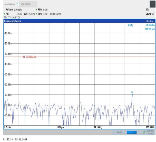
Band12_1.4MHz_16QAM_23173_1RB#0_0.009~0.15_0.009~0.15
