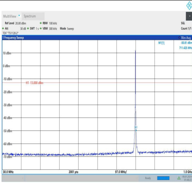
Band12_1.4MHz_QPSK_23095_6RB#0_30~1000_30~1000
