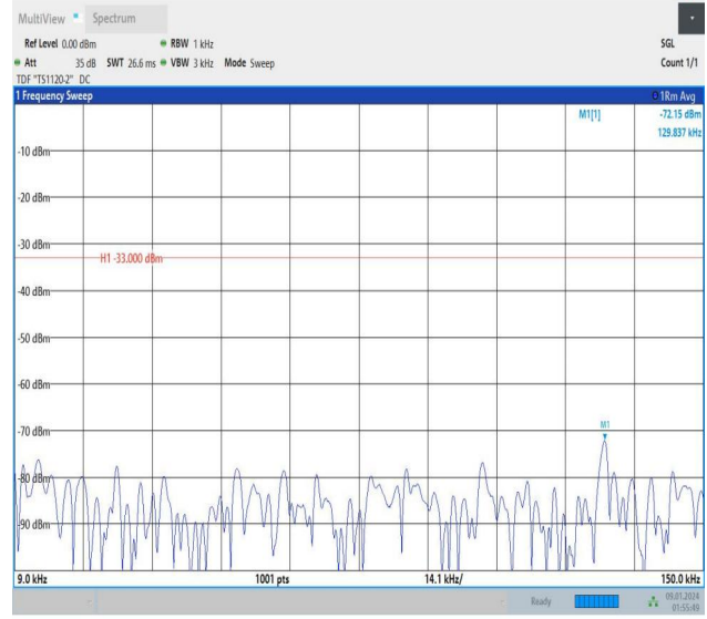
Band12_3MHz_16QAM_23025_1RB#14_0.009~0.15_0.009~0.15
