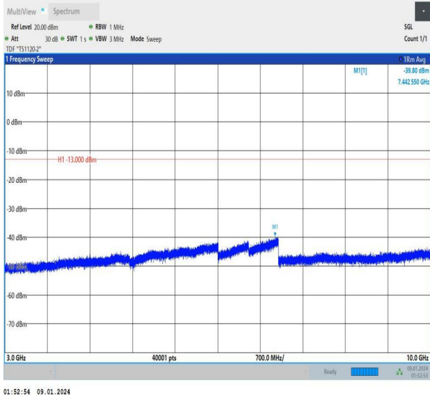
Band12_1.4MHz_QPSK_23173_6RB#0_3000~10000_3000~10000
