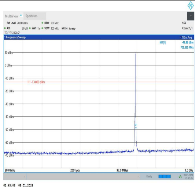
Band12_1.4MHz_16QAM_23017_6RB#0_30~1000_30~1000
