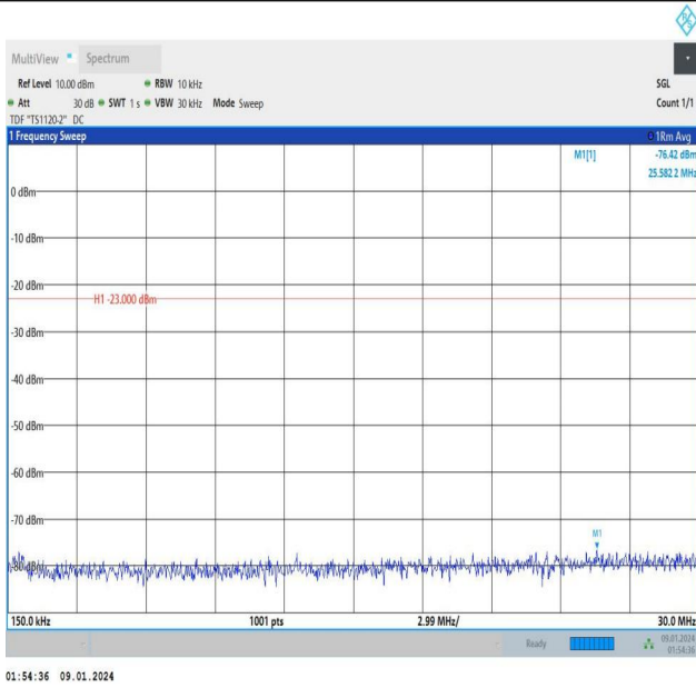
Band12_3MHz_16QAM_23025_1RB#0_0.15~30_0.15~30
