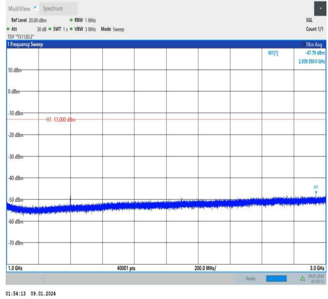
Band12_3MHz_QPSK_23025_1RB#0_1000~3000_1000~3000
