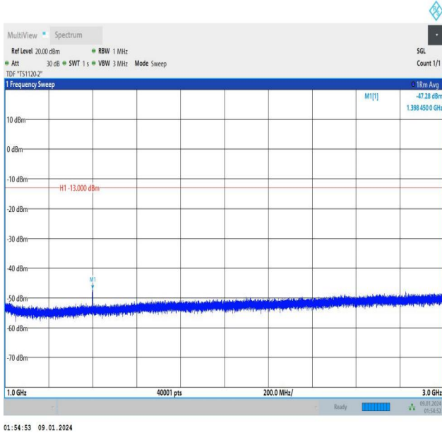
Band12_3MHz_16QAM_23025_1RB#0_1000~3000_1000~30
