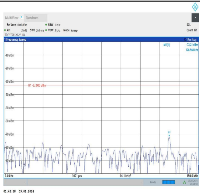
Band12_1.4MHz_16QAM_23095_6RB#0_0.009~0.15_0.009~0.15
