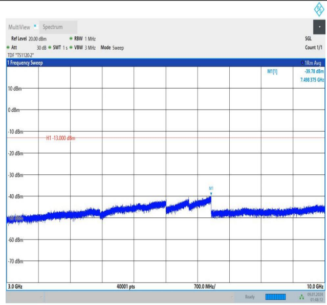
Band12_1.4MHz_16QAM_23095_1RB#5_3000~10000_3000~10000
