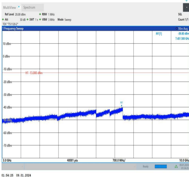
Band12_3MHz_QPSK_23025_1RB#0_3000~10000_3000~10000
