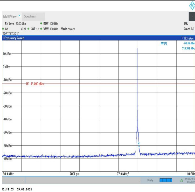
Band12_3MHz_QPSK_23095_1RB#0_30~1000_30~1000
