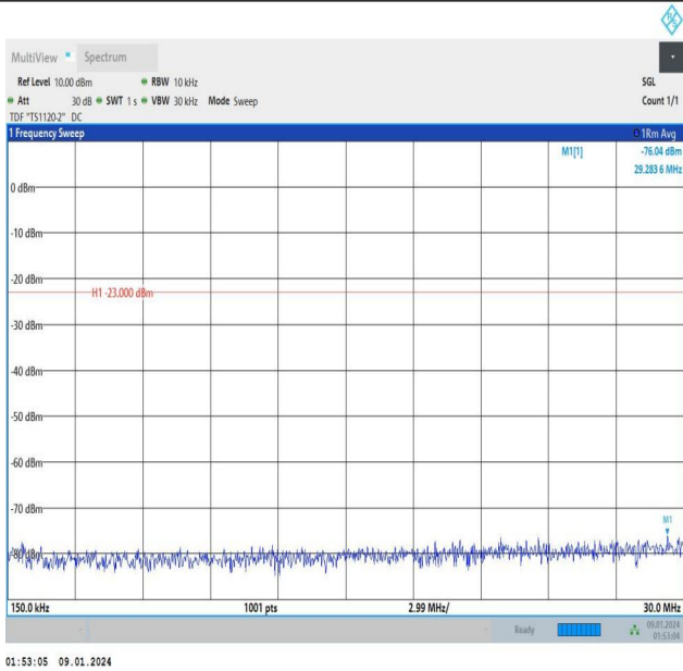
Band12_1.4MHz_16QAM_23173_6RB#0_0.15~30_0.15~30
