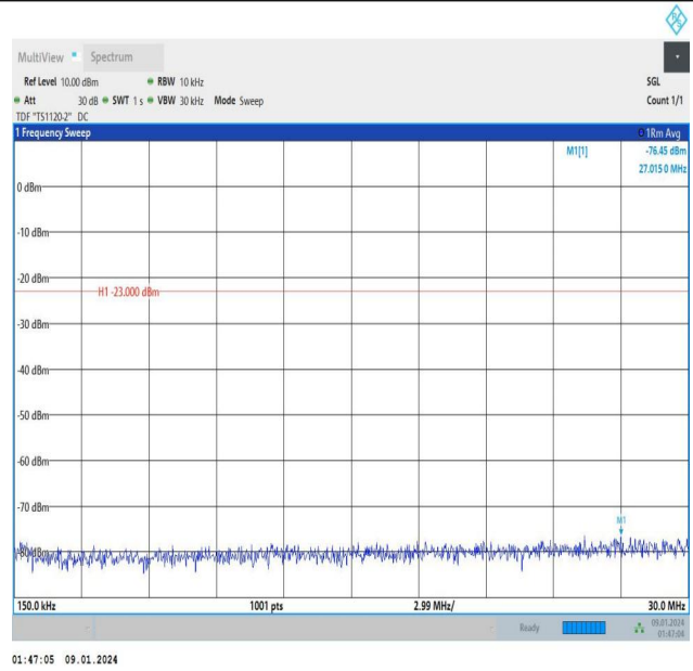
Band12_1.4MHz_QPSK_23095_1RB#5_0.15~30_0.15~30
