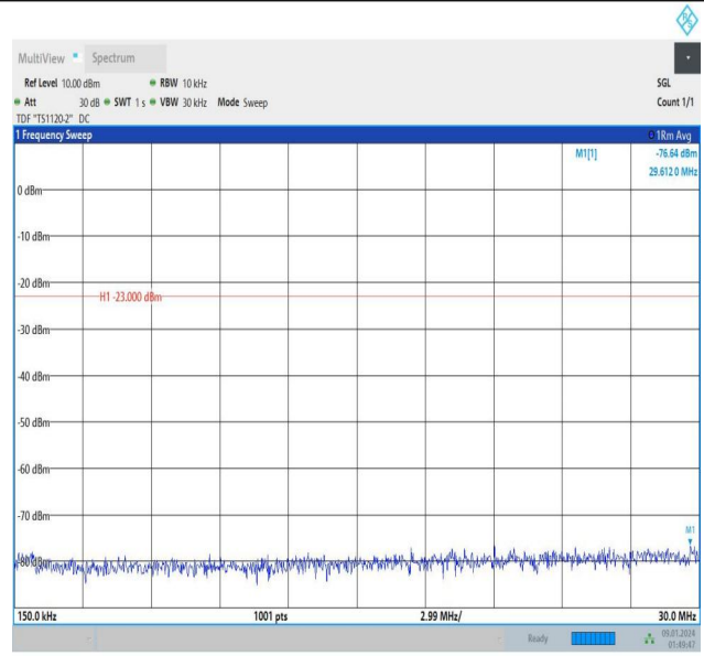
Band12_1.4MHz_QPSK_23173_1RB#0_0.15~30_0.15~30
