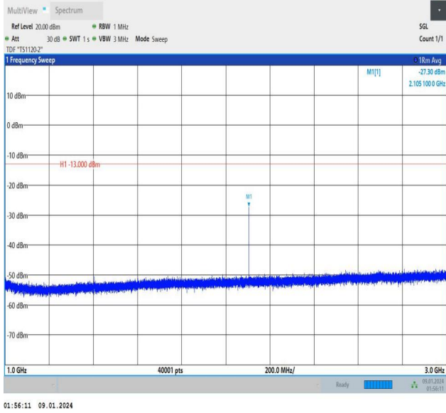
Band12_3MHz_16QAM_23025_1RB#14_1000~3000_1000~3000
