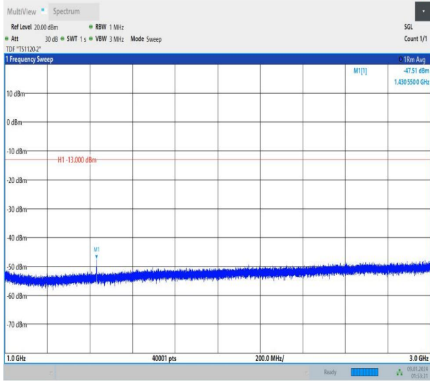
Band12_1.4MHz_16QAM_23173_6RB#0_1000~3000_1000~3000
