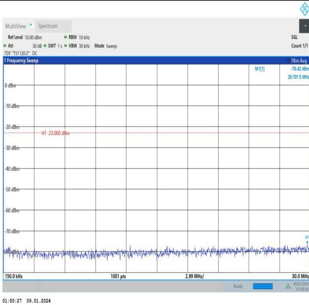
Band12_1.4MHz_16QAM_23173_1RB#0_0.15~30_0.15~30
