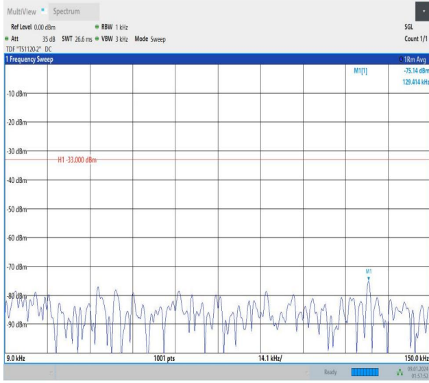
Band12_3MHz_QPSK_23095_1RB#0_0.009~0.15_0.009~0.1
