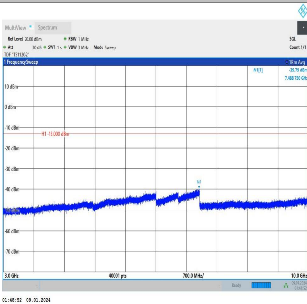
Band12_1.4MHz_QPSK_23095_6RB#0_3000~10000_3000~10000
