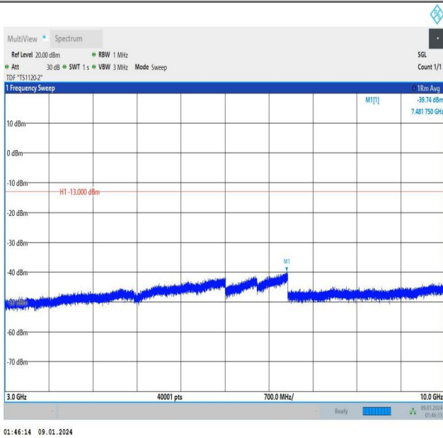
Band12_1.4MHz_QPSK_23095_1RB#0_3000~10000_3000~10000
