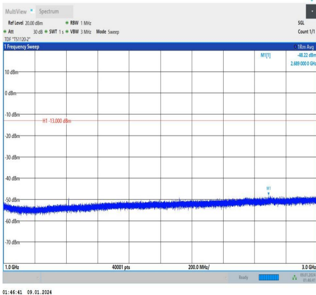
Band12_1.4MHz_16QAM_23095_1RB#0_1000~3000_1000~3000
