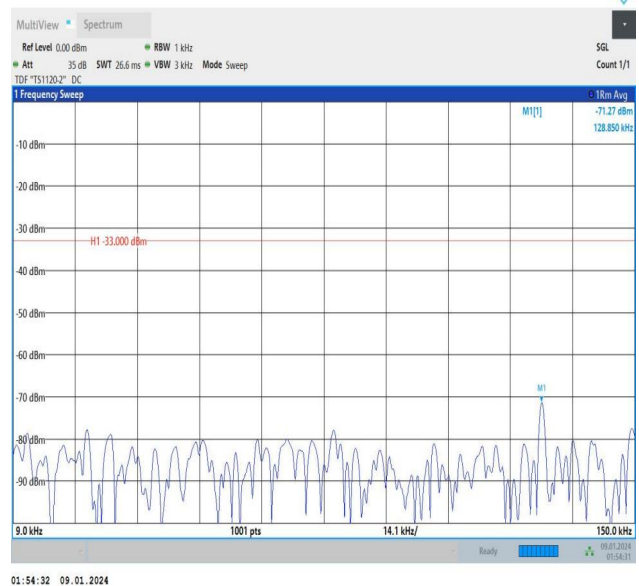
Band12_3MHz_16QAM_23025_1RB#0_0.009~0.15_0.009~0.1
