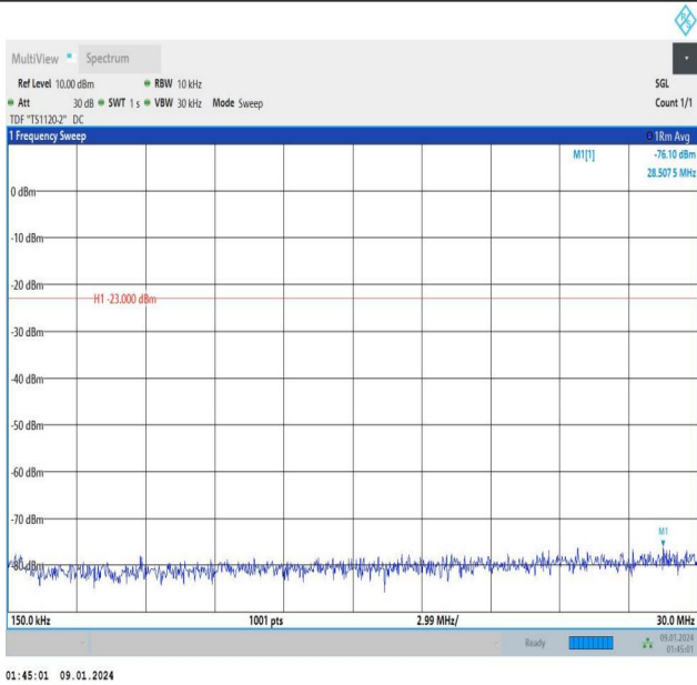
Band12_1.4MHz_16QAM_23017_6RB#0_0.15~30_0.15~30
