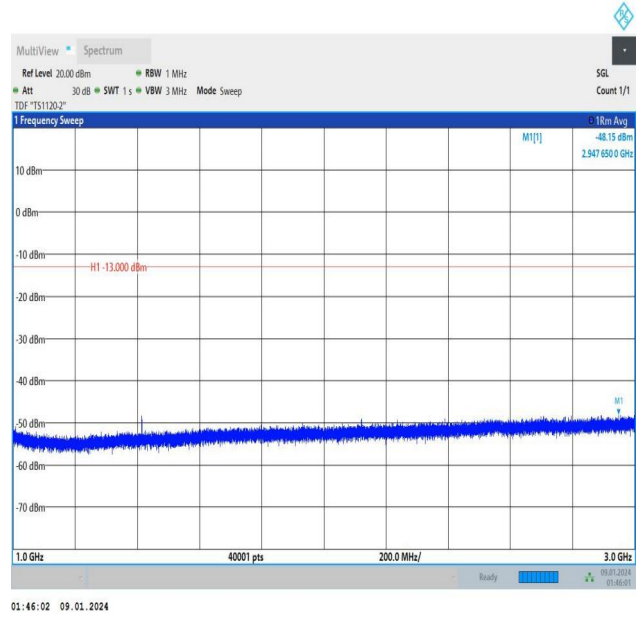
Band12_1.4MHz_QPSK_23095_1RB#0_1000~3000_1000~3000
