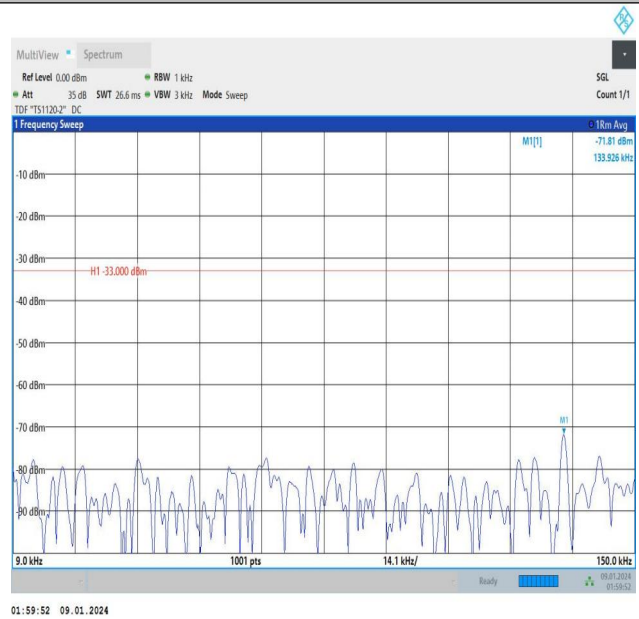
Band12_3MHz_16QAM_23095_1RB#14_0.009~0.15_0.009~0. 15
