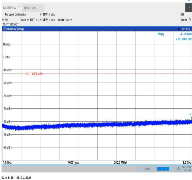
Band12_1.4MHz_16QAM_23017_1RB#5_1000~3000_1000~3000
