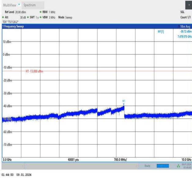
Band12_1.4MHz_QPSK_23017_6RB#0_3000~10000_3000~10000
