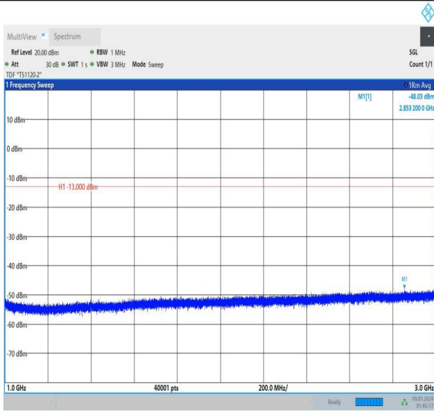
Band12_1.4MHz_16QAM_23017_6RB#0_1000~3000_1000~3000
