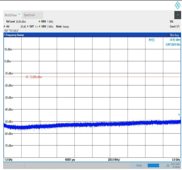
Band12_1.4MHz_QPSK_23095_6RB#0_1000~3000_1000~3000
