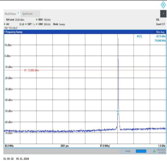
Band12_1.4MHz_16QAM_23173_1RB#0_30~1000_30~1000
