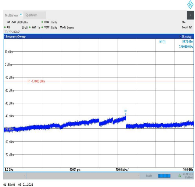
Band12_3MHz_16QAM_23025_1RB#0_3000~10000_3000~10
