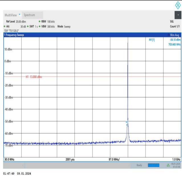
Band12_1.4MHz_16QAM_23095_1RB#5_30~1000_30~1000
