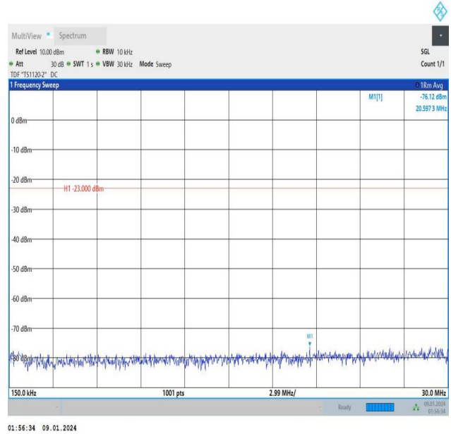
Band12_3MHz_QPSK_23025_15RB#0_0.15~30_0.15~30
