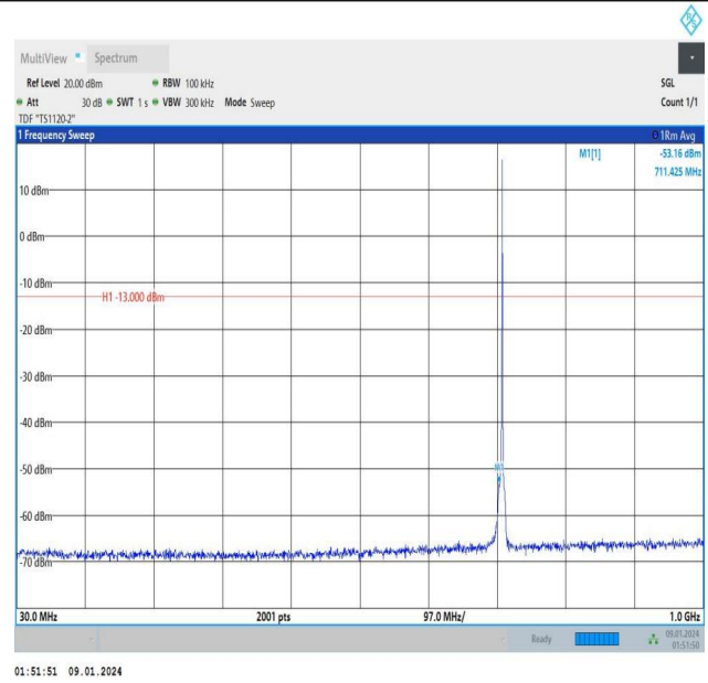
Band12_1.4MHz_16QAM_23173_1RB#5_30~1000_30~1000
