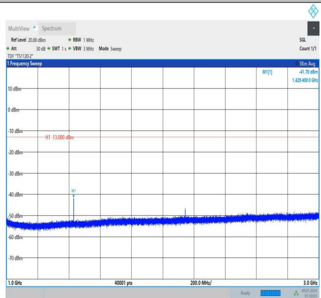
Band12_1.4MHz_QPSK_23173_1RB#0_1000~3000_1000~3000
