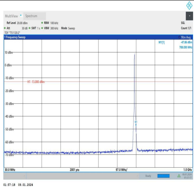
Band12_3MHz_16QAM_23025_15RB#0_30~1000_30~1000
