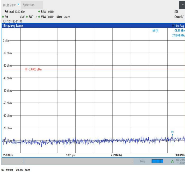
Band12_1.4MHz_16QAM_23095_6RB#0_0.15~30_0.15~30
