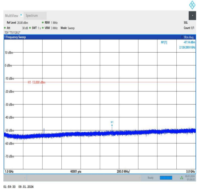
Band12_3MHz_QPSK_23095_1RB#14_1000~3000_1000~300 0
