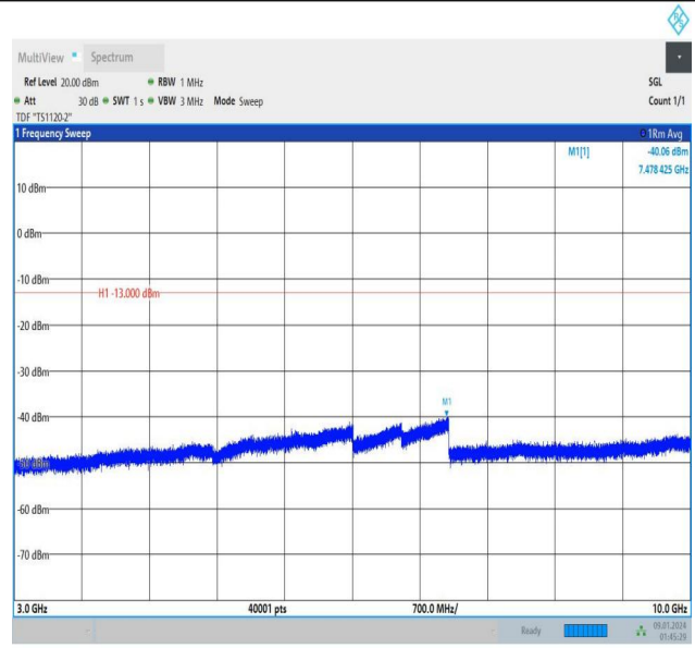
Band12_1.4MHz_16QAM_23017_6RB#0_3000~10000_3000~10000
