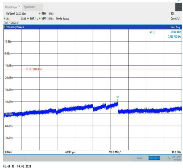
Band12_1.4MHz_16QAM_23095_6RB#0_3000~10000_3000~10000
