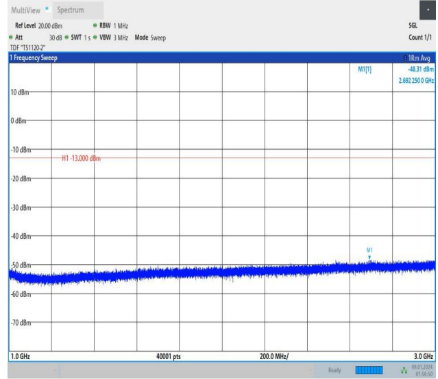
Band12_3MHz_QPSK_23025_15RB#0_1000~3000_1000~300 0
