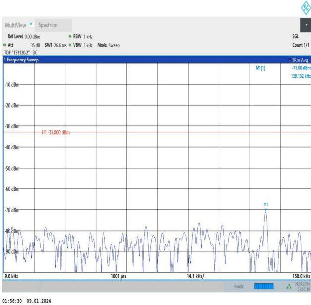
Band12_3MHz_QPSK_23025_15RB#0_0.009~0.15_0.009~0.15
