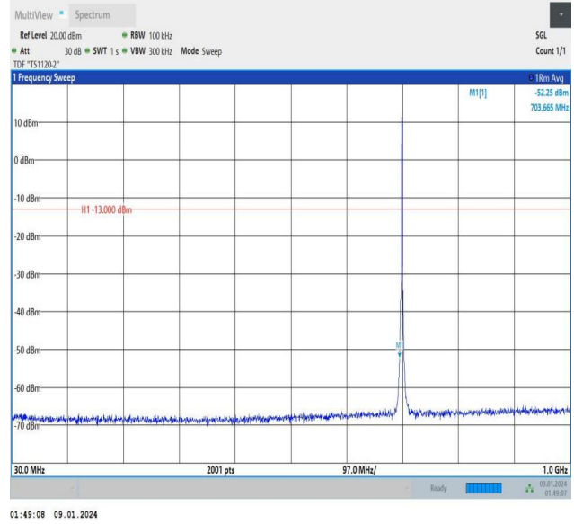
Band12_1.4MHz_16QAM_23095_6RB#0_30~1000_30~1000
