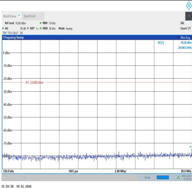
Band12_3MHz_16QAM_23025_1RB#14_0.15~30_0.15~30
