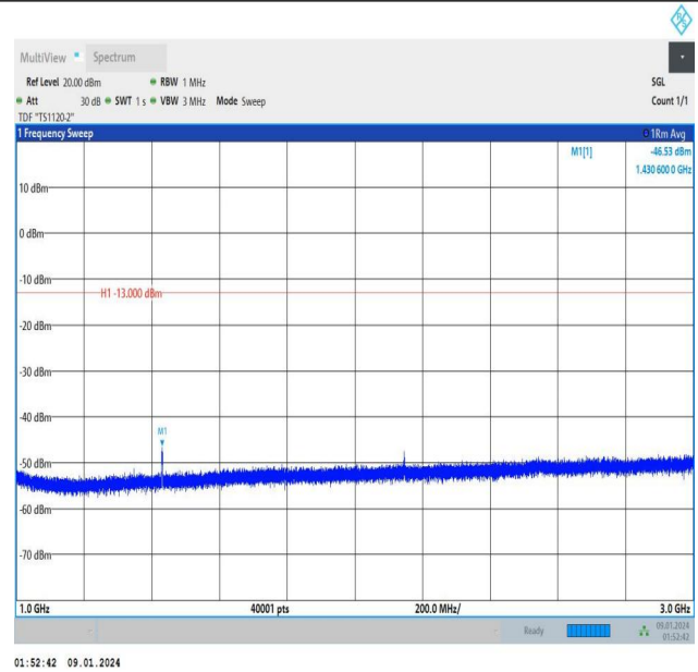
Band12_1.4MHz_QPSK_23173_6RB#0_1000~3000_1000~3000
