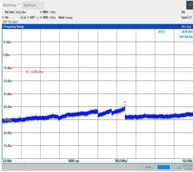
Band12_3MHz_QPSK_23025_1RB#14_3000~10000_3000~10000
