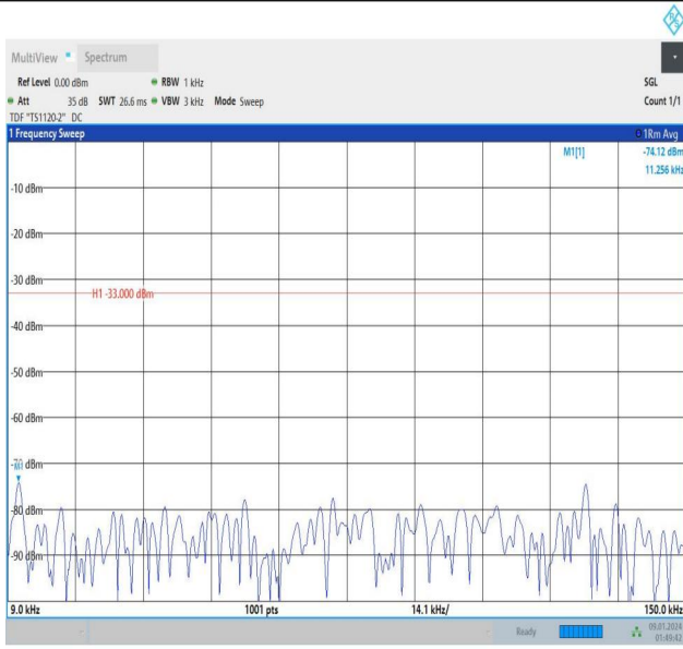
Band12_1.4MHz_QPSK_23173_1RB#0_0.009~0.15_0.009~0.15
