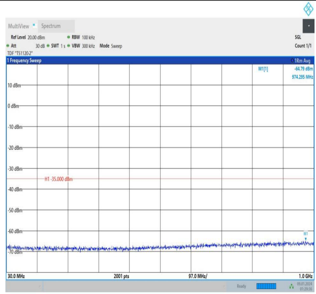
Band7_15MHz_QPSK_21375_75RB#0_30~1000_30~1000
