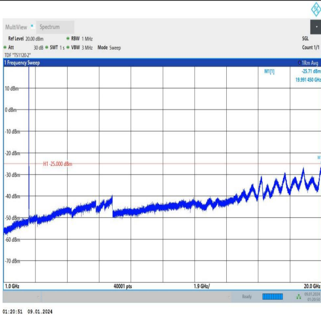
Band7_15MHz_QPSK_20825_1RB#0_1000~20000_1000~20000
