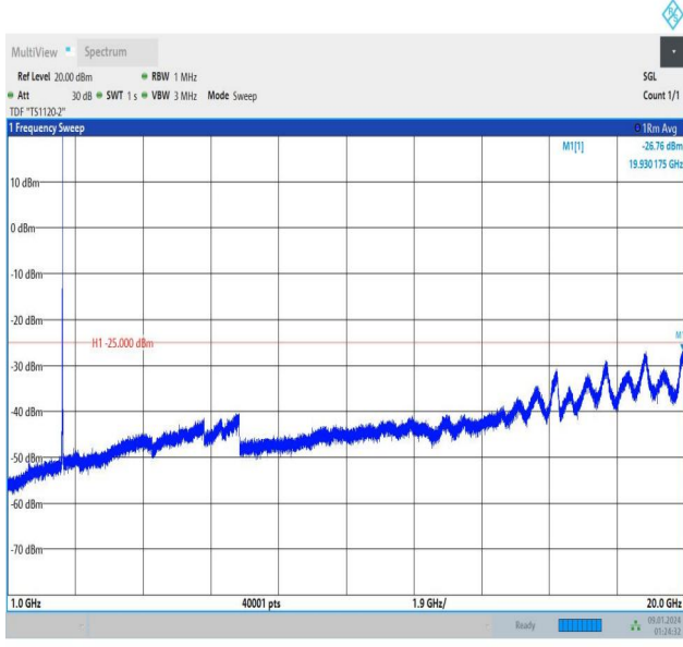
Band7_15MHz_QPSK_21100_1RB#74_1000~20000_1000~20000
