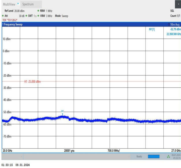
Band7_20MHz_QPSK_21100_1RB#0_20000~27000_20000~27000
