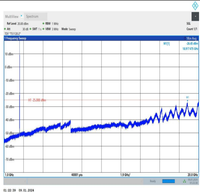
Band7_15MHz_16QAM_20825_1RB#74_1000~20000_1000~20000
