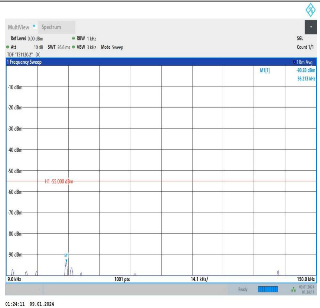
Band7_15MHz_QPSK_21100_1RB#74_0.009~0.15_0.009~0.15
