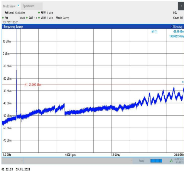
Band7_20MHz_16QAM_20850_1RB#99_1000~20000_1000~20000
