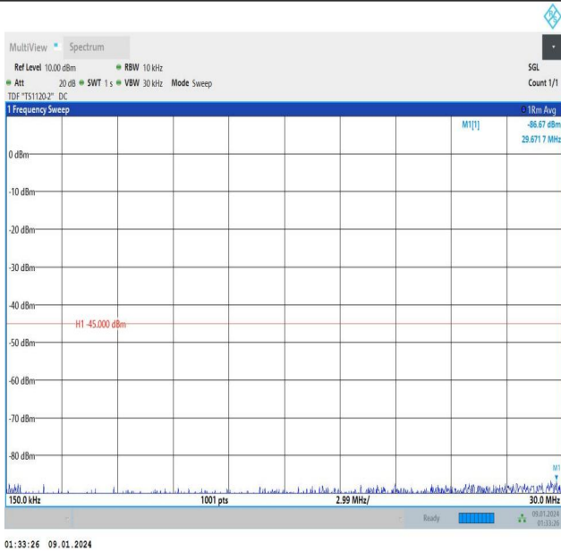
Band7_20MHz_16QAM_21100_1RB#0_0.15~30_0.15~30
