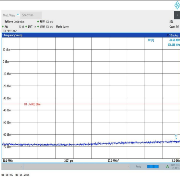
Band7_15MHz_QPSK_21100_75RB#0_30~1000_30~1000
