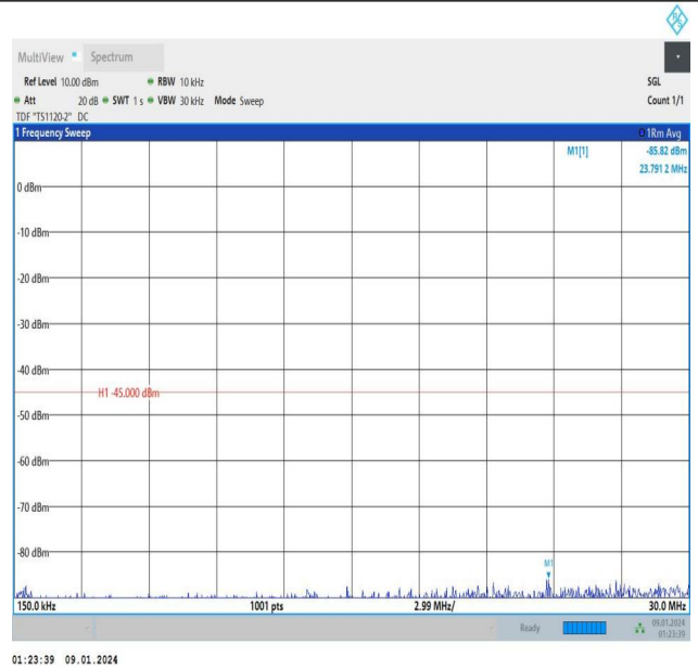
Band7_15MHz_16QAM_21100_1RB#0_0.15~30_0.15~30 15
