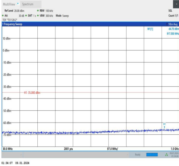
Band7_20MHz_QPSK_21100_1RB#99_30~1000_30~1000
