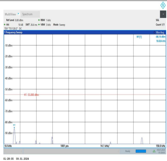
Band7_15MHz_QPSK_20825_75RB#0_0.009~0.15_0.009~0.
