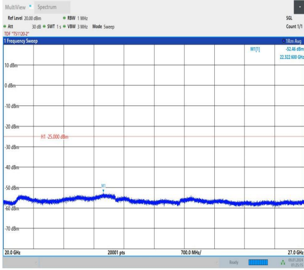
Band7_15MHz_16QAM_21100_1RB#74_20000~27000_2000 0~27000
