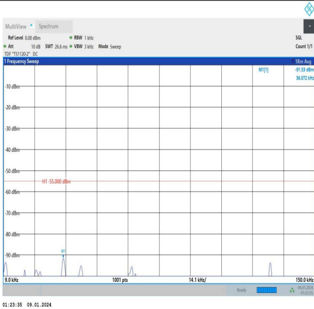
Band7_15MHz_16QAM_21100_1RB#0_0.009~0.15_0.009~0.15 15
