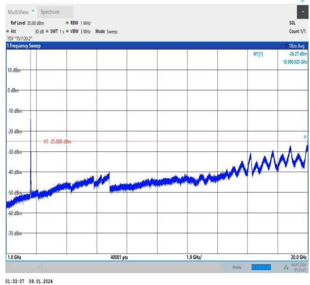
Band7_20MHz_QPSK_21100_1RB#0_1000~20000_1000~2000
