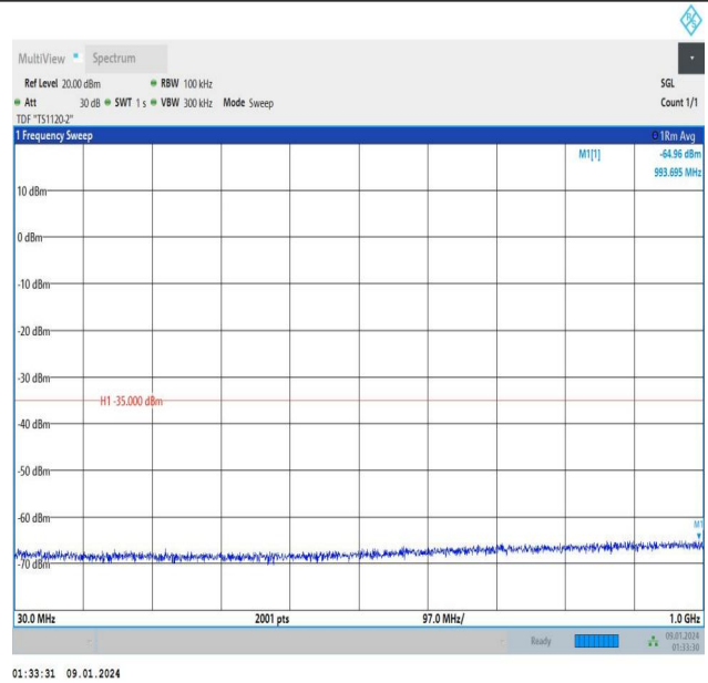
Band7_20MHz_16QAM_21100_1RB#0_30~1000_30~1000
