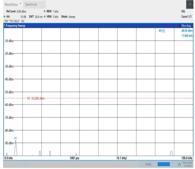
Band7_20MHz_16QAM_20850_1RB#0_0.009~0.15_0.009~0.15
