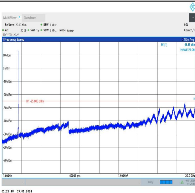
Band7_15MHz_QPSK_21375_75RB#0_1000~20000_1000~20000
