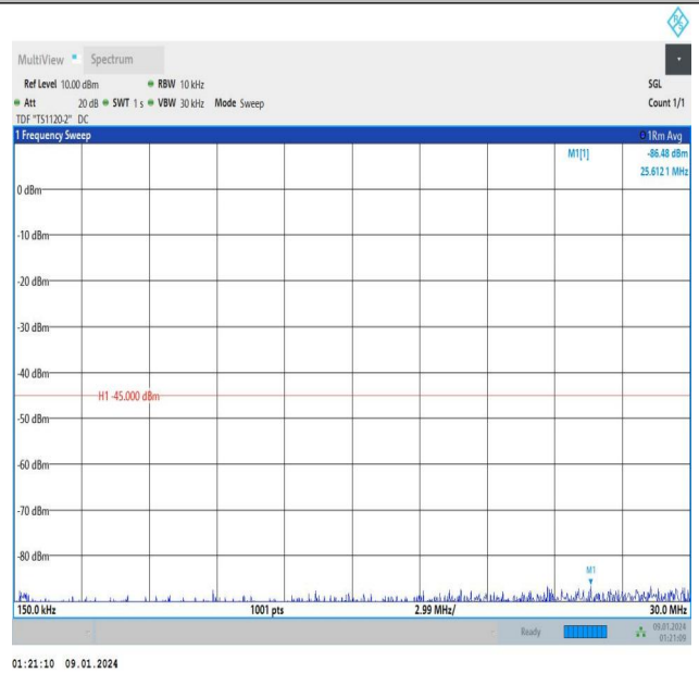
Band7_15MHz_16QAM_20825_1RB#0_0.15~30_0.15~30
