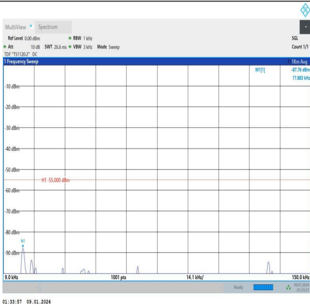
Band7_20MHz_QPSK_21100_1RB#99_0.009~0.15_0.009~0.1
