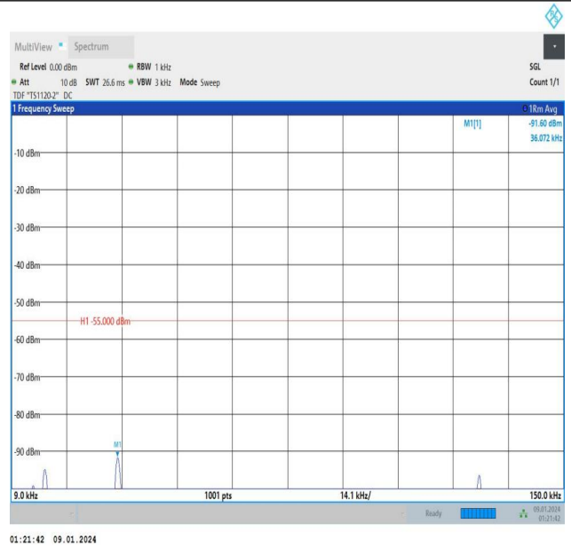
Band7_15MHz_QPSK_20825_1RB#74_0.009~0.15_0.009~0.15
