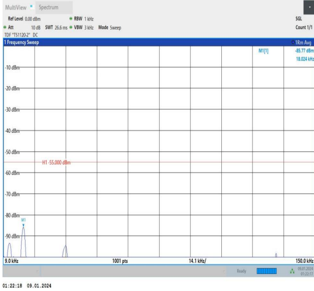
Band7_15MHz_16QAM_20825_1RB#74_0.009~0.15_0.009~0.15
