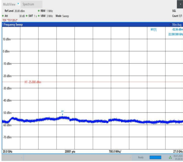
Band7_10MHz_QPSK_21400_50RB#0_20000~27000_20000~27000
