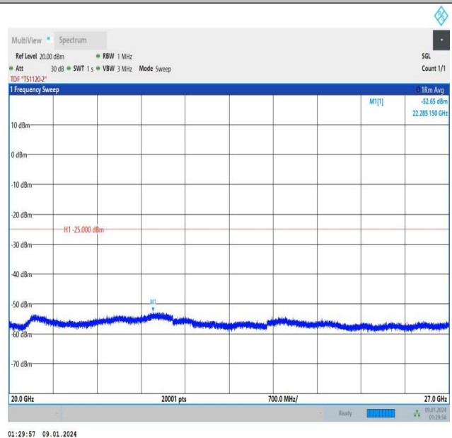
Band7_15MHz_QPSK_21375_75RB#0_20000~27000_20000~27000
