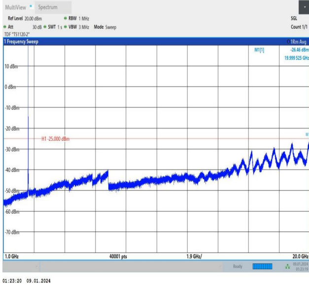
Band7_15MHz_QPSK_21100_1RB#0_1000~20000_1000~200 00
