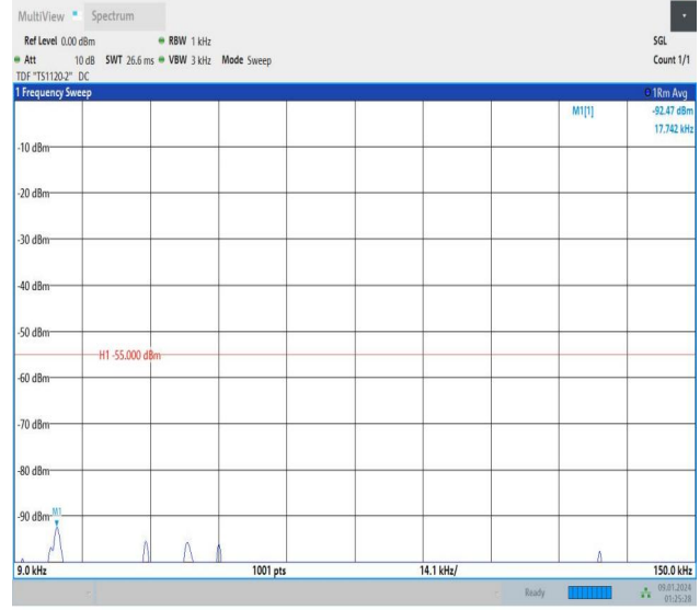
Band7_15MHz_QPSK_21375_1RB#0_0.009~0.15_0.009~0.1 5
