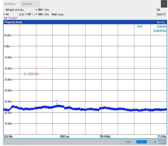
Band7_15MHz_QPSK_20825_75RB#0_20000~27000_20000~27000
