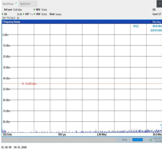
Band7_20MHz_16QAM_20850_1RB#99_0.15~30_0.15~30
