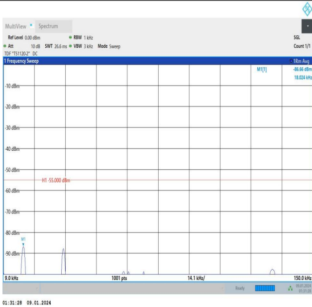
Band7_20MHz_QPSK_20850_1RB#99_0.009~0.15_0.009~0.15
