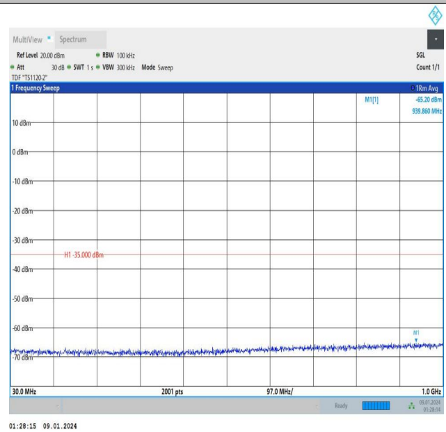
Band7_15MHz_QPSK_20825_75RB#0_30~1000_30~1000
