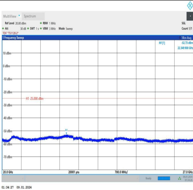
Band7_20MHz_QPSK_21100_1RB#99_20000~27000_20000~27000
