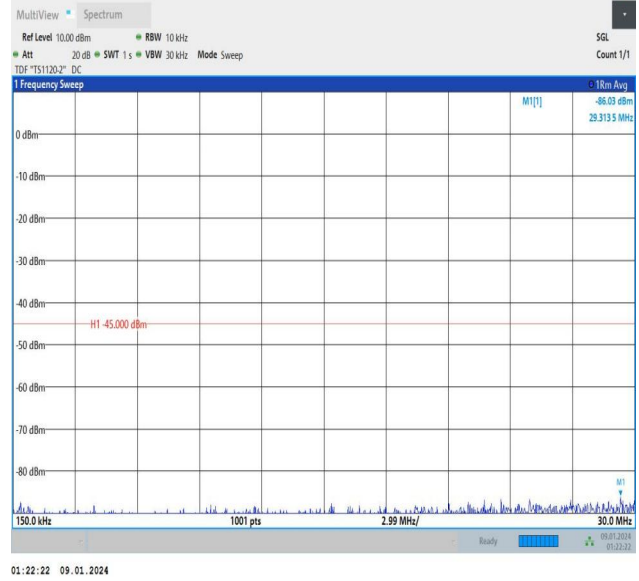
Band7_15MHz_16QAM_20825_1RB#74_0.15~30_0.15~30
