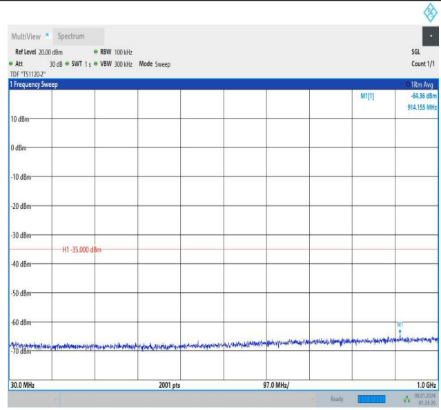
Band7_15MHz_QPSK_21100_1RB#74_30~1000_30~1000
