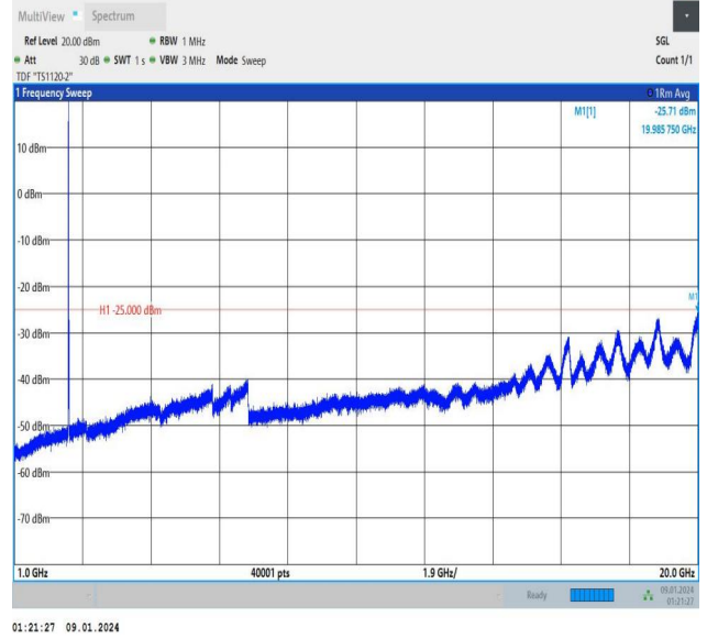
Band7_15MHz_16QAM_20825_1RB#0_1000~20000_1000~20000
