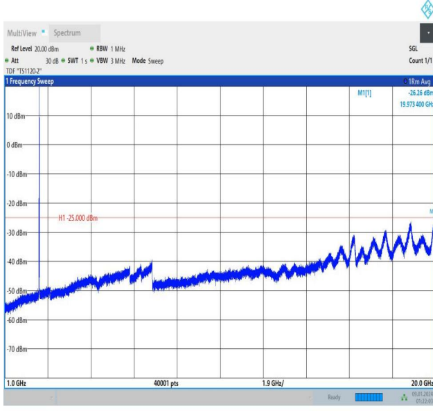
Band7_15MHz_QPSK_20825_1RB#74_1000~20000_1000~20000
