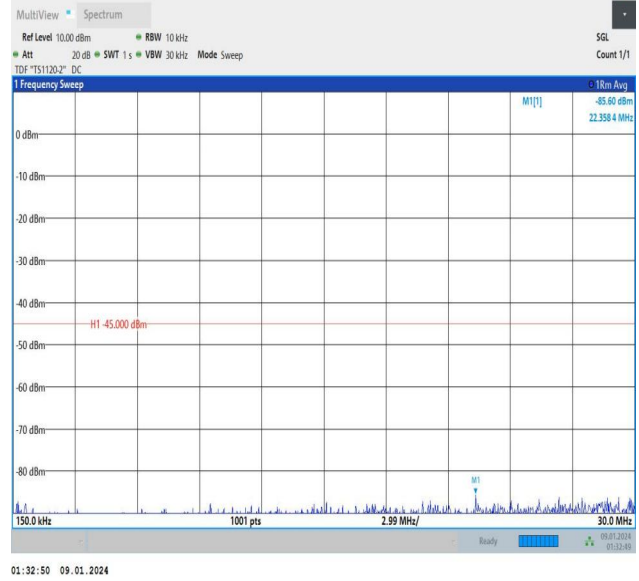
Band7_20MHz_QPSK_21100_1RB#0_0.15~30_0.15~30
