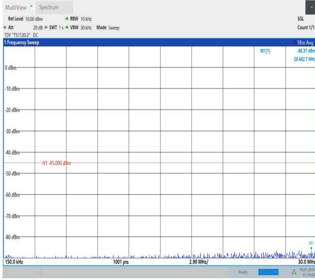
Band7_10MHz_QPSK_21100_50RB#0_0.15~30_0.15~30
