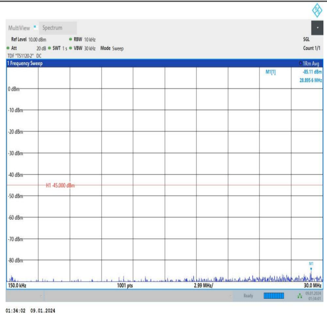
Band7_20MHz_QPSK_21100_1RB#99_0.15~30_0.15~30
