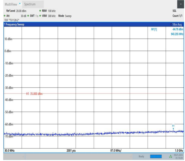
Band7_10MHz_QPSK_21100_50RB#0_30~1000_30~1000
