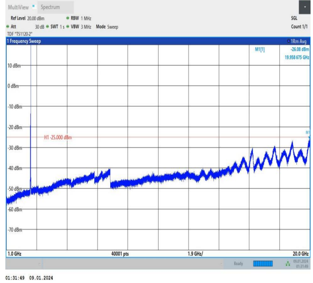
Band7_20MHz_QPSK_20850_1RB#99_1000~20000_1000~20000
