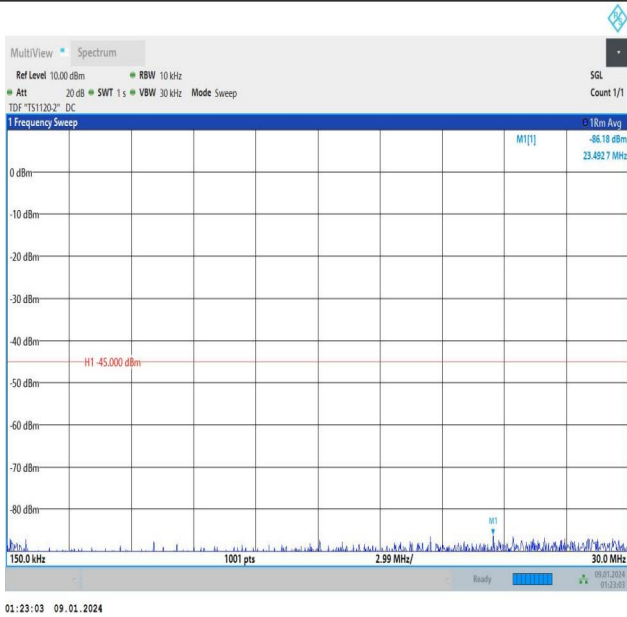
Band7_15MHz_QPSK_21100_1RB#0_0.15~30_0.15~30
