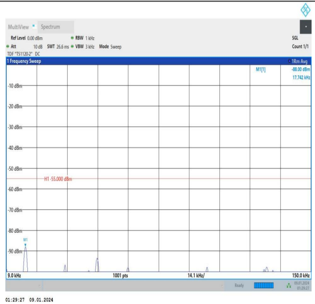
Band7_15MHz_QPSK_21375_75RB#0_0.009~0.15_0.009~0.15
