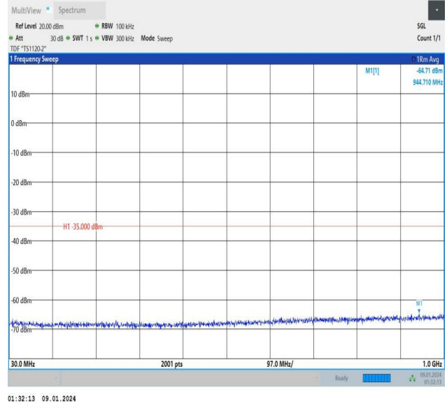
Band7_20MHz_16QAM_20850_1RB#99_30~1000_30~1000
