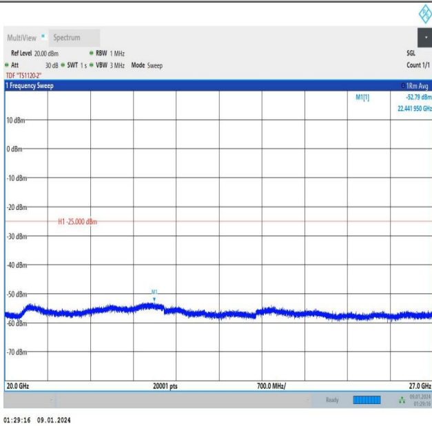
Band7_15MHz_QPSK_21100_75RB#0_20000~27000_20000~27000
