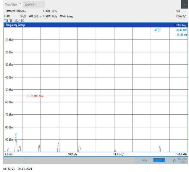
Band7_20MHz_16QAM_21100_1RB#0_0.009~0.15_0.009~0.15
