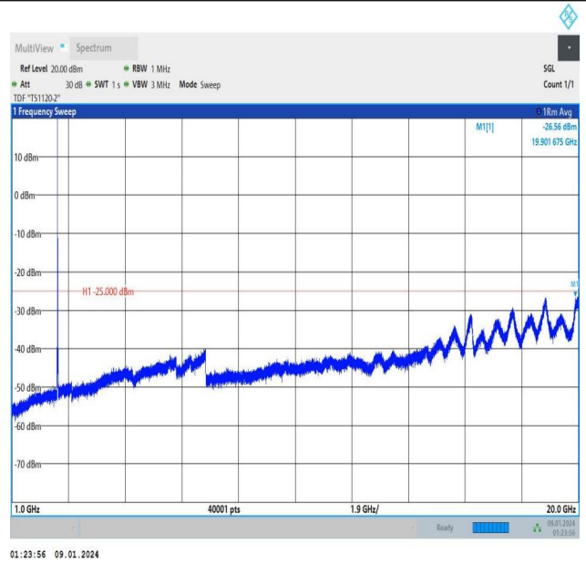
Band7_15MHz_16QAM_21100_1RB#0_1000~20000_1000~20000
