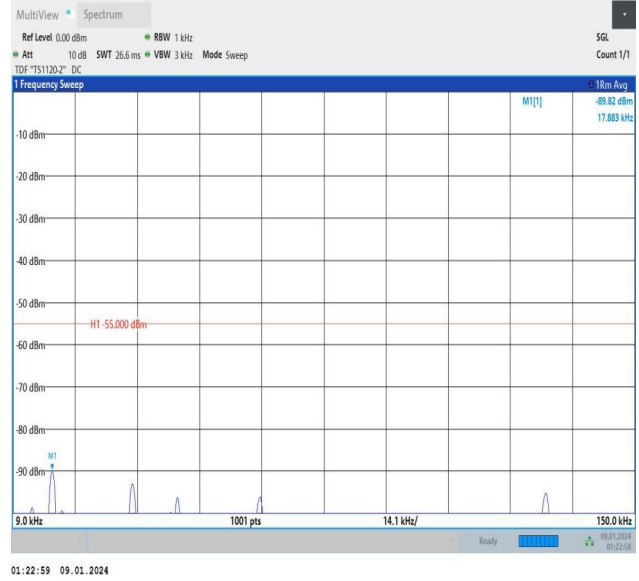
Band7_15MHz_QPSK_21100_1RB#0_0.009~0.15_0.009~0.15
