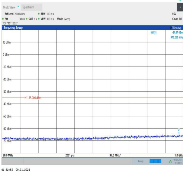
Band7_20MHz_QPSK_21100_1RB#0_30~1000_30~1000
