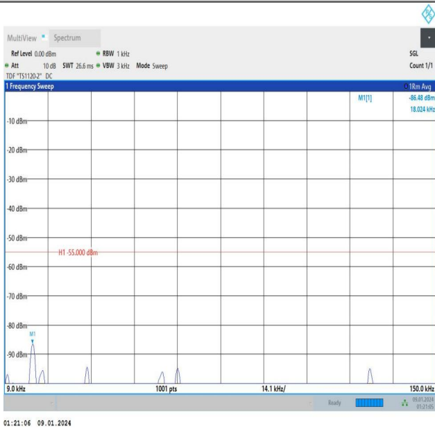
Band7_15MHz_16QAM_20825_1RB#0_0.009~0.15_0.009~0.15
