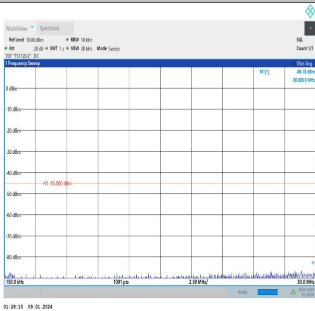
Band7_15MHz_QPSK_20825_75RB#0_0.15~30_0.15~30
