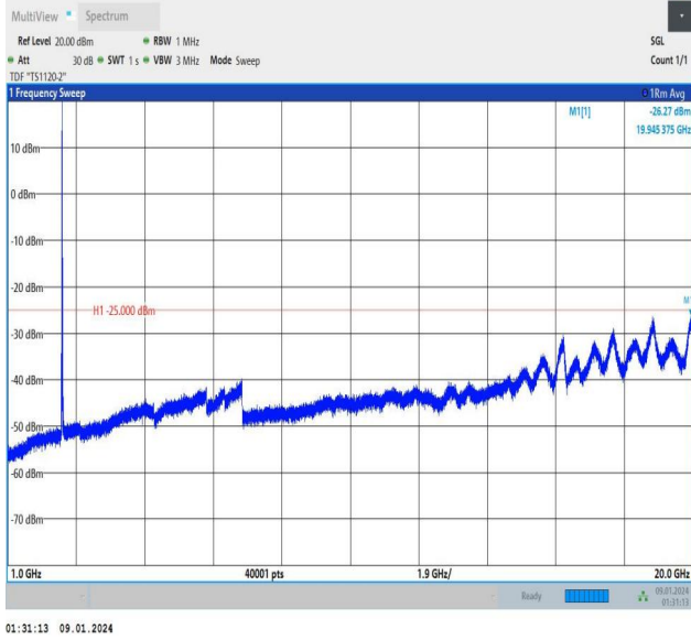
Band7_20MHz_16QAM_20850_1RB#0_1000~20000_1000~20000
