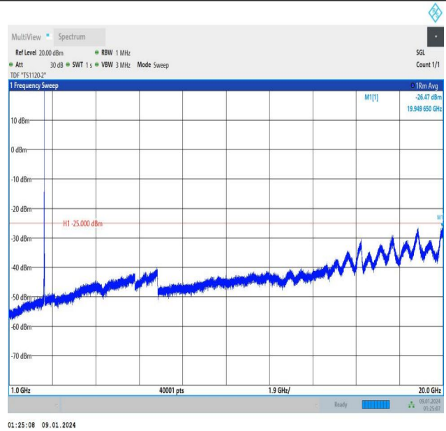
Band7_15MHz_16QAM_21100_1RB#74_1000~20000_1000~20000
