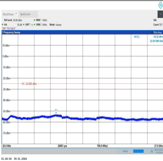
Band7_15MHz_16QAM_21100_1RB#0_20000~27000_20000~27000
