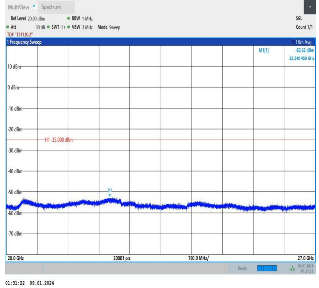
Band7_20MHz_16QAM_20850_1RB#0_20000~27000_20000~27000
