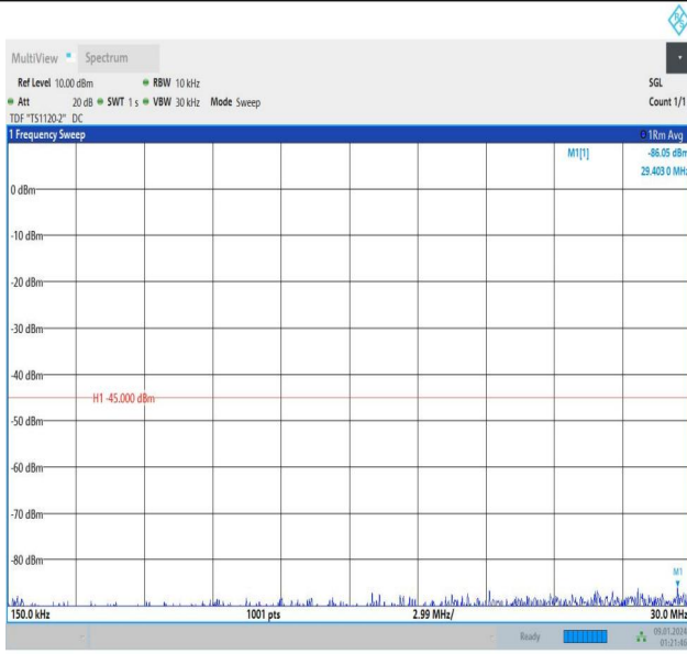
Band7_15MHz_QPSK_20825_1RB#74_0.15~30_0.15~30
