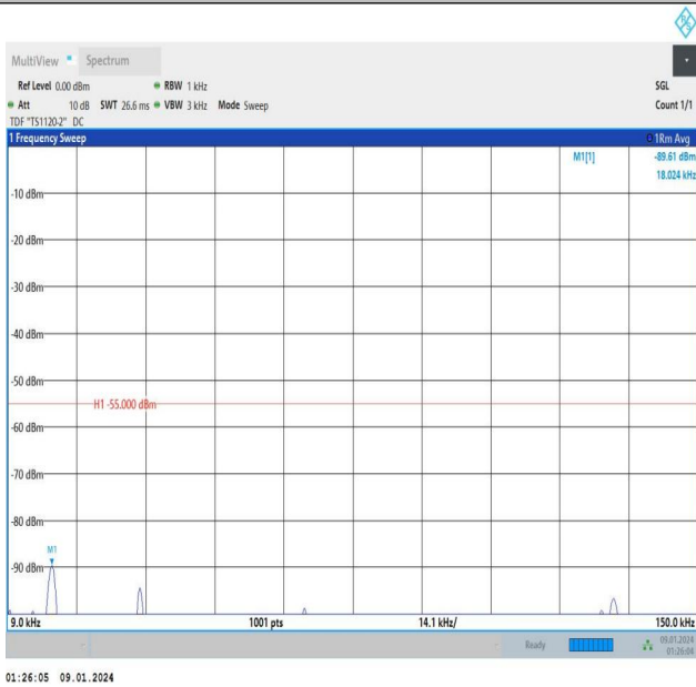
Band7_15MHz_16QAM_21375_1RB#0_0.009~0.15_0.009~0.15
