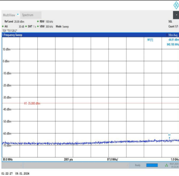
Band7_15MHz_16QAM_20825_1RB#74_30~1000_30~1000
