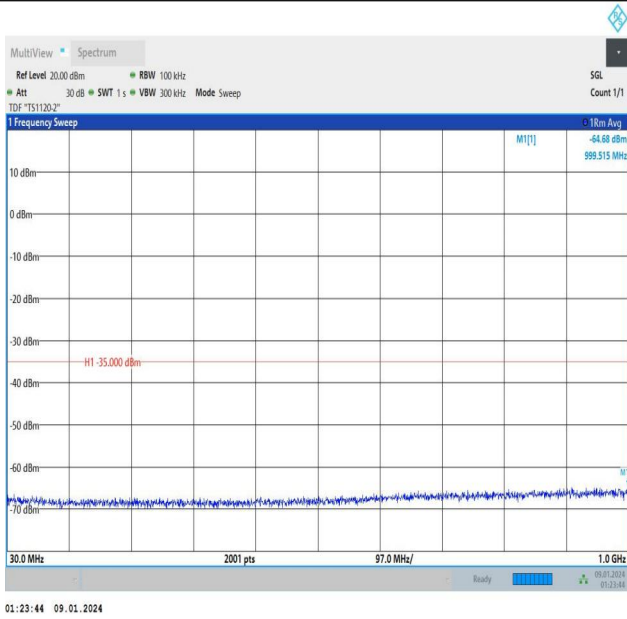
Band7_15MHz_16QAM_21100_1RB#0_30~1000_30~1000
