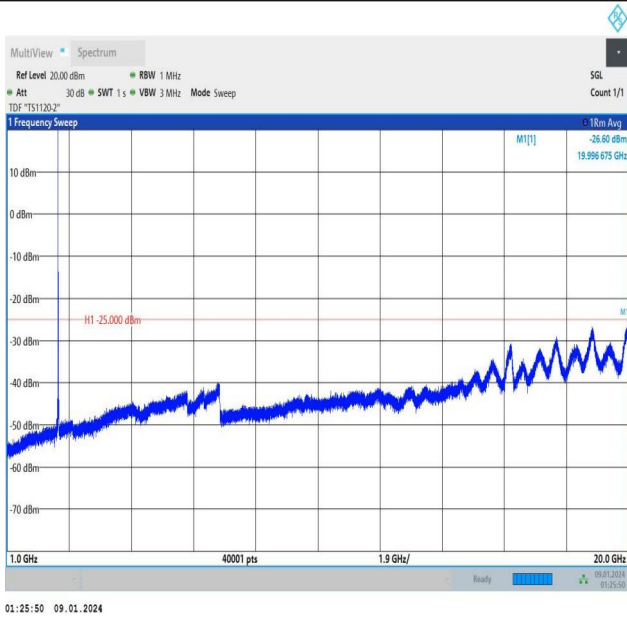
Band7_15MHz_QPSK_21375_1RB#0_1000~20000_1000~20000
