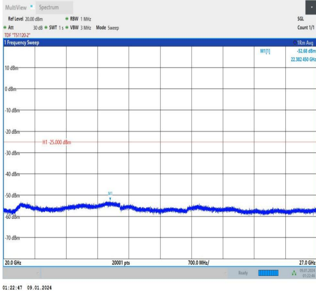
Band7_15MHz_16QAM_20825_1RB#74_20000~27000_2000 0~27000
