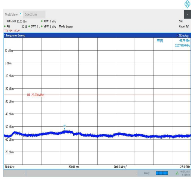
Band7_15MHz_QPSK_21100_1RB#74_20000~27000_20000~27000
