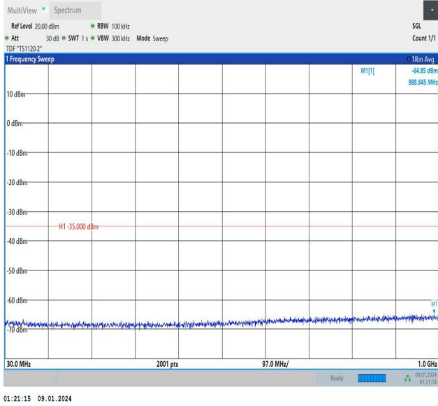
Band7_15MHz_16QAM_20825_1RB#0_30~1000_30~1000
