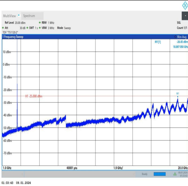
Band7_20MHz_16QAM_21100_1RB#0_1000~20000_1000~20000
