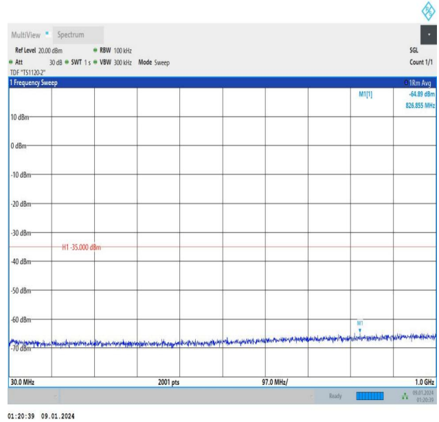
Band7_15MHz_QPSK_20825_1RB#0_30~1000_30~1000
