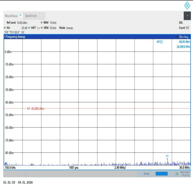
Band7_20MHz_QPSK_20850_1RB#99_0.15~30_0.15~30
