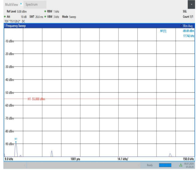
Band7_15MHz_QPSK_20825_1RB#0_0.009~0.15_0.009~0.1 5
