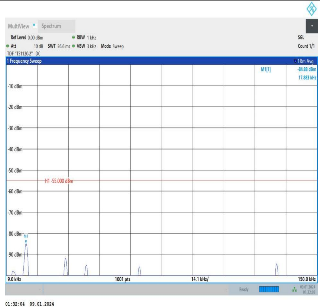
Band7_20MHz_16QAM_20850_1RB#99_0.009~0.15_0.009~0.15
