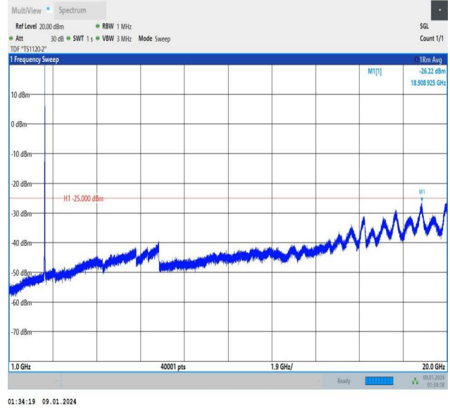
Band7_20MHz_QPSK_21100_1RB#99_1000~20000_1000~20000
