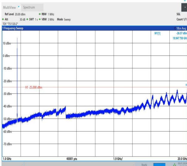
Band7_10MHz_QPSK_21100_50RB#0_1000~20000_1000~20000
