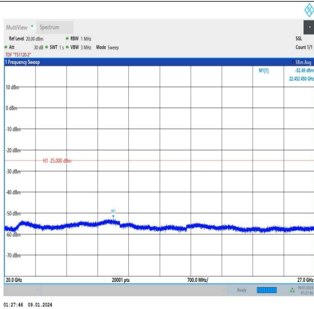
Band7_15MHz_16QAM_21375_1RB#74_20000~27000_2000 0~27000
