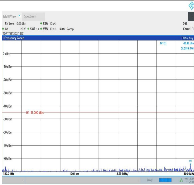
Band7_15MHz_QPSK_21375_75RB#0_0.15~30_0.15~30
