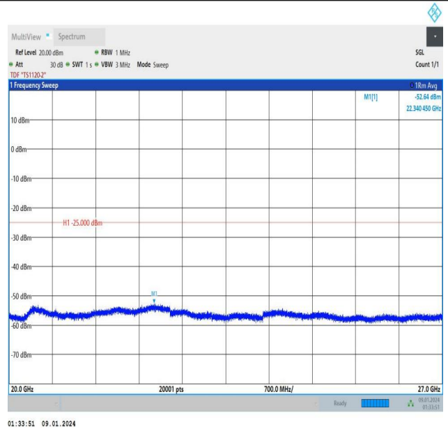
Band7_20MHz_16QAM_21100_1RB#0_20000~27000_20000
