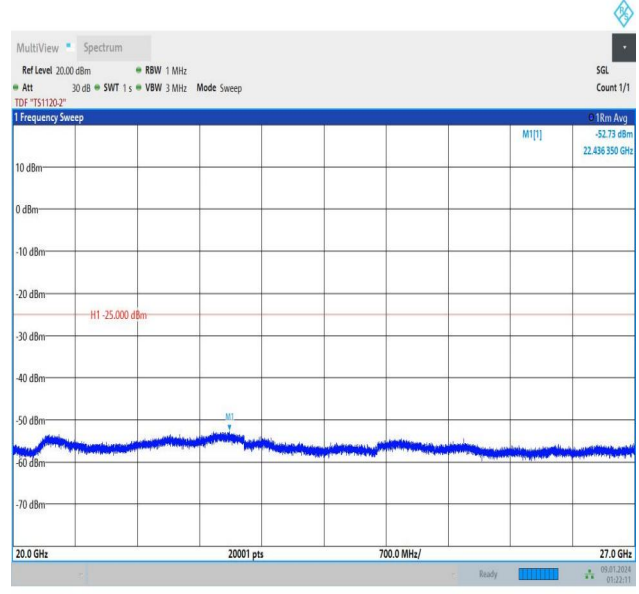
Band7_15MHz_QPSK_20825_1RB#74_20000~27000_20000~27000
