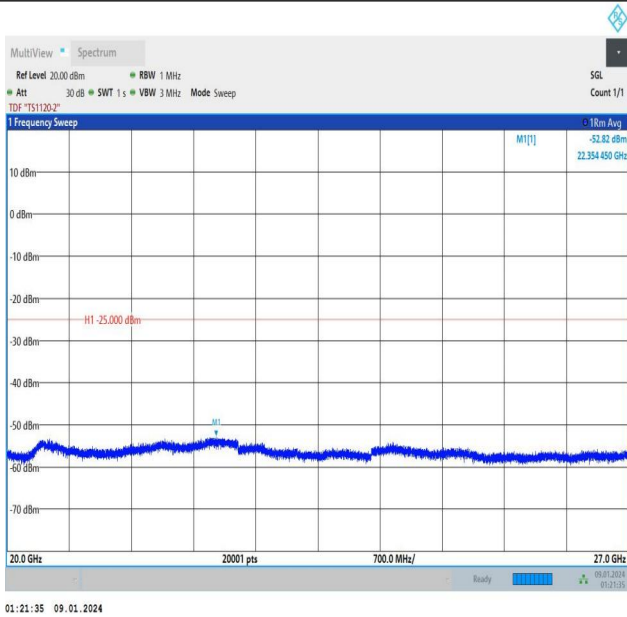
Band7_15MHz_16QAM_20825_1RB#0_20000~27000_20000~27000
