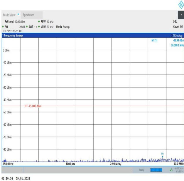
Band7_15MHz_QPSK_20825_1RB#0_0.15~30_0.15~30
