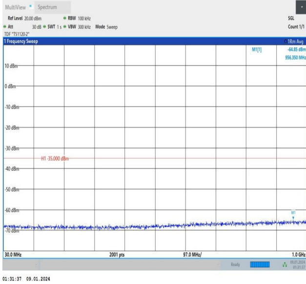
Band7_20MHz_QPSK_20850_1RB#99_30~1000_30~1000
