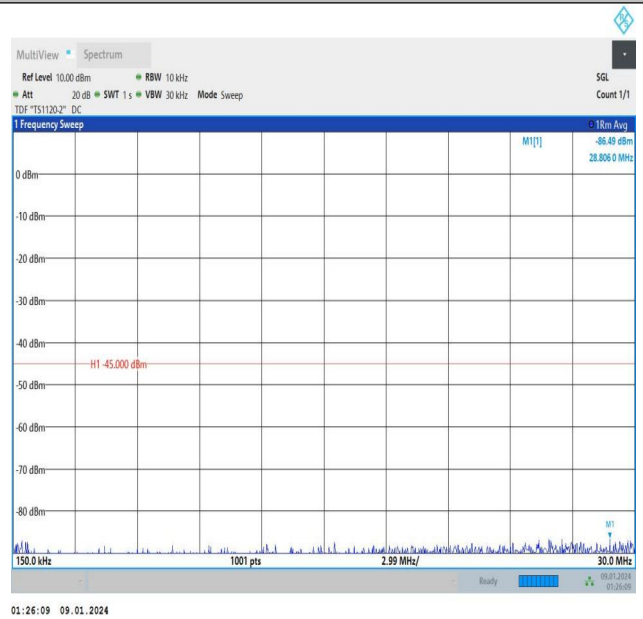
Band7_15MHz_16QAM_21375_1RB#0_0.15~30_0.15~30
