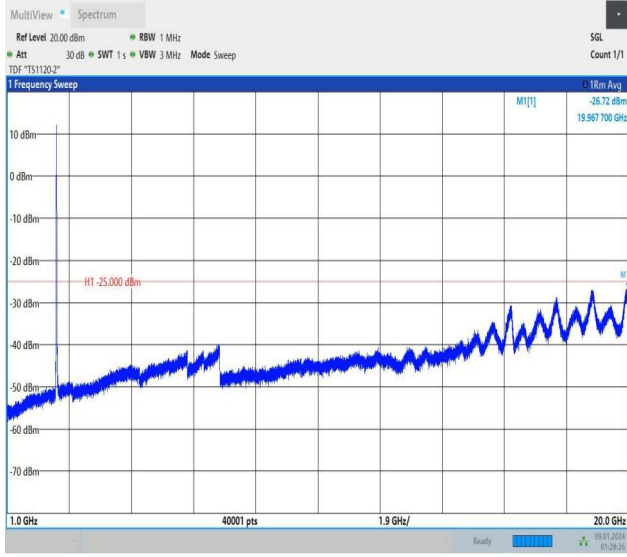
Band7_15MHz_QPSK_20825_75RB#0_1000~20000_1000~20000
