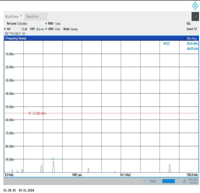
Band7_20MHz_16QAM_21100_1RB#99_0.009~0.15_0.009~0.15
