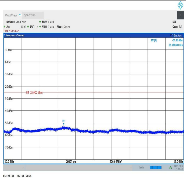
Band7_15MHz_QPSK_20825_1RB#0_20000~27000_20000~27000
