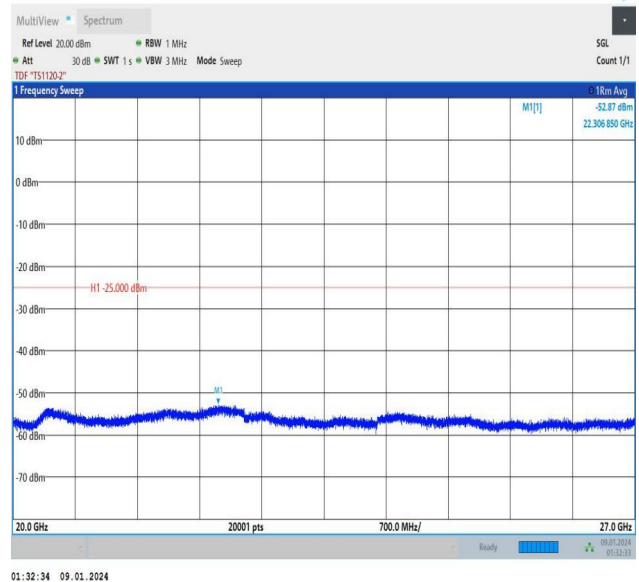
Band7_20MHz_16QAM_20850_1RB#99_20000~27000_20000~27000
