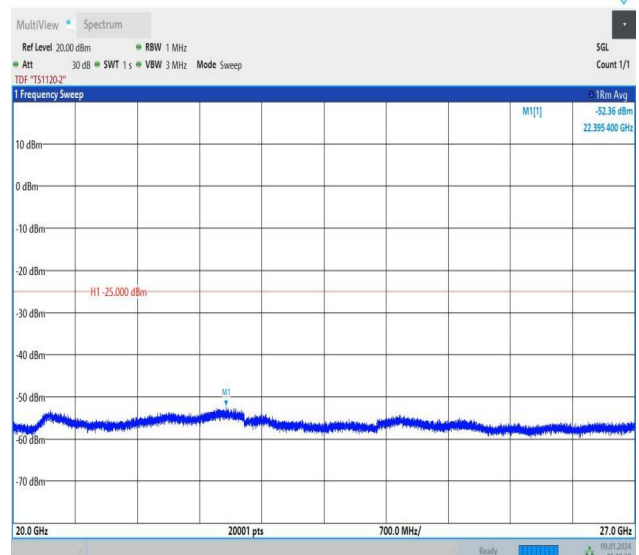
Band7_10MHz_QPSK_21100_50RB#0_20000~27000_20000~27000
