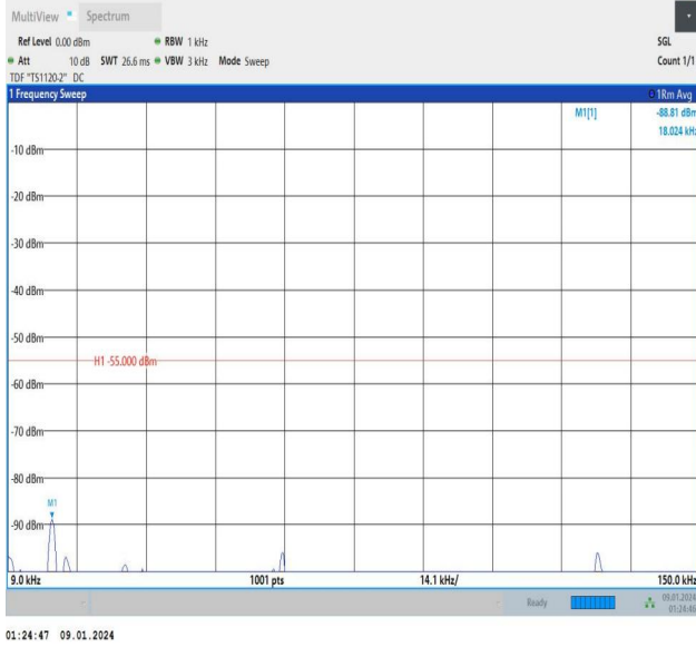
Band7_15MHz_16QAM_21100_1RB#74_0.009~0.15_0.009~0.15
