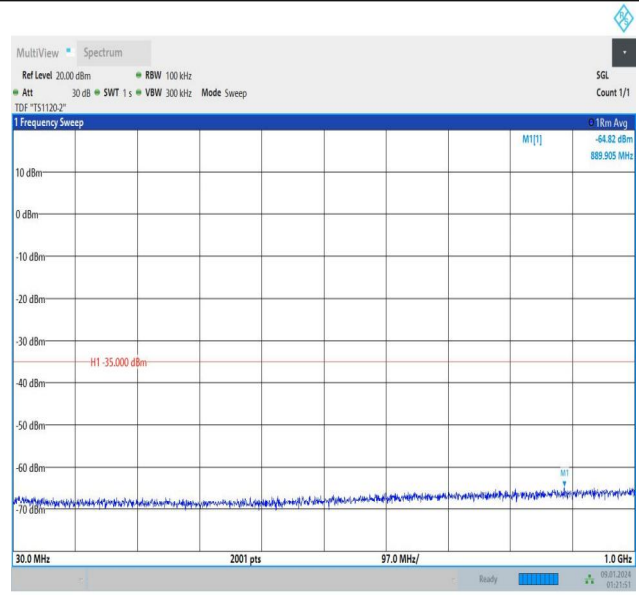
Band7_15MHz_QPSK_20825_1RB#74_30~1000_30~1000
