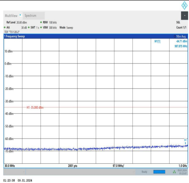
Band7_15MHz_QPSK_21100_1RB#0_30~1000_30~1000
