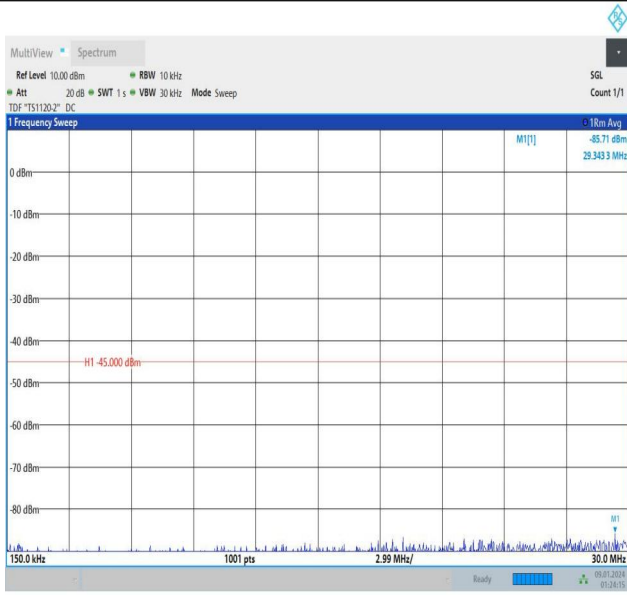
Band7_15MHz_QPSK_21100_1RB#74_0.15~30_0.15~30
