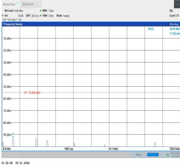
Band7_20MHz_QPSK_21100_1RB#0_0.009~0.15_0.009~0.15
