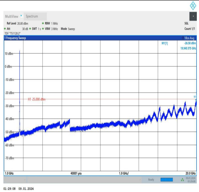
Band7_15MHz_QPSK_21100_75RB#0_1000~20000_1000~20000
