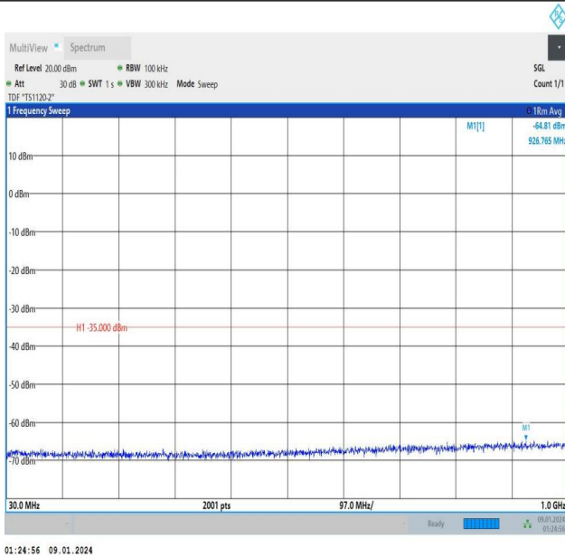
Band7_15MHz_16QAM_21100_1RB#74_30~1000_30~1000
