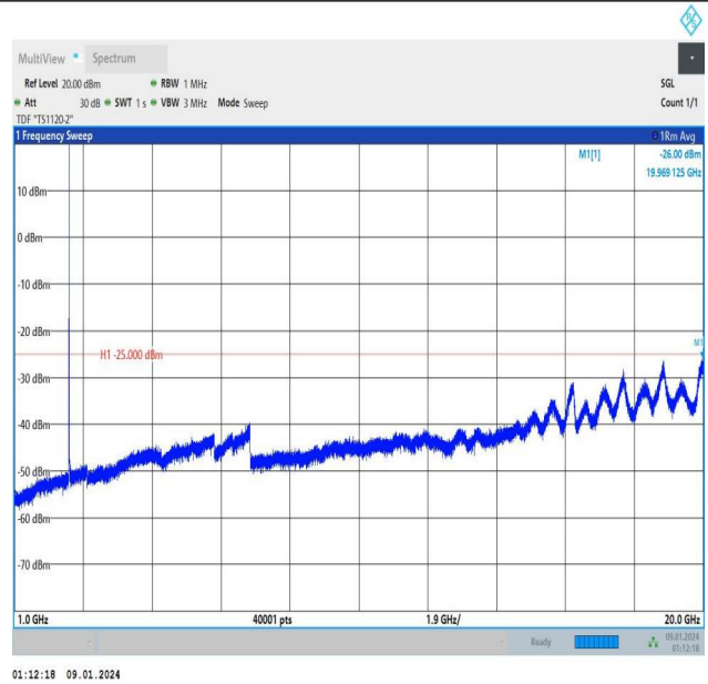
Band7_10MHz_QPSK_20800_1RB#49_1000~20000_1000~20000
