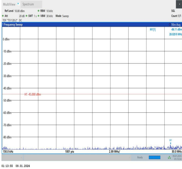
Band7_10MHz_16QAM_21100_1RB#0_0.15~30_0.15~30
