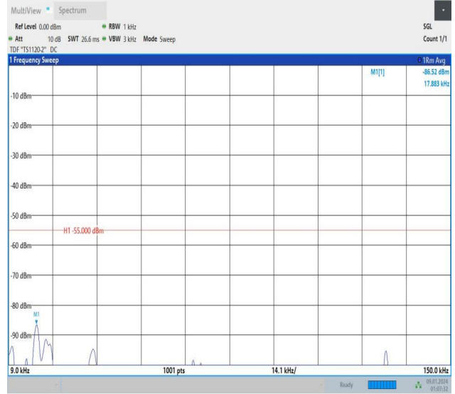
Band7_5MHz_16QAM_21425_1RB#0_0.009~0.15_0.009~0.15
