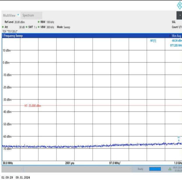
Band7_5MHz_QPSK_21425_25RB#0_30~1000_30~1000
