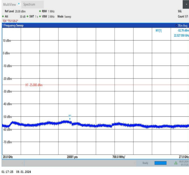
Band7_10MHz_QPSK_21400_1RB#49_20000~27000_20000~27000
