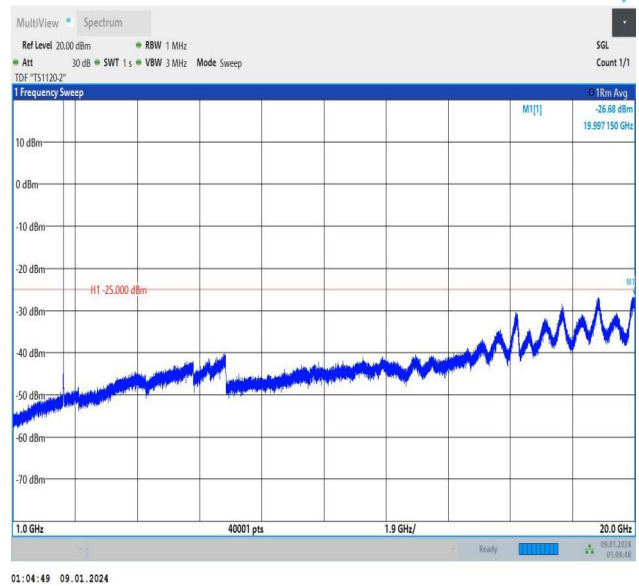
Band7_5MHz_QPSK_21100_1RB#24_1000~20000_1000~200
