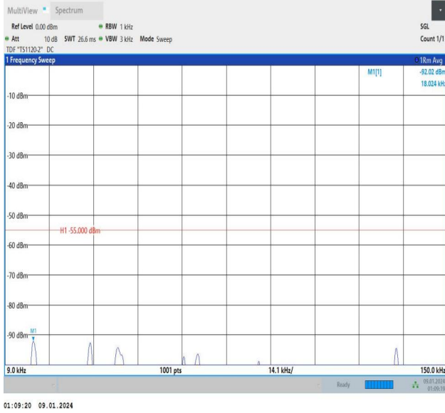
Band7_5MHz_QPSK_21425_25RB#0_0.009~0.15_0.009~0.1
