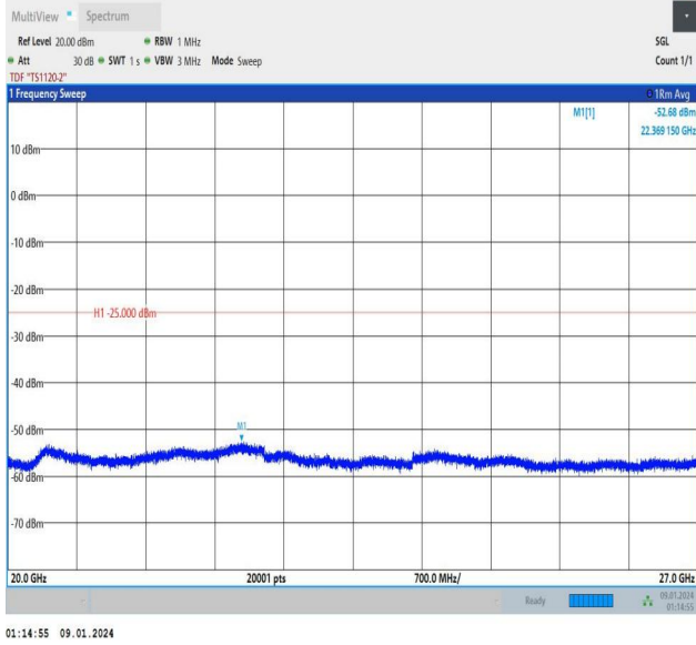
Band7_10MHz_QPSK_21100_1RB#49_20000~27000_20000~27000
