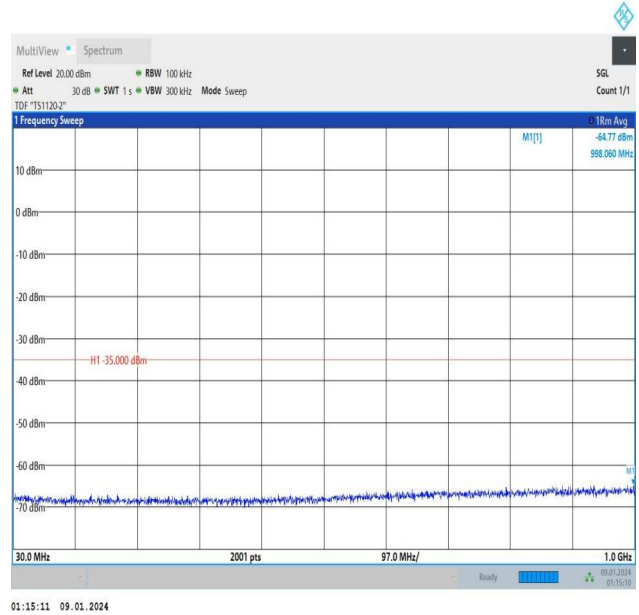
Band7_10MHz_16QAM_21100_1RB#49_30~1000_30~1000
