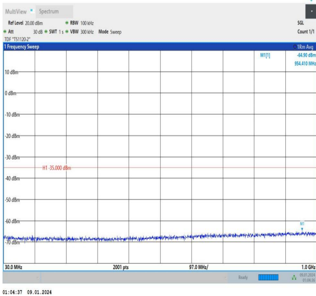
Band7_5MHz_QPSK_21100_1RB#24_30~1000_30~1000
