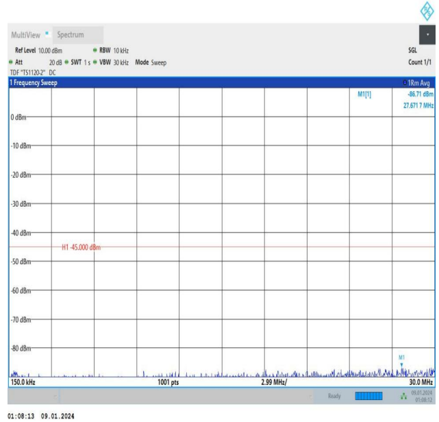
Band7_5MHz_QPSK_21425_1RB#24_0.15~30_0.15~30
