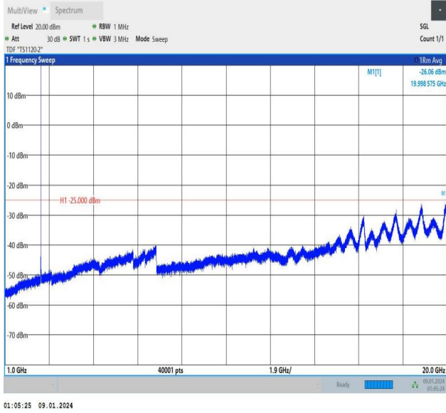
Band7_5MHz_16QAM_21100_1RB#24_1000~20000_1000~20000
