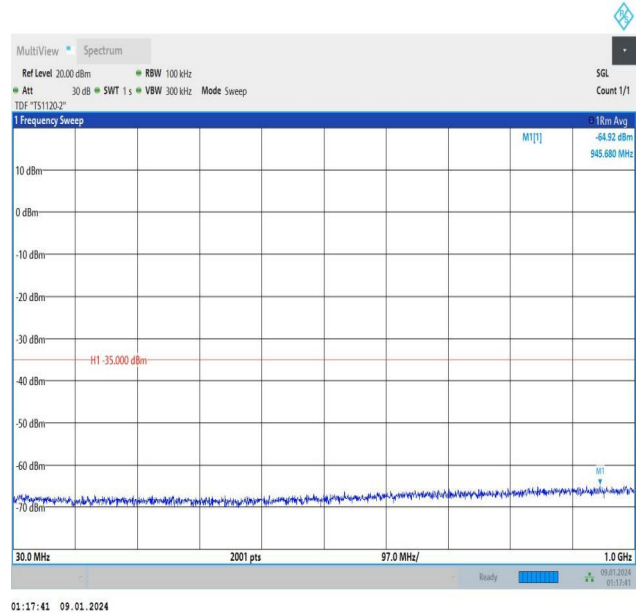
Band7_10MHz_16QAM_21400_1RB#49_30~1000_30~1000
