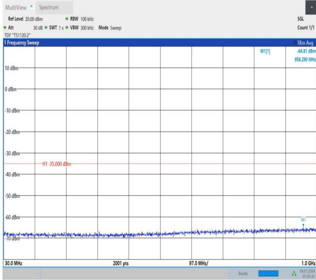
Band7_5MHz_QPSK_21100_25RB#0_30~1000_30~1000
