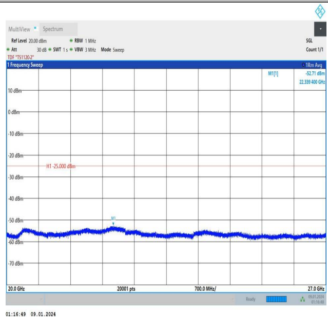
Band7_10MHz_16QAM_21400_1RB#0_20000~27000_20000~27000
