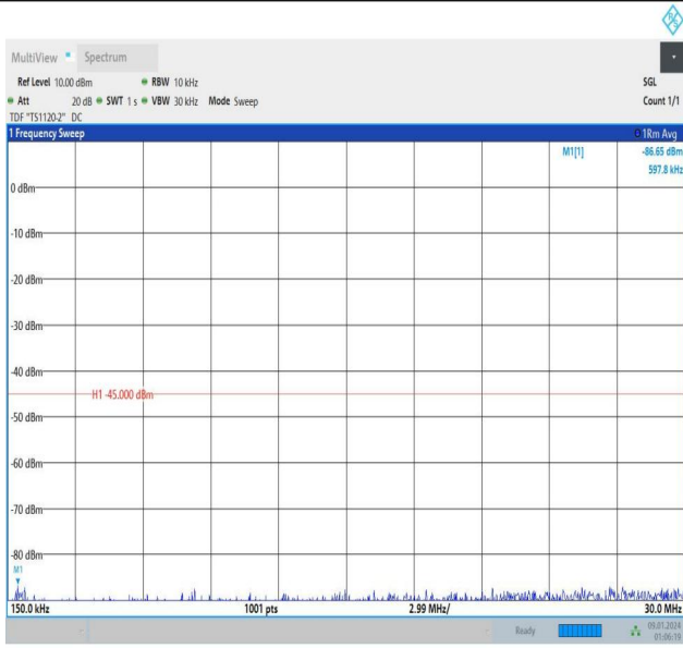
Band7_5MHz_16QAM_21100_25RB#0_0.15~30_0.15~30
