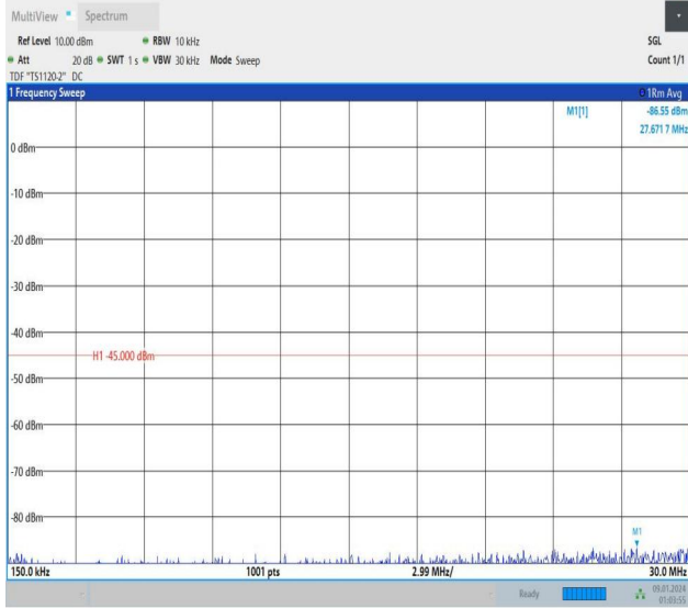
Band7_5MHz_16QAM_21100_1RB#0_0.15~30_0.15~30
