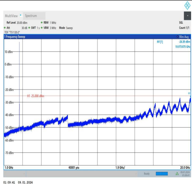
Band7_5MHz_QPSK_21425_25RB#0_1000~20000_1000~20000
