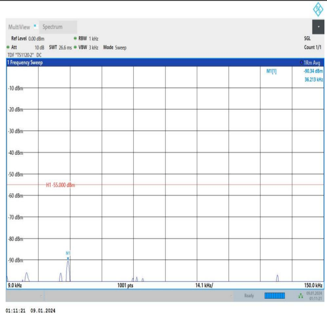
Band7_10MHz_16QAM_20800_1RB#0_0.009~0.15_0.009~0.15
