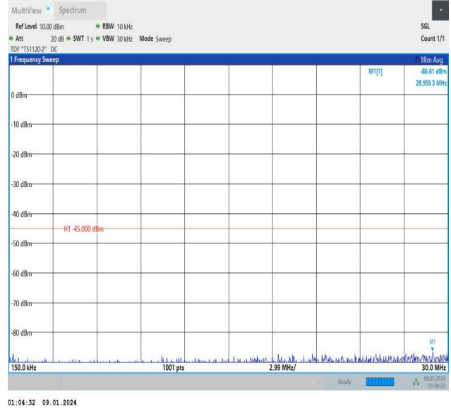
Band7_5MHz_QPSK_21100_1RB#24_0.15~30_0.15~30
