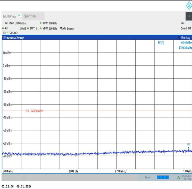
Band7_10MHz_QPSK_20800_1RB#49_30~1000_30~1000
