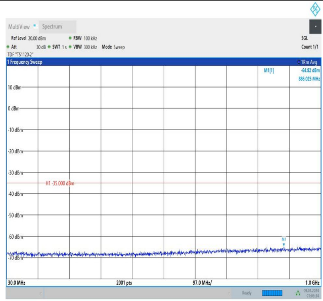
Band7_5MHz_16QAM_21100_25RB#0_30~1000_30~1000
