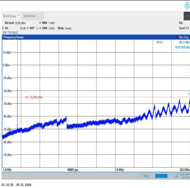
Band7_10MHz_16QAM_21100_1RB#49_1000~20000_1000~20000
