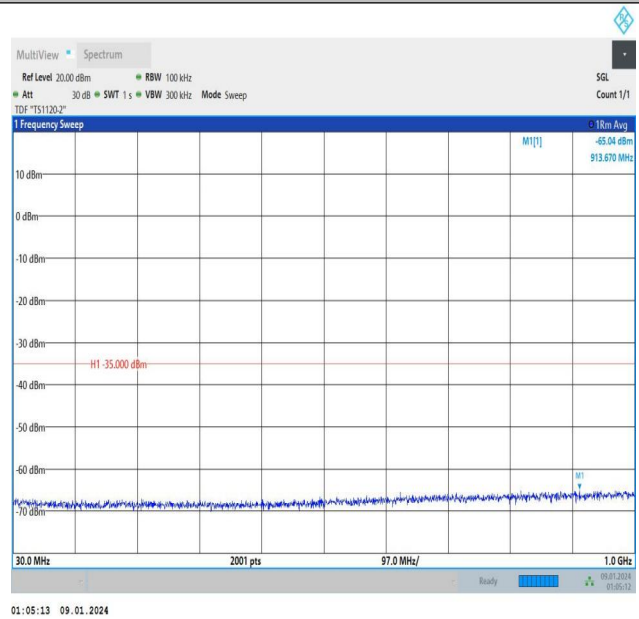
Band7_5MHz_16QAM_21100_1RB#24_30~1000_30~1000
