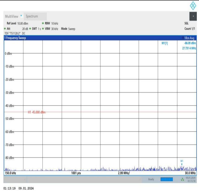
Band7_10MHz_QPSK_21100_1RB#0_0.15~30_0.15~30
