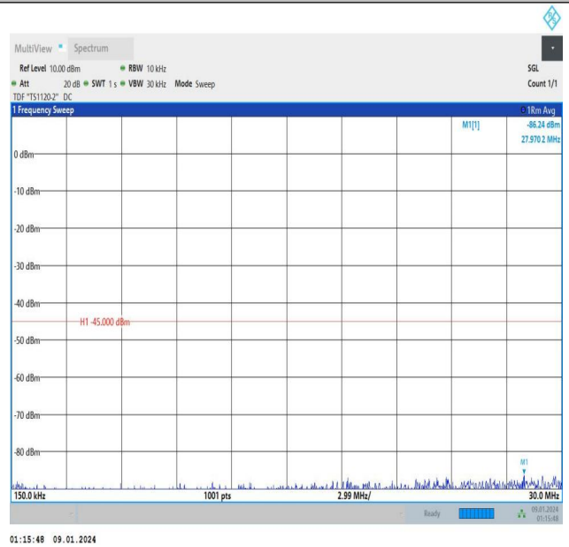
Band7_10MHz_QPSK_21400_1RB#0_0.15~30_0.15~30
