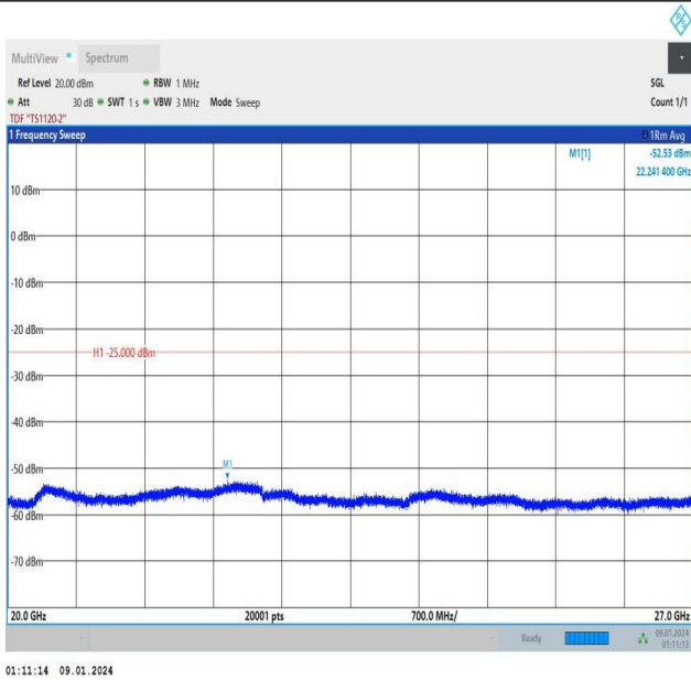
Band7_10MHz_QPSK_20800_1RB#0_20000~27000_20000~27000
