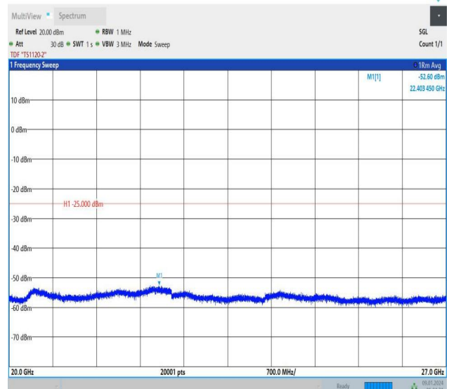
Band7_5MHz_16QAM_21100_1RB#0_20000~27000_20000~27000
