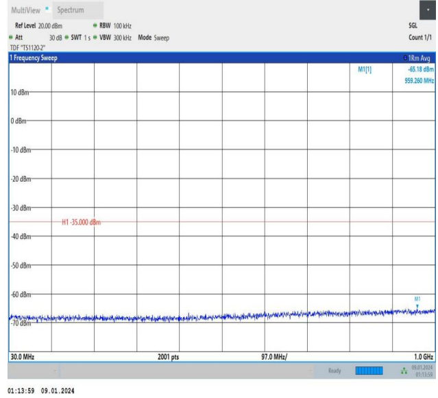
Band7_10MHz_16QAM_21100_1RB#0_30~1000_30~1000
