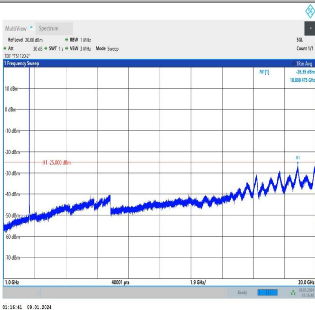
Band7_10MHz_16QAM_21400_1RB#0_1000~20000_1000~20000
