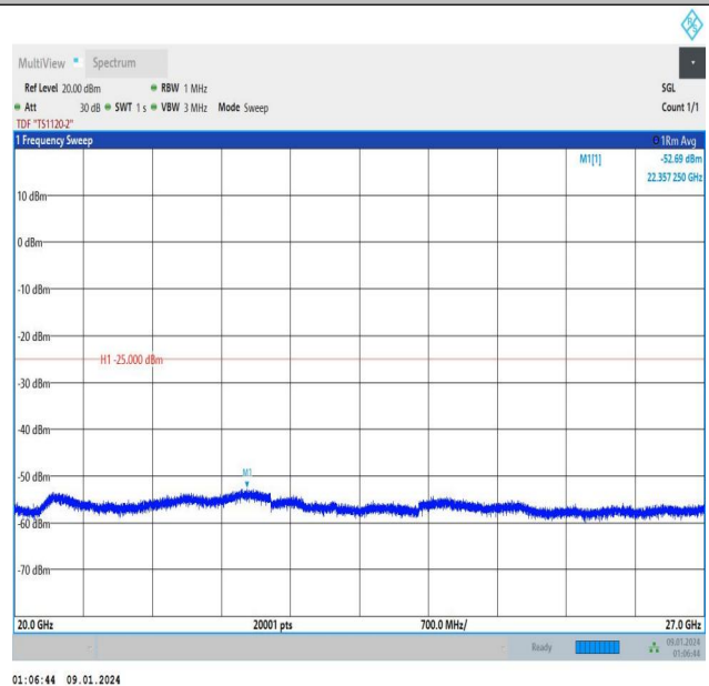
Band7_5MHz_16QAM_21100_25RB#0_20000~27000_20000~27000
