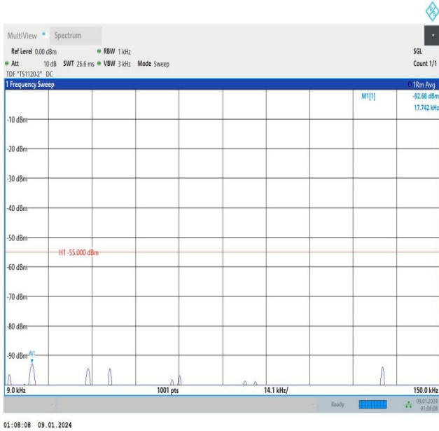
Band7_5MHz_QPSK_21425_1RB#24_0.009~0.15_0.009~0.15
