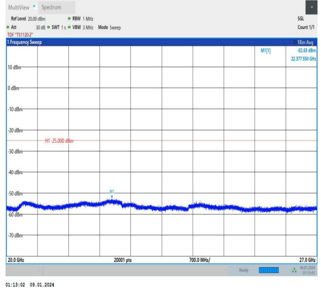
Band7_10MHz_16QAM_20800_1RB#49_20000~27000_2000~27000
