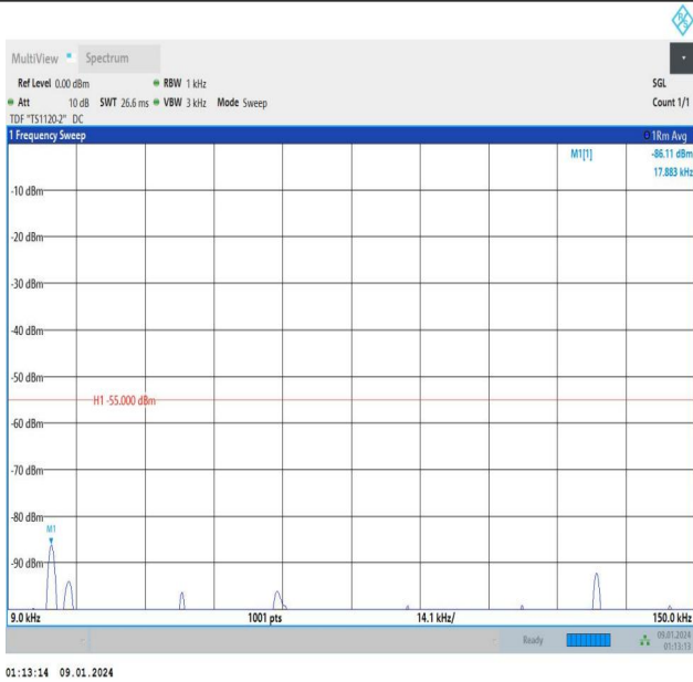
Band7_10MHz_QPSK_21100_1RB#0_0.009~0.15_0.009~0.15
