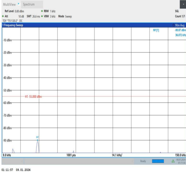
Band7_10MHz_QPSK_20800_1RB#49_0.009~0.15_0.009~0.15
