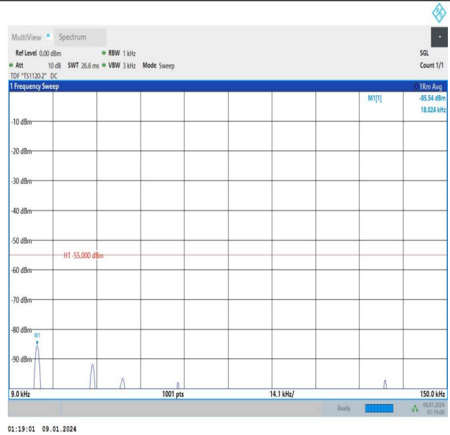
Band7_10MHz_QPSK_21100_50RB#0_0.009~0.15_0.009~0.1
