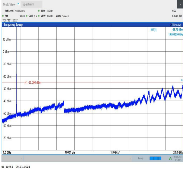
Band7_10MHz_16QAM_20800_1RB#49_1000~20000_1000~20000
