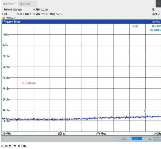
Band7_10MHz_QPSK_20800_50RB#0_30~1000_30~1000
