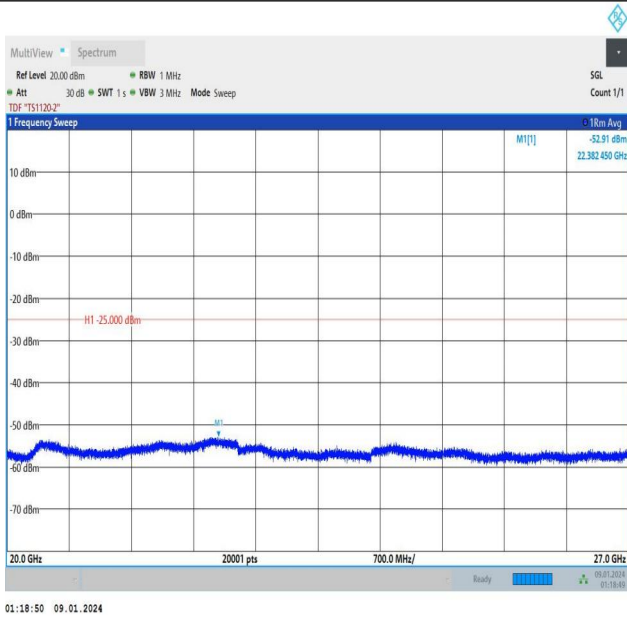
Band7_10MHz_QPSK_20800_50RB#0_20000~27000_20000~27000
