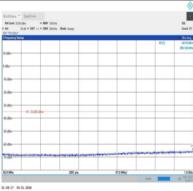
Band7_5MHz_QPSK_21425_1RB#24_30~1000_30~1000
