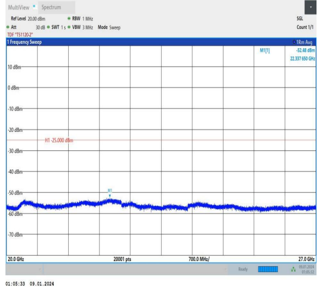
Band7_5MHz_16QAM_21100_1RB#24_20000~27000_20000~27000
