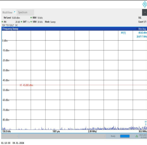
Band7_5MHz_16QAM_21425_25RB#0_0.15~30_0.15~30
