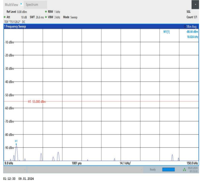
Band7_10MHz_16QAM_20800_1RB#49_0.009~0.15_0.009~0.15
