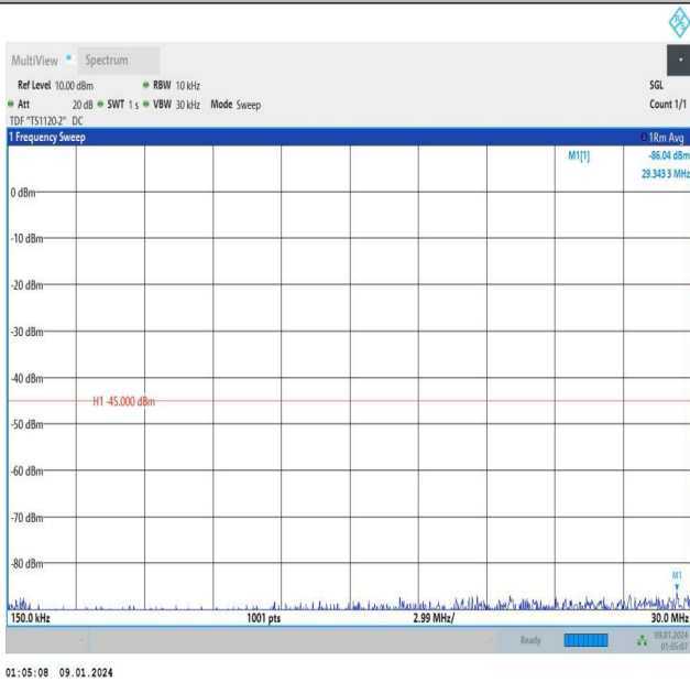
Band7_5MHz_16QAM_21100_1RB#24_0.15~30_0.15~30
