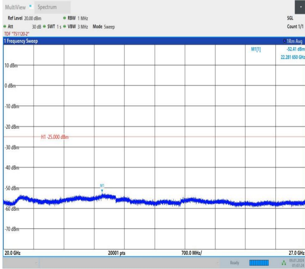
Band7_5MHz_QPSK_21425_1RB#0_20000~27000_20000~27000
