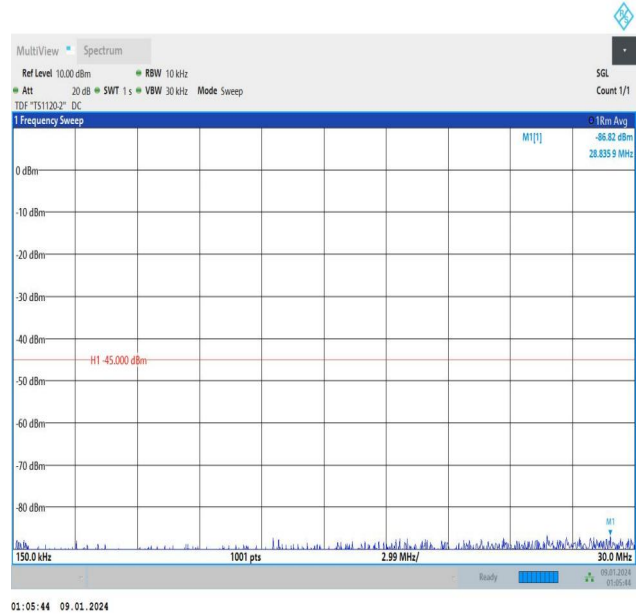
Band7_5MHz_QPSK_21100_25RB#0_0.15~30_0.15~30
