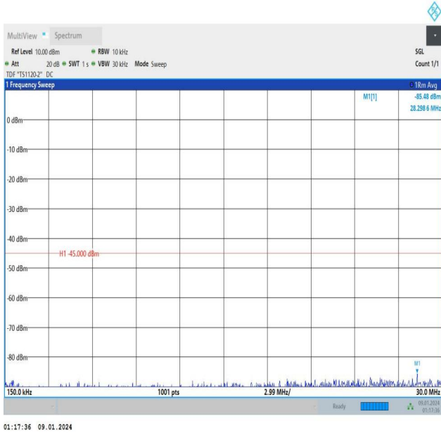
Band7_10MHz_16QAM_21400_1RB#49_0.15~30_0.15~30
