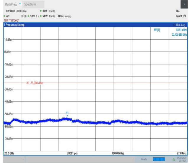
Band7_5MHz_16QAM_21425_25RB#0_20000~27000_20000~27000
