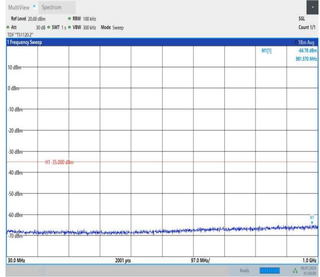
Band7_5MHz_16QAM_21100_1RB#0_30~1000_30~1000
