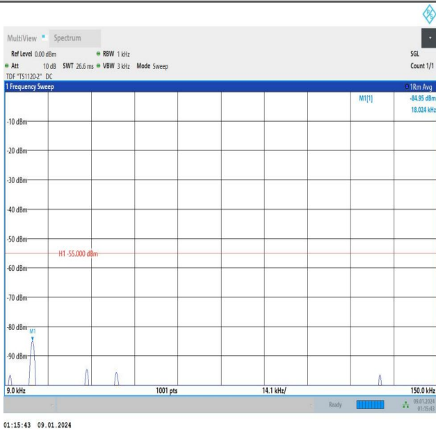
Band7_10MHz_QPSK_21400_1RB#0_0.009~0.15_0.009~0.1
