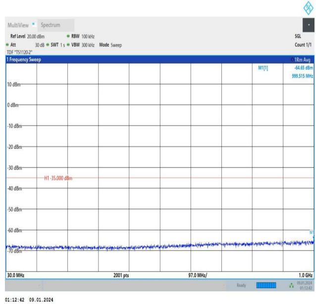
Band7_10MHz_16QAM_20800_1RB#49_30~1000_30~1000
