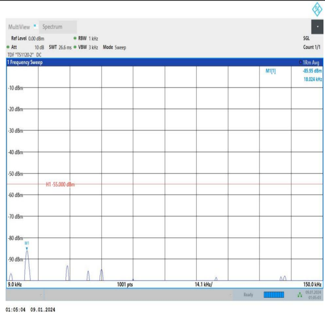
Band7_5MHz_16QAM_21100_1RB#24_0.009~0.15_0.009~0.15
