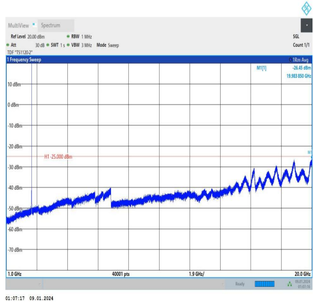
Band7_5MHz_QPSK_21425_1RB#0_1000~20000_1000~2000
