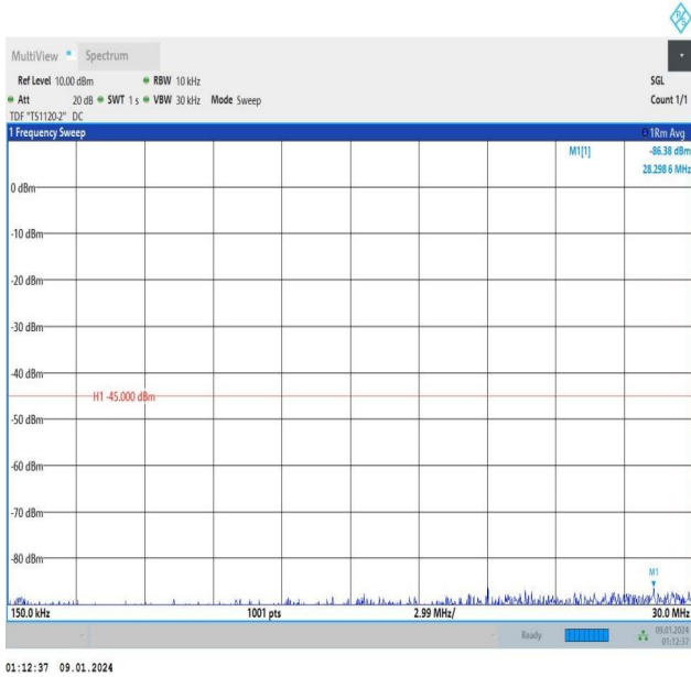
Band7_10MHz_16QAM_20800_1RB#49_0.15~30_0.15~30
