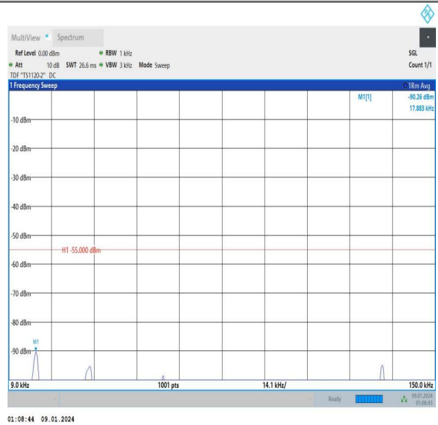
Band7_5MHz_16QAM_21425_1RB#24_0.009~0.15_0.009~0.15
