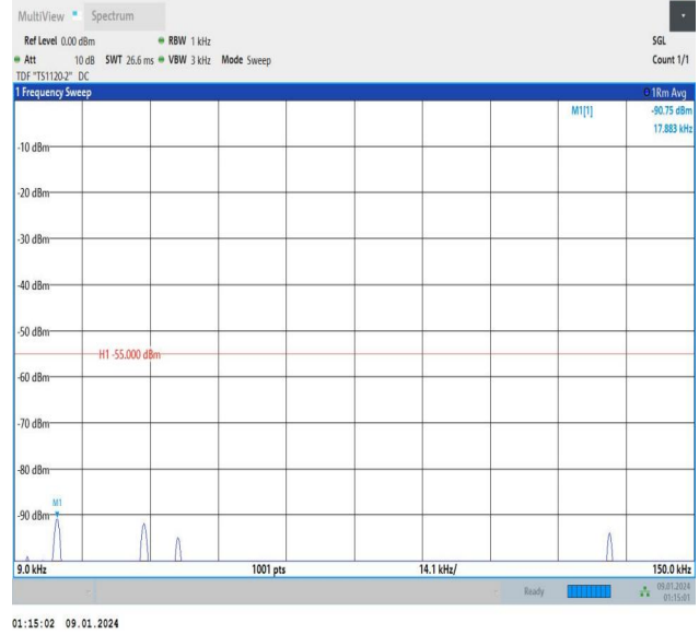
Band7_10MHz_16QAM_21100_1RB#49_0.009~0.15_0.009~0.15
