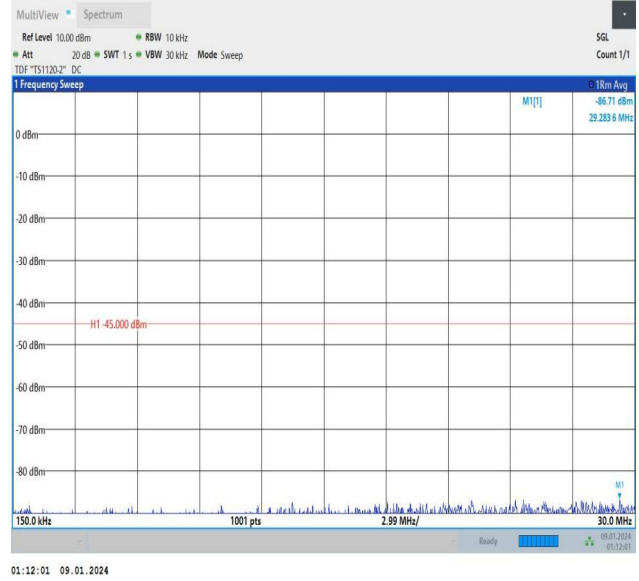
Band7_10MHz_QPSK_20800_1RB#49_0.15~30_0.15~30
