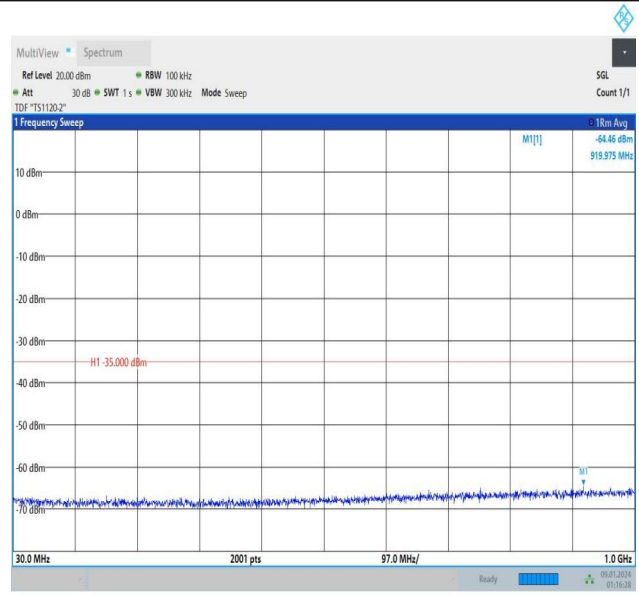
Band7_10MHz_16QAM_21400_1RB#0_30~1000_30~1000
