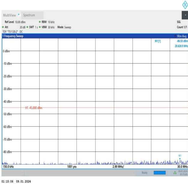
Band7_10MHz_16QAM_21100_1RB#49_0.15~30_0.15~30
