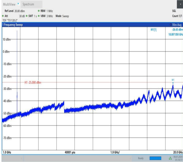
Band7_5MHz_16QAM_21425_25RB#0_1000~20000_1000~20000
