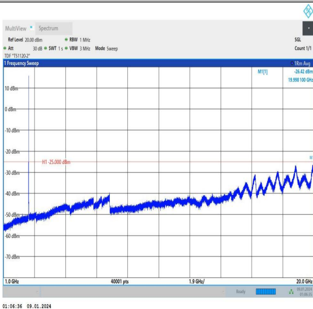
Band7_5MHz_16QAM_21100_25RB#0_1000~20000_1000~20000
