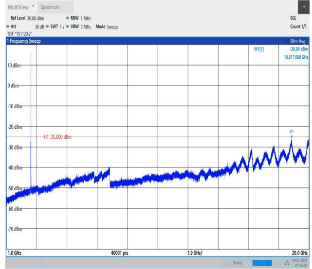
Band7_5MHz_QPSK_21100_25RB#0_1000~20000_1000~20000
