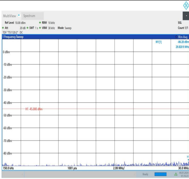
Band7_10MHz_16QAM_21400_1RB#0_0.15~30_0.15~30
