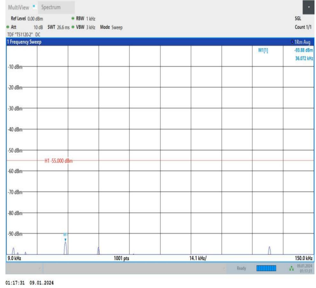
Band7_10MHz_16QAM_21400_1RB#49_0.009~0.15_0.009~0.15
