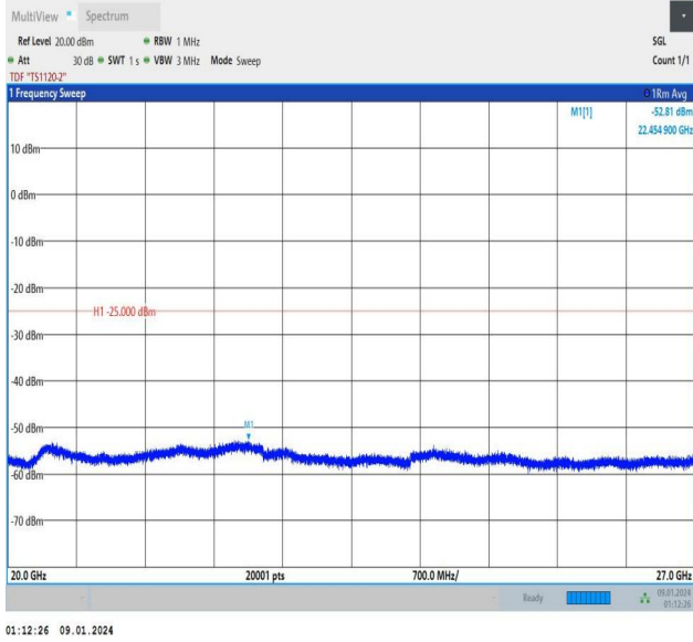
Band7_10MHz_QPSK_20800_1RB#49_20000~27000_20000~27000
