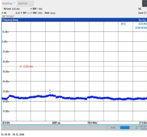
Band7_5MHz_QPSK_21425_25RB#0_20000~27000_20000~27000
