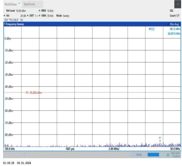
Band7_5MHz_QPSK_21425_25RB#0_0.15~30_0.15~30
