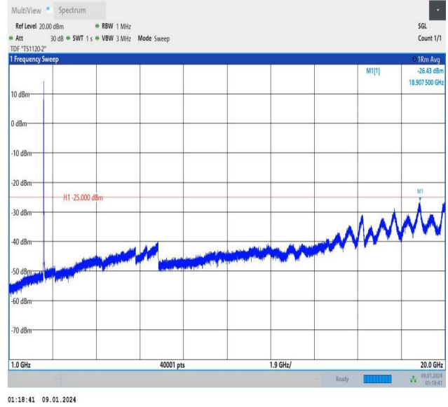
Band7_10MHz_QPSK_20800_50RB#0_1000~20000_1000~20000
