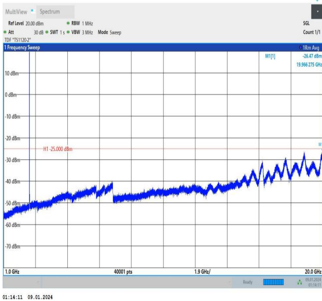
Band7_10MHz_16QAM_21100_1RB#0_1000~20000_1000~20000
