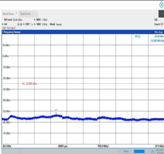
Band7_5MHz_QPSK_21100_25RB#0_20000~27000_20000~27000
