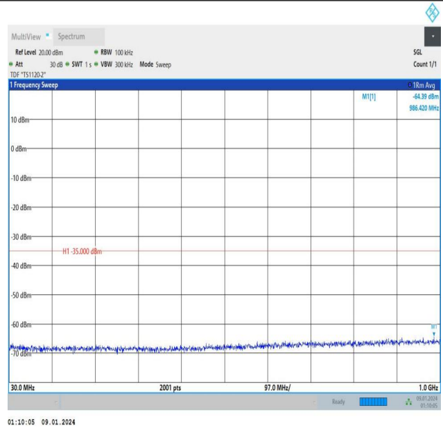
Band7_5MHz_16QAM_21425_25RB#0_30~1000_30~1000
