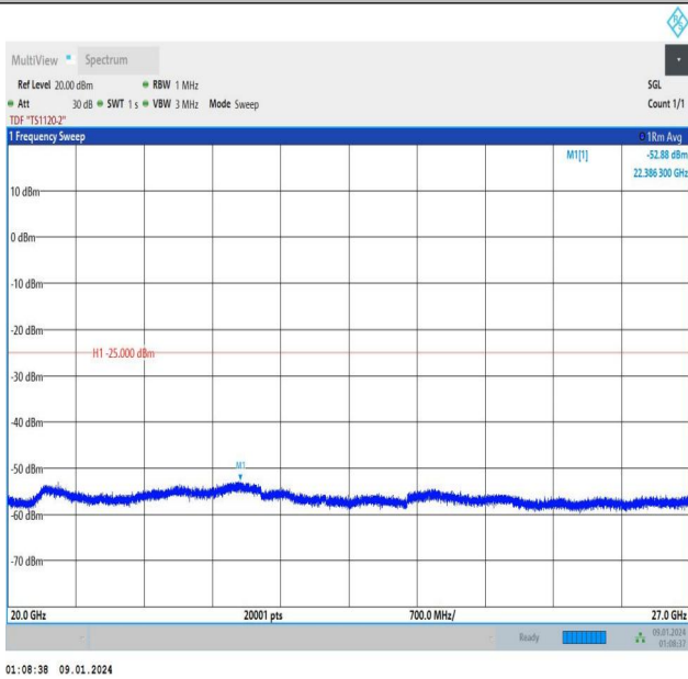
Band7_5MHz_QPSK_21425_1RB#24_20000~27000_20000~27000
