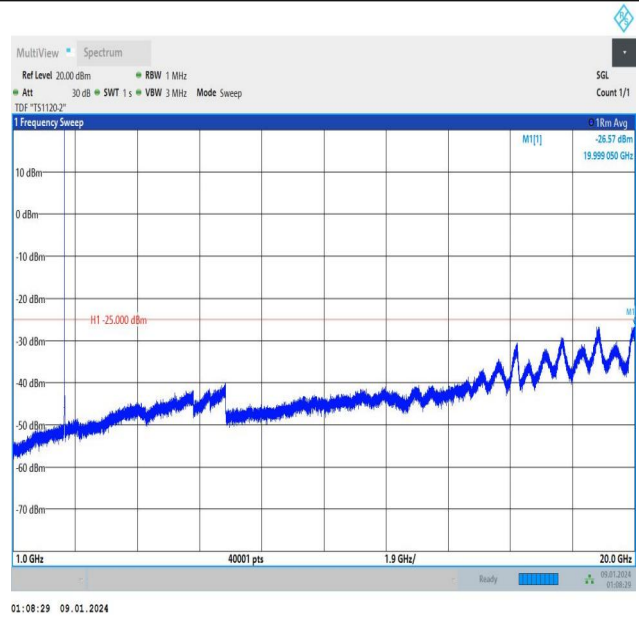
Band7_5MHz_QPSK_21425_1RB#24_1000~20000_1000~20000
