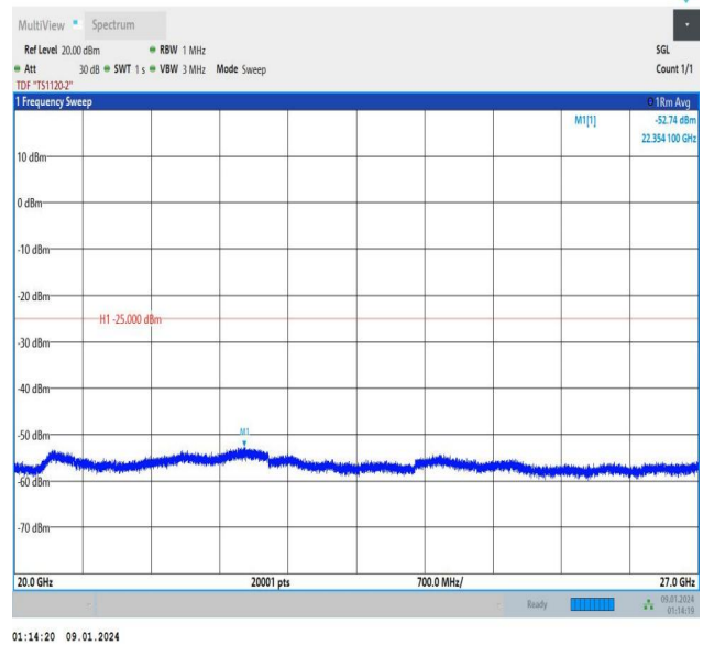
Band7_10MHz_16QAM_21100_1RB#0_20000~27000_20000~27000
