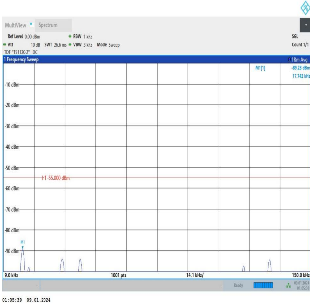
Band7_5MHz_QPSK_21100_25RB#0_0.009~0.15_0.009~0.15
