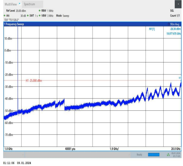
Band7_10MHz_QPSK_20800_1RB#0_1000~20000_1000~20000
