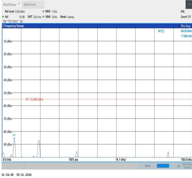
Band7_5MHz_QPSK_21100_1RB#24_0.009~0.15_0.009~0.15
