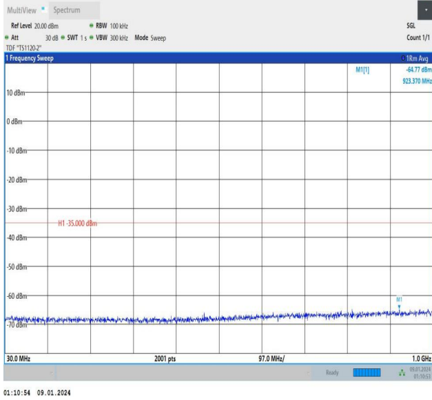
Band7_10MHz_QPSK_20800_1RB#0_30~1000_30~1000
