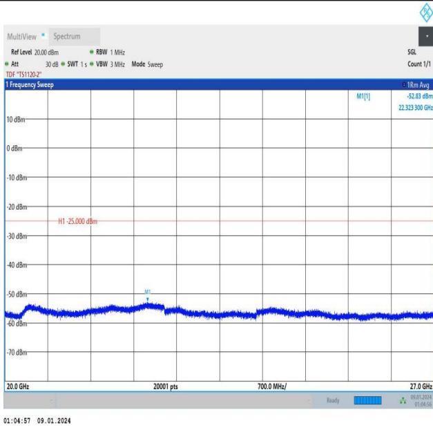
Band7_5MHz_QPSK_21100_1RB#24_20000~27000_20000~27000
