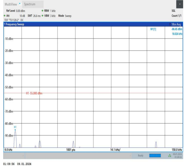
Band7_5MHz_16QAM_21425_25RB#0_0.009~0.15_0.009~0.15
