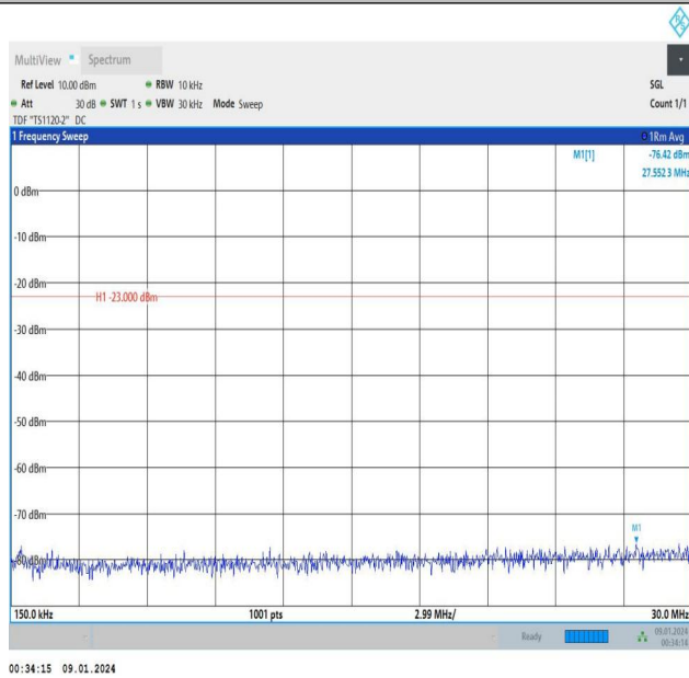
Band5_3MHz_16QAM_20635_1RB#14_0.15~30_0.15~30
