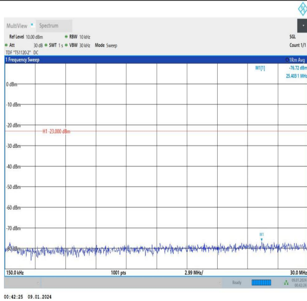
Band5_5MHz_16QAM_20525_1RB#24_0.15~30_0.15~30
