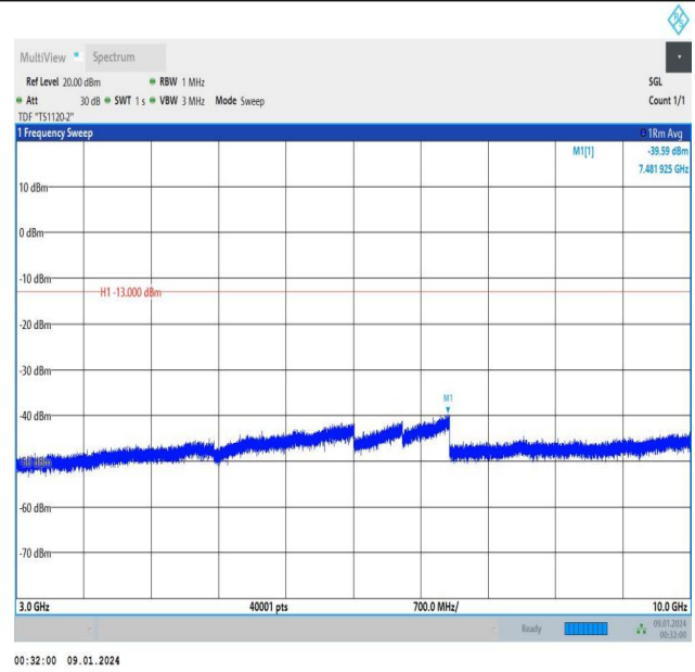
Band5_3MHz_16QAM_20525_15RB#0_3000~10000_3000~10
