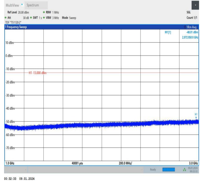
Band5_3MHz_QPSK_20635_1RB#0_1000~3000_1000~3000
