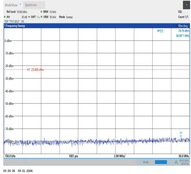
Band5_3MHz_QPSK_20635_1RB#14_0.15~30_0.15~30
