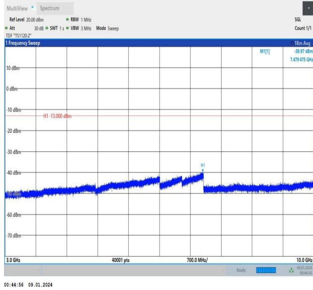
Band5_5MHz_QPSK_20625_1RB#0_3000~10000_3000~10000
