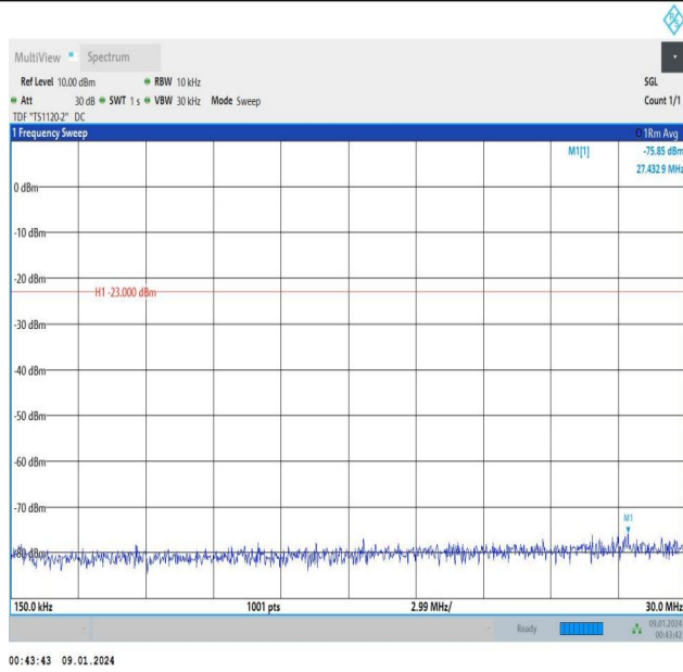
Band5_5MHz_16QAM_20525_25RB#0_0.15~30_0.15~30
