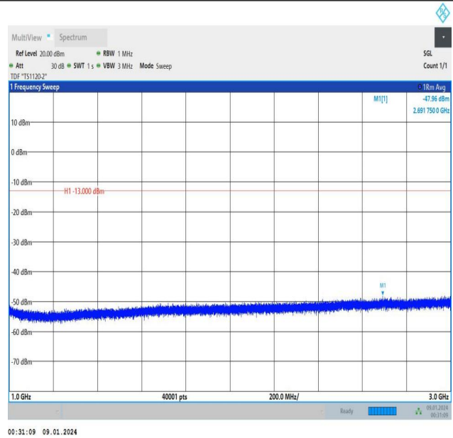
Band5_3MHz_QPSK_20525_15RB#0_1000~3000_1000~3000
