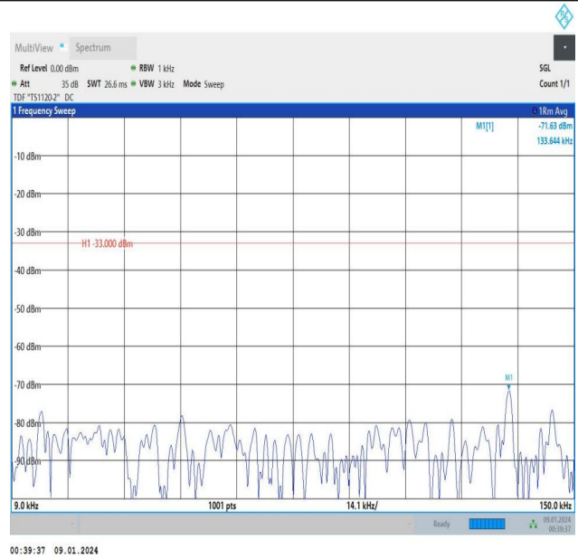
Band5_5MHz_16QAM_20425_25RB#0_0.009~0.15_0.009~0.15
