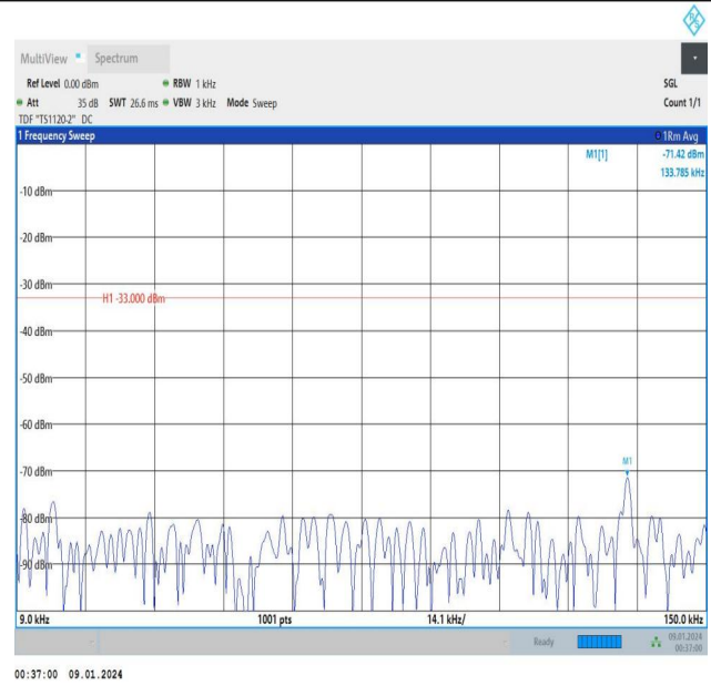
Band5_5MHz_16QAM_20425_1RB#0_0.009~0.15_0.009~0.15
