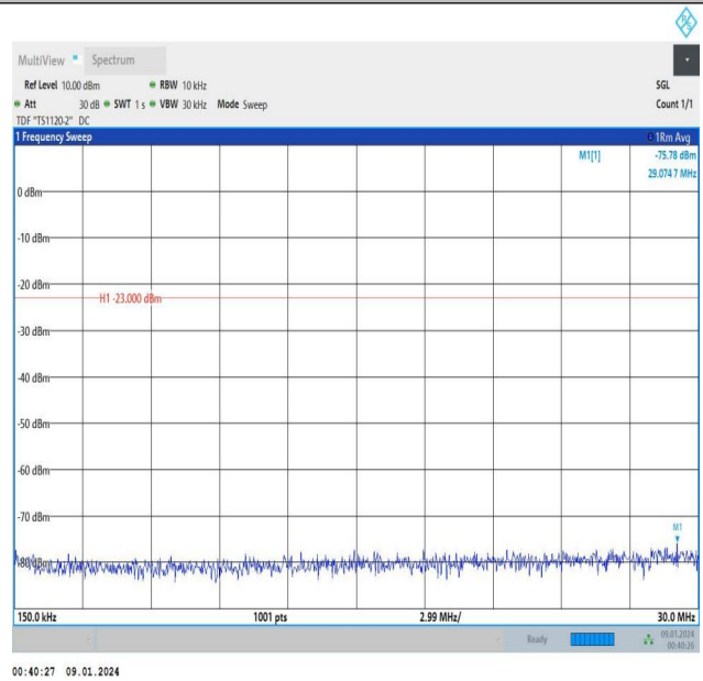
Band5_5MHz_QPSK_20525_1RB#0_0.15~30_0.15~30
