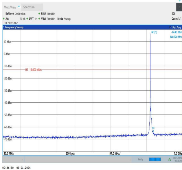
Band5_5MHz_QPSK_20425_1RB#0_30~1000_30~1000
