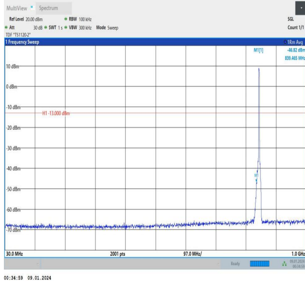
Band5_3MHz_QPSK_20635_15RB#0_30~1000_30~1000
