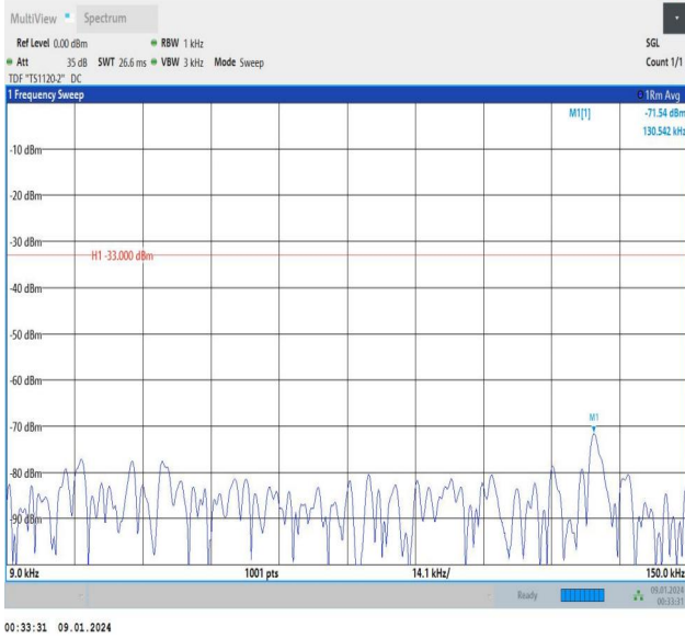
Band5_3MHz_QPSK_20635_1RB#14_0.009~0.15_0.009~0.1
