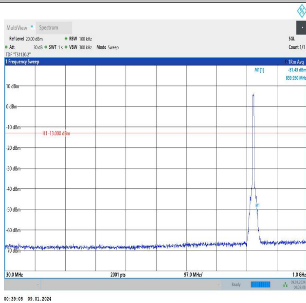
Band5_5MHz_QPSK_20425_25RB#0_30~1000_30~1000
