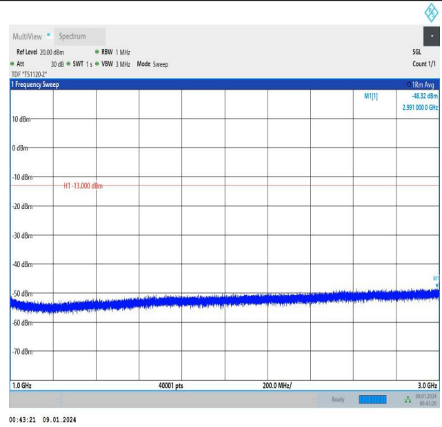
Band5_5MHz_QPSK_20525_25RB#0_1000~3000_1000~3000
