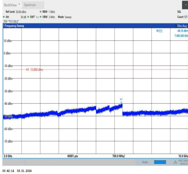
Band5_5MHz_QPSK_20525_1RB#24_3000~10000_3000~10000
