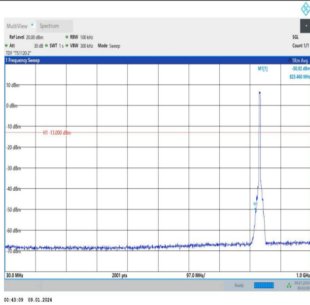
Band5_5MHz_QPSK_20525_25RB#0_30~1000_30~1000
