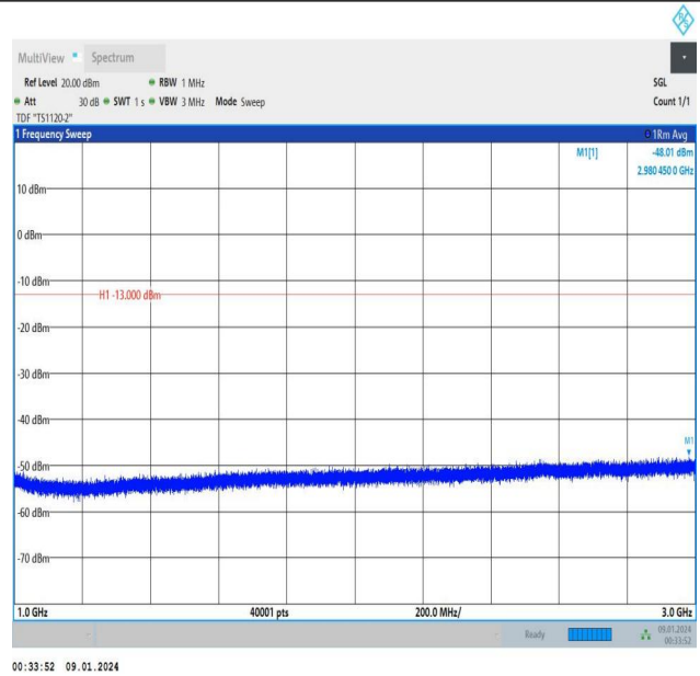
Band5_3MHz_QPSK_20635_1RB#14_1000~3000_1000~3000
