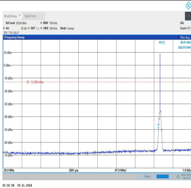
Band5_3MHz_QPSK_20525_15RB#0_30~1000_30~1000
