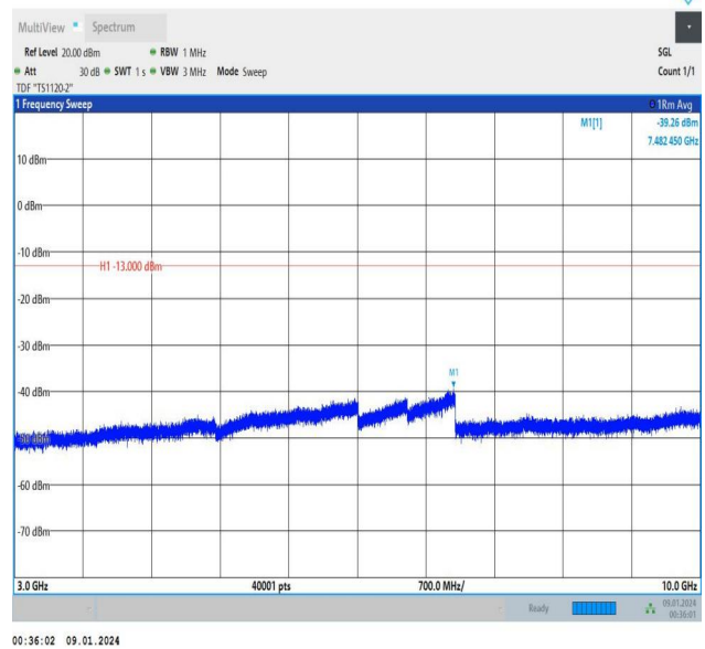
Band5_3MHz_16QAM_20635_15RB#0_3000~10000_3000~10
