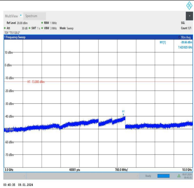
Band5_5MHz_16QAM_20625_1RB#0_3000~10000_3000~10000
