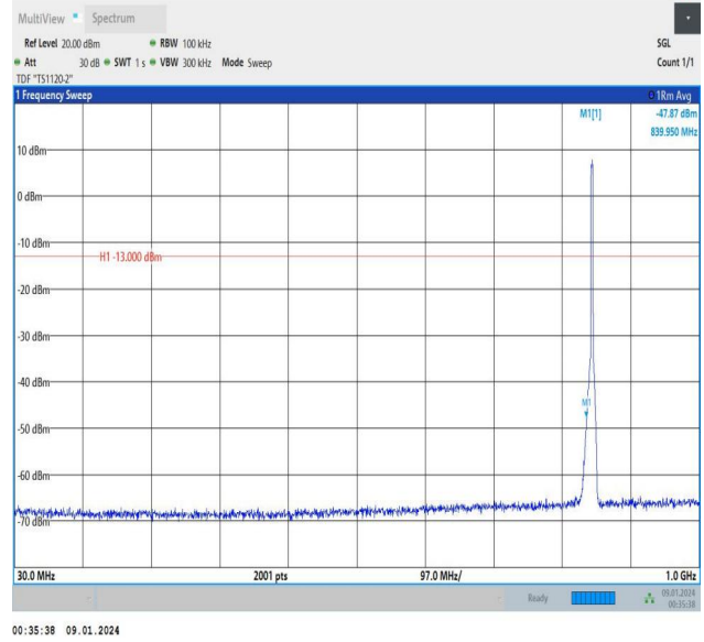
Band5_3MHz_16QAM_20635_15RB#0_30~1000_30~1000
