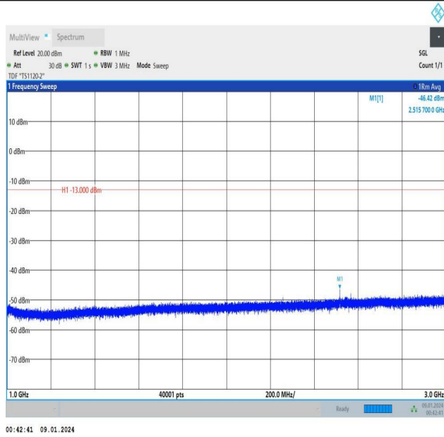
Band5_5MHz_16QAM_20525_1RB#24_1000~3000_1000~30
