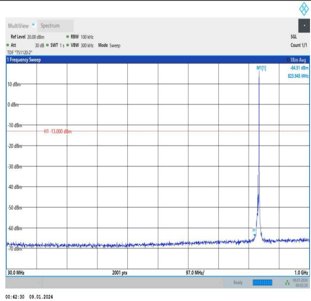
Band5_5MHz_16QAM_20525_1RB#24_30~1000_30~1000
