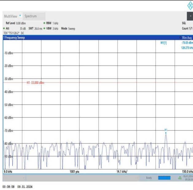
Band5_5MHz_QPSK_20425_25RB#0_0.009~0.15_0.009~0.1
