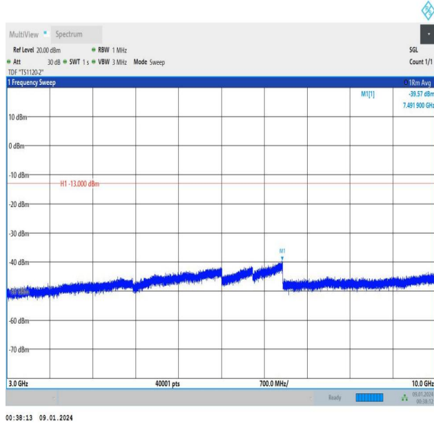
Band5_5MHz_QPSK_20425_1RB#24_3000~10000_3000~10000 000
