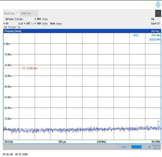
Band5_5MHz_QPSK_20525_1RB#24_0.15~30_0.15~30
