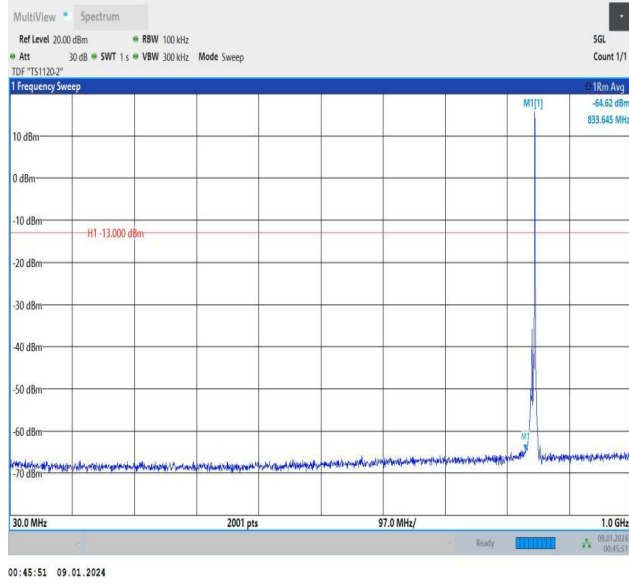
Band5_5MHz_QPSK_20625_1RB#24_30~1000_30~1000
