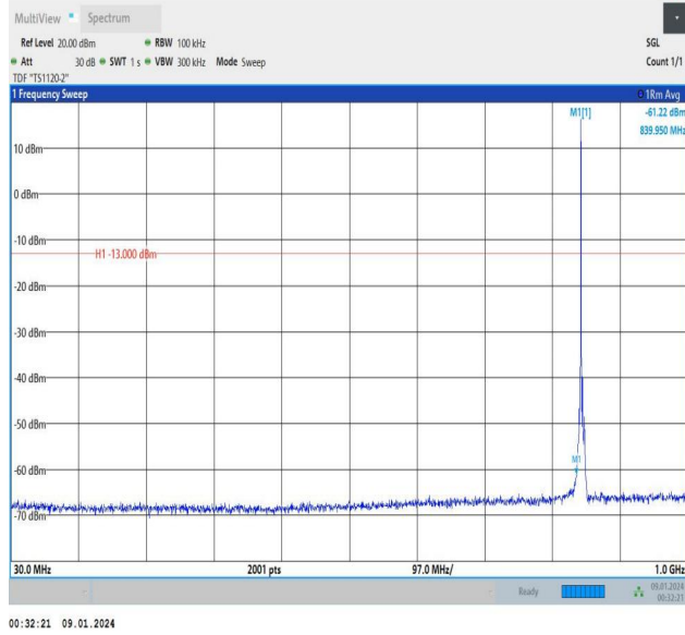
Band5_3MHz_QPSK_20635_1RB#0_30~1000_30~1000
