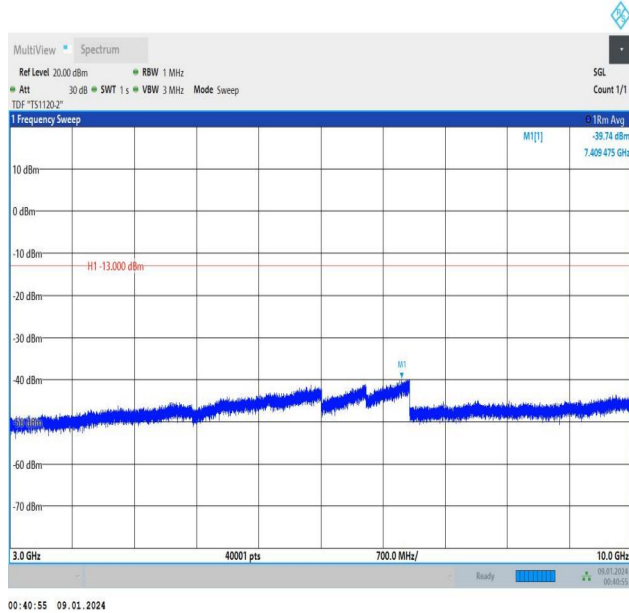
Band5_5MHz_QPSK_20525_1RB#0_3000~10000_3000~10000
