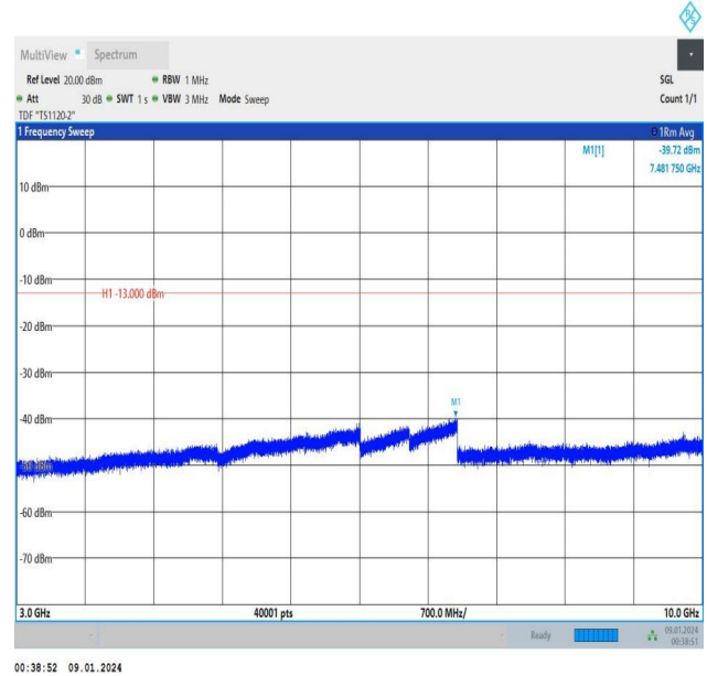
Band5_5MHz_16QAM_20425_1RB#24_3000~10000_3000~10
