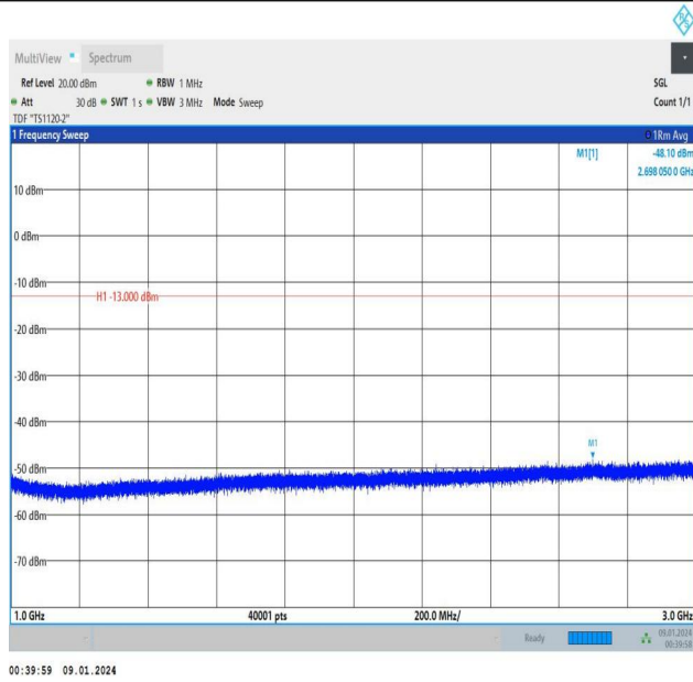
Band5_5MHz_16QAM_20425_25RB#0_1000~3000_1000~30
