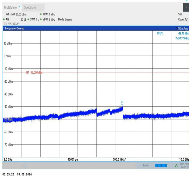
Band5_3MHz_QPSK_20635_15RB#0_3000~10000_3000~10000
