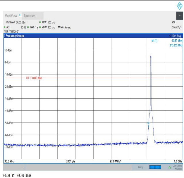
Band5_5MHz_16QAM_20425_25RB#0_30~1000_30~1000
