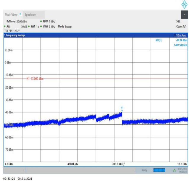
Band5_3MHz_16QAM_20635_1RB#0_3000~10000_3000~10000
