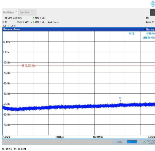
Band5_3MHz_16QAM_20635_1RB#0_1000~3000_1000~3000
