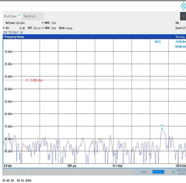
Band5_5MHz_QPSK_20525_1RB#0_0.009~0.15_0.009~0.15
