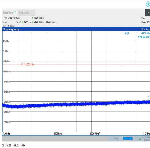
Band5_3MHz_16QAM_20635_1RB#14_1000~3000_1000~30
