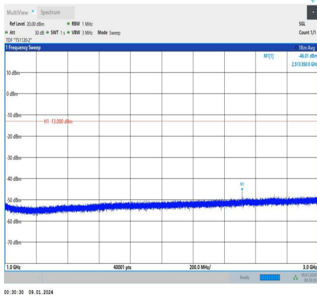
Band5_3MHz_16QAM_20525_1RB#14_1000~3000_1000~30
