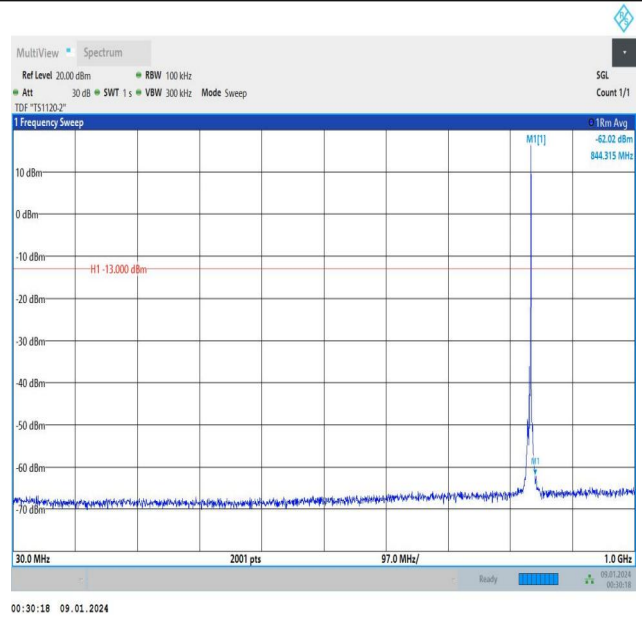
Band5_3MHz_16QAM_20525_1RB#14_30~1000_30~1000
