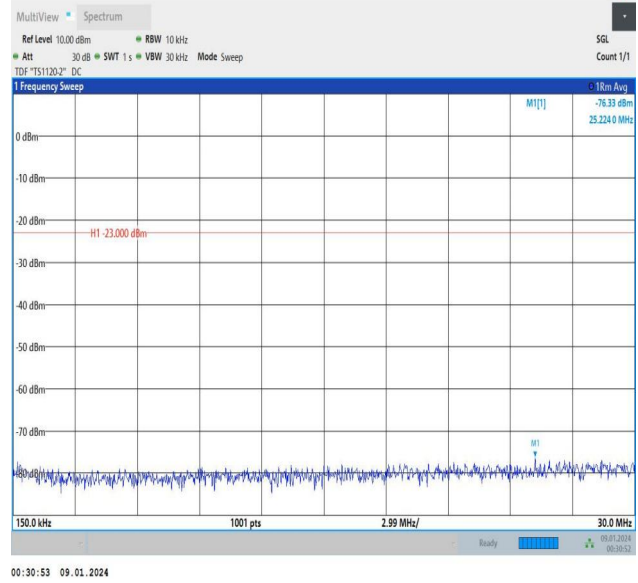
Band5_3MHz_QPSK_20525_15RB#0_0.15~30_0.15~30
