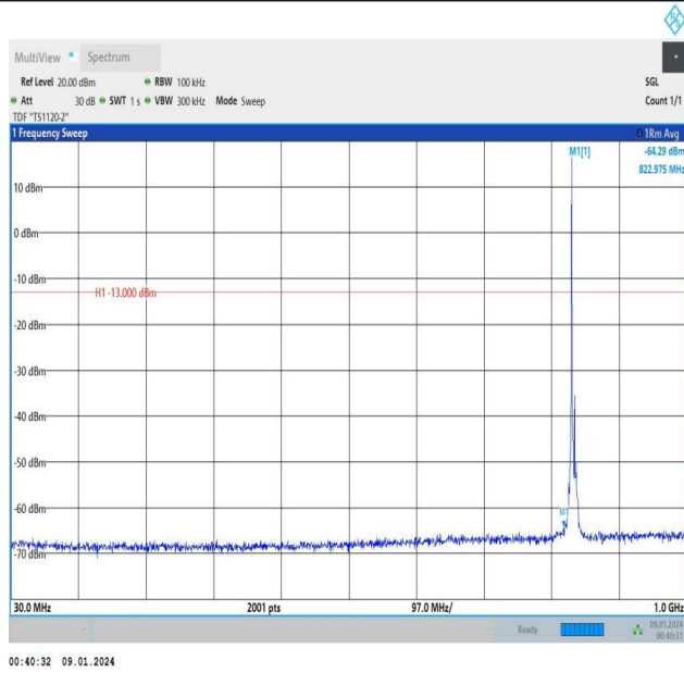
Band5_5MHz_QPSK_20525_1RB#0_30~1000_30~1000
