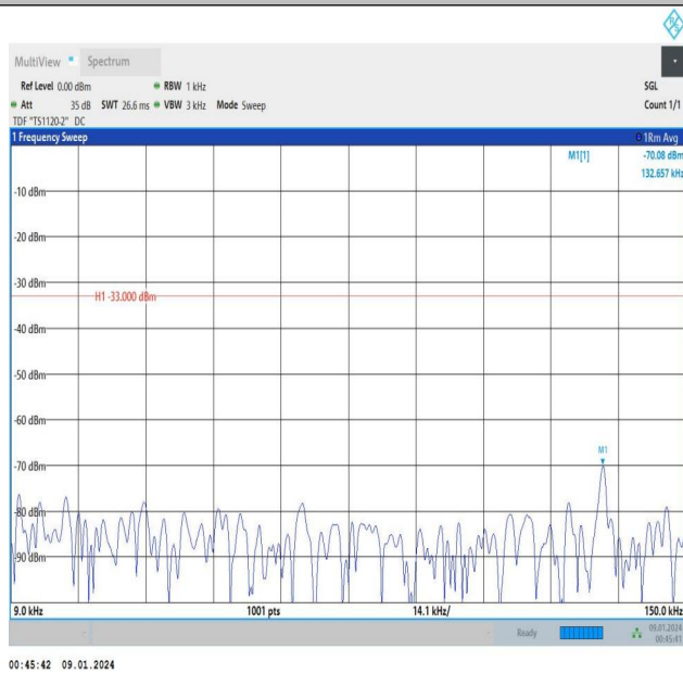
Band5_5MHz_QPSK_20625_1RB#24_0.009~0.15_0.009~0.1
