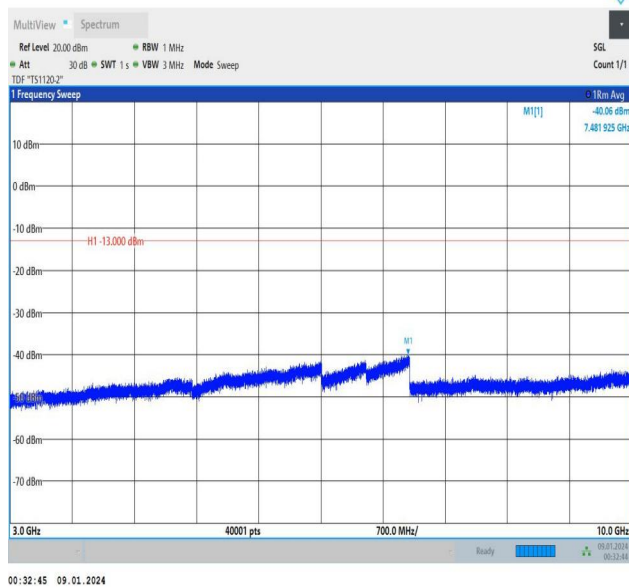
Band5_3MHz_QPSK_20635_1RB#0_3000~10000_3000~10000
