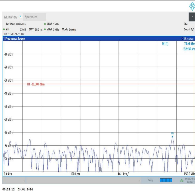
Band5_3MHz_QPSK_20635_1RB#0_0.009~0.15_0.009~0.15
