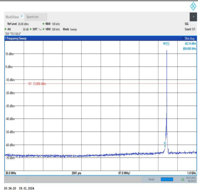
Band5_3MHz_16QAM_20635_1RB#14_30~1000_30~1000
