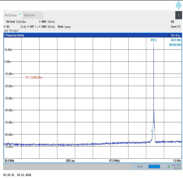
Band5_3MHz_16QAM_20635_1RB#0_30~1000_30~1000
