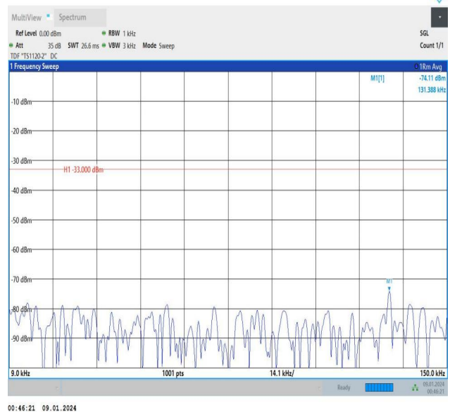
Band5_5MHz_16QAM_20625_1RB#24_0.009~0.15_0.009~0.1
