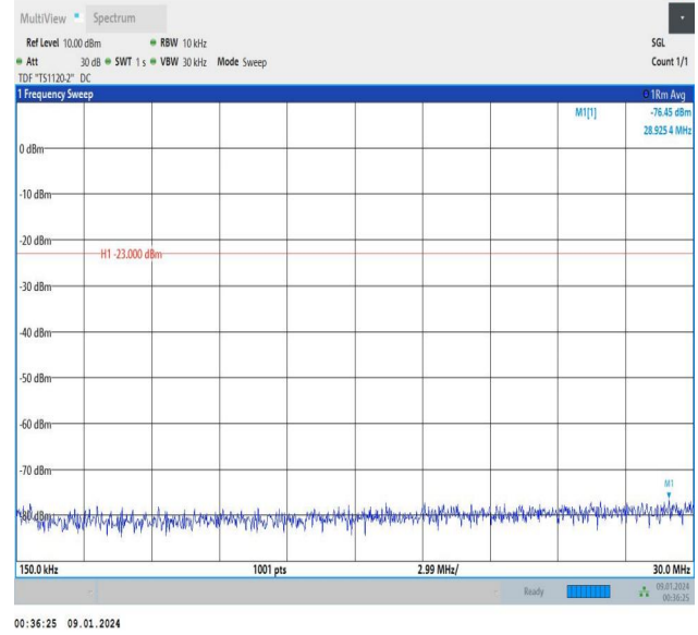
Band5_5MHz_QPSK_20425_1RB#0_0.15~30_0.15~30
