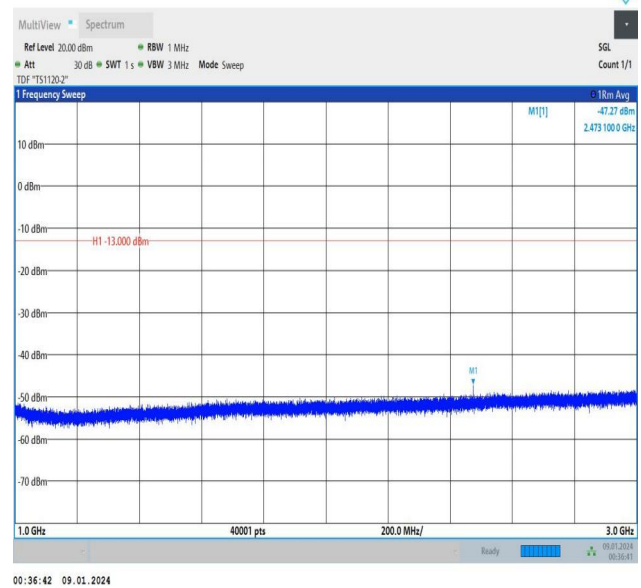
Band5_5MHz_QPSK_20425_1RB#0_1000~3000_1000~3000
