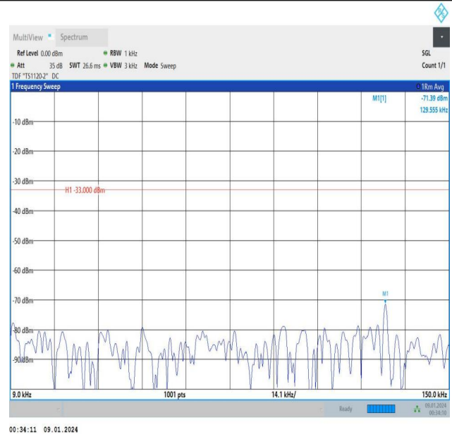
Band5_3MHz_16QAM_20635_1RB#14_0.009~0.15_0.009~0.15
