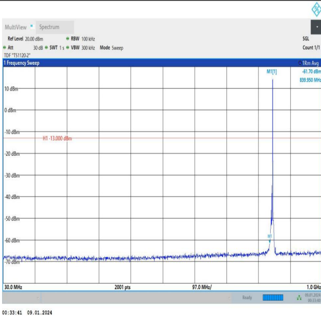
Band5_3MHz_QPSK_20635_1RB#14_30~1000_30~1000
