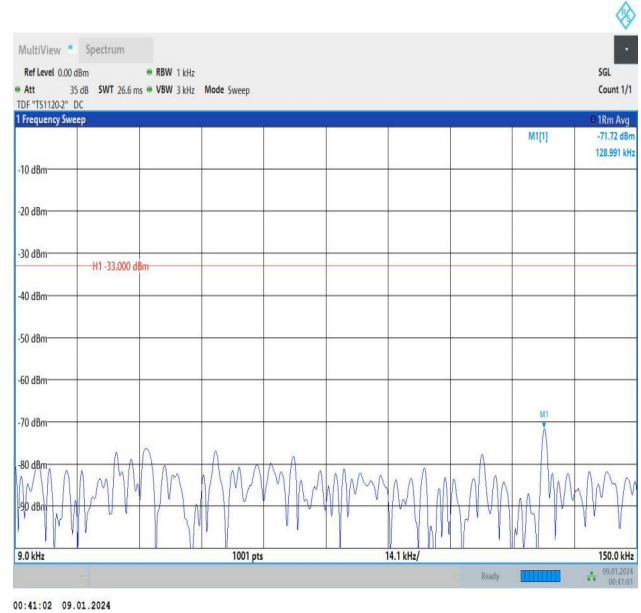
Band5_5MHz_QPSK_20525_1RB#0_1000~3000_1000~3000
