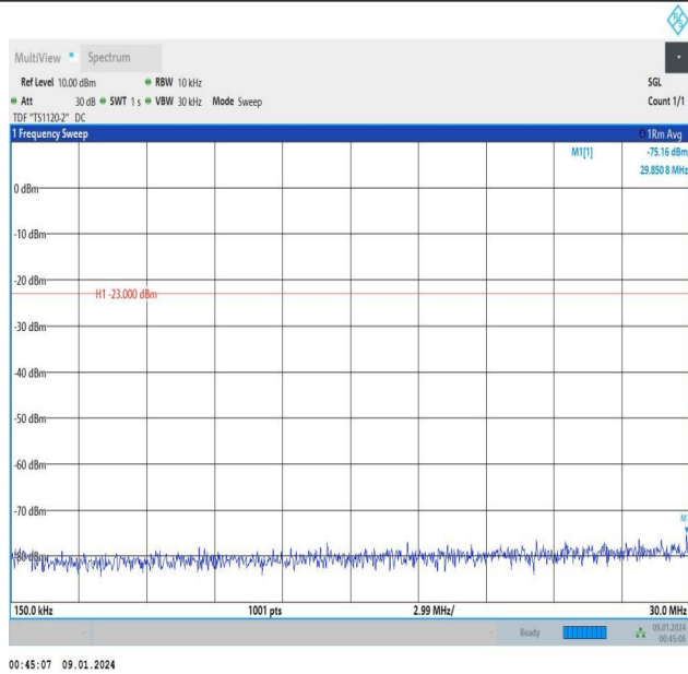
Band5_5MHz_16QAM_20625_1RB#0_0.15~30_0.15~30
