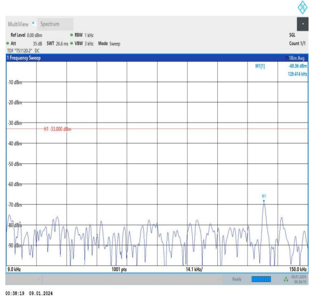
Band5_5MHz_16QAM_20425_1RB#24_0.009~0.15_0.009~0.1 5
