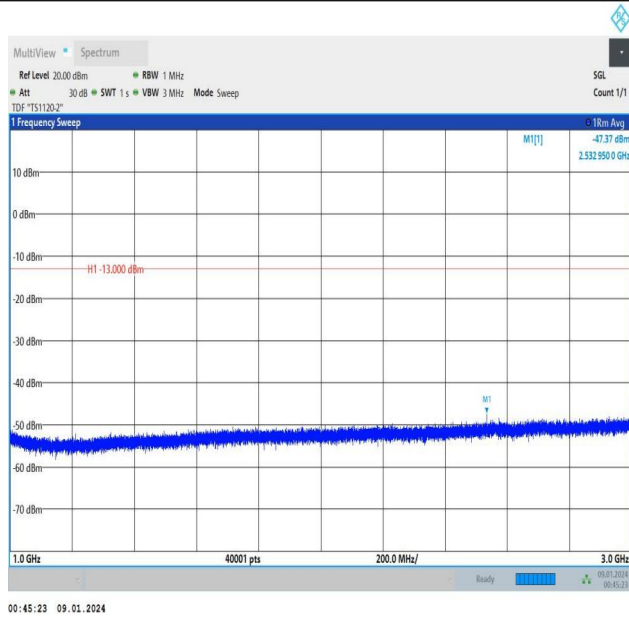
Band5_5MHz_16QAM_20625_1RB#0_1000~3000_1000~3000
