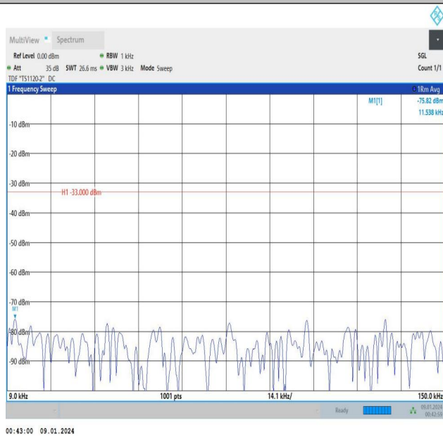
Band5_5MHz_QPSK_20525_25RB#0_0.009~0.15_0.009~0.1
