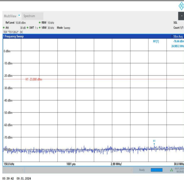
Band5_5MHz_16QAM_20425_25RB#0_0.15~30_0.15~30
