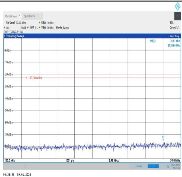
Band5_3MHz_QPSK_20635_15RB#0_0.15~30_0.15~30
