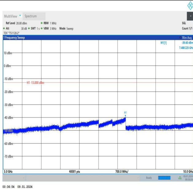
Band5_5MHz_QPSK_20425_1RB#0_3000~10000_3000~10000
