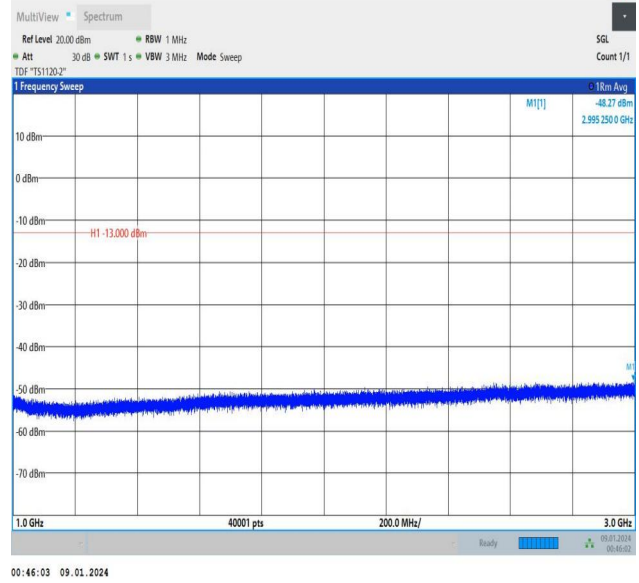
Band5_5MHz_QPSK_20625_1RB#24_1000~3000_1000~3000
