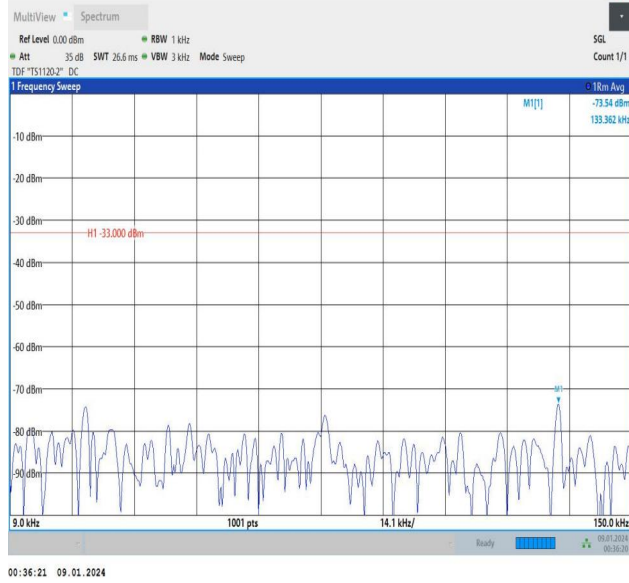
Band5_5MHz_QPSK_20425_1RB#0_0.009~0.15_0.009~0.15
