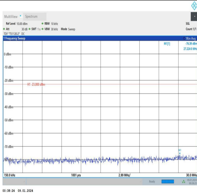
Band5_5MHz_16QAM_20425_1RB#24_0.15~30_0.15~30
