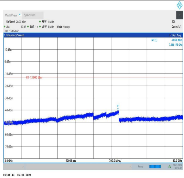
Band5_3MHz_16QAM_20635_1RB#14_3000~10000_3000~10
