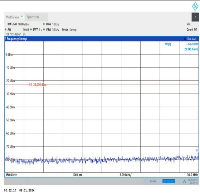
Band5_3MHz_QPSK_20635_1RB#0_0.15~30_0.15~30
