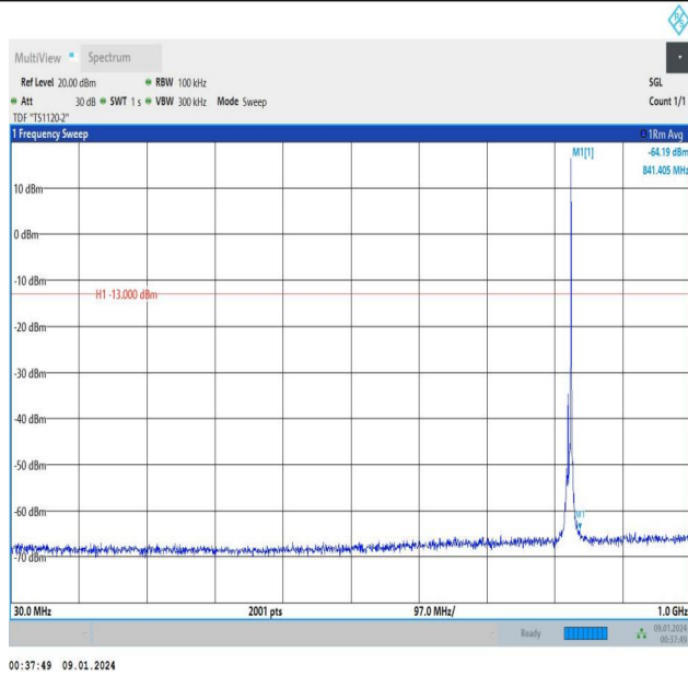
Band5_5MHz_QPSK_20425_1RB#24_30~1000_30~1000
