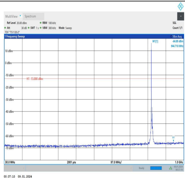
Band5_5MHz_16QAM_20425_1RB#0_30~1000_30~1000
