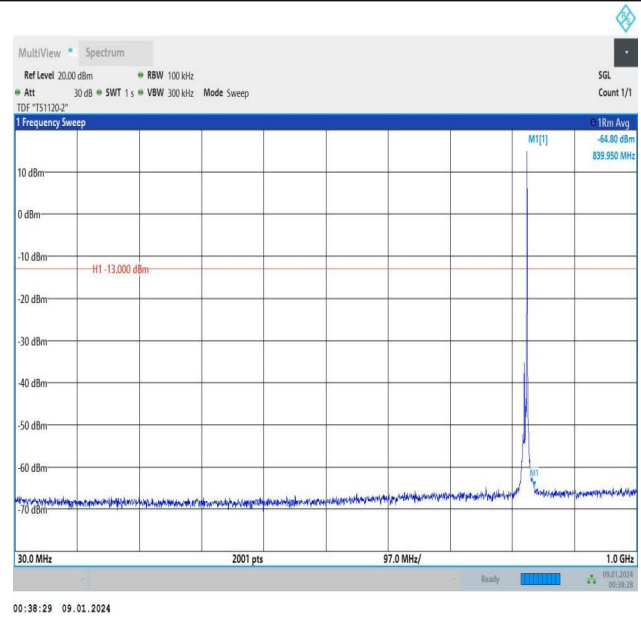
Band5_5MHz_16QAM_20425_1RB#24_30~1000_30~1000
