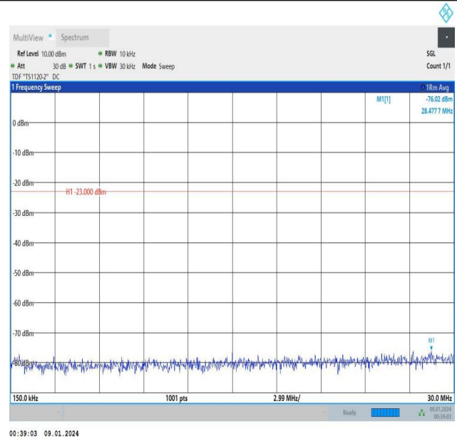
Band5_5MHz_QPSK_20425_25RB#0_0.15~30_0.15~30
