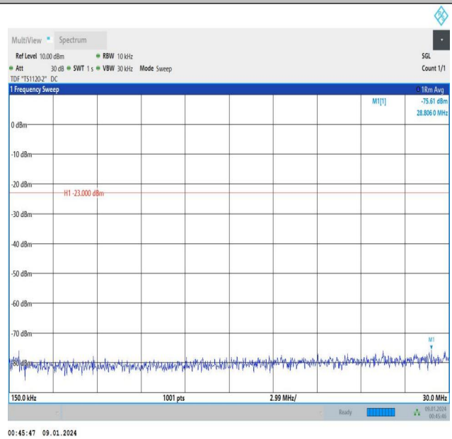
Band5_5MHz_QPSK_20625_1RB#24_0.15~30_0.15~30
