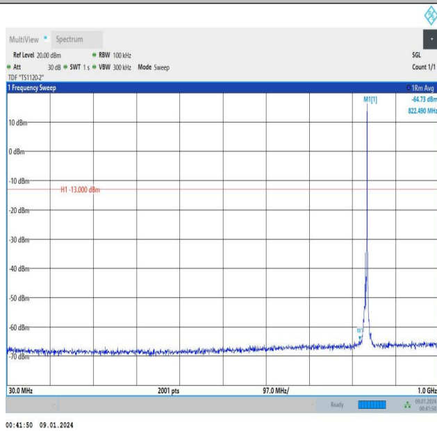
Band5_5MHz_QPSK_20525_1RB#24_30~1000_30~1000
