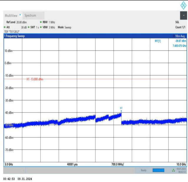
Band5_5MHz_16QAM_20525_1RB#24_3000~10000_3000~10
