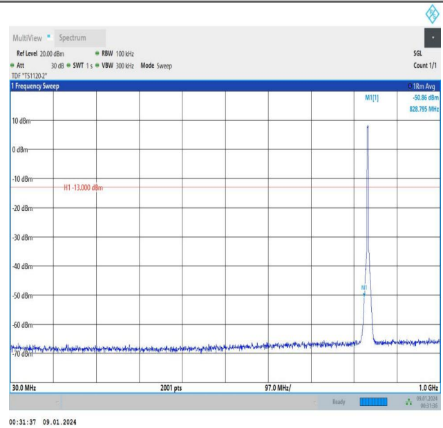
Band5_3MHz_16QAM_20525_15RB#0_30~1000_30~1000
