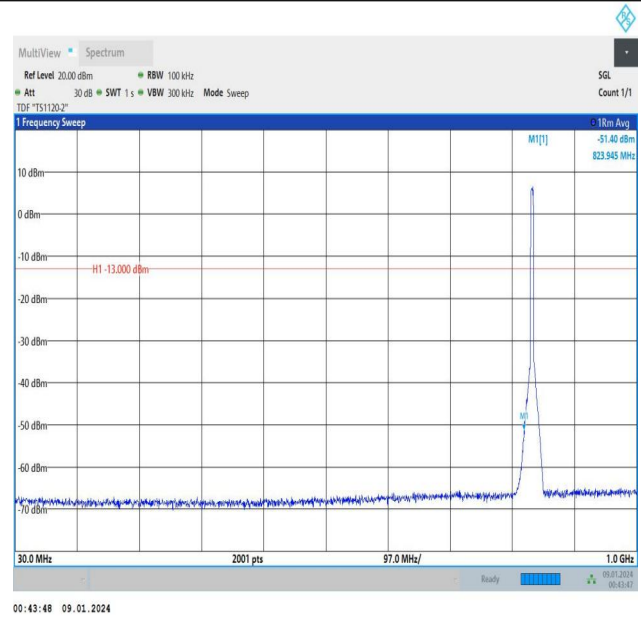
Band5_5MHz_16QAM_20525_25RB#0_30~1000_30~1000
