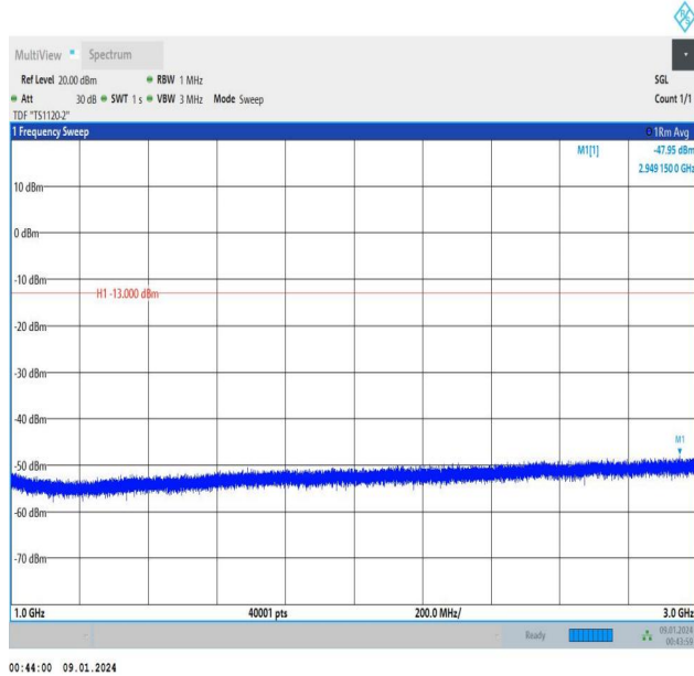
Band5_5MHz_16QAM_20525_25RB#0_1000~3000_1000~30
