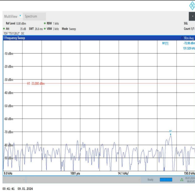
Band5_5MHz_QPSK_20525_1RB#24_0.009~0.15_0.009~0.1
