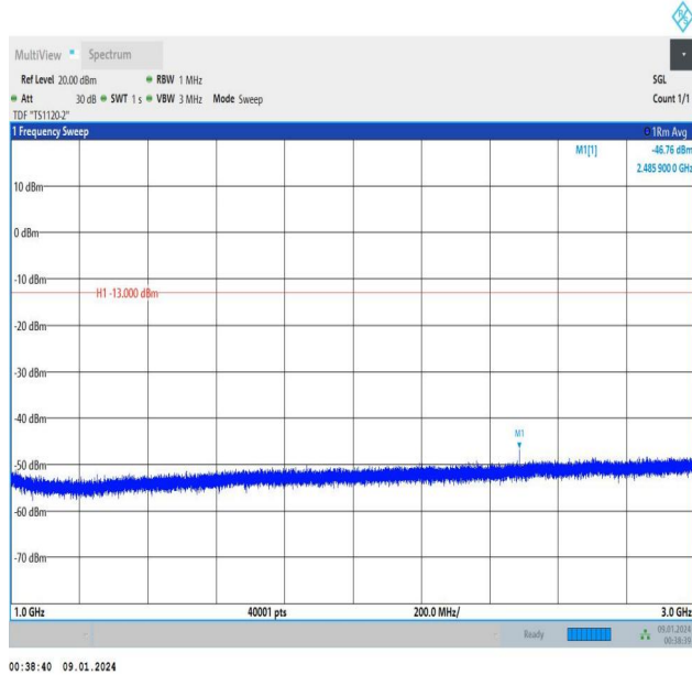
Band5_5MHz_16QAM_20425_1RB#24_1000~3000_1000~30
