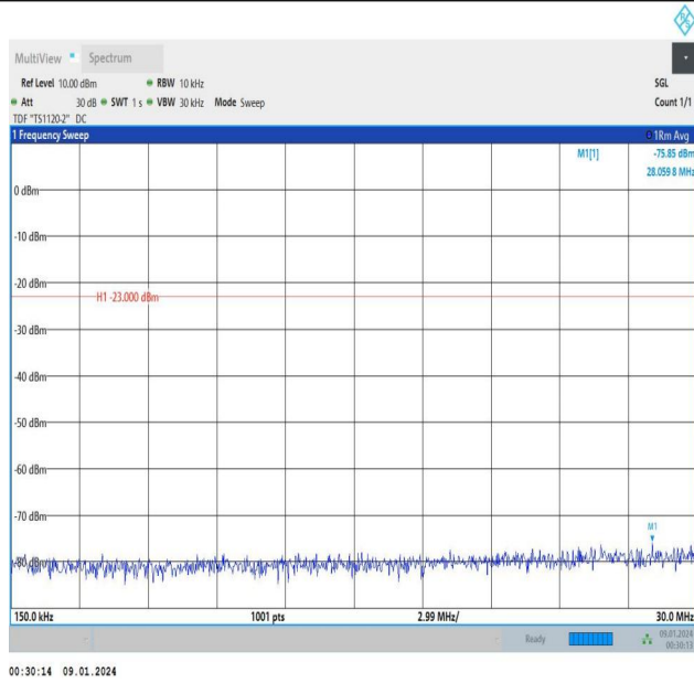
Band5_3MHz_16QAM_20525_1RB#14_0.15~30_0.15~30
