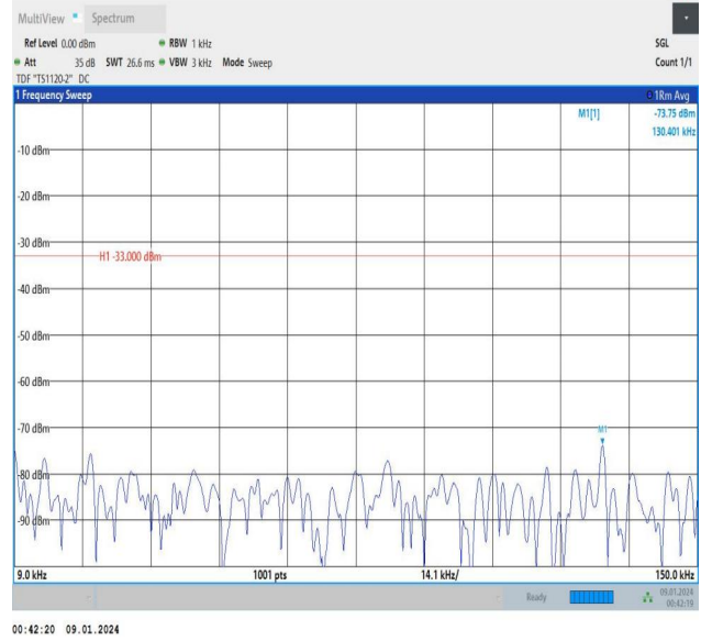
Band5_5MHz_16QAM_20525_1RB#24_0.009~0.15_0.009~0.155
