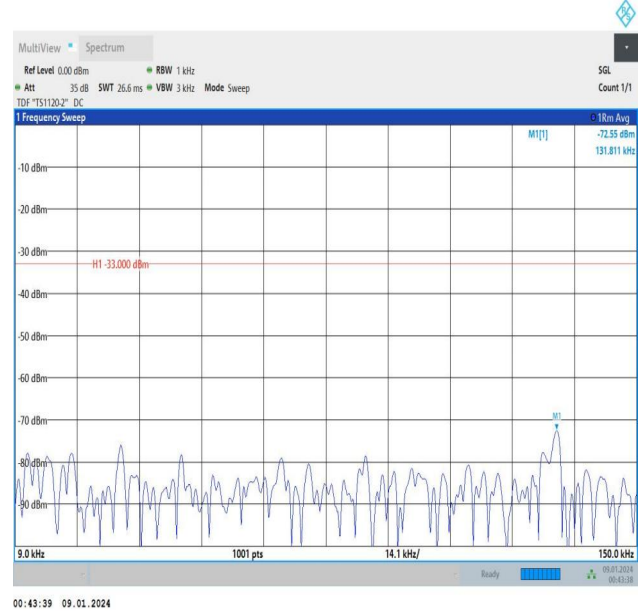
Band5_5MHz_16QAM_20525_25RB#0_0.009~0.15_0.009~0.1
