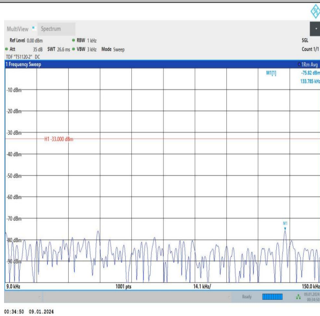
Band5_3MHz_QPSK_20635_15RB#0_0.009~0.15_0.009~0.1
