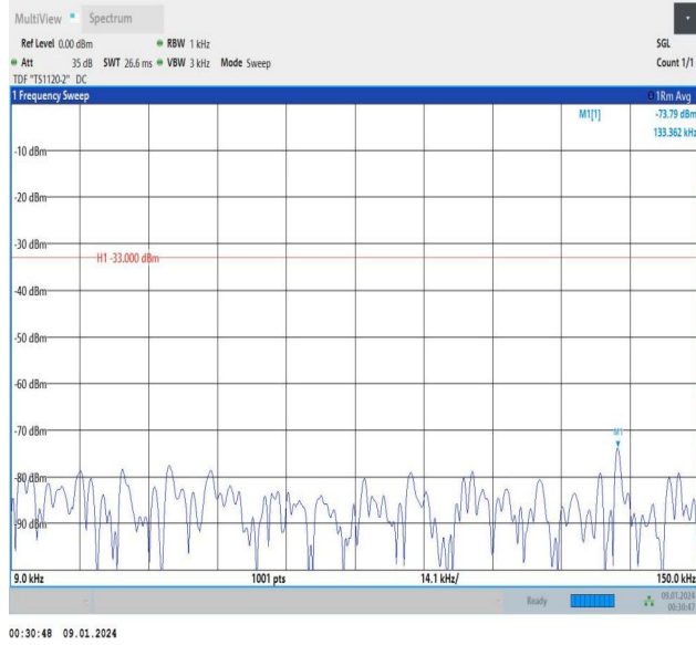
Band5_3MHz_QPSK_20525_15RB#0_0.009~0.15_0.009~0.1
