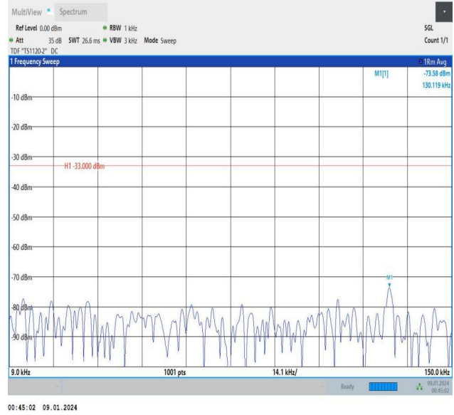
Band5_5MHz_16QAM_20625_1RB#0_0.009~0.15_0.009~0.15
