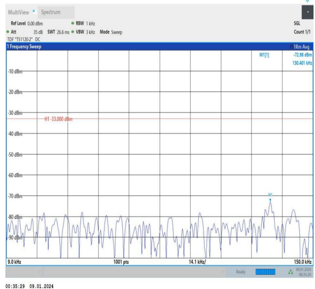
Band5_3MHz_16QAM_20635_15RB#0_0.009~0.15_0.009~0.1
