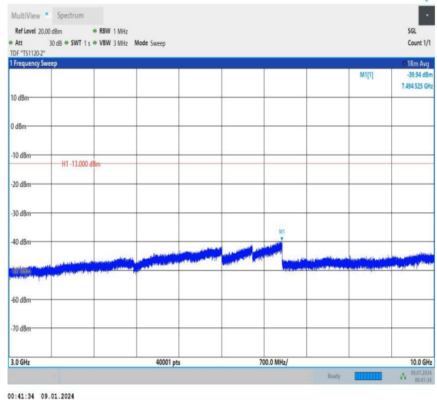
Band5_5MHz_16QAM_20525_1RB#0_3000~10000_3000~10000
