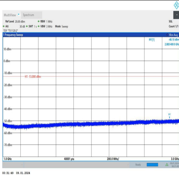
Band5_3MHz_16QAM_20525_15RB#0_1000~3000_1000~30
