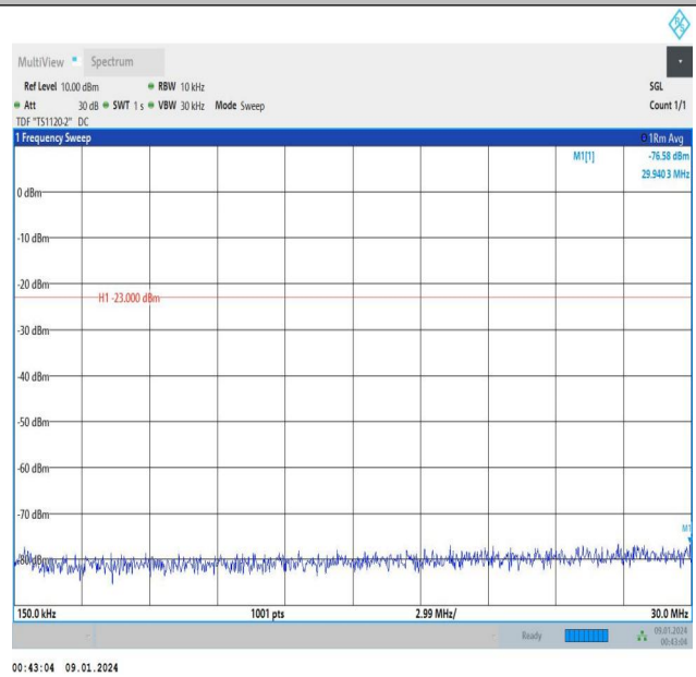
Band5_5MHz_QPSK_20525_25RB#0_0.15~30_0.15~30
