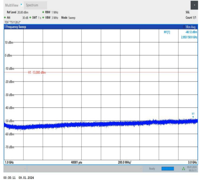
Band5_3MHz_QPSK_20635_15RB#0_1000~3000_1000~3000
