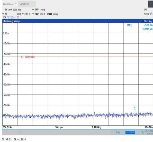
Band5_3MHz_16QAM_20635_15RB#0_0.15~30_0.15~30
