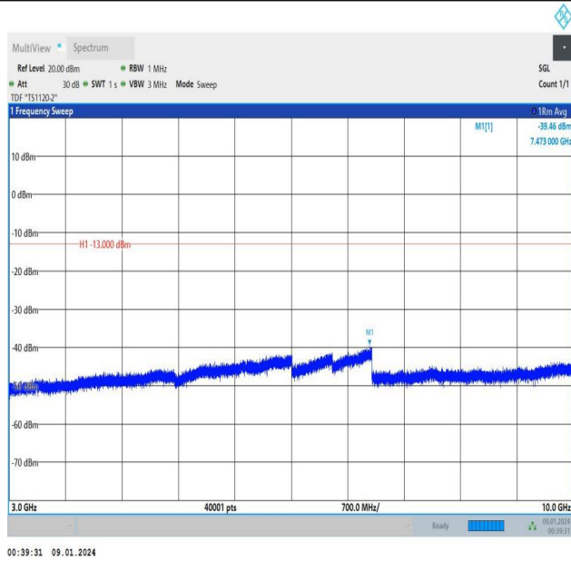
Band5_5MHz_QPSK_20425_25RB#0_3000~10000_3000~10000
