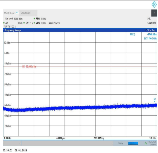
Band5_5MHz_QPSK_20425_1RB#24_1000~3000_1000~3000
