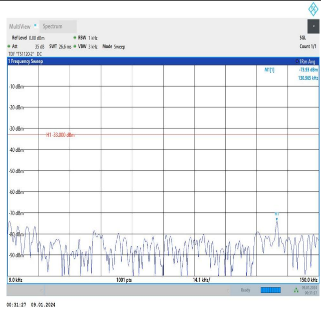
Band5_3MHz_16QAM_20525_15RB#0_0.009~0.15_0.009~0.15
