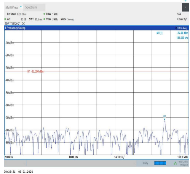
Band5_3MHz_16QAM_20635_1RB#0_0.009~0.15_0.009~0.15
