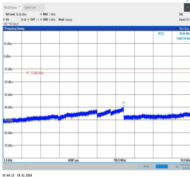
Band5_5MHz_QPSK_20625_1RB#24_3000~10000_3000~10000
