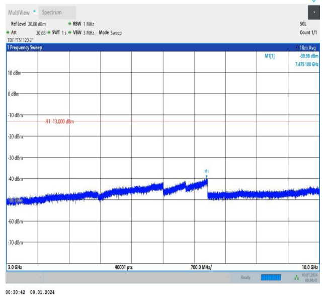
Band5_3MHz_16QAM_20525_1RB#14_3000~10000_3000~10
