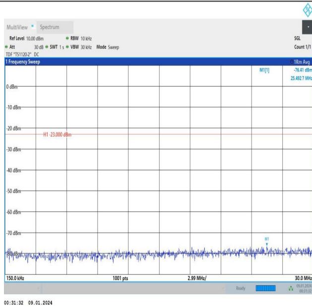
Band5_3MHz_16QAM_20525_15RB#0_0.15~30_0.15~30
