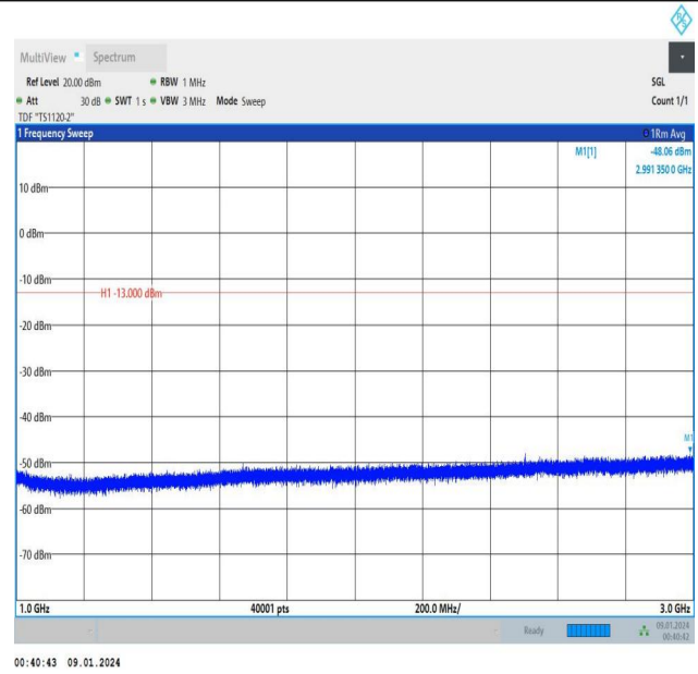
Band5_5MHz_QPSK_20525_1RB#0_1000~3000_1000~3000
