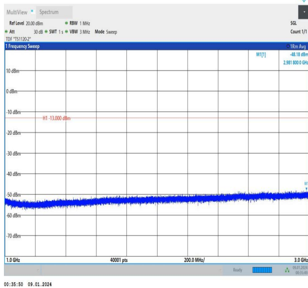
Band5_3MHz_16QAM_20635_15RB#0_1000~3000_1000~30
