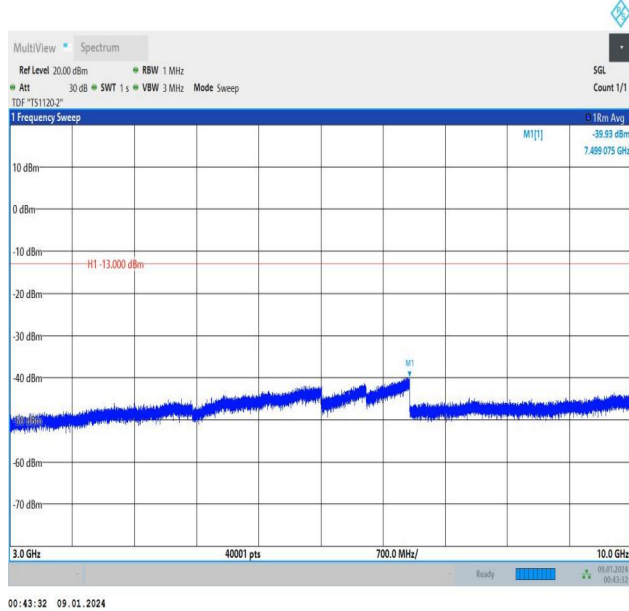
Band5_5MHz_QPSK_20525_25RB#0_3000~10000_3000~10000
