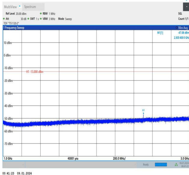
Band5_5MHz_16QAM_20525_1RB#0_1000~3000_1000~3000
