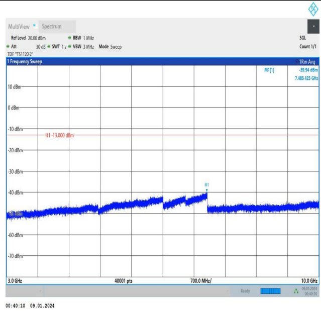
Band5_5MHz_16QAM_20425_25RB#0_3000~10000_3000~10
