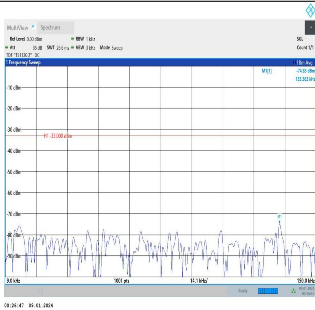
Band5_3MHz_QPSK_20415_15RB#0_0.009~0.15_0.009~0.1
