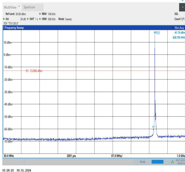
Band5_3MHz_QPSK_20525_1RB#0_30~1000_30~1000
