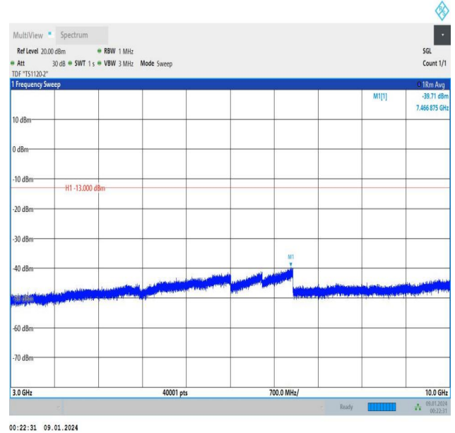
Band5_1.4MHz_16QAM_20643_1RB#5_3000~10000_3000~10000
