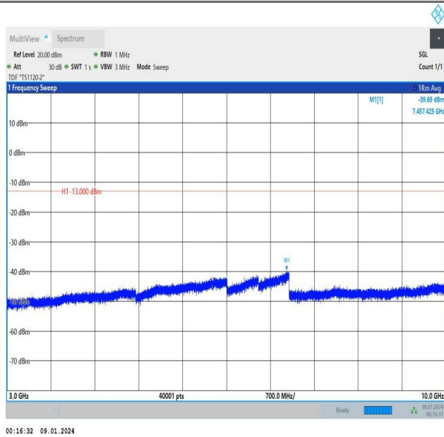
Band5_1.4MHz_QPSK_20525_1RB#0_3000~10000_3000~1 0000
