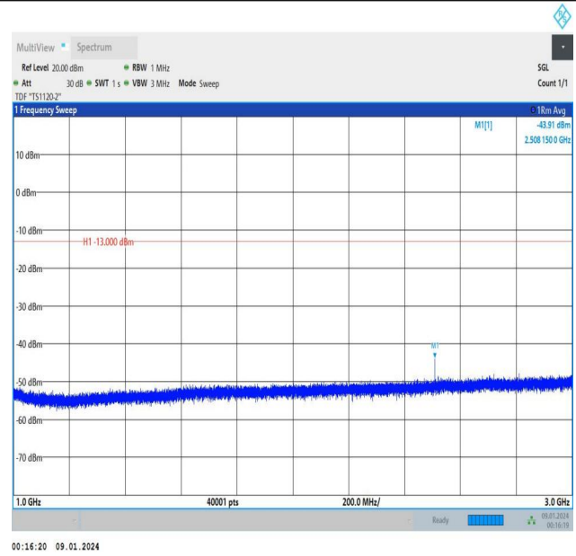
Band5_1.4MHz_QPSK_20525_1RB#0_1000~3000_1000~300 0
