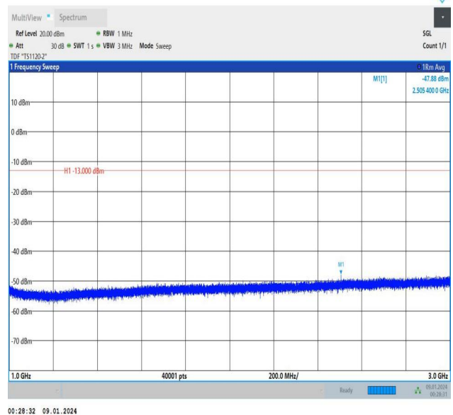
Band5_3MHz_QPSK_20525_1RB#0_1000~3000_1000~3000
