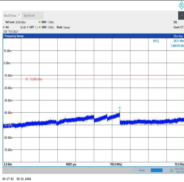
Band5_1.4MHz_QPSK_20525_1RB#5_3000~10000_3000~10000
