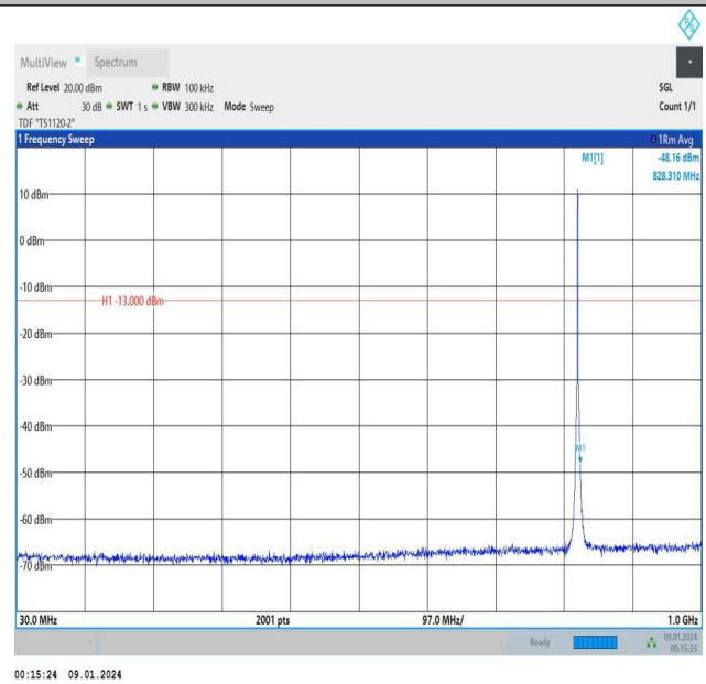
Band5_1.4MHz_16QAM_20407_6RB#0_30~1000_30~1000
