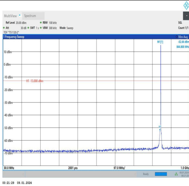
Band5_1.4MHz_QPSK_20643_1RB#5_30~1000_30~1000
