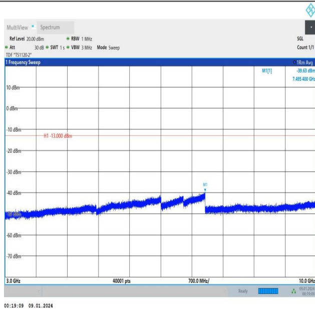
Band5_1.4MHz_QPSK_20525_6RB#0_3000~10000_3000~1 0000
