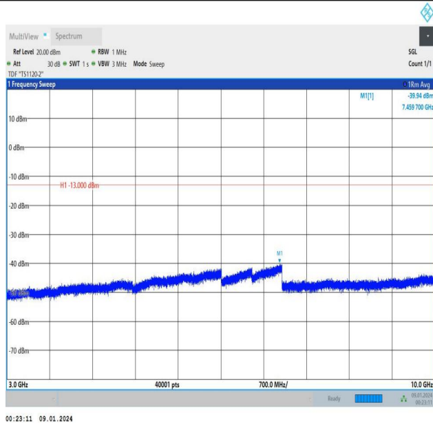
Band5_1.4MHz_QPSK_20643_6RB#0_3000~10000_3000~10000
