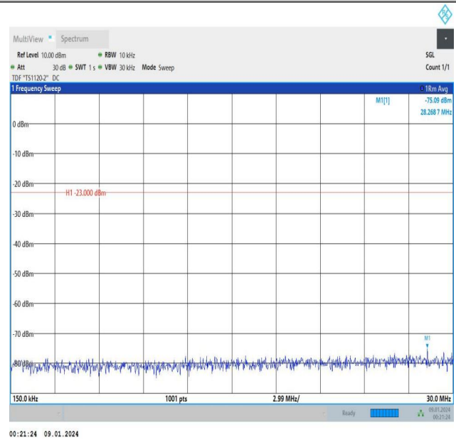
Band5_1.4MHz_QPSK_20643_1RB#5_0.15~30_0.15~30
