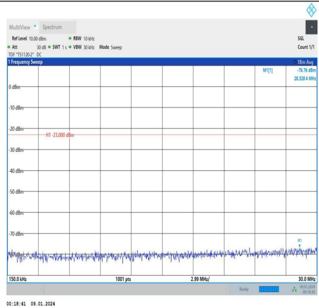
Band5_1.4MHz_QPSK_20525_6RB#0_0.15~30_0.15~30
