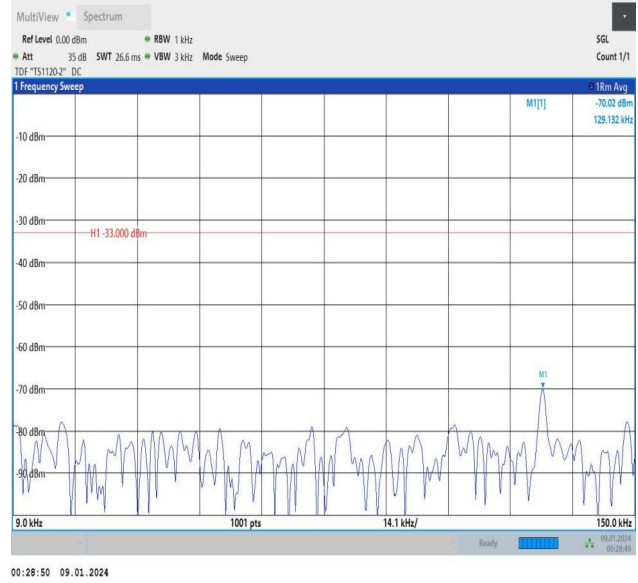
Band5_3MHz_16QAM_20525_1RB#0_0.009~0.15_0.009~0.15
