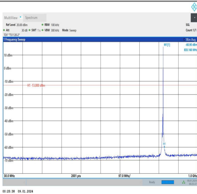
Band5_3MHz_QPSK_20415_1RB#14_30~1000_30~1000
