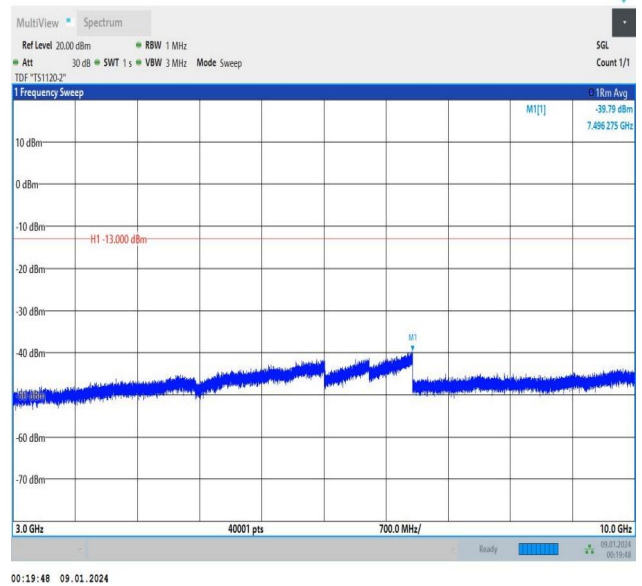
Band5_1.4MHz_16QAM_20525_6RB#0_3000~10000_3000~10000
