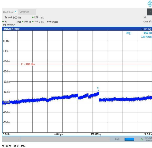
Band5_3MHz_QPSK_20525_1RB#14_3000~10000_3000~10000
