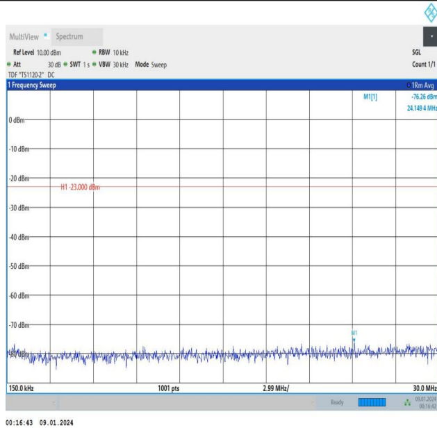
Band5_1.4MHz_16QAM_20525_1RB#0_0.15~30_0.15~30
