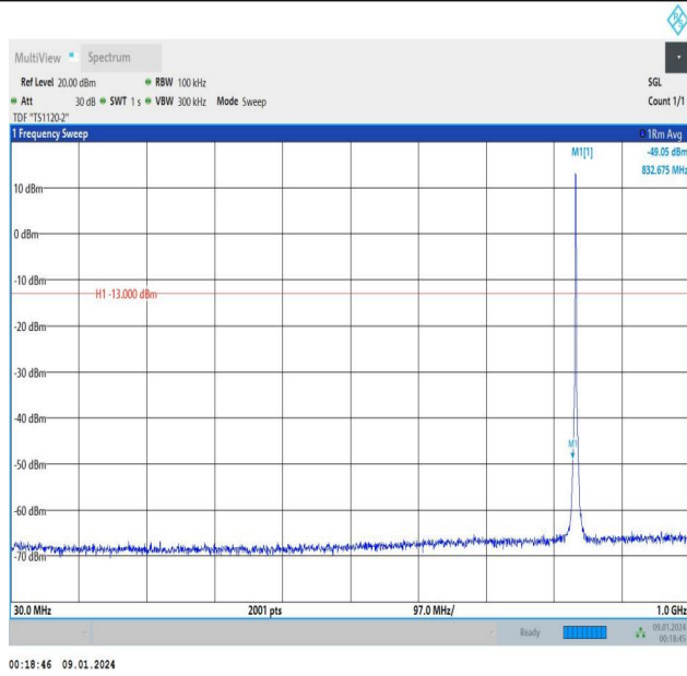
Band5_1.4MHz_QPSK_20525_6RB#0_30~1000_30~1000
