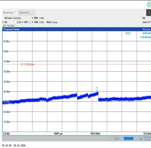
Band5_1.4MHz_QPSK_20407_6RB#0_3000~10000_3000~10000
