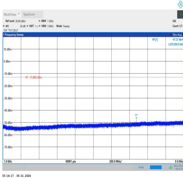
Band5_1.4MHz_16QAM_20407_1RB#5_1000~3000_1000~3000
