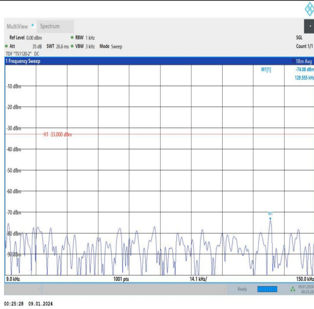
Band5_3MHz_QPSK_20415_1RB#14_0.009~0.15_0.009~0.1
