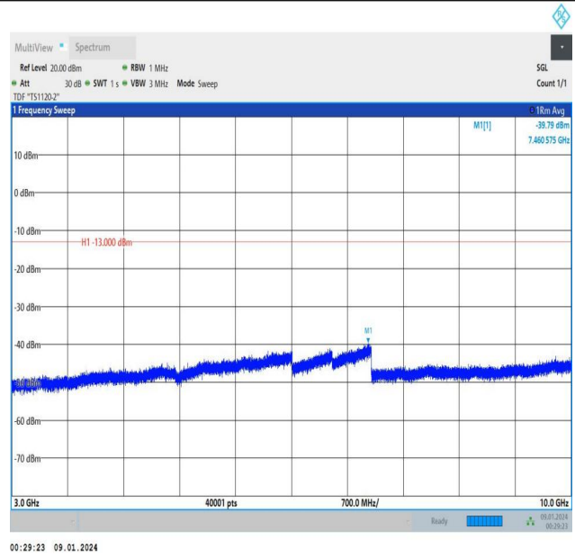
Band5_3MHz_16QAM_20525_1RB#0_3000~10000_3000~10000
