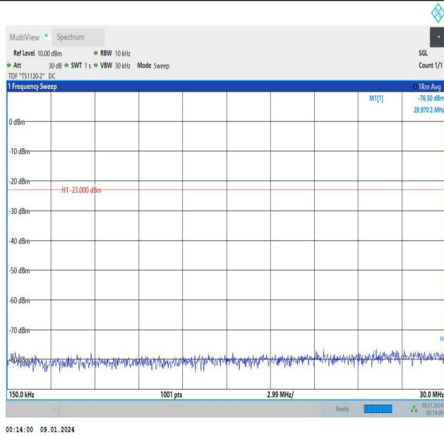
Band5_1.4MHz_16QAM_20407_1RB#5_0.15~30_0.15~30
