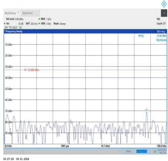
Band5_3MHz_16QAM_20415_15RB#0_0.009~0.15_0.009~0.1
