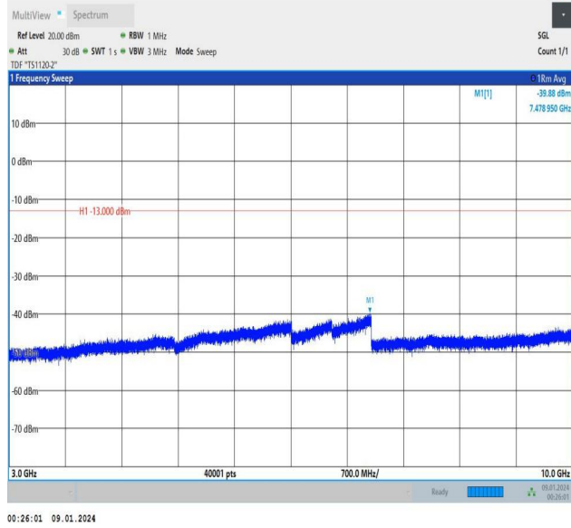
Band5_3MHz_QPSK_20415_1RB#14_3000~10000_3000~10000
