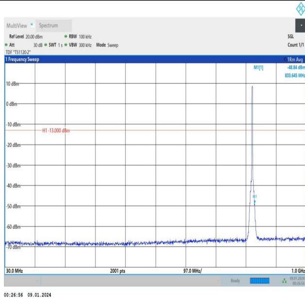
Band5_3MHz_QPSK_20415_15RB#0_30~1000_30~1000
