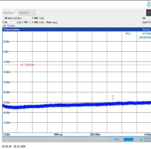
Band5_3MHz_16QAM_20415_1RB#14_1000~3000_1000~30
