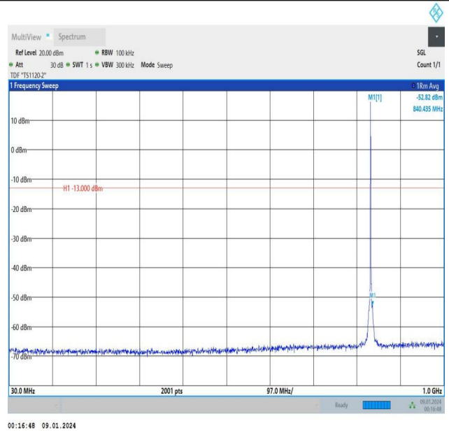
Band5_1.4MHz_16QAM_20525_1RB#0_30~1000_30~1000
