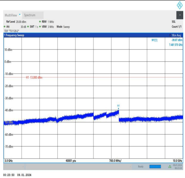
Band5_1.4MHz_16QAM_20643_6RB#0_3000~10000_3000~10000
