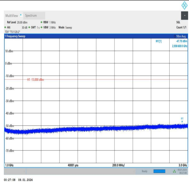
Band5_3MHz_QPSK_20415_15RB#0_1000~3000_1000~3000
