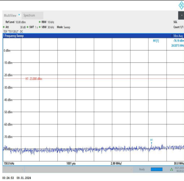
Band5_3MHz_16QAM_20415_1RB#0_0.15~30_0.15~30
