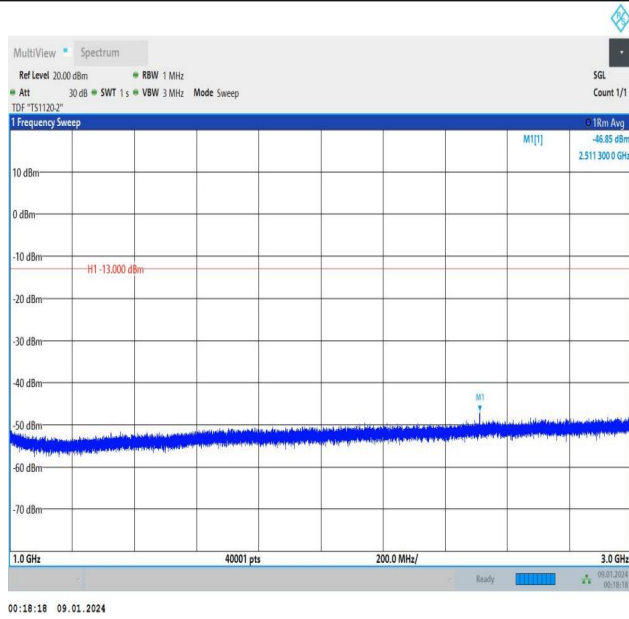
Band5_1.4MHz_16QAM_20525_1RB#5_1000~3000_1000~3000
