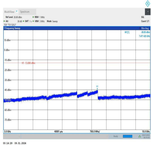
Band5_1.4MHz_16QAM_20407_1RB#5_3000~10000_3000~10000
