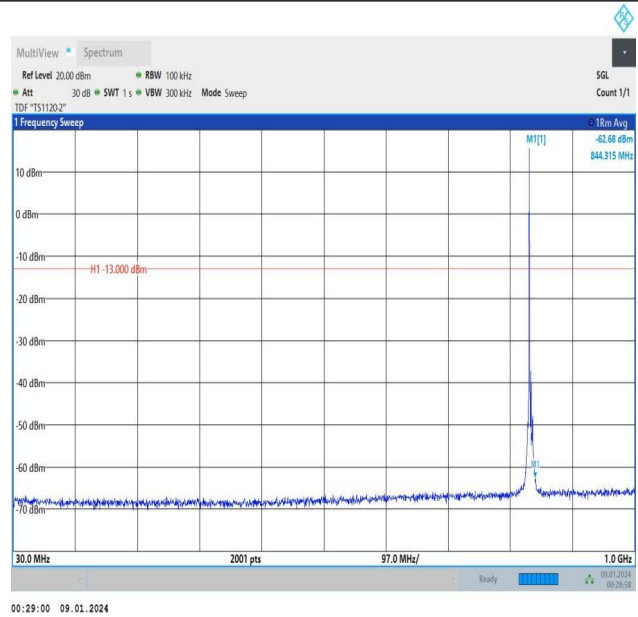
Band5_3MHz_16QAM_20525_1RB#0_30~1000_30~1000
