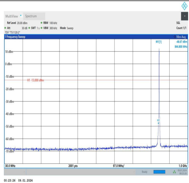
Band5_1.4MHz_16QAM_20643_6RB#0_30~1000_30~1000
