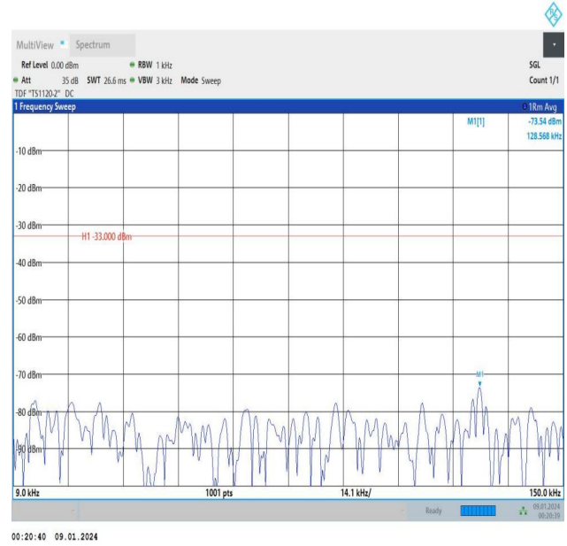
Band5_1.4MHz_16QAM_20643_1RB#0_0.009~0.15_0.009~0.15
