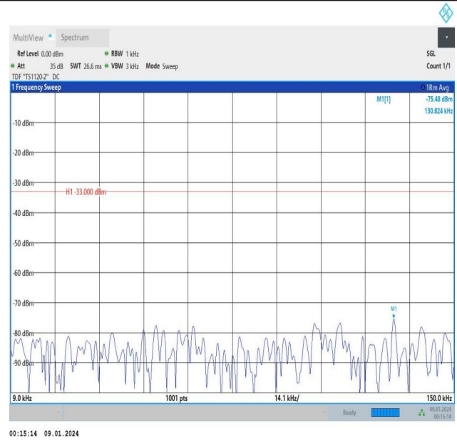
Band5_1.4MHz_16QAM_20407_6RB#0_0.009~0.15_0.009~0.15
