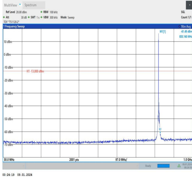
Band5_3MHz_QPSK_20415_1RB#0_30~1000_30~1000
