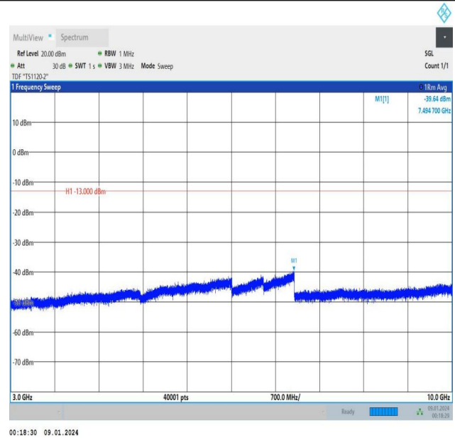
Band5_1.4MHz_16QAM_20525_1RB#5_3000~10000_3000~10000
