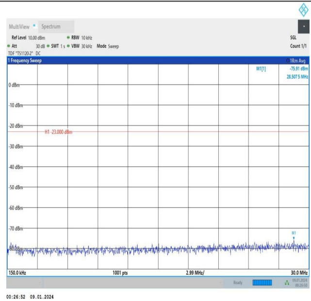
Band5_3MHz_QPSK_20415_15RB#0_0.15~30_0.15~30
