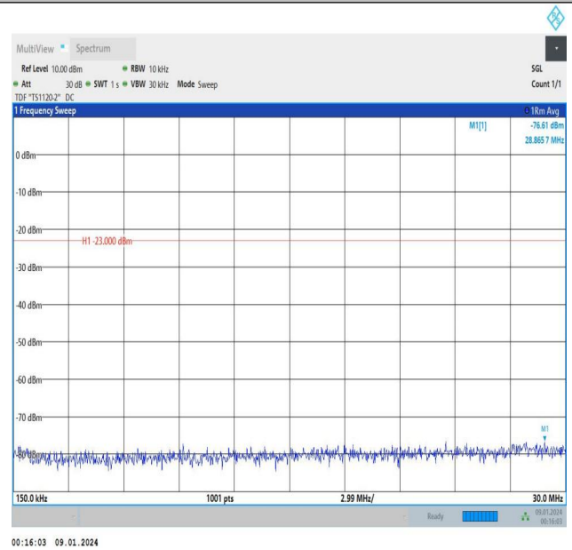
Band5_1.4MHz_QPSK_20525_1RB#0_0.15~30_0.15~30
