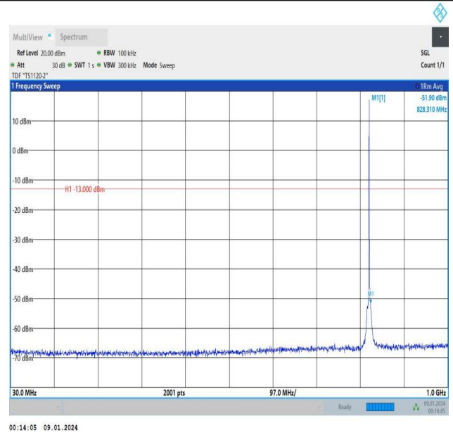
Band5_1.4MHz_16QAM_20407_1RB#5_30~1000_30~1000
