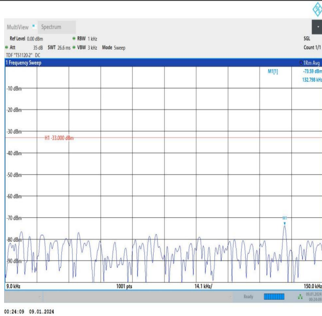
Band5_3MHz_QPSK_20415_1RB#0_0.009~0.15_0.009~0.15
