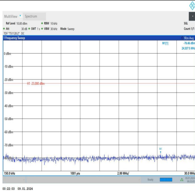
Band5_1.4MHz_16QAM_20643_1RB#5_0.15~30_0.15~30
