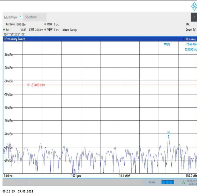
Band5_1.4MHz_QPSK_20525_1RB#0_0.009~0.15_0.009~0.15
