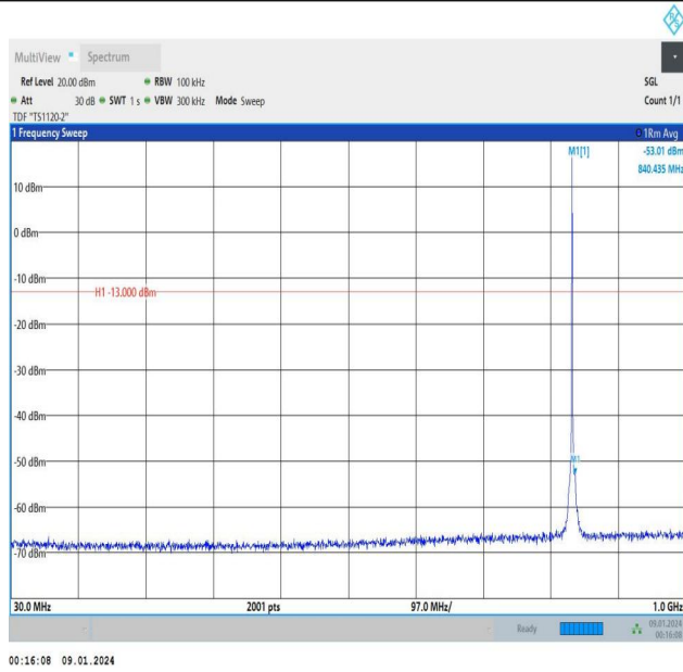
Band5_1.4MHz_QPSK_20525_1RB#0_30~1000_30~1000
