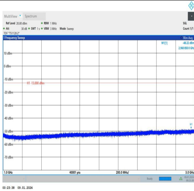
Band5_1.4MHz_16QAM_20643_6RB#0_1000~3000_1000~3000
