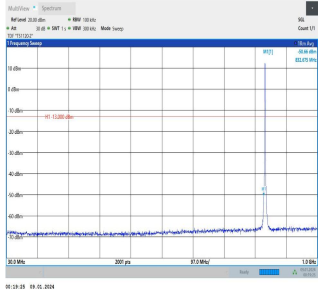
Band5_1.4MHz_16QAM_20525_6RB#0_30~1000_30~1000
