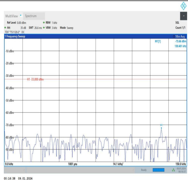
Band5_1.4MHz_16QAM_20525_1RB#0_0.009~0.15_0.009~0. 15
