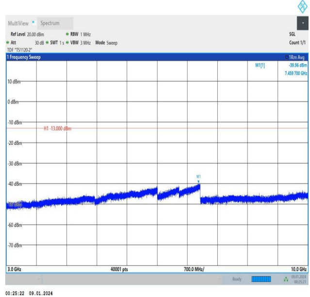
Band5_3MHz_16QAM_20415_1RB#0_3000~10000_3000~100
