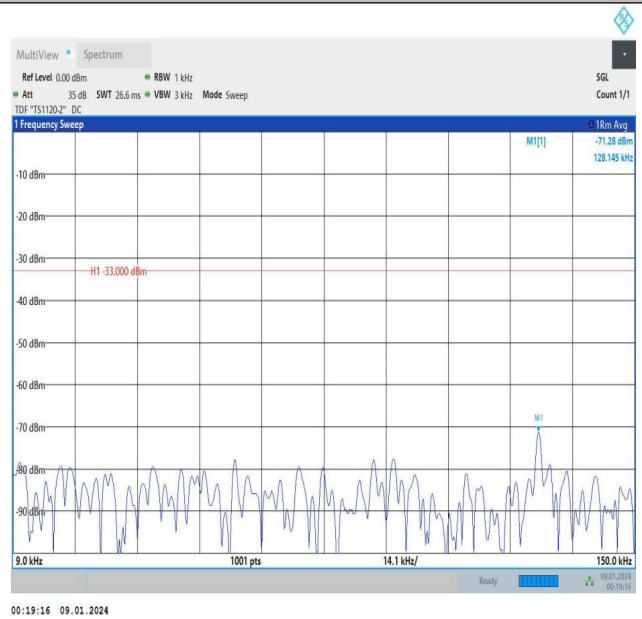
Band5_1.4MHz_16QAM_20525_6RB#0_0.009~0.15_0.009~0. 15
