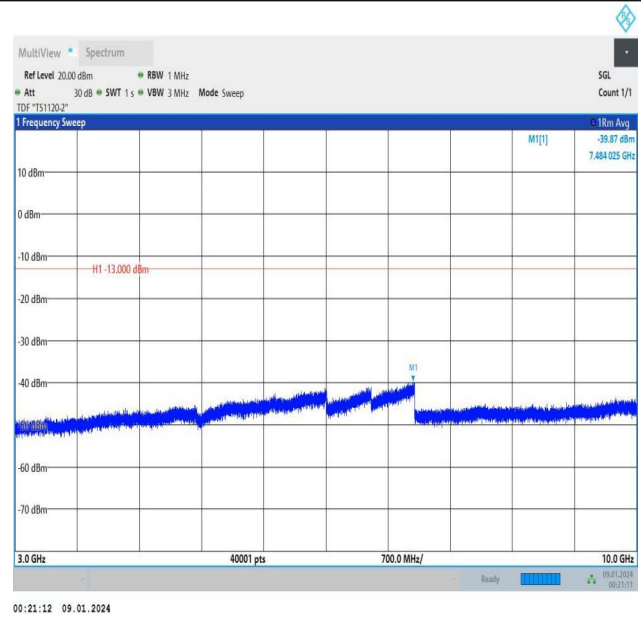
Band5_1.4MHz_16QAM_20643_1RB#0_3000~10000_3000~10000
