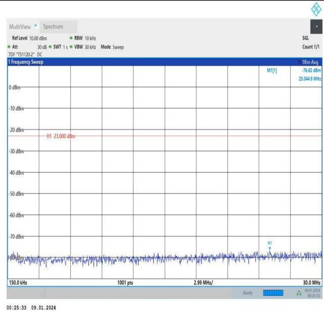
Band5_3MHz_QPSK_20415_1RB#14_0.15~30_0.15~30
