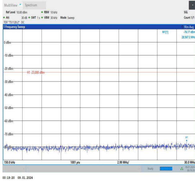
Band5_1.4MHz_16QAM_20525_6RB#0_0.15~30_0.15~30
