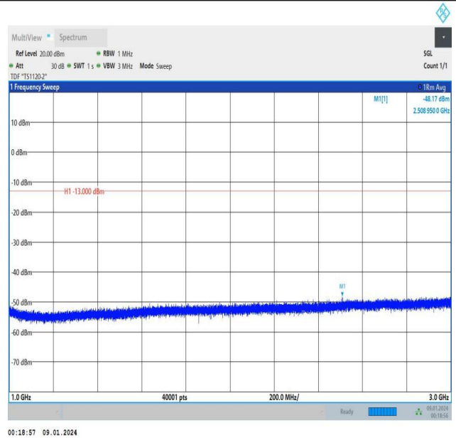
Band5_1.4MHz_QPSK_20525_6RB#0_1000~3000_1000~300 0
