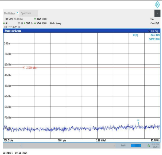
Band5_3MHz_QPSK_20415_1RB#0_0.15~30_0.15~30
