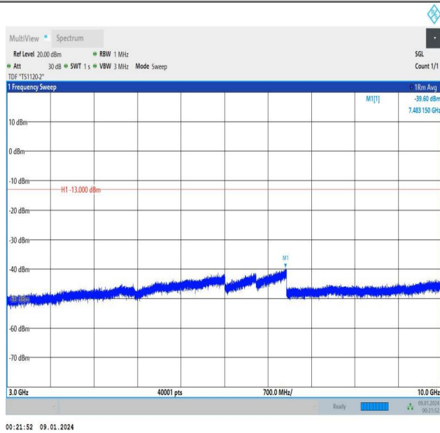
Band5_1.4MHz_QPSK_20643_1RB#5_3000~10000_3000~1
