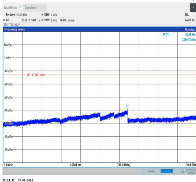
Band5_3MHz_QPSK_20415_1RB#0_3000~10000_3000~10000 00
