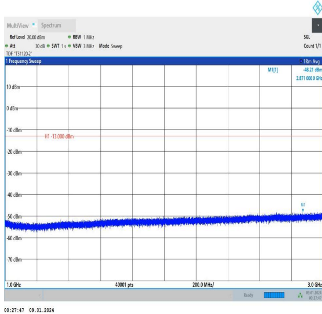
Band5_3MHz_16QAM_20415_15RB#0_1000~3000_1000~30 00
