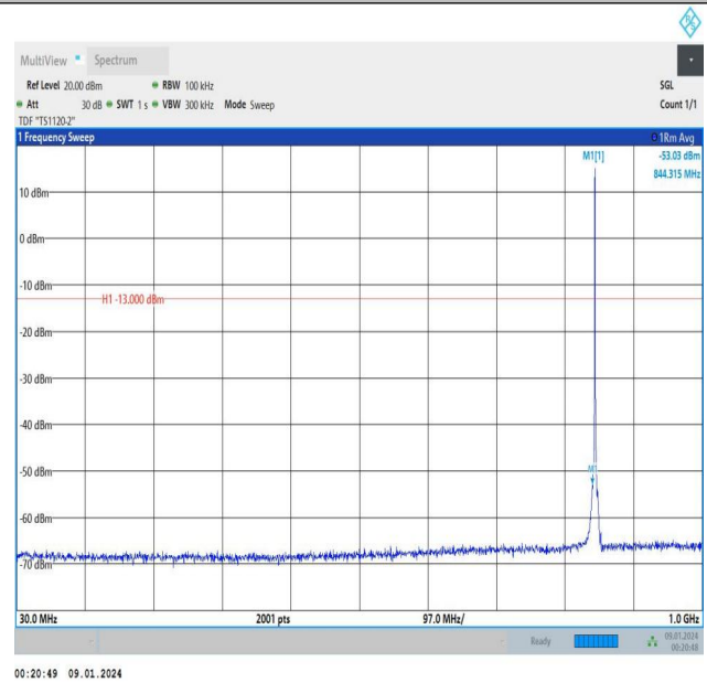
Band5_1.4MHz_16QAM_20643_1RB#0_30~1000_30~1000
