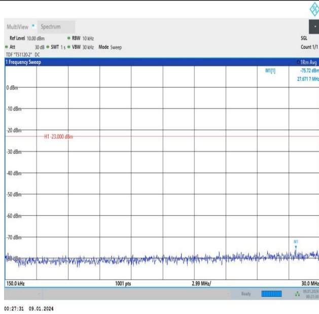
Band5_3MHz_16QAM_20415_15RB#0_0.15~30_0.15~30
