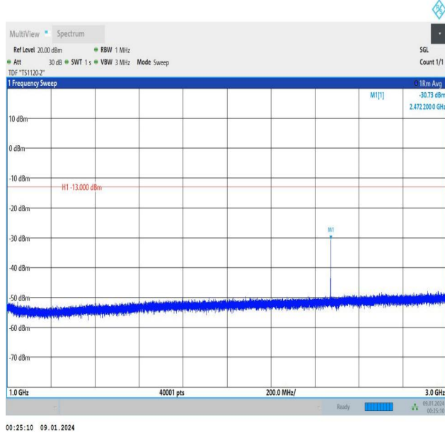
Band5_3MHz_16QAM_20415_1RB#0_1000~3000_1000~300
