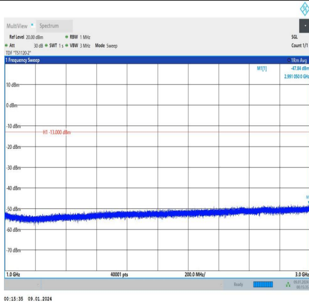
Band5_1.4MHz_16QAM_20407_6RB#0_1000~3000_1000~3000
