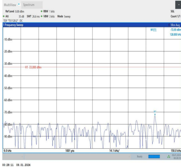
Band5_3MHz_QPSK_20525_1RB#0_0.009~0.15_0.009~0.15
