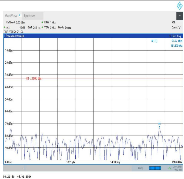
Band5_1.4MHz_16QAM_20643_1RB#5_0.009~0.15_0.009~0.
