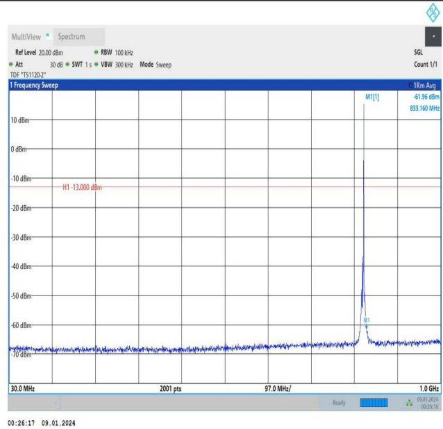
Band5_3MHz_16QAM_20415_1RB#14_30~1000_30~1000
