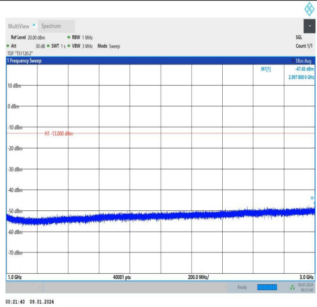
Band5_1.4MHz_QPSK_20643_1RB#5_1000~3000_1000~300
