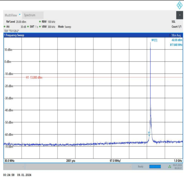
Band5_3MHz_16QAM_20415_1RB#0_30~1000_30~1000
