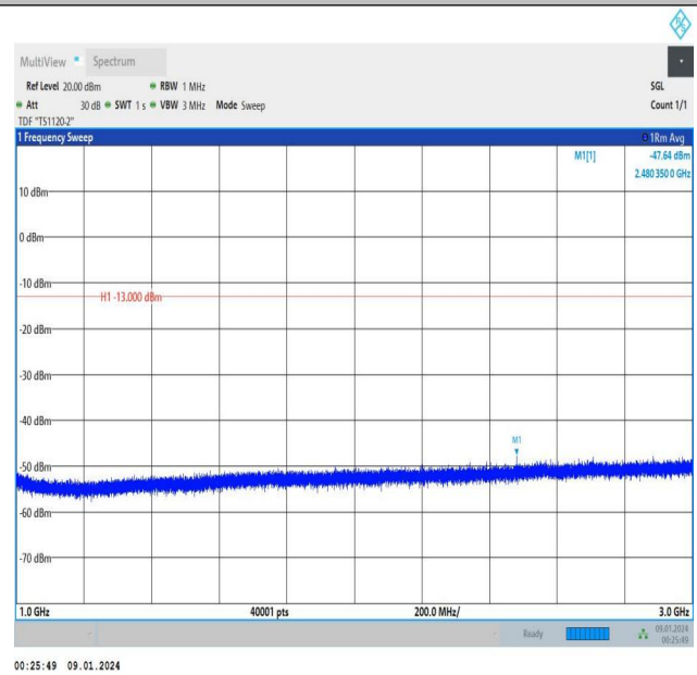
Band5_3MHz_QPSK_20415_1RB#14_1000~3000_1000~3000
