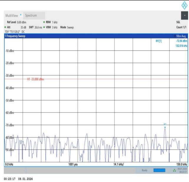
Band5_1.4MHz_16QAM_20643_6RB#0_0.009~0.15_0.009~0.15
