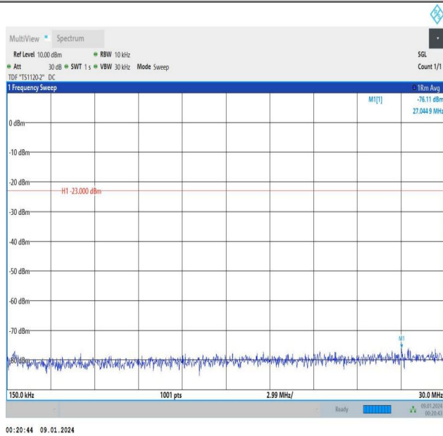
Band5_1.4MHz_16QAM_20643_1RB#0_0.15~30_0.15~30
