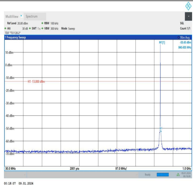
Band5_1.4MHz_16QAM_20525_1RB#5_30~1000_30~1000
