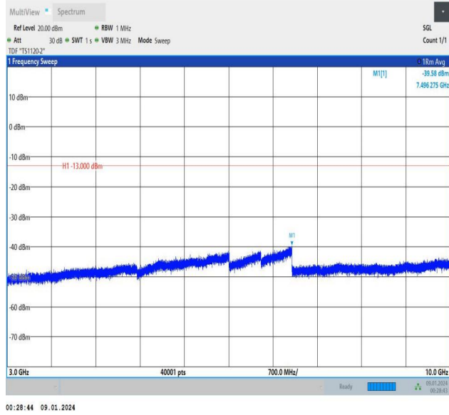
Band5_3MHz_QPSK_20525_1RB#0_3000~10000_3000~10000
