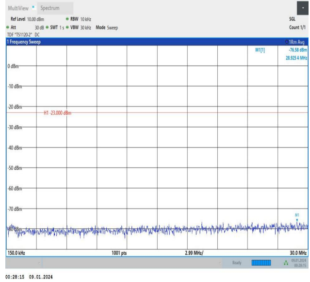
Band5_3MHz_QPSK_20525_1RB#0_0.15~30_0.15~30
