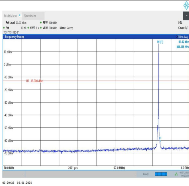
Band5_3MHz_QPSK_20525_1RB#14_30~1000_30~1000
