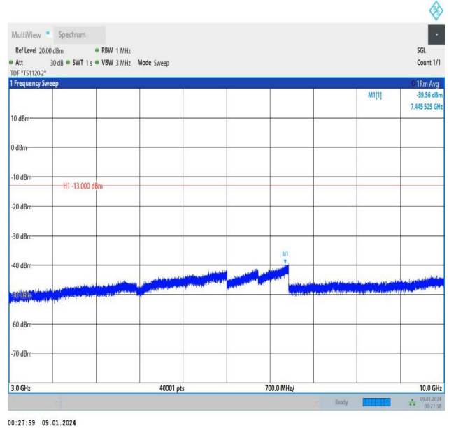
Band5_3MHz_16QAM_20415_15RB#0_3000~10000_3000~10 000
