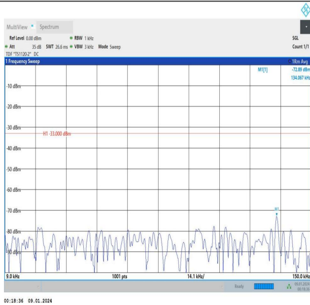
Band5_1.4MHz_QPSK_20525_6RB#0_0.009~0.15_0.009~0.15
