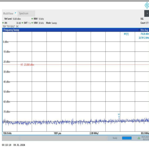
Band5_1.4MHz_16QAM_20407_6RB#0_0.15~30_0.15~30
