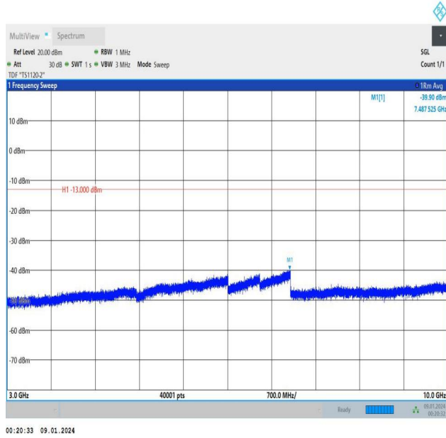
Band5_1.4MHz_QPSK_20643_1RB#0_3000~10000_3000~10000
