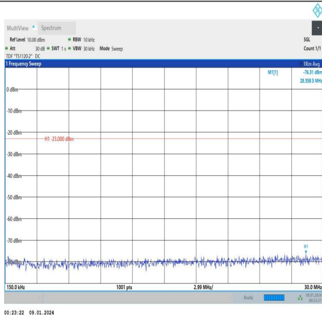
Band5_1.4MHz_16QAM_20643_6RB#0_0.15~30_0.15~30
