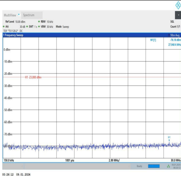
Band5_3MHz_16QAM_20415_1RB#14_0.15~30_0.15~30
