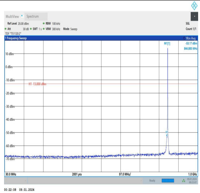
Band5_1.4MHz_16QAM_20643_1RB#5_30~1000_30~1000
