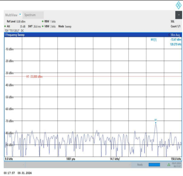
Band5_1.4MHz_16QAM_20525_1RB#5_0.009~0.15_0.009~0.15
