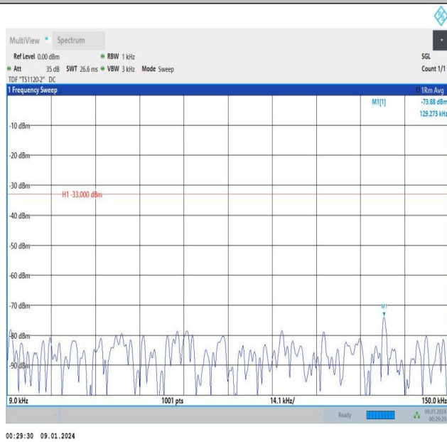
Band5_3MHz_QPSK_20525_1RB#14_0.009~0.15_0.009~0.1
