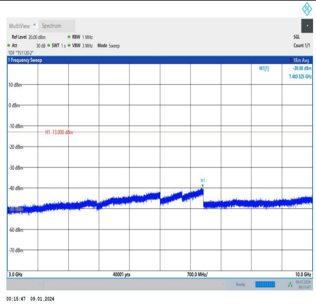
Band5_1.4MHz_16QAM_20407_6RB#0_3000~10000_3000~10000
