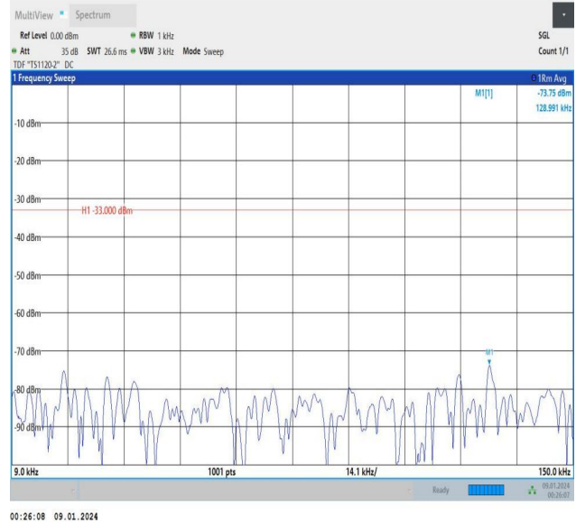
Band5_3MHz_16QAM_20415_1RB#14_0.009~0.15_0.009~0.15
