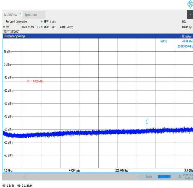
Band5_1.4MHz_16QAM_20525_1RB#0_1000~3000_1000~3000
