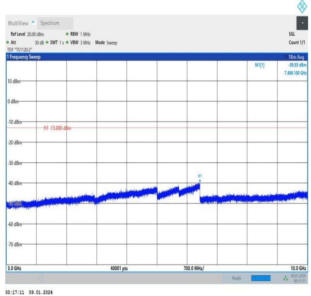
Band5_1.4MHz_16QAM_20525_1RB#0_3000~10000_3000~10000
