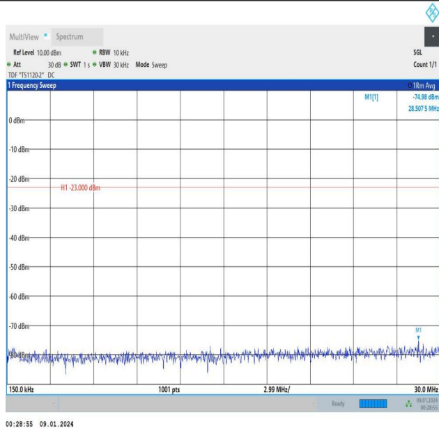
Band5_3MHz_16QAM_20525_1RB#0_0.15~30_0.15~30
