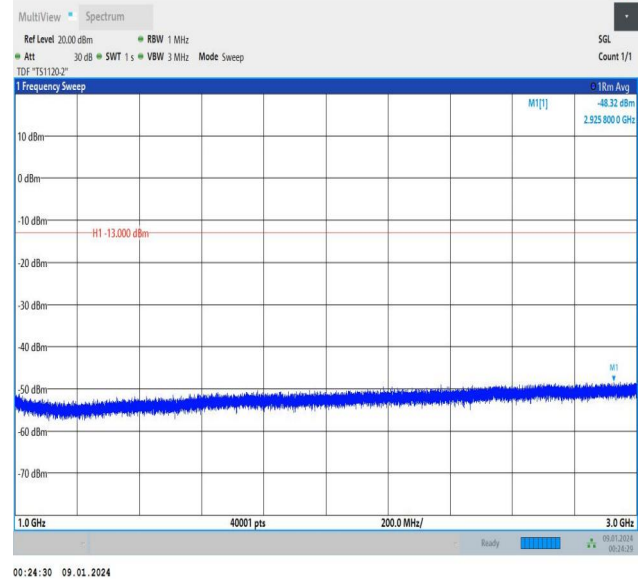
Band5_3MHz_QPSK_20415_1RB#0_1000~3000_1000~3000
