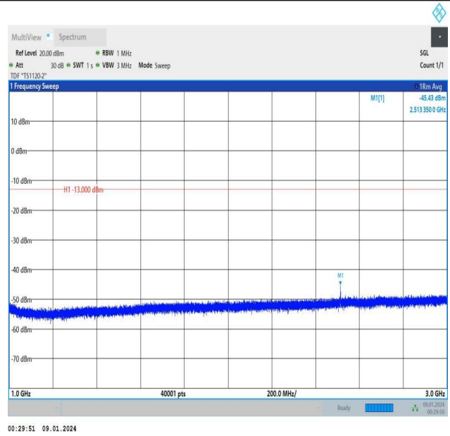
Band5_3MHz_QPSK_20525_1RB#14_1000~3000_1000~3000
