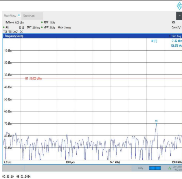
Band5_1.4MHz_QPSK_20643_1RB#5_0.009~0.15_0.009~0.15
