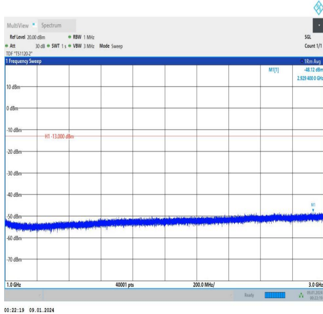
Band5_1.4MHz_16QAM_20643_1RB#5_1000~3000_1000~3000
