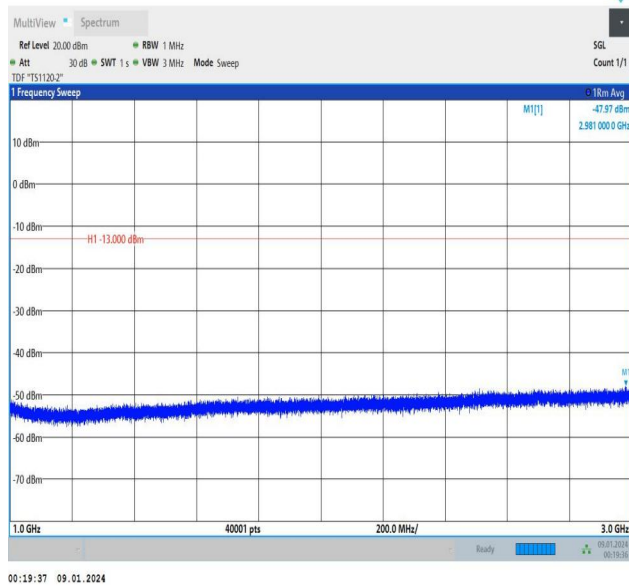
Band5_1.4MHz_16QAM_20525_6RB#0_1000~3000_1000~3000
