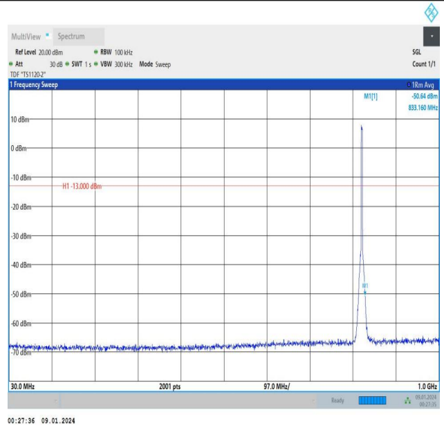
Band5_3MHz_16QAM_20415_15RB#0_30~1000_30~1000
