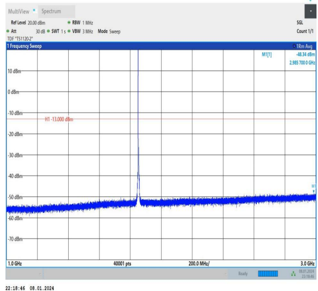
Band2_5MHz_QPSK_18625_1RB#0_1000~3000_1000~3000
