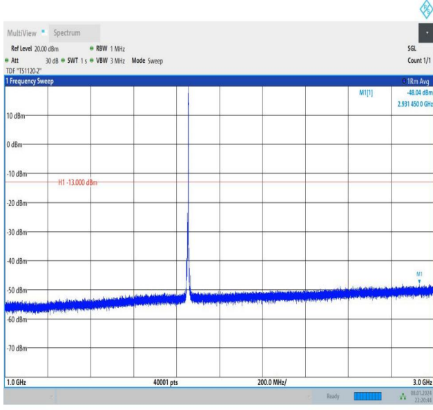
Band2_5MHz_16QAM_18625_1RB#24_1000~3000_1000~30 00
