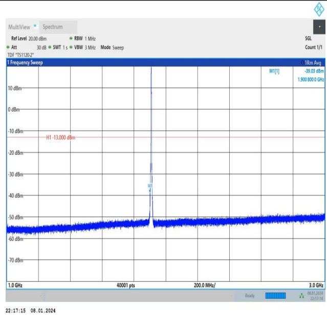
Band2_3MHz_QPSK_19185_15RB#0_1000~3000_1000~300 0
