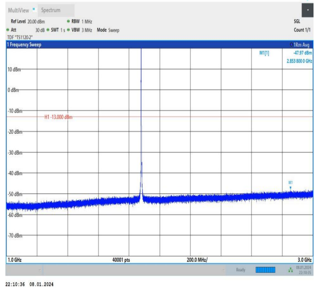
Band2_3MHz_QPSK_18900_1RB#0_1000~3000_1000~3000
