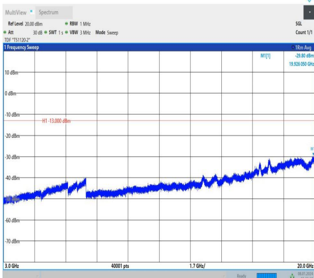
Band2_5MHz_QPSK_18900_1RB#0_3000~20000_3000~20000
