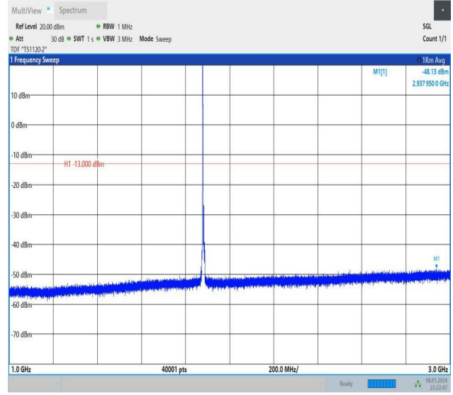
Band2_5MHz_QPSK_18900_1RB#0_1000~3000_1000~3000
