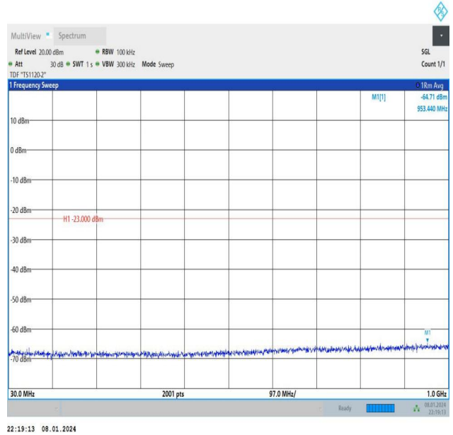
Band2_5MHz_16QAM_18625_1RB#0_30~1000_30~1000
