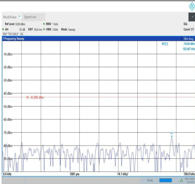
Band2_3MHz_16QAM_19185_1RB#14_1000~3000_1000~30 00
