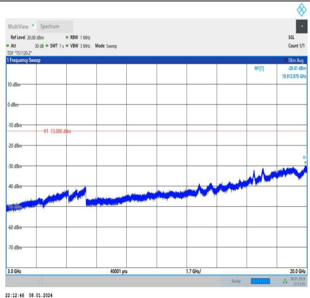
Band2_3MHz_16QAM_18900_1RB#14_3000~20000_3000~2 0000
