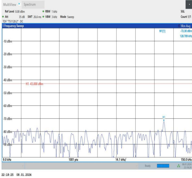
Band2_5MHz_QPSK_18625_1RB#0_0.009~0.15_0.009~0.15
