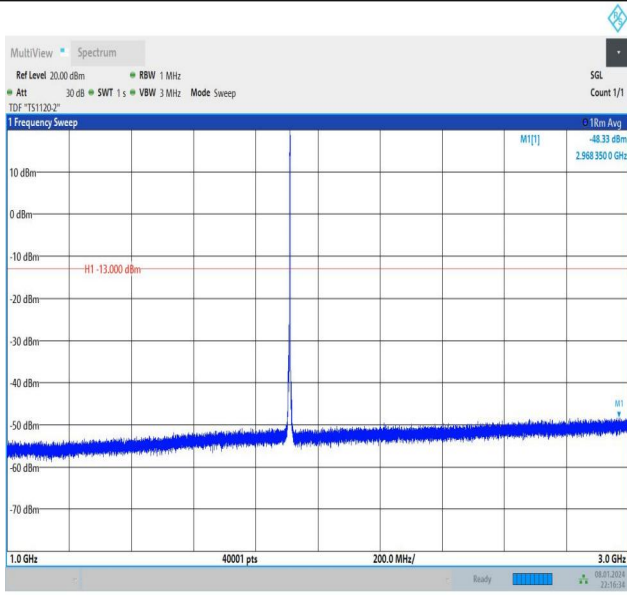
Band2_3MHz_16QAM_19185_1RB#14_1000~3000_1000~30 00
