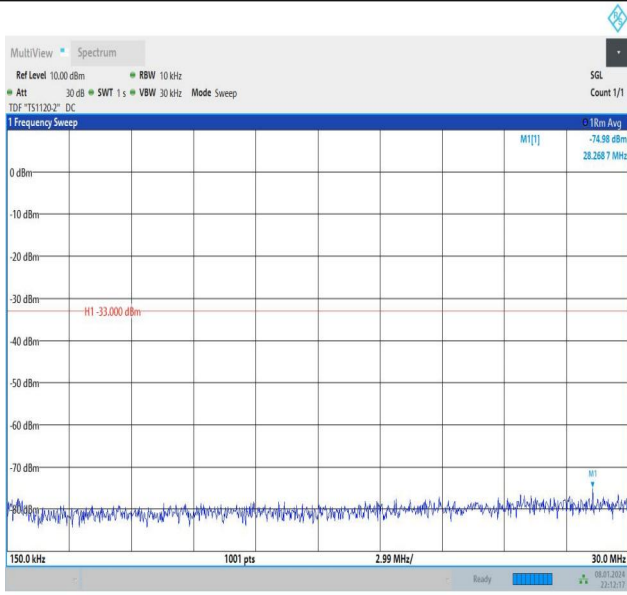
Band2_3MHz_16QAM_18900_1RB#14_0.15~30_0.15~30
