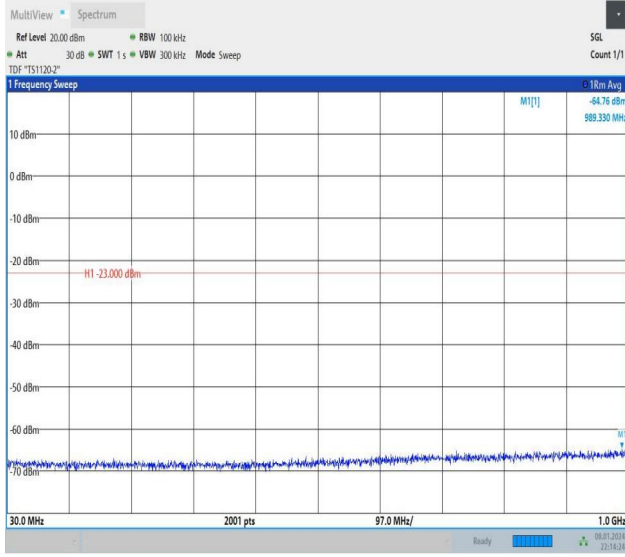
Band2_3MHz_QPSK_19185_1RB#0_30~1000_30~1000
