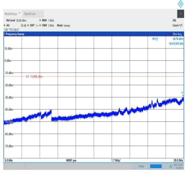
Band2_5MHz_16QAM_18625_1RB#24_3000~20000_3000~2 0000
