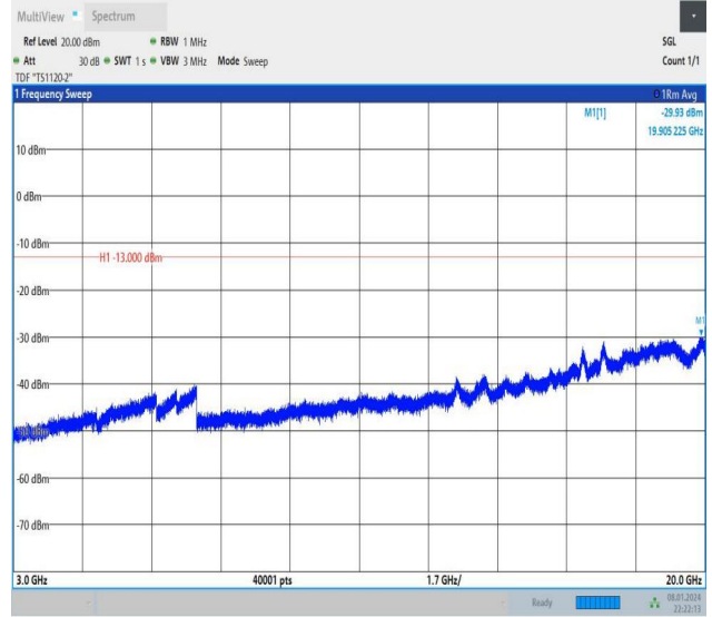
Band2_5MHz_16QAM_18625_25RB#0_3000~20000_3000~2
