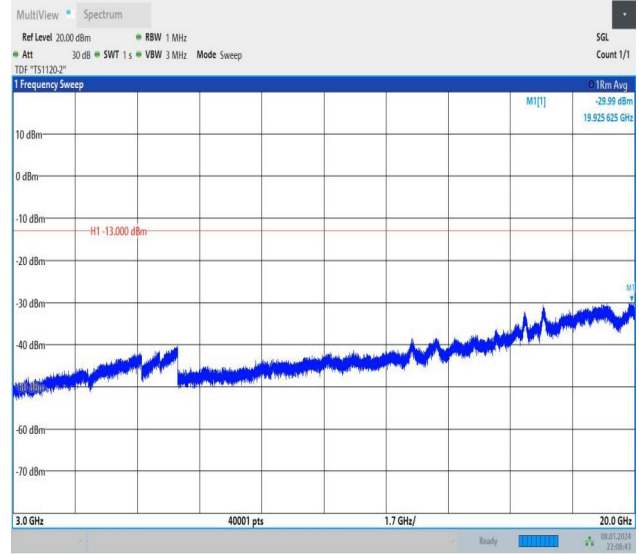
Band2_3MHz_16QAM_18615_1RB#14_3000~20000_3000~2 0000
