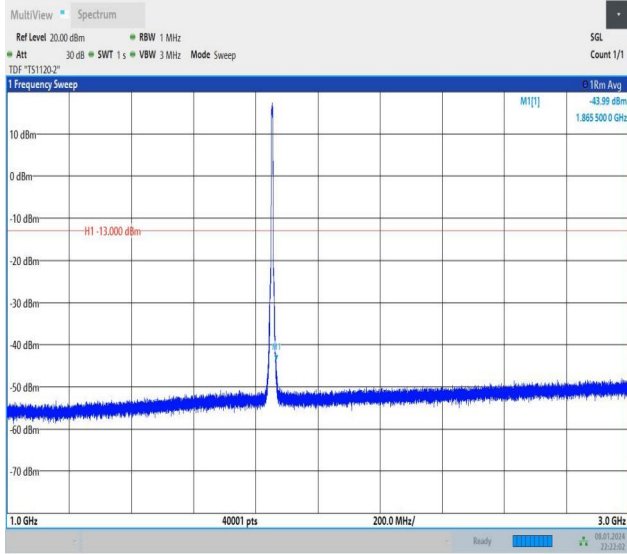
Band2_5MHz_16QAM_18625_25RB#0_1000~3000_1000~30
