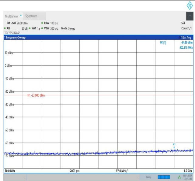
Band2_3MHz_16QAM_19185_15RB#0_30~1000_30~1000
