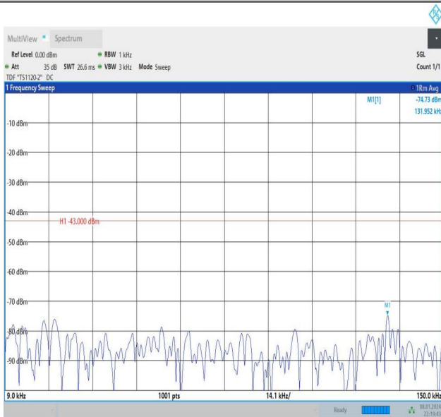
Band2_5MHz_QPSK_18625_1RB#24_0.009~0.15_0.009~0.1
