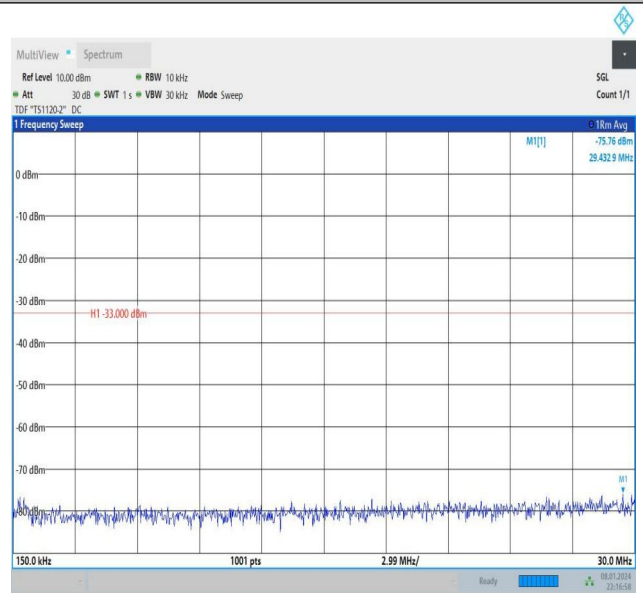
Band2_3MHz_16QAM_19185_1RB#14_3000~20000_3000~2 0000
