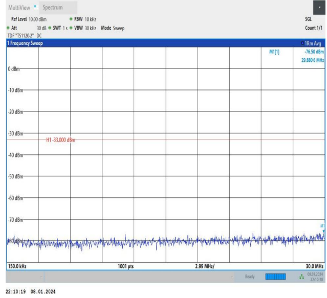
Band2_3MHz_QPSK_18900_1RB#0_0.15~30_0.15~30
