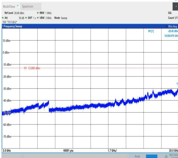
Band2_3MHz_QPSK_19185_1RB#0_3000~20000_3000~2000 00
