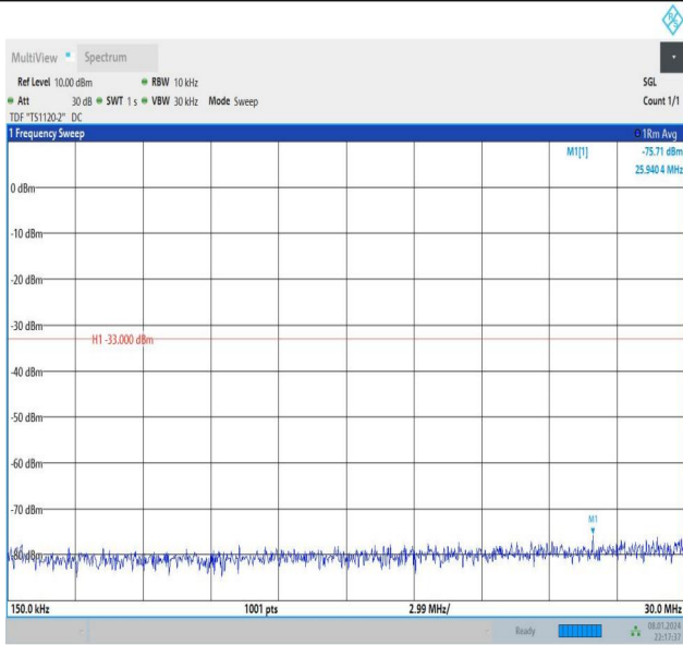
Band2_3MHz_16QAM_19185_15RB#0_0.15~30_0.15~30
