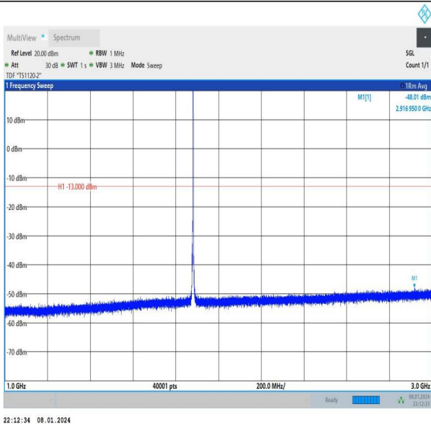
Band2_3MHz_16QAM_18900_1RB#14_1000~3000_1000~30 00
