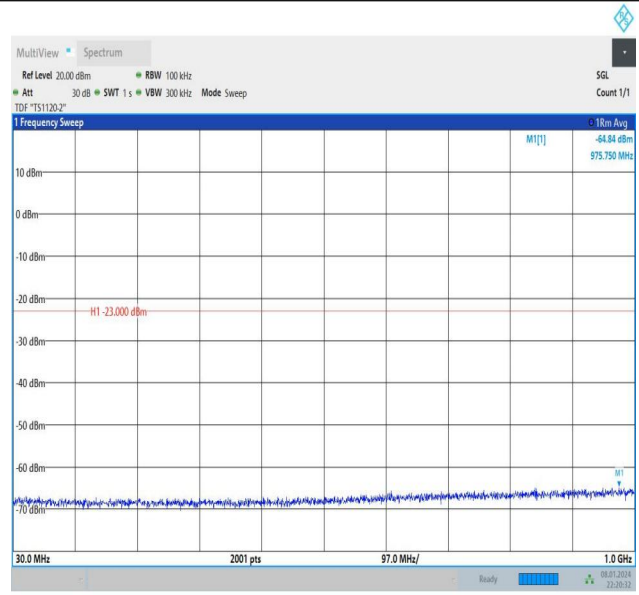
Band2_5MHz_16QAM_18625_1RB#24_30~1000_30~1000
