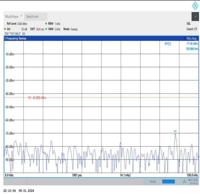
Band2_3MHz_16QAM_18900_1RB#0_0.009~0.15_0.009~0.15
