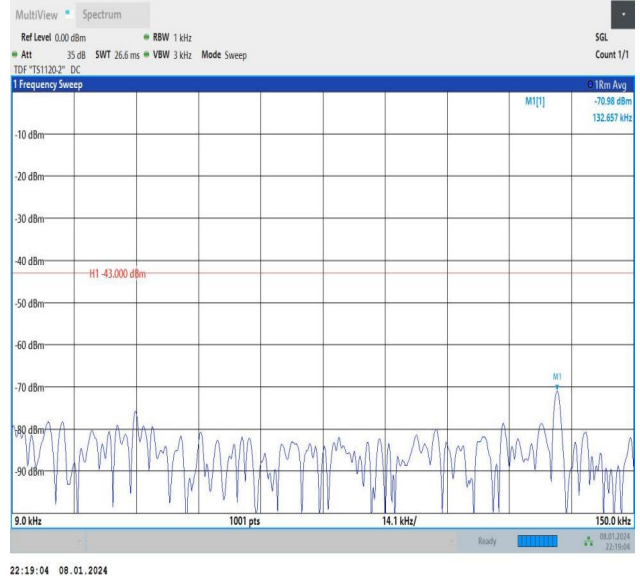
Band2_5MHz_16QAM_18625_1RB#0_0.009~0.15_0.009~0.15 5
