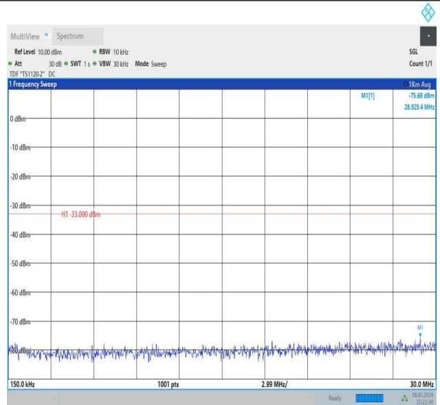
Band2_5MHz_QPSK_18900_1RB#0_0.15~30_0.15~30
