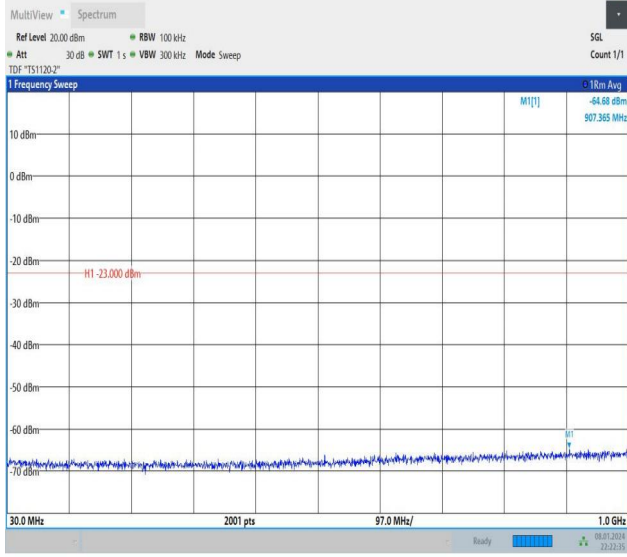
Band2_5MHz_QPSK_18900_1RB#0_30~1000_30~1000
