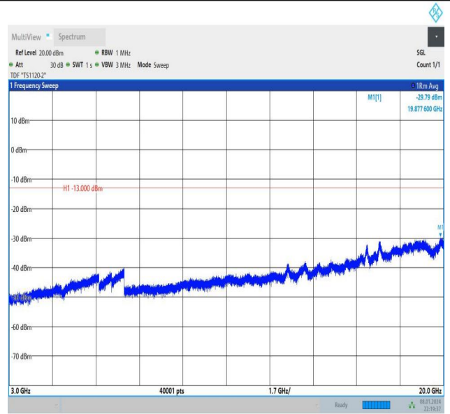
Band2_5MHz_16QAM_18625_1RB#0_3000~20000_3000~20000
