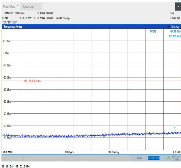
Band2_5MHz_QPSK_18625_1RB#0_30~1000_30~1000
