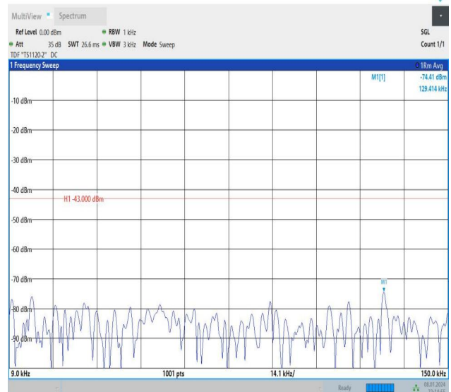
Band2_3MHz_16QAM_19185_1RB#0_0.009~0.15_0.009~0.1 5
