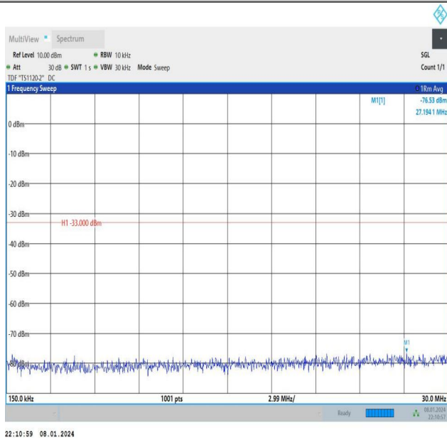
Band2_3MHz_16QAM_18900_1RB#0_0.15~30_0.15~30
