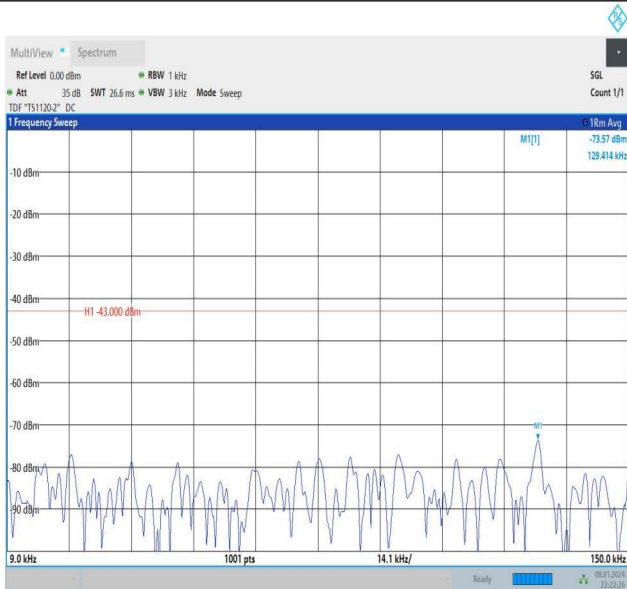
Band2_5MHz_QPSK_18900_1RB#0_0.009~0.15_0.009~0.15
