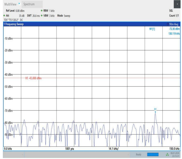
Band2_3MHz_16QAM_18900_15RB#0_0.009~0.15_0.009~0.15
