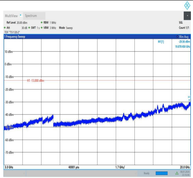
Band2_3MHz_16QAM_19185_1RB#14_3000~20000_3000~2 0000
