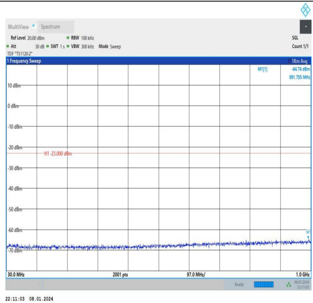
Band2_3MHz_16QAM_18900_1RB#0_30~1000_30~1000
