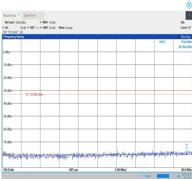
Band2_3MHz_QPSK_18900_15RB#0_3000~20000_3000~20000
