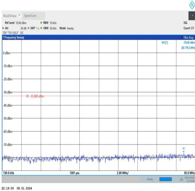
Band2_5MHz_16QAM_18625_1RB#0_0.15~30_0.15~30
