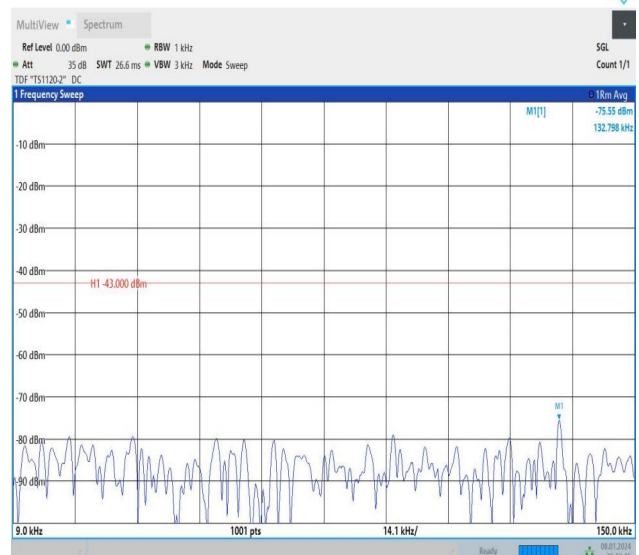
Band2_5MHz_16QAM_18900_1RB#0_0.009~0.15_0.009~0.1
