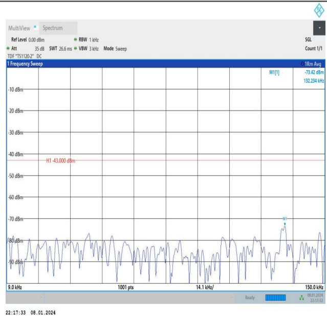
Band2_3MHz_16QAM_19185_15RB#0_0.009~0.15_0.009~0. 15
