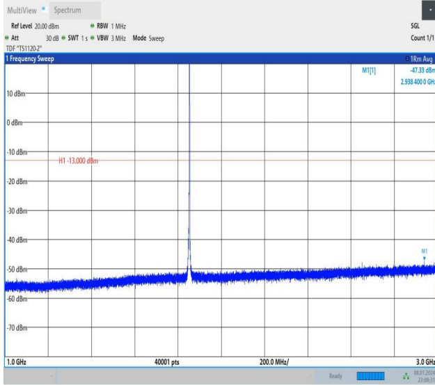
Band2_3MHz_16QAM_18615_1RB#14_1000~3000_1000~30 00
