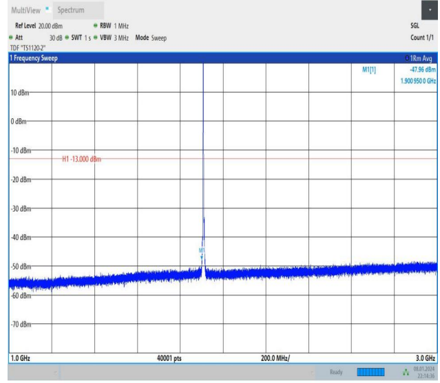
Band2_3MHz_QPSK_19185_1RB#0_1000~3000_1000~3000
