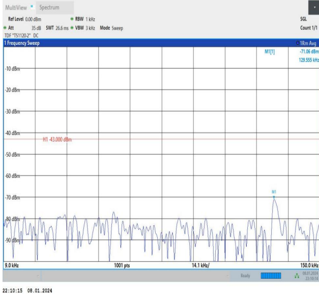
Band2_3MHz_QPSK_18900_1RB#0_0.009~0.15_0.009~0.15
