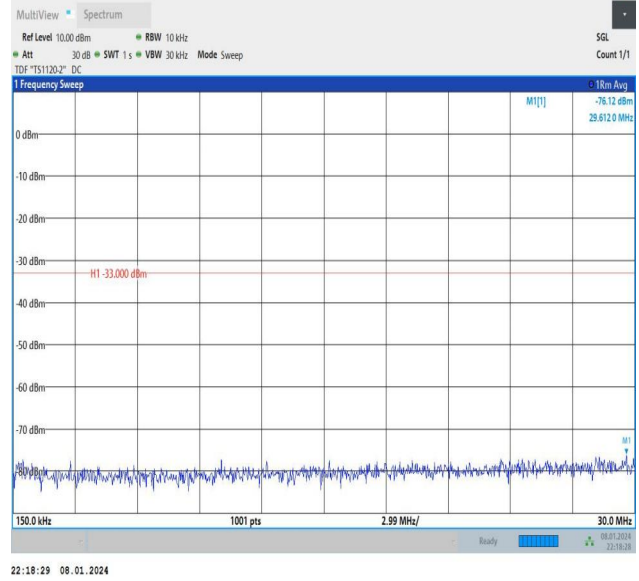
Band2_5MHz_QPSK_18625_1RB#0_0.15~30_0.15~30
