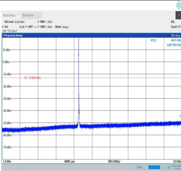
Band2_5MHz_16QAM_18625_1RB#0_1000~3000_1000~300
