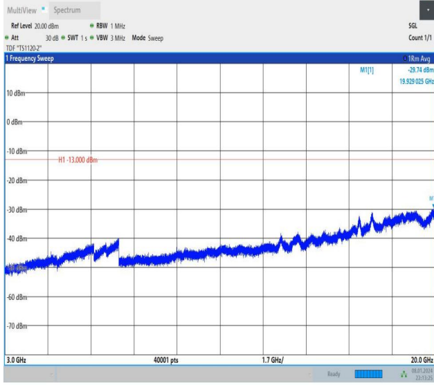
Band2_3MHz_QPSK_18900_15RB#0_3000~20000_3000~20000
