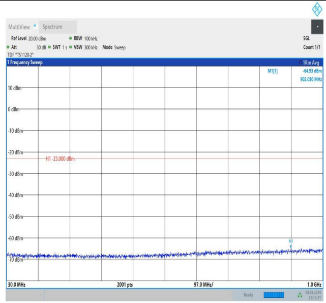
Band2_3MHz_16QAM_18900_1RB#14_30~1000_30~1000
