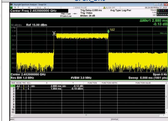
Pulse Width π/4DQPSK_2-DH5
