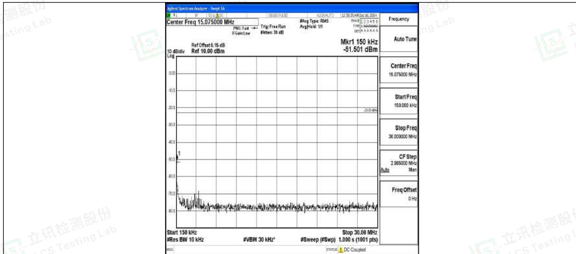
Band17_10MHz_QPSK_23780_1RB#0_0.15~30_0.15~30
