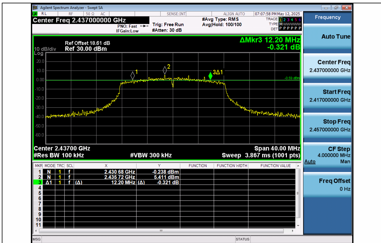
11G-Ant1-2437-PASS
