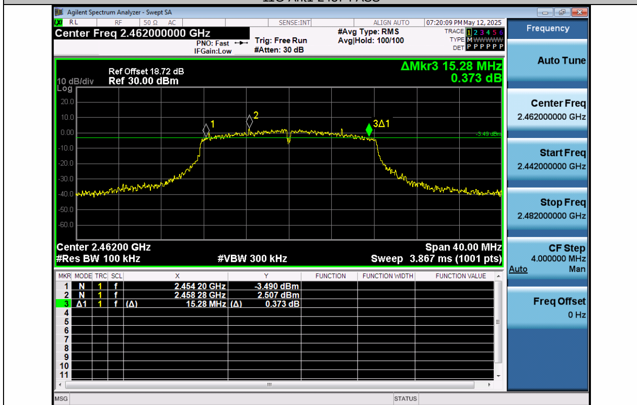
11G-Ant1-2462-PASS
