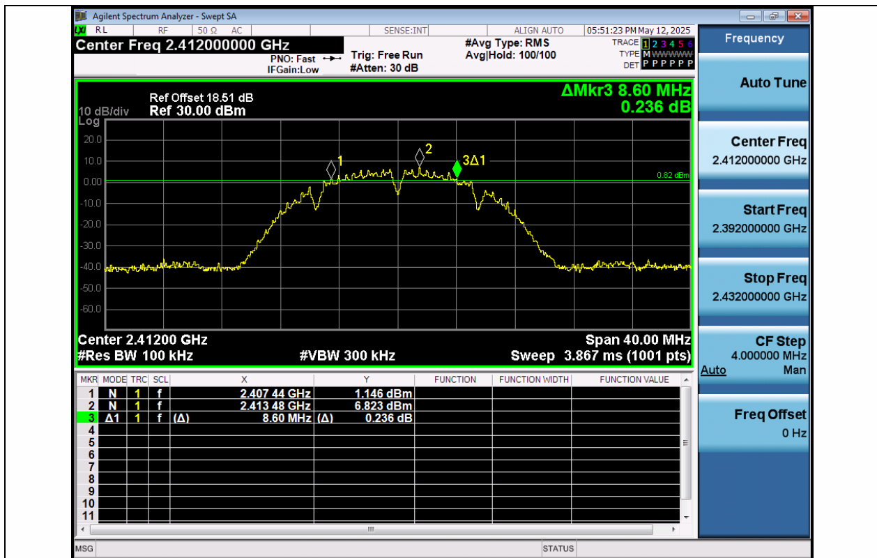
11B-Ant1-2412-PASS
