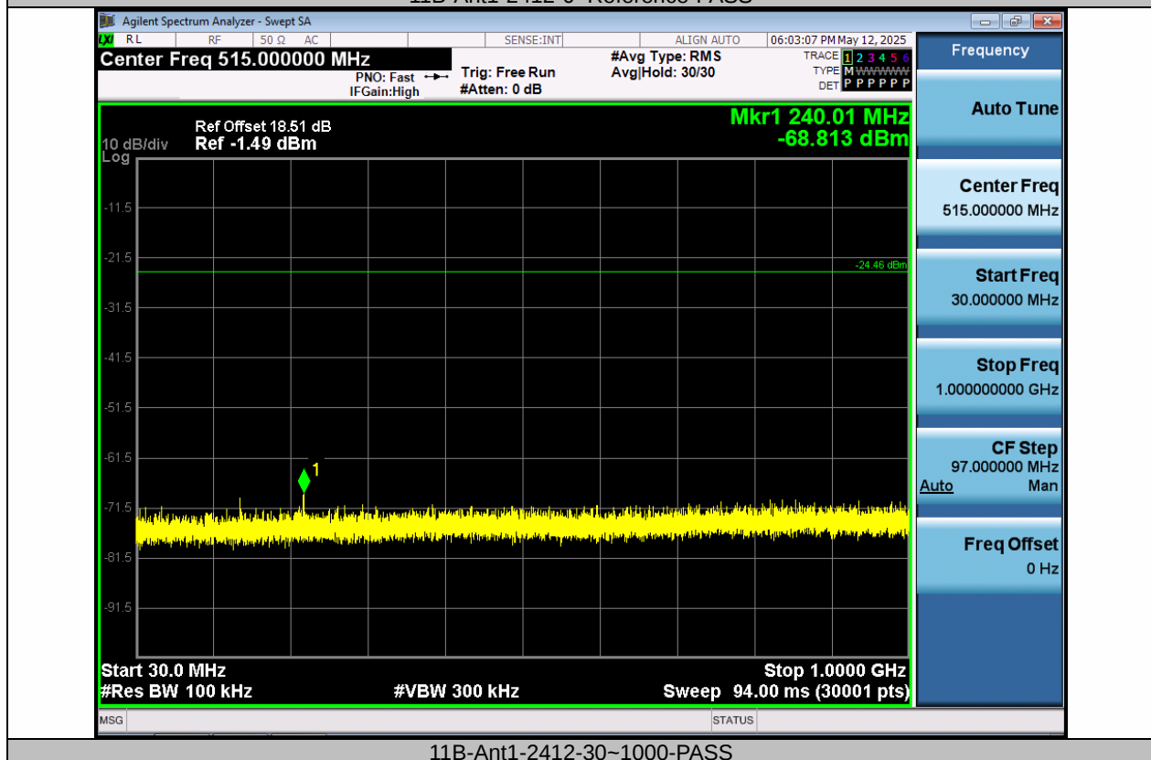
11B-Ant1-2412-30~1000-PASS
