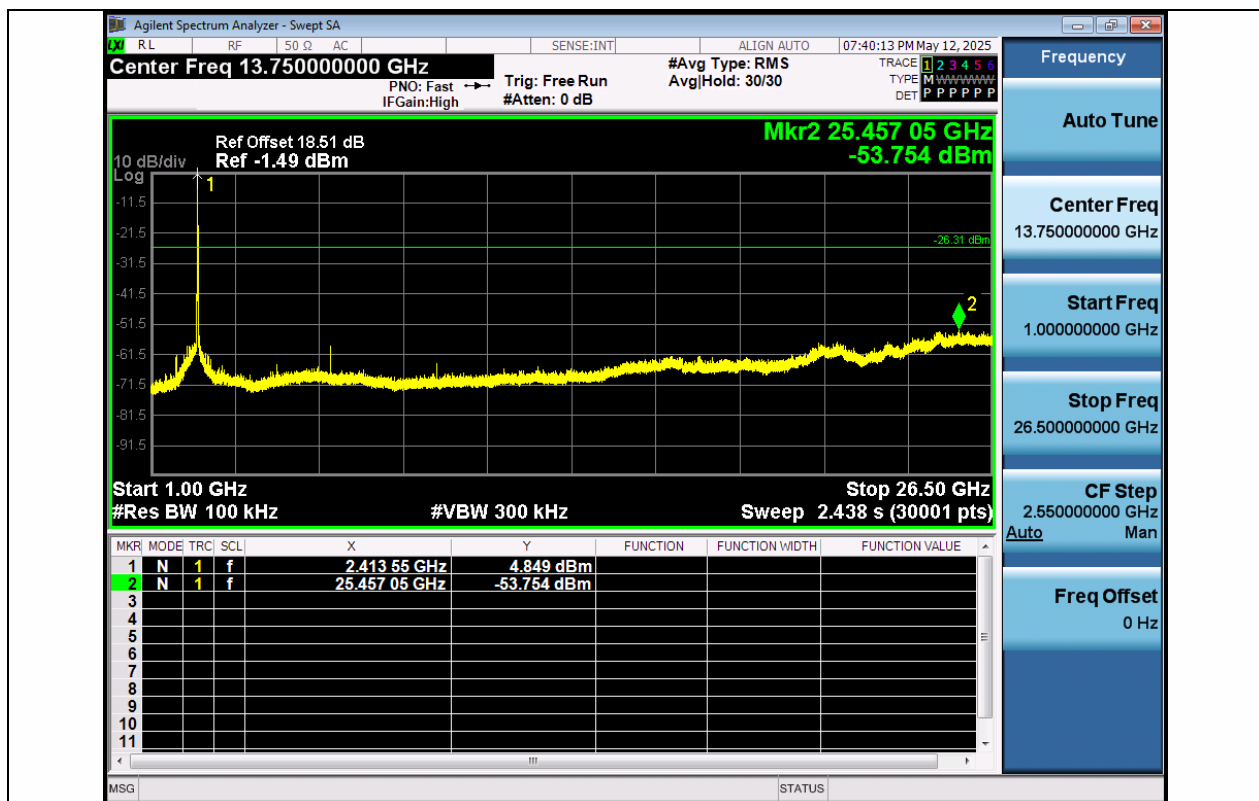
11N20SISO-Ant1-2412-1000~26500-PASS
