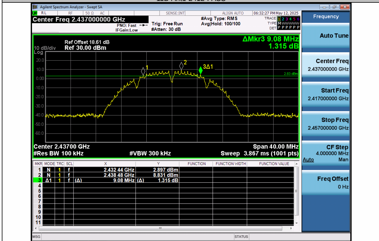
11B-Ant1-2437-PASS
