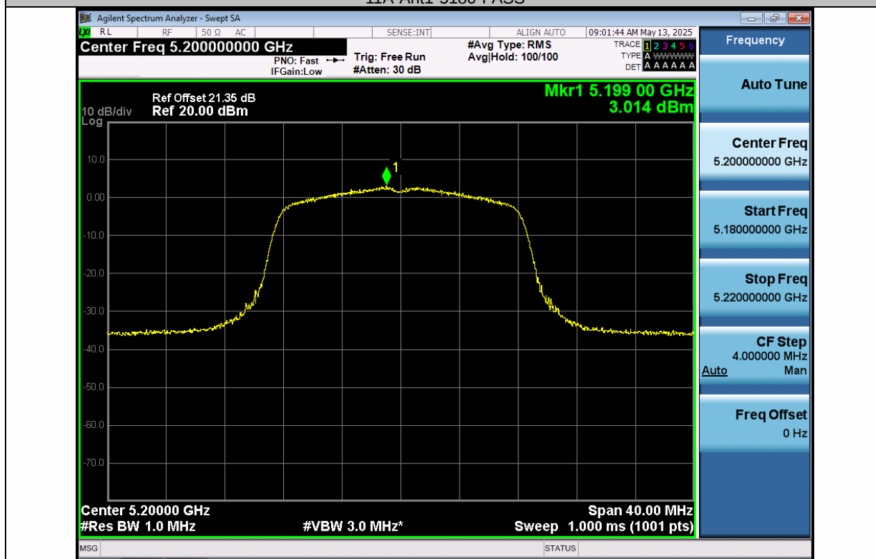
11A-Ant1-5200-PASS
