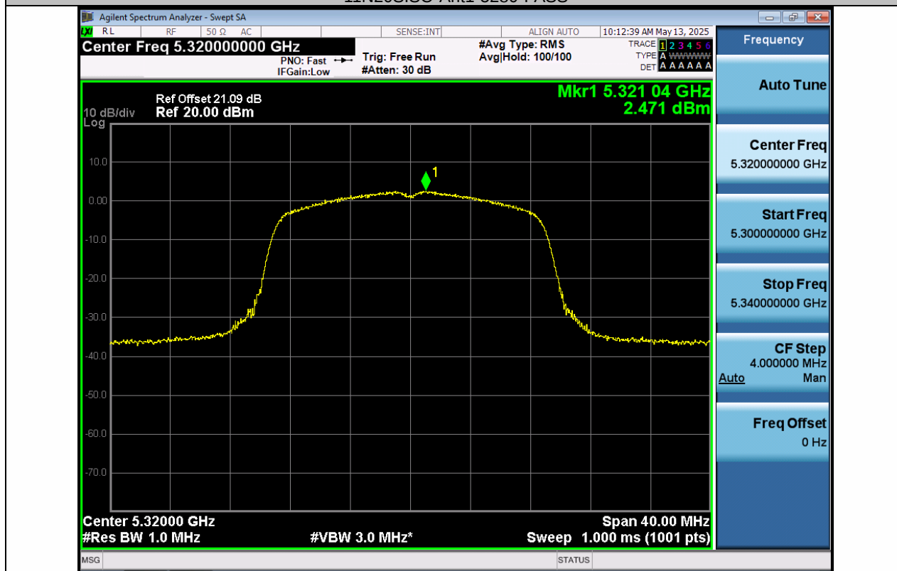
11N20SISO-Ant1-5320-PASS
