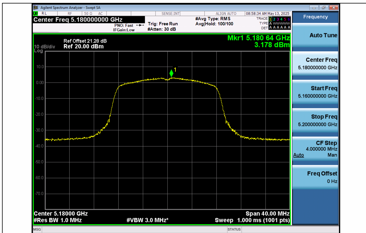
11A-Ant1-5180-PASS
