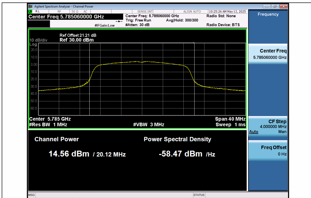
11N20SISO-Ant1-5785-PASS
