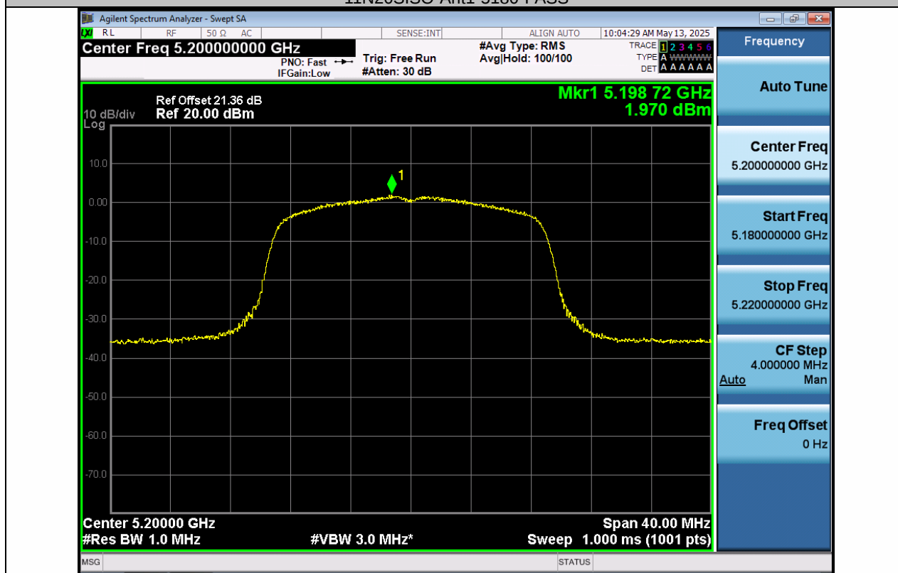
11N20SISO-Ant1-5200-PASS
