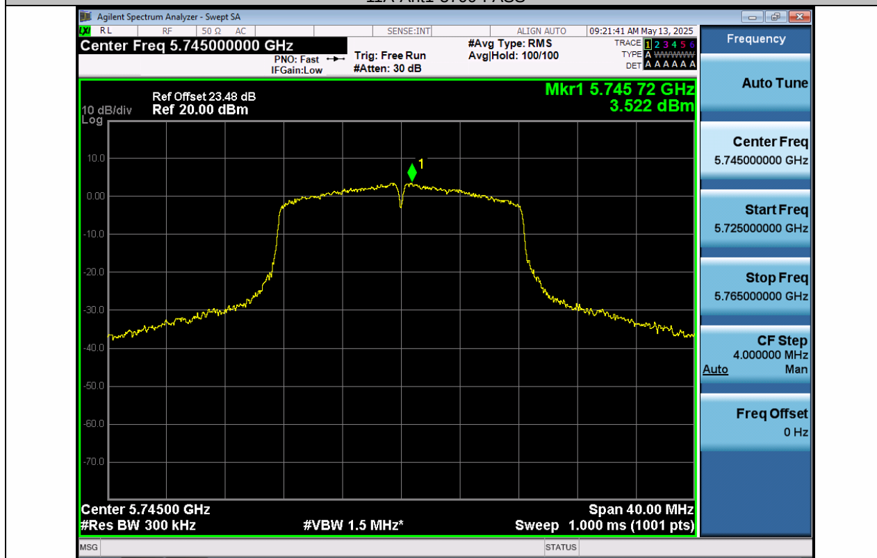
11A-Ant1-5745-PASS
