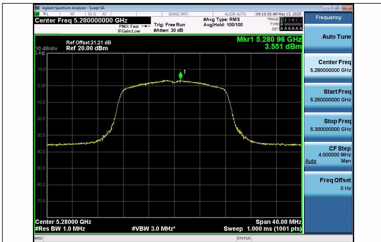
11A-Ant1-5280-PASS
