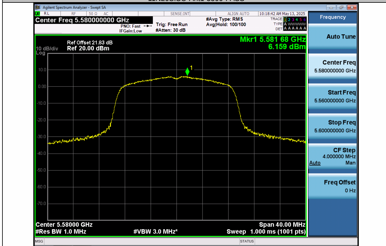
11N20SISO-Ant1-5580-PASS
