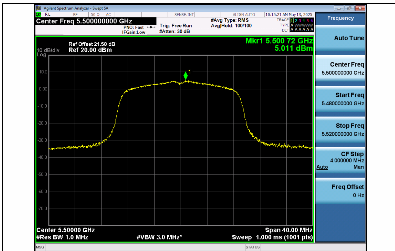
11N20SISO-Ant1-5500-PASS
