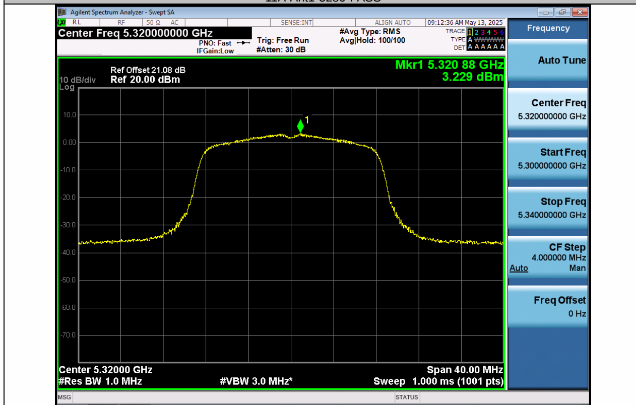
11A-Ant1-5320-PASS
