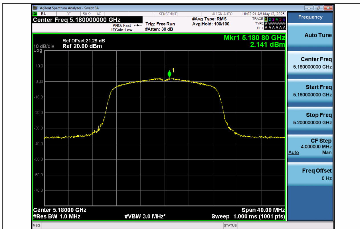
11N20SISO-Ant1-5180-PASS
