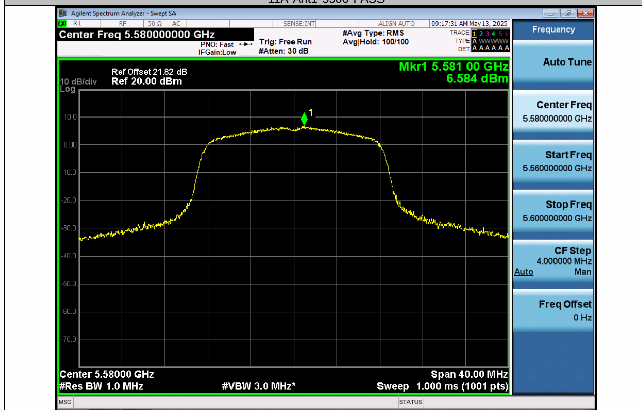
11A-Ant1-5580-PASS
