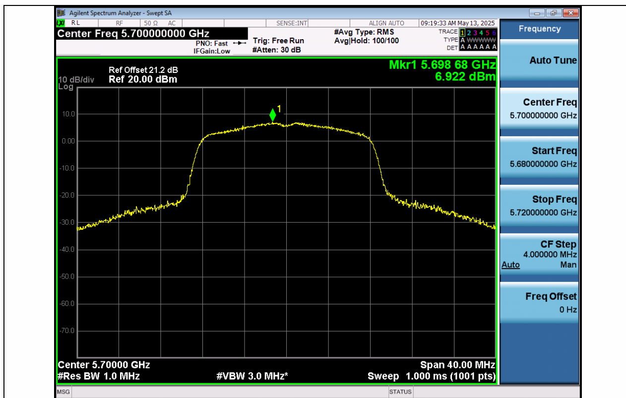
11A-Ant1-5700-PASS
