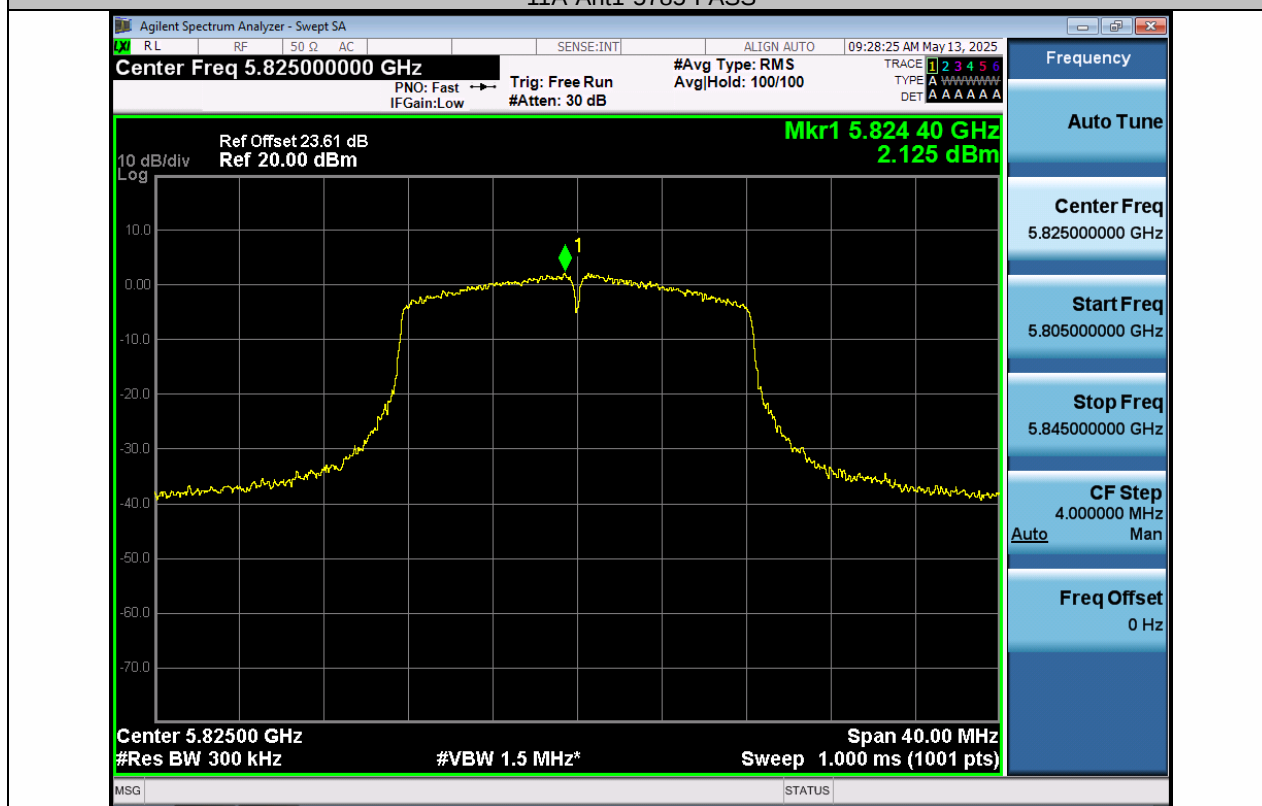
11A-Ant1-5825-PASS
