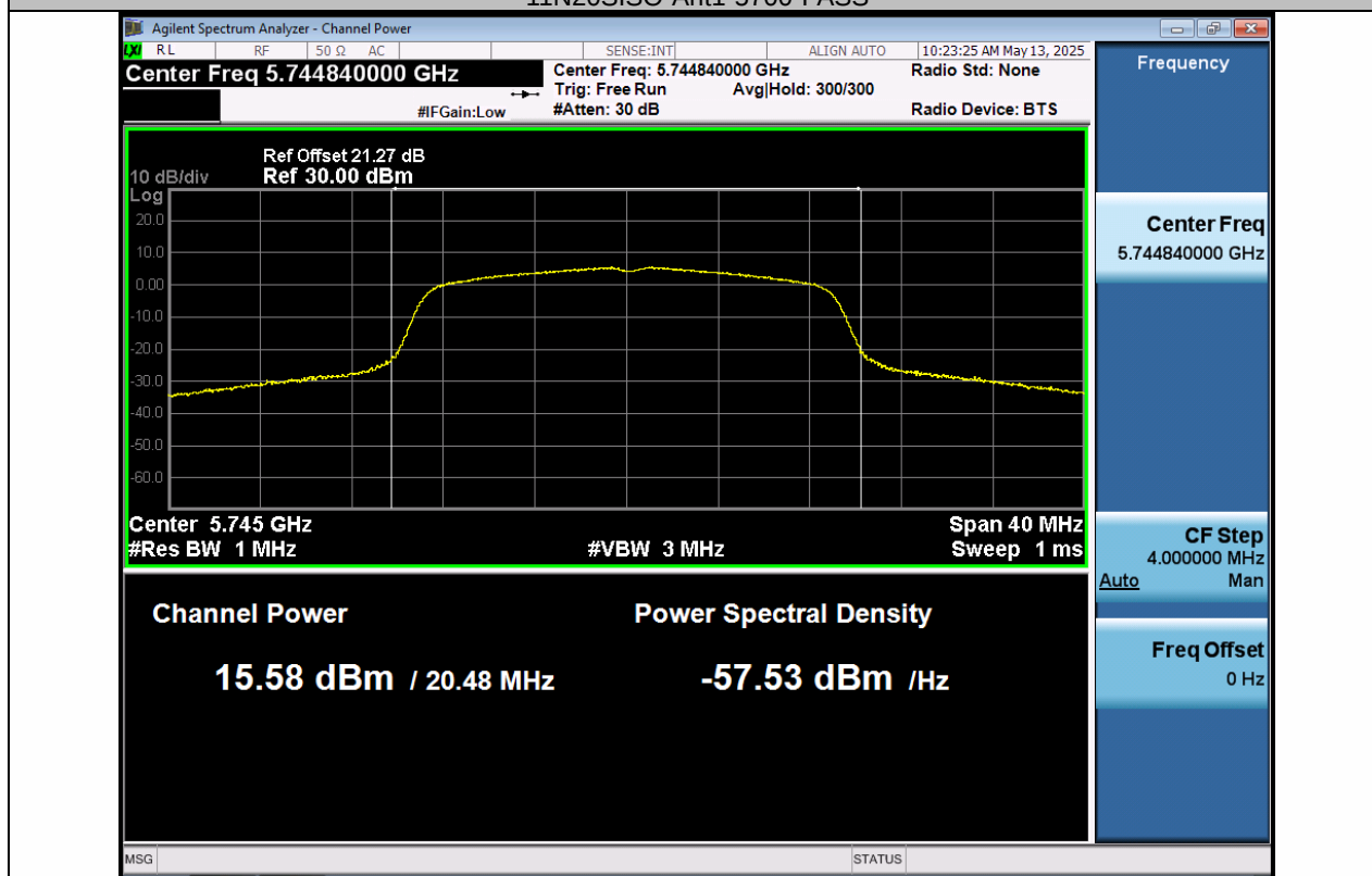
11N20SISO-Ant1-5745-PASS
