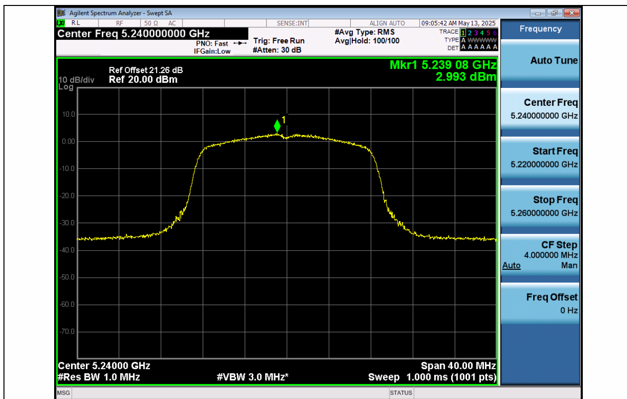
11A-Ant1-5240-PASS
