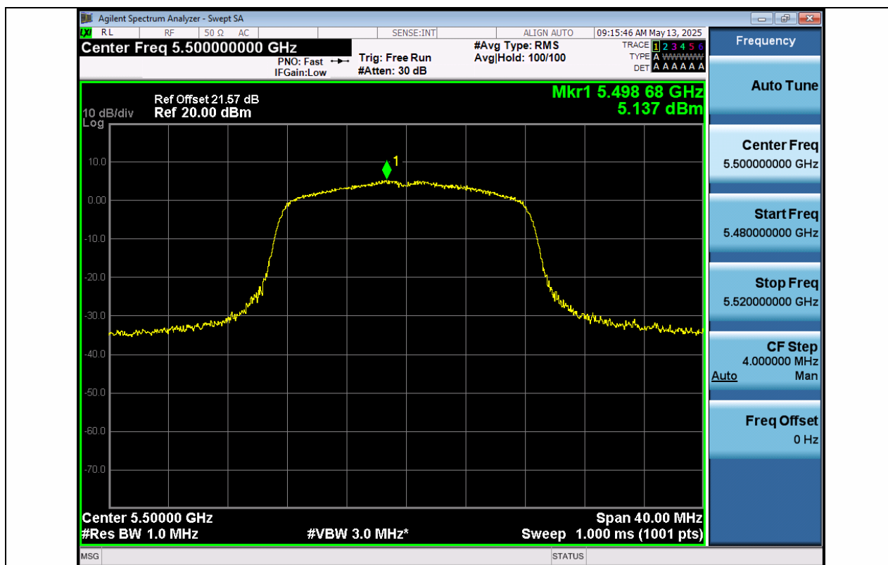
11A-Ant1-5500-PASS
