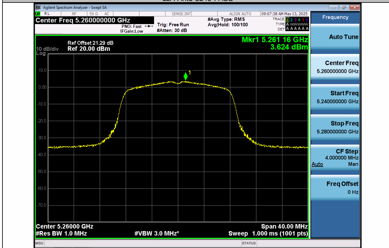
11A-Ant1-5260-PASS
