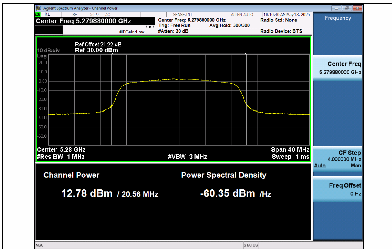
11N20SISO-Ant1-5280-PASS
