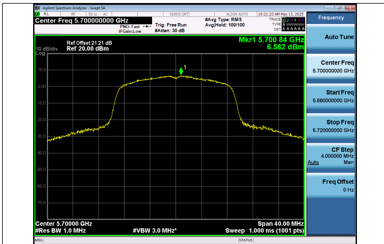
11N20SISO-Ant1-5700-PASS
