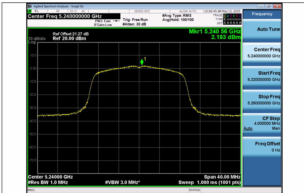
11N20SISO-Ant1-5240-PASS
