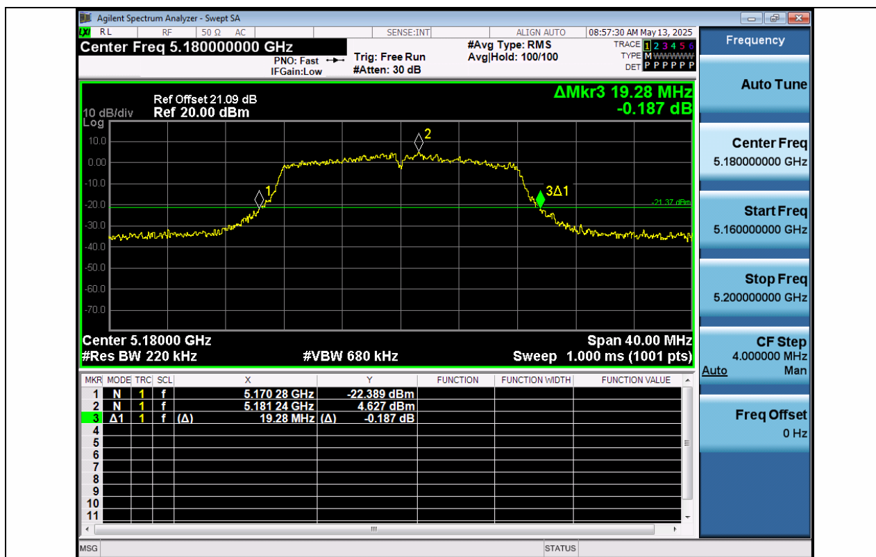
11A-Ant1-5180
