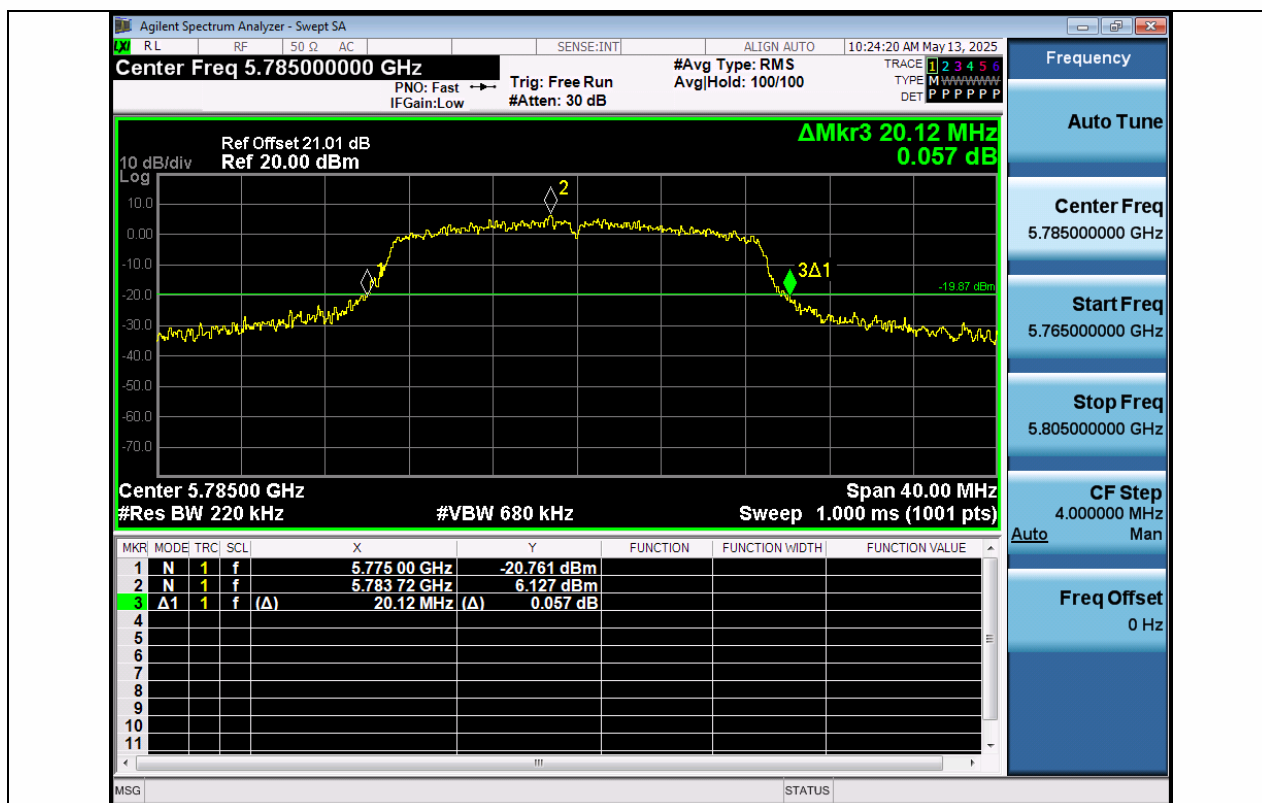
11N20SISO-Ant1-5785
