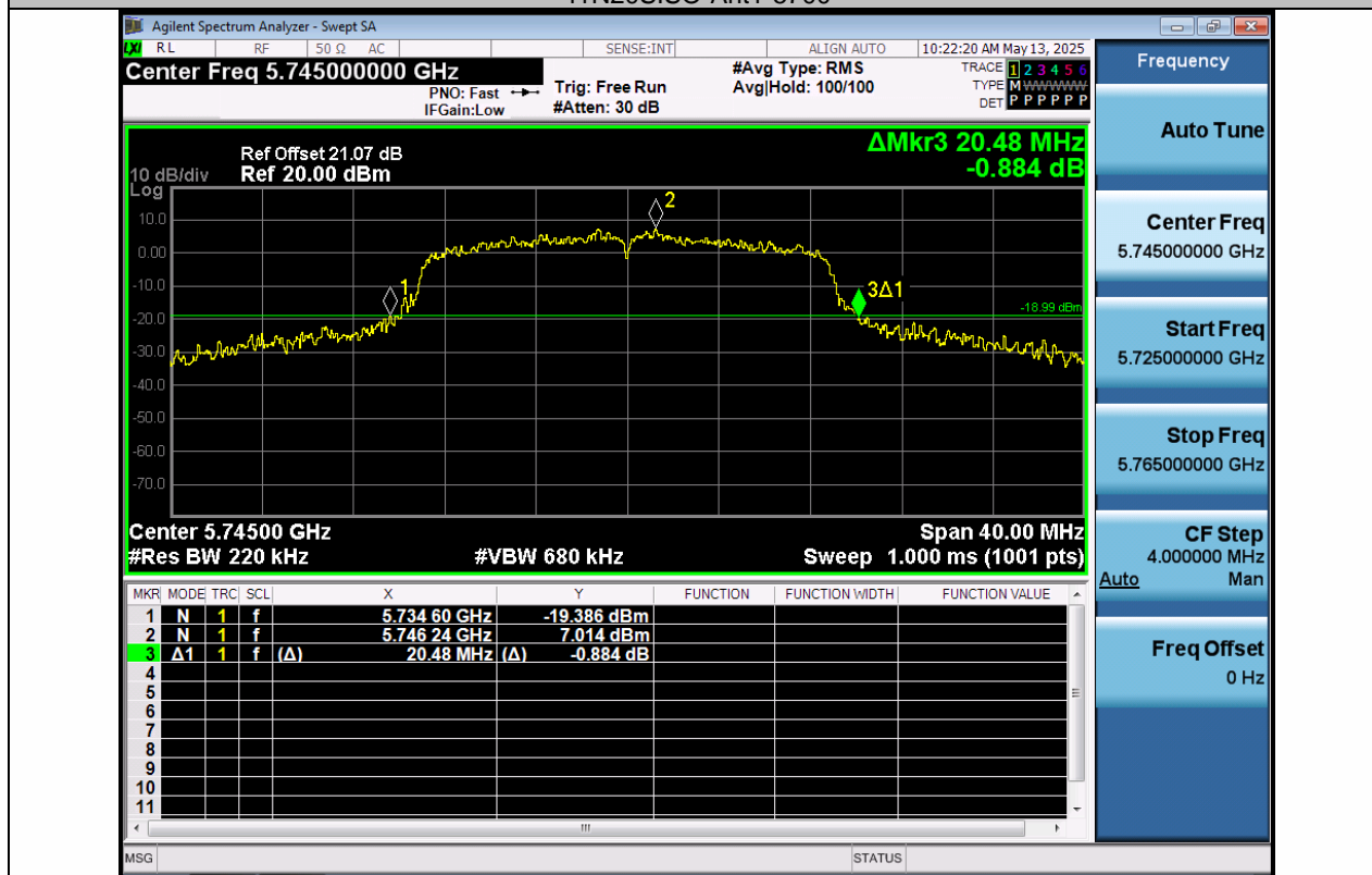
11N20SISO-Ant1-5745
