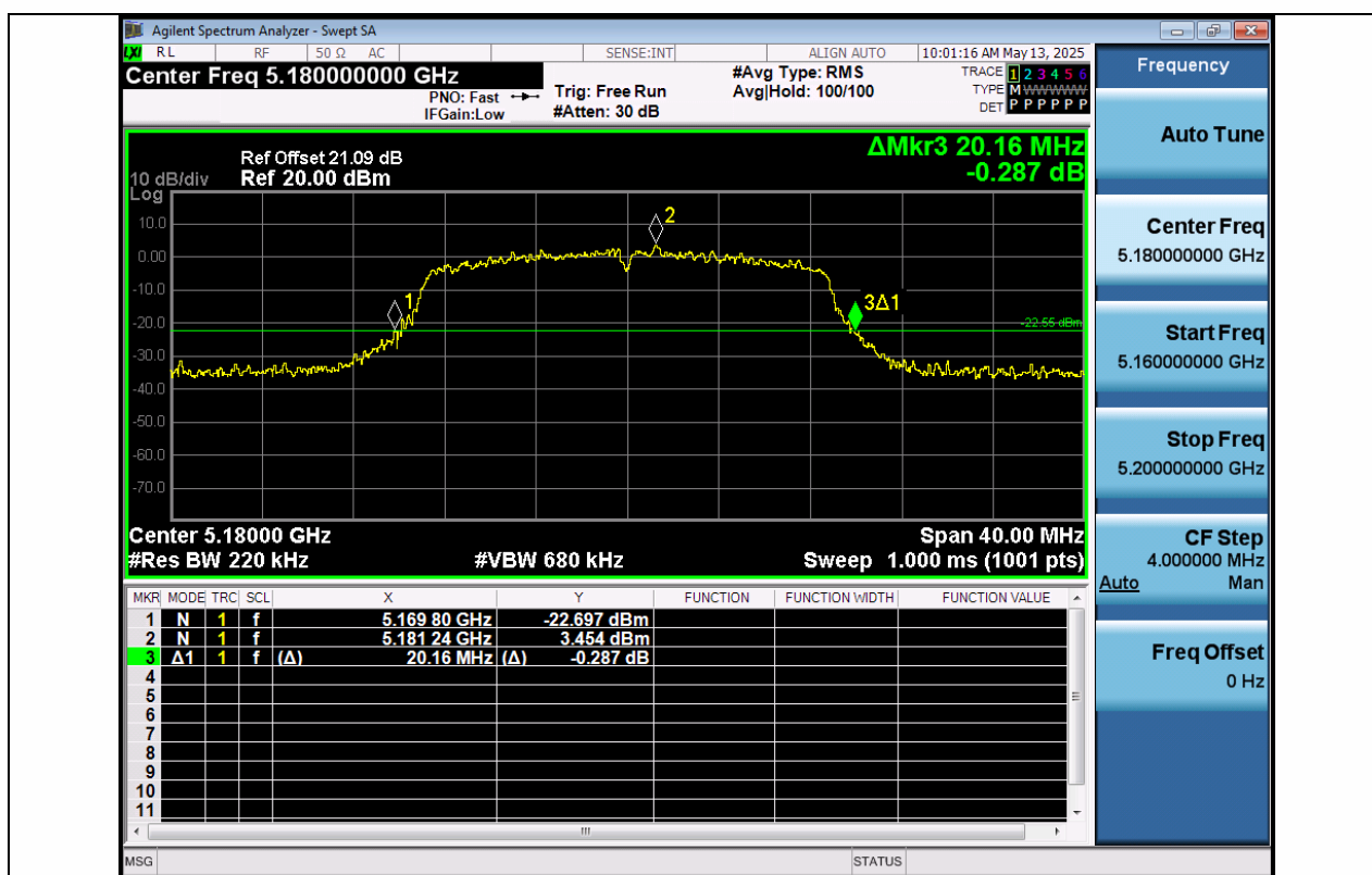
11N20SISO-Ant1-5180
