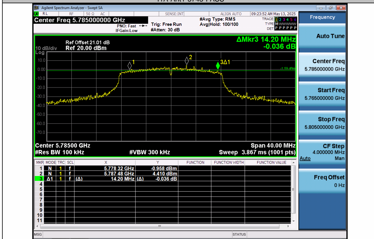
11A-Ant1-5785-PASS
