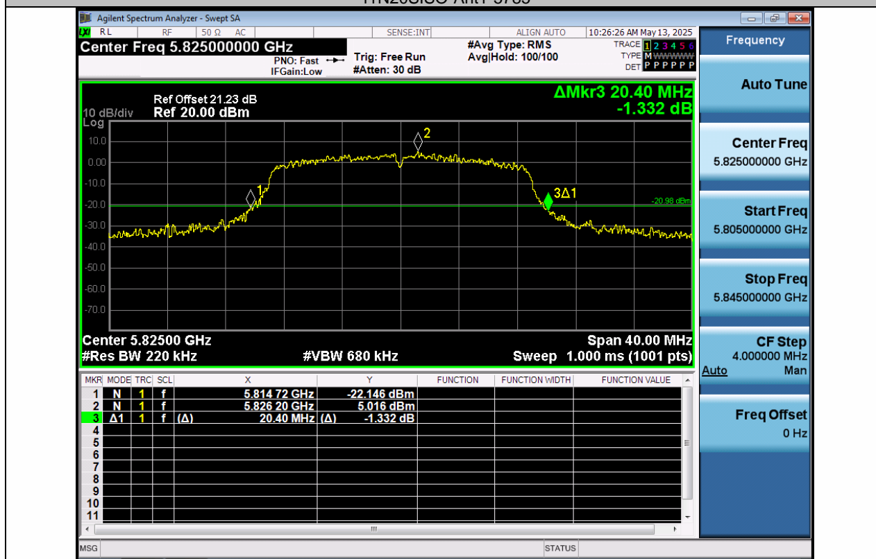
11N20SISO-Ant1-5825
