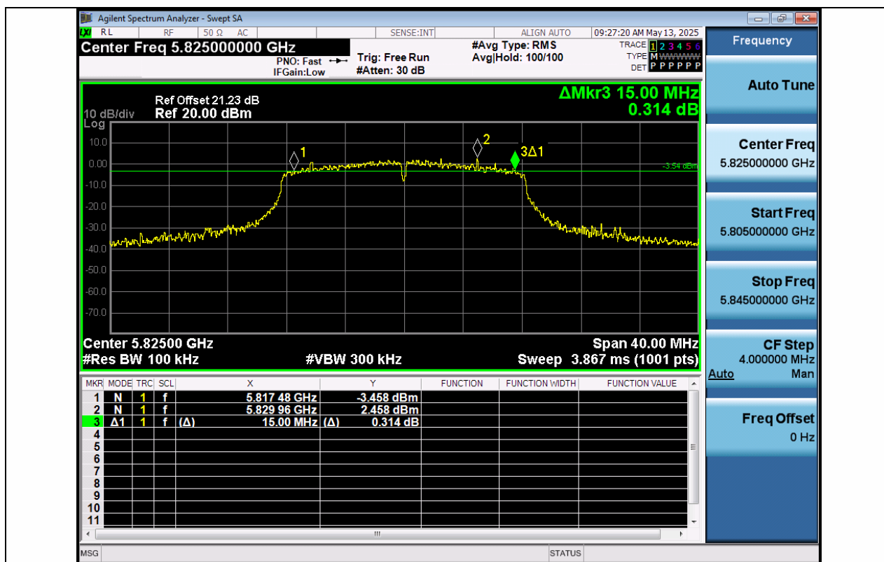
11A-Ant1-5825-PASS
