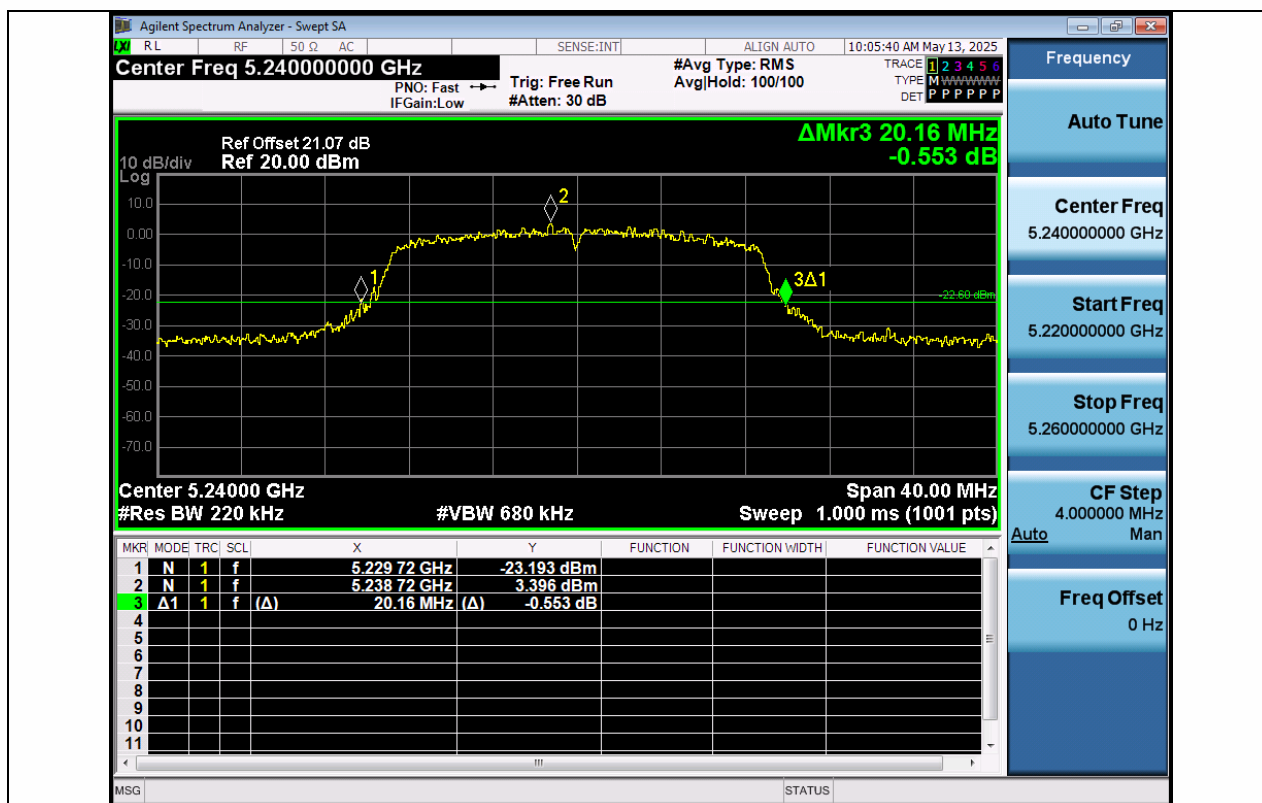
11N20SISO-Ant1-5240
