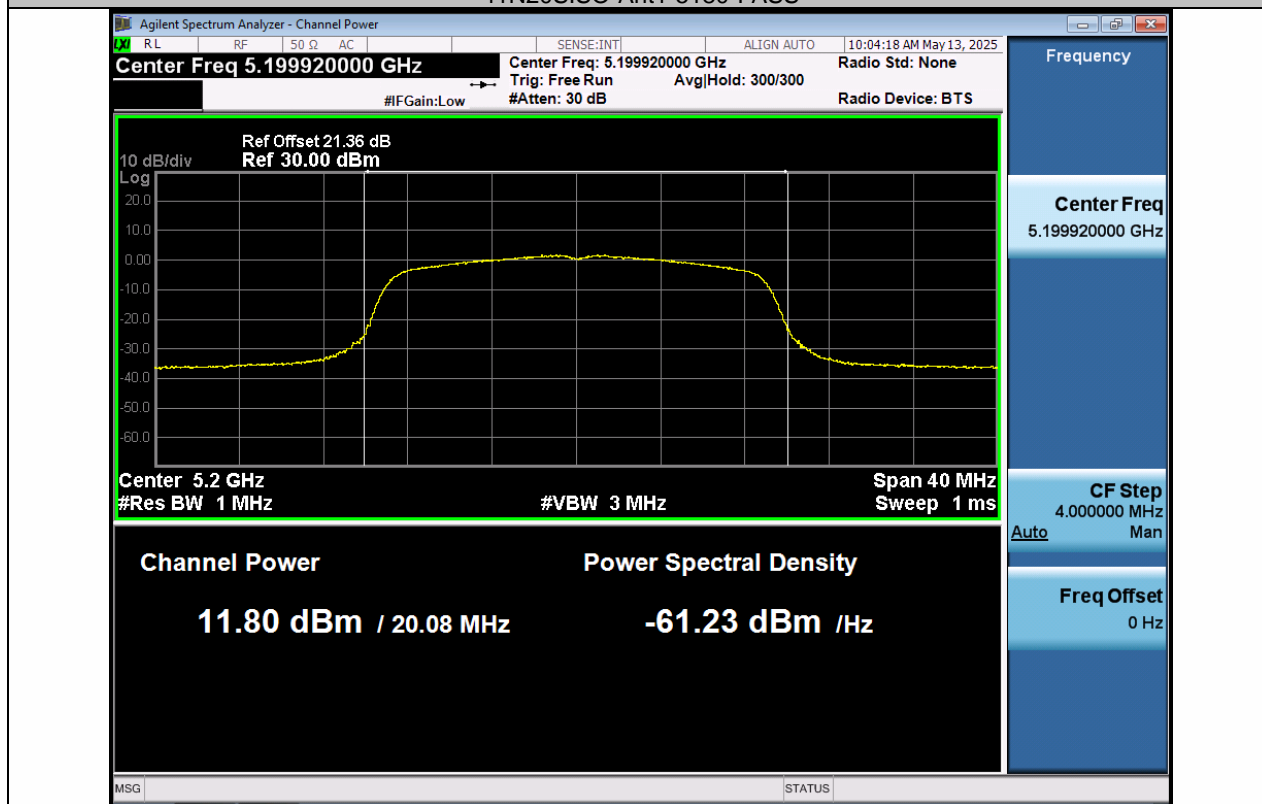
11N20SISO-Ant1-5200-PASS
