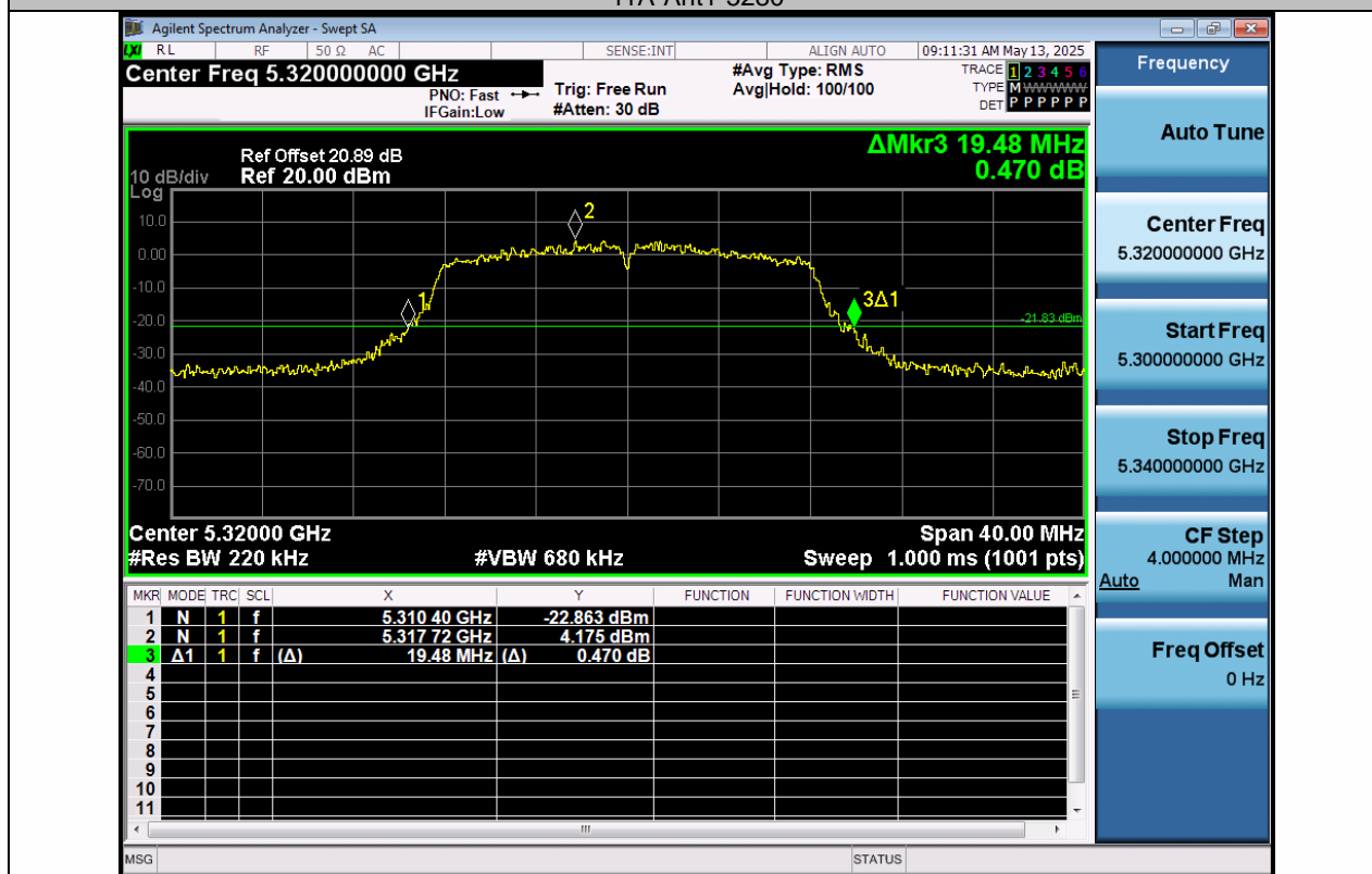
11A-Ant1-5320
