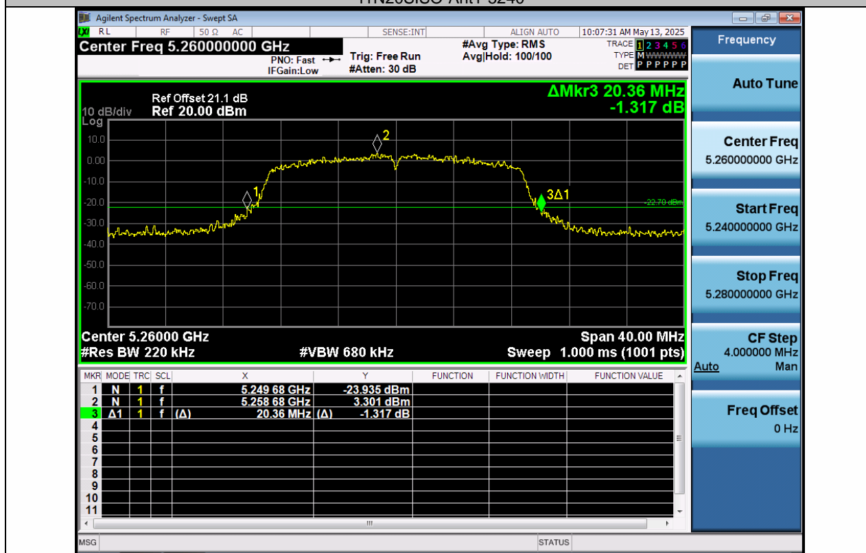
11N20SISO-Ant1-5260
