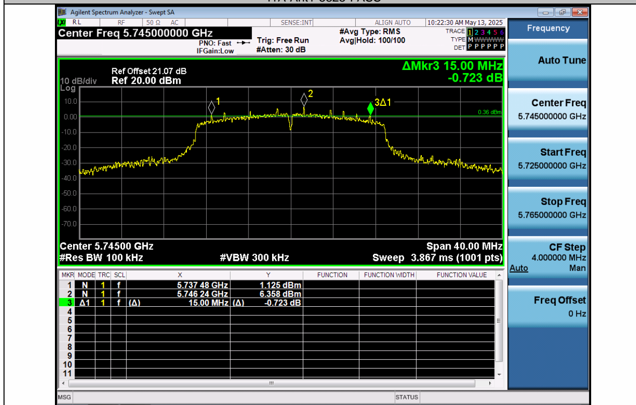
11N20SISO-Ant1-5745-PASS
