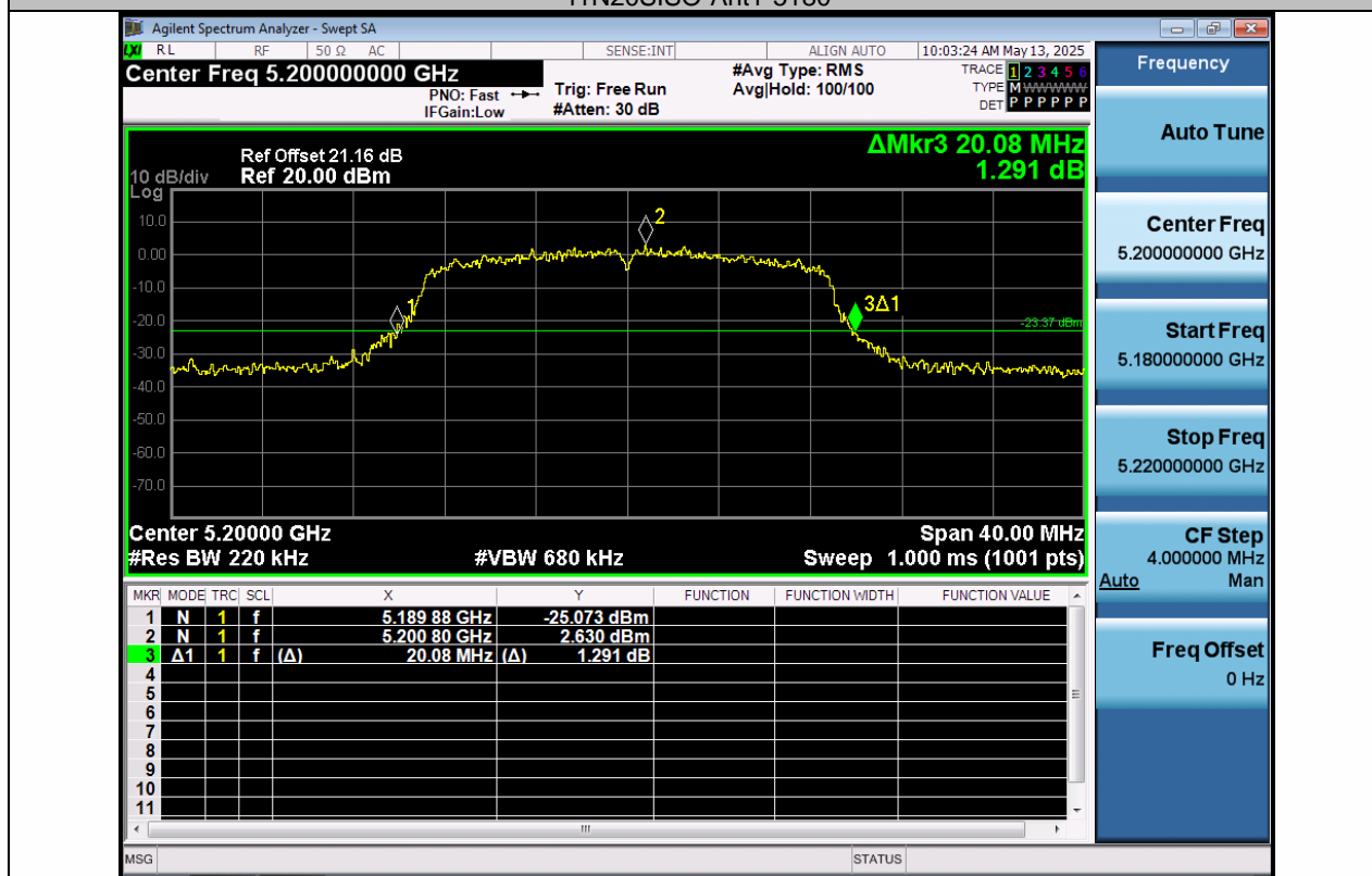
11N20SISO-Ant1-5200
