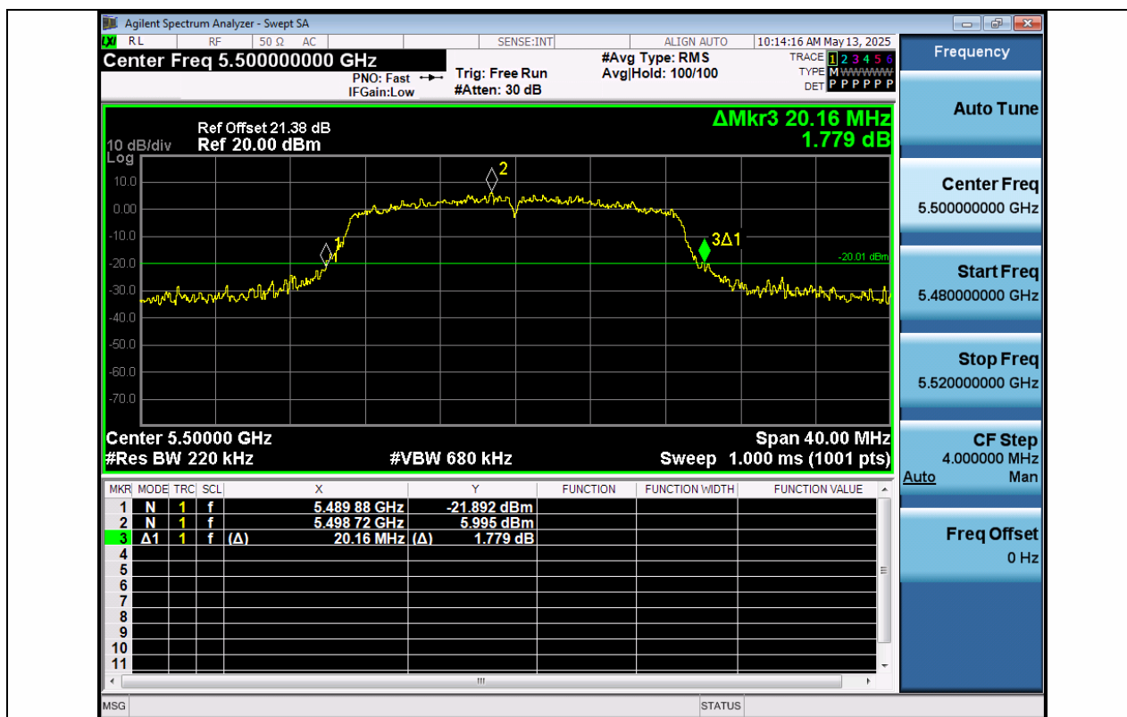
11N20SISO-Ant1-5500
