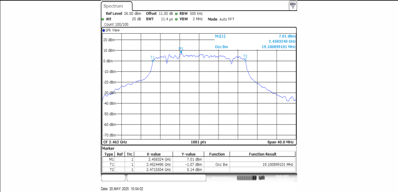
11AX20SISO-Ant1-2462
