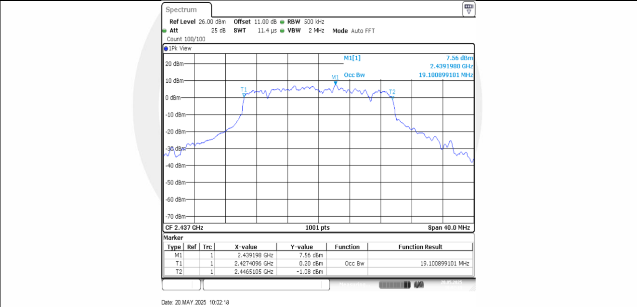
11AX20SISO-Ant1-2437
