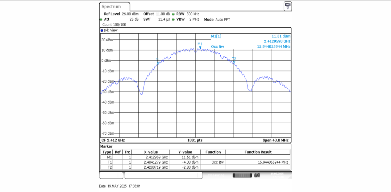
11B-Ant1-2412
