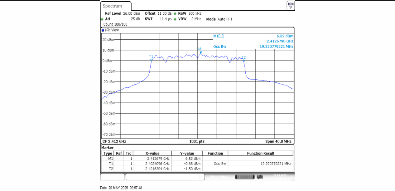
11AX20SISO-Ant1-2412
