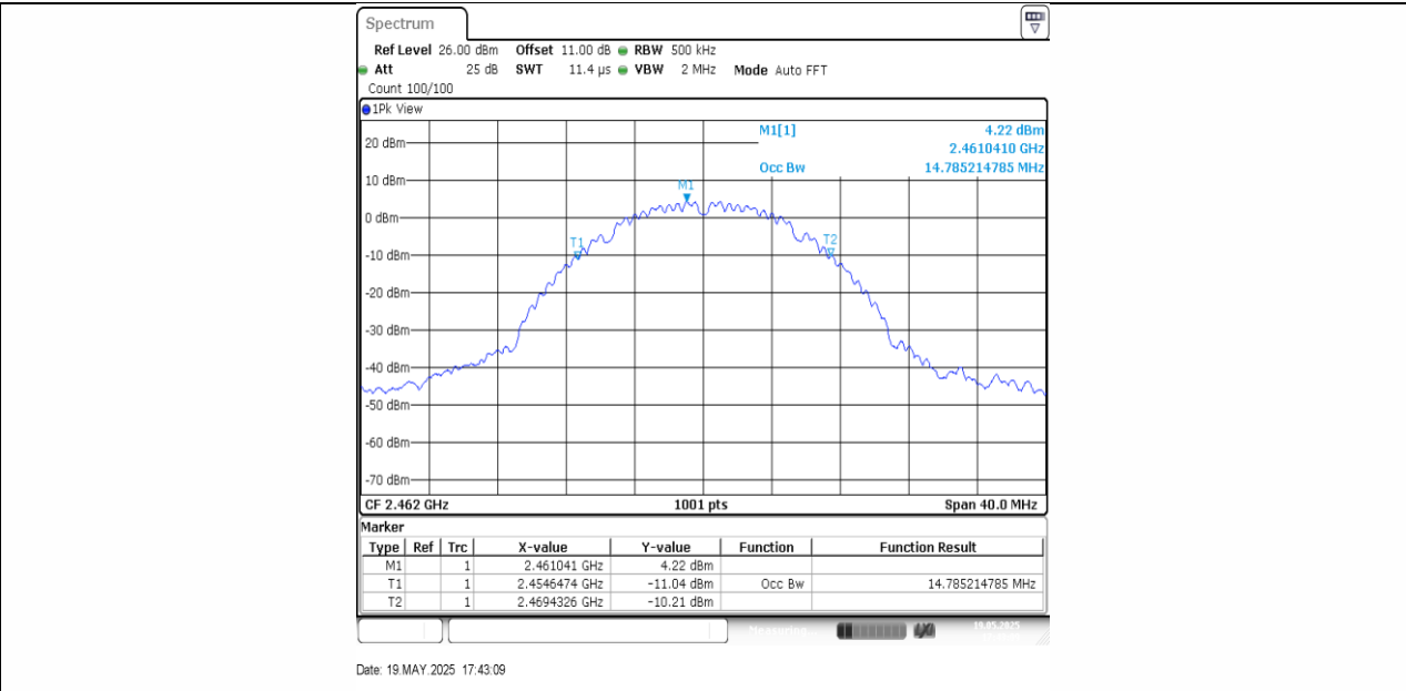
11B-Ant1-2462
