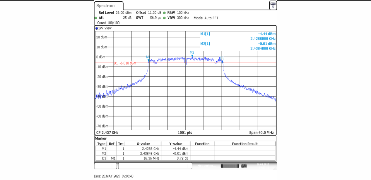
11G-Ant1-2437-PASS
