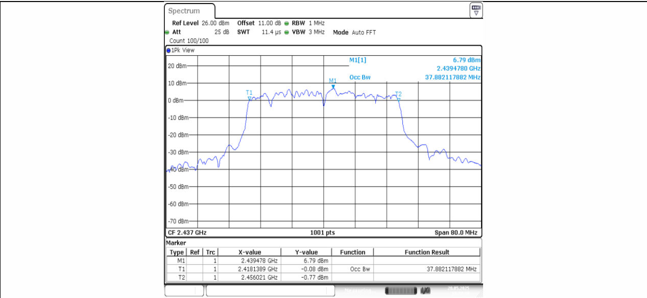
11AX40SISO-Ant1-2437
