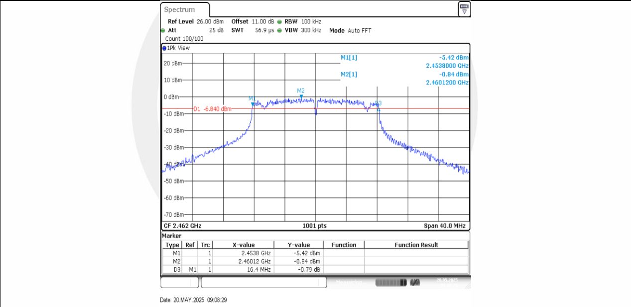
11G-Ant1-2462-PASS
