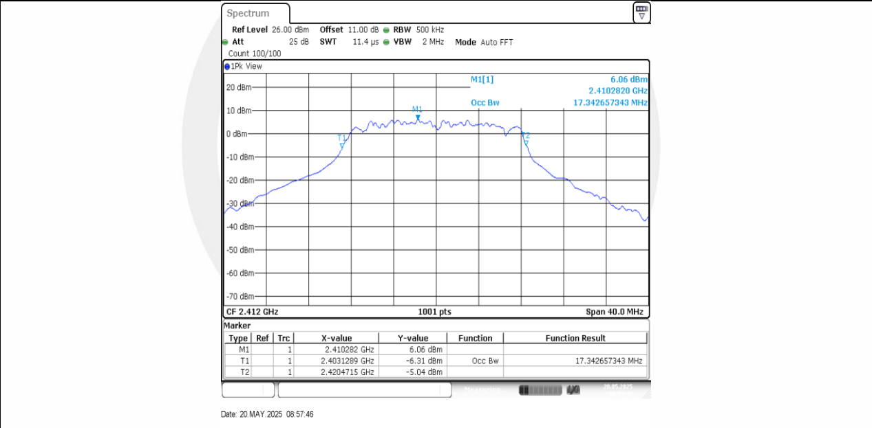
11G-Ant1-2412
