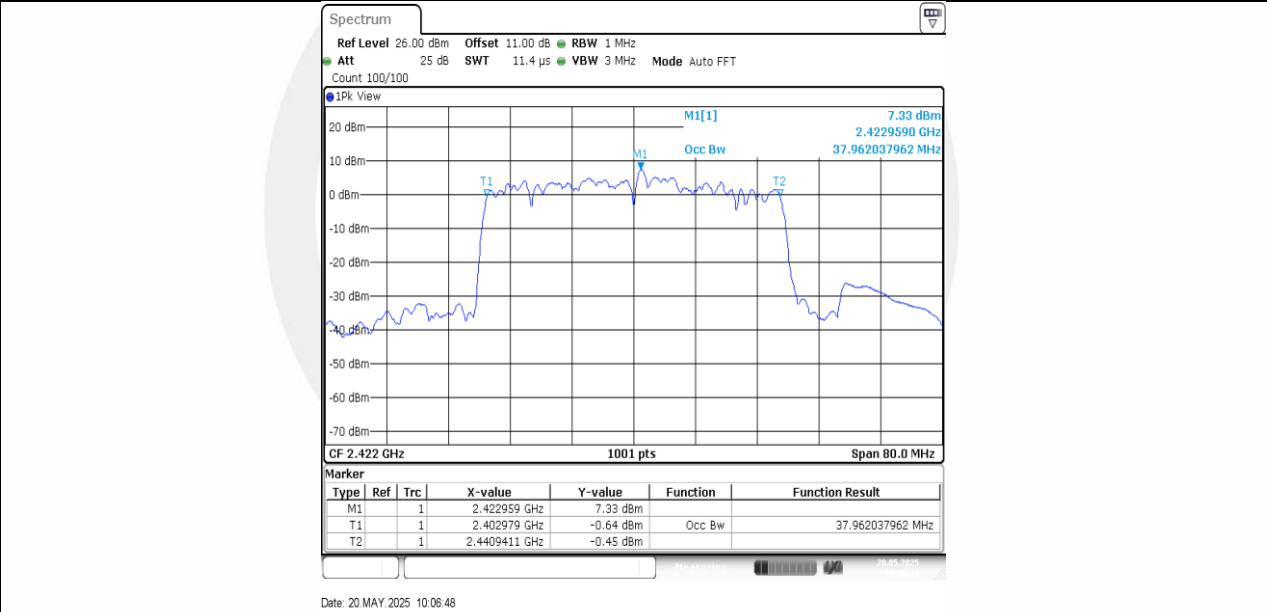
11AX40SISO-Ant1-2422
