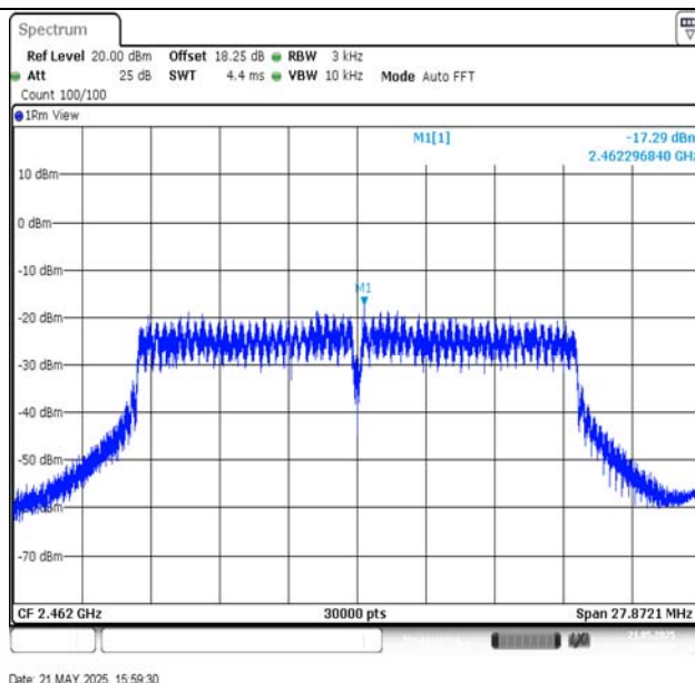
11N20SISO-Ant1-2462-PASS
