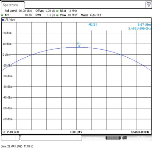
DH5-Ant1-2480-PASS
