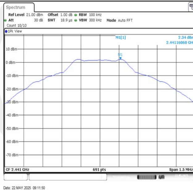
DH5-Ant1-2441-0~Reference-PASS
