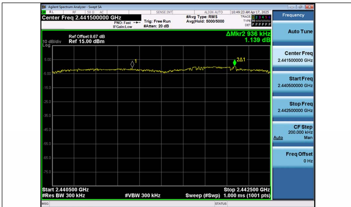
2DH5-Ant1-Hop_2441-PASS
