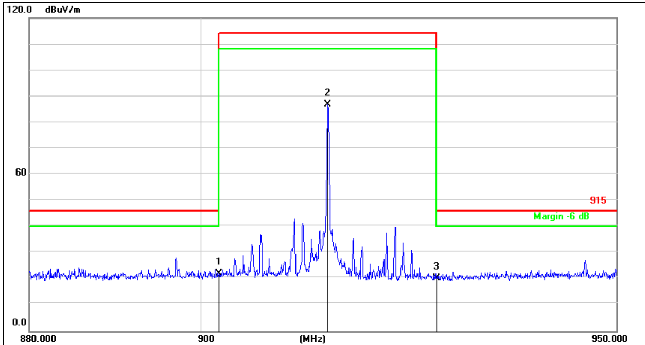
915 MHz Horizontal
