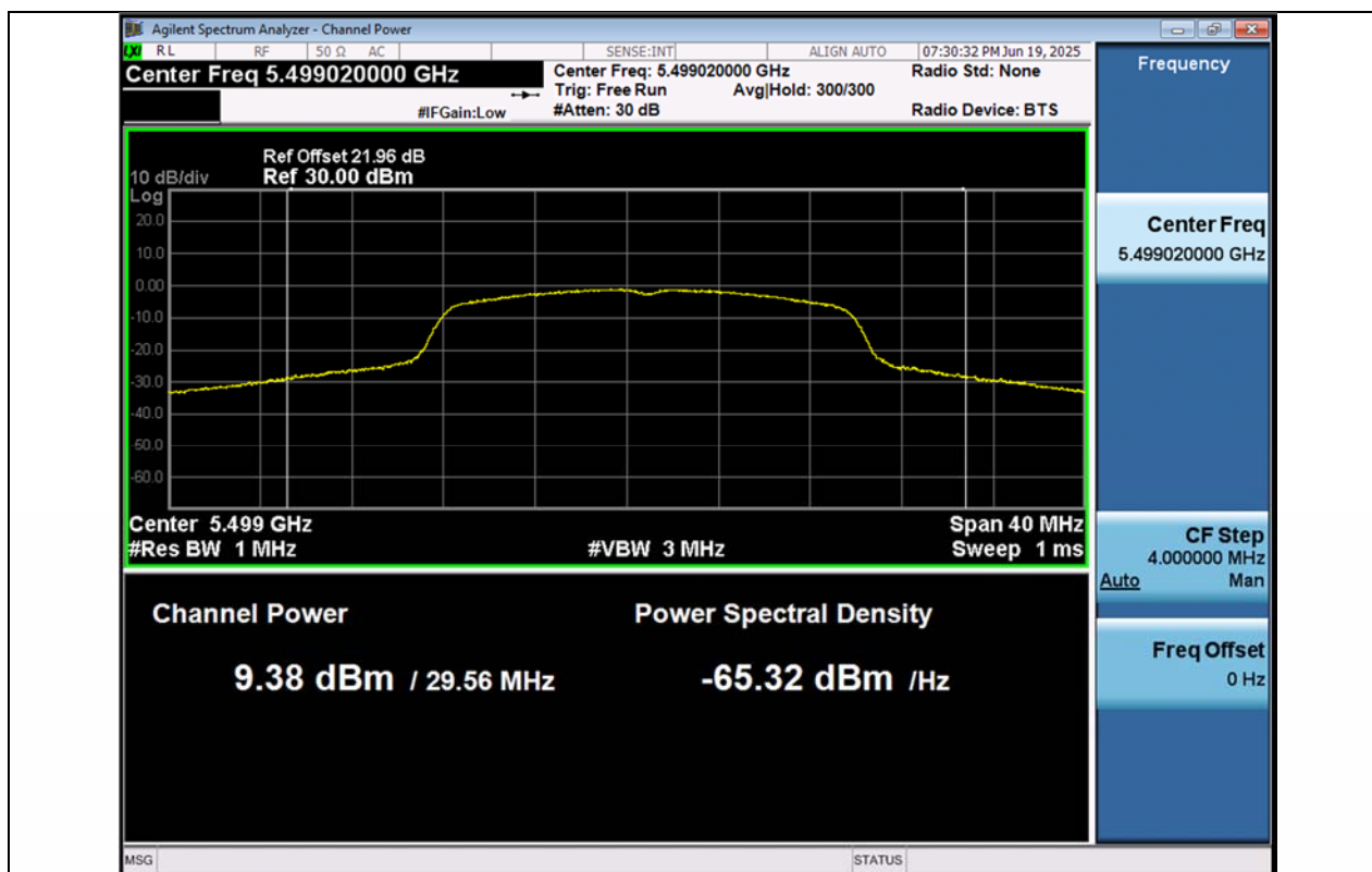
11N20SISO-Ant1-5500-PASS
