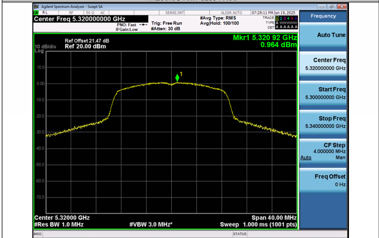
11N20SISO-Ant1-5320-PASS
