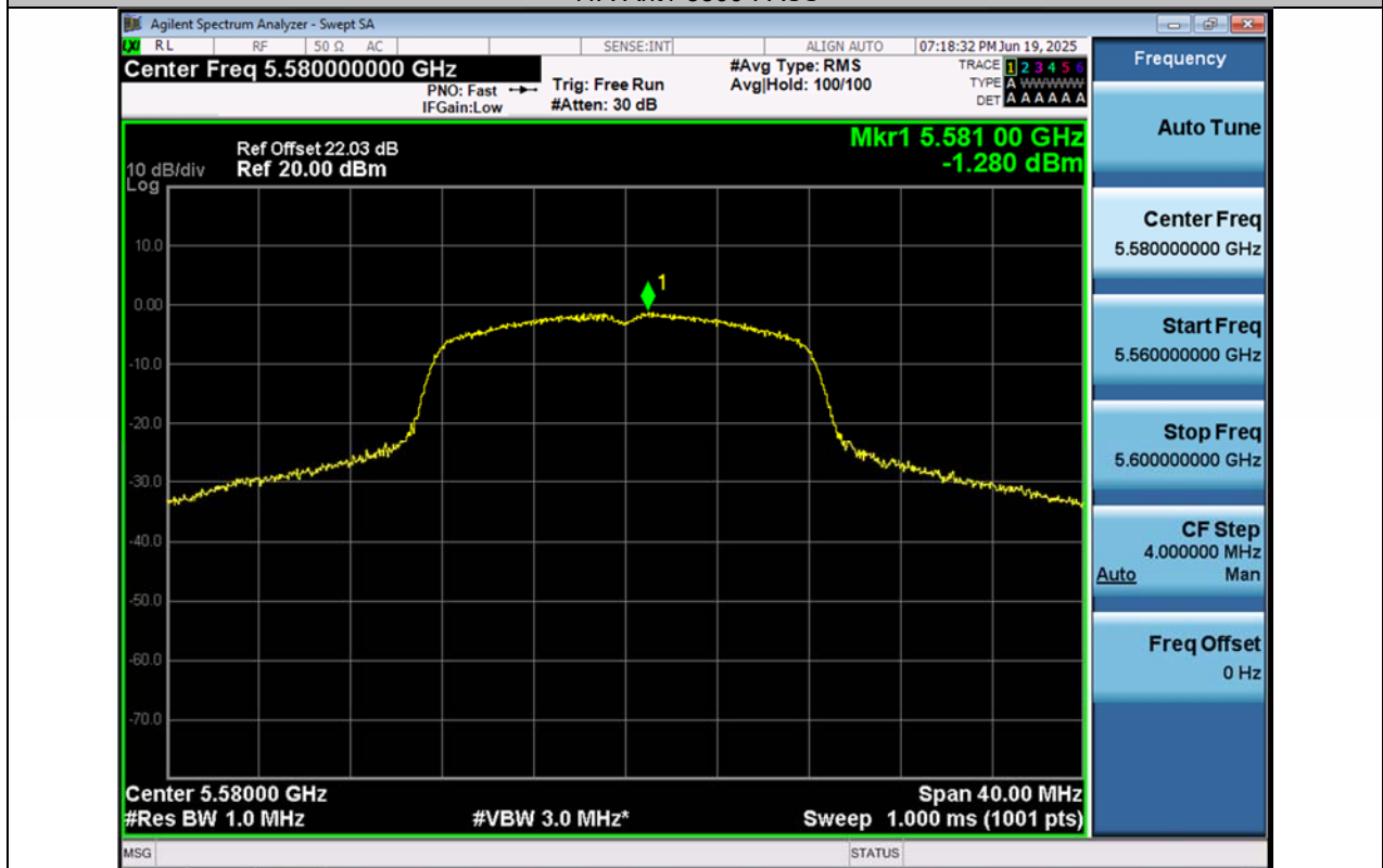
11A-Ant1-5580-PASS
