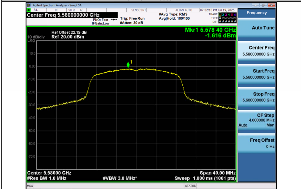
11N20SISO-Ant1-5580-PASS
