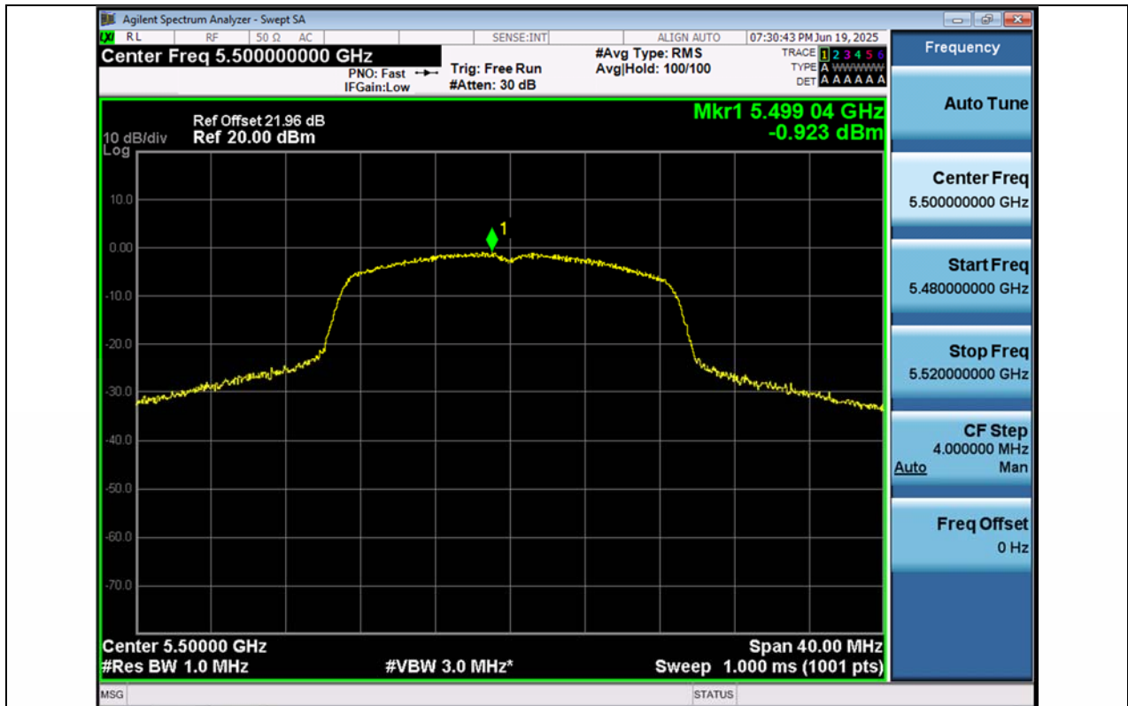
11N20SISO-Ant1-5500-PASS
