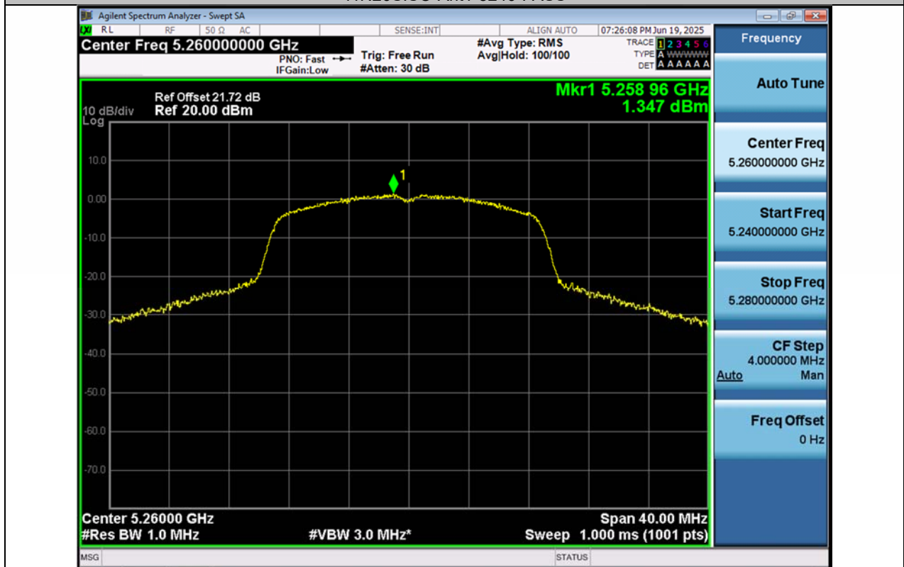
11N20SISO-Ant1-5260-PASS
