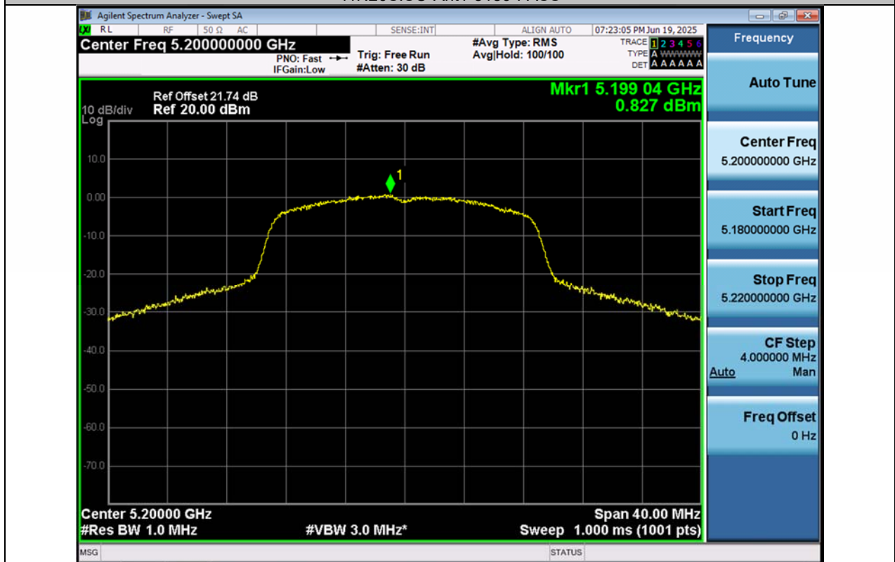
11N20SISO-Ant1-5200-PASS
