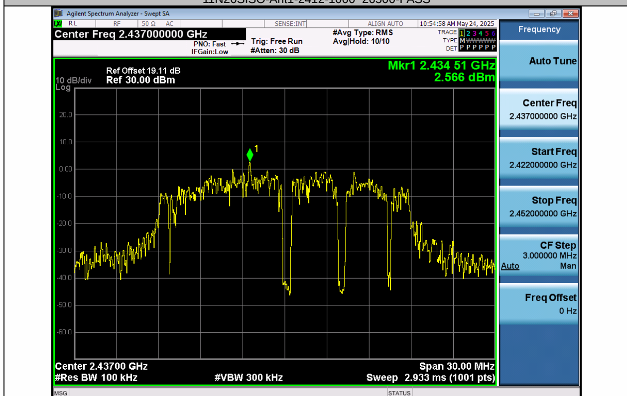
11N20SISO-Ant1-2437-0-Reference-PASS
