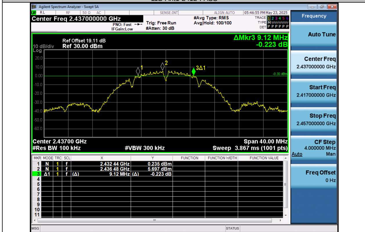
11B-Ant1-2437-PASS
