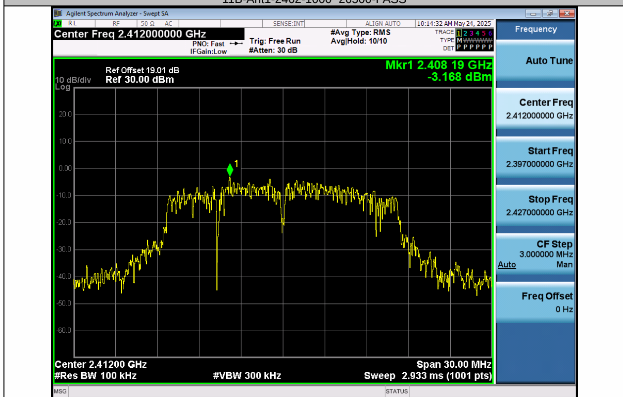
11G-Ant1-2412-0~Reference-PASS
