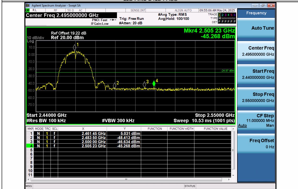
11B-Ant1-2462-PASS
