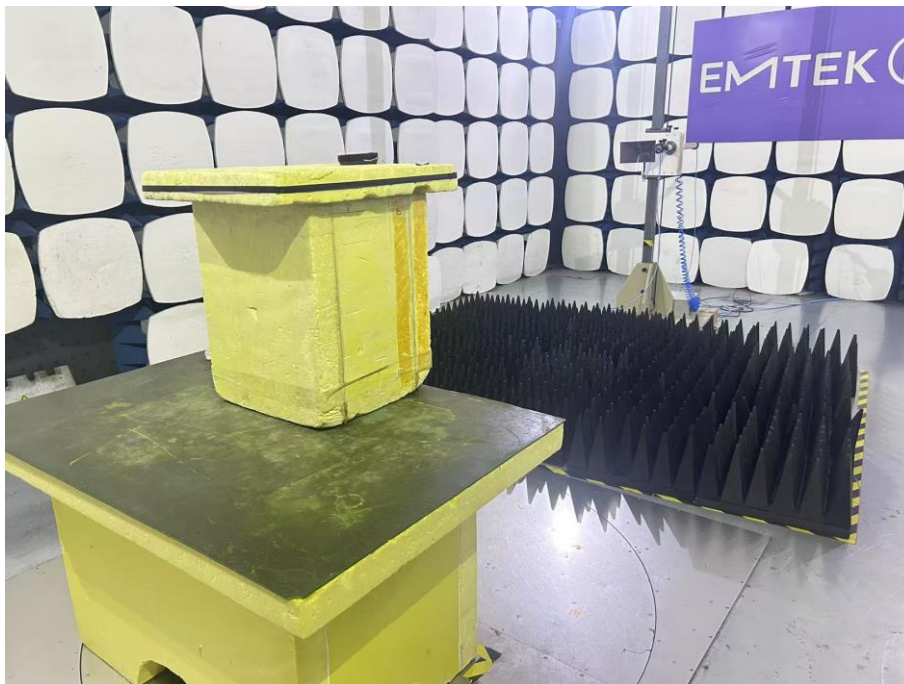
Spurious Emission Test Setup (Above 1GHz) FPC Antenna 1:
