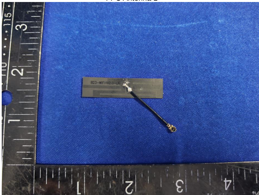
FPC Antenna 1
