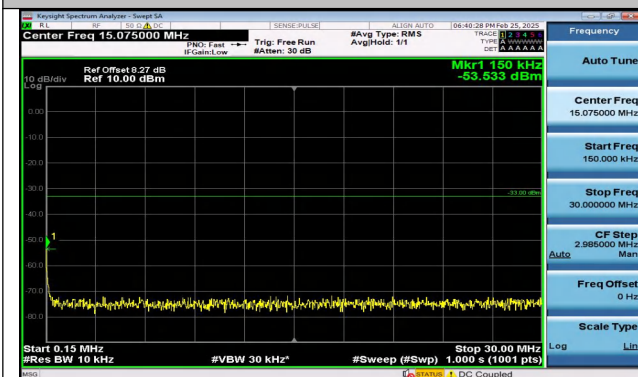
Band66_5MHz_16QAM_132322_1RB#0_0.15~30_0.15~3
