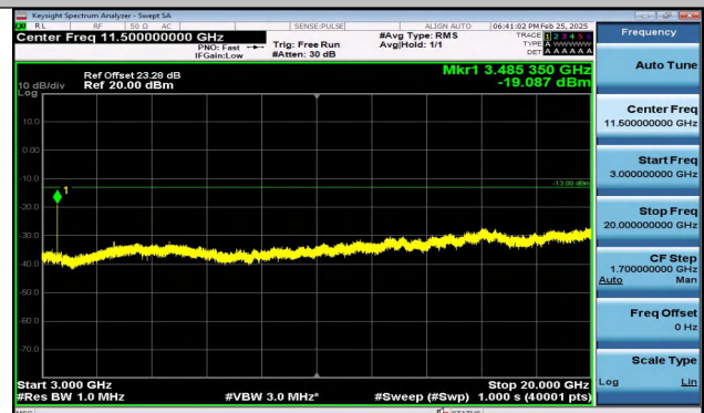
Band66_5MHz_16QAM_132322_1RB#0_3000~20000_30
