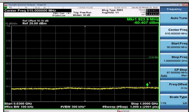
Band66_5MHz_16QAM_132322_1RB#0_30~1000_30~10
