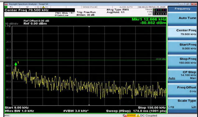
Band66_5MHz_16QAM_132322_1RB#0_0.009~0.15_0.00
