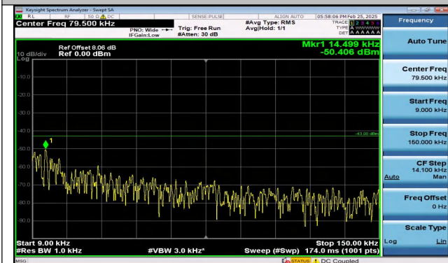
Band66_3MHz_16QAM_132322_1RB#14_0.009~0.15_0.0 09~0.15
