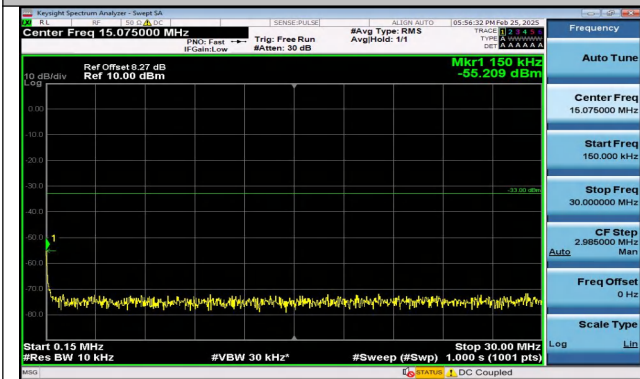
Band66_3MHz_16QAM_132322_1RB#0_0.15~30_0.15~3 0
