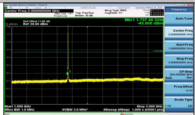
Band66_3MHz_QPSK_132322_1RB#0_1000~3000_1000 ~3000
