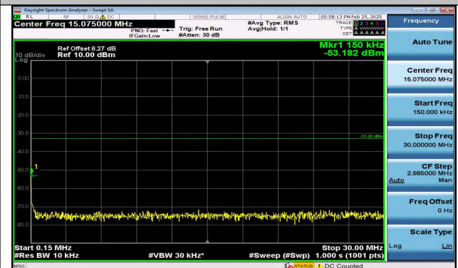
Band66_3MHz_16QAM_132322_1RB#14_0.15~30_0.15~ 30
