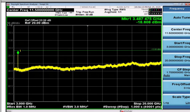
Band66_3MHz_QPSK_132322_1RB#0_3000~20000_300 0~20000
