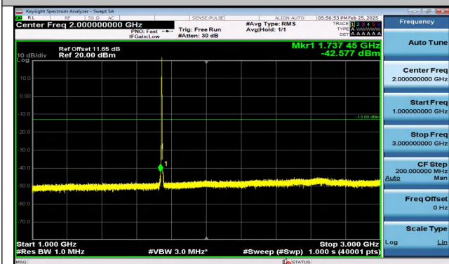
Band66_3MHz_16QAM_132322_1RB#0_1000~3000_100 0~3000
