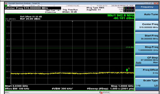
Band66_3MHz_16QAM_132322_1RB#0_30~1000_30~10 00
