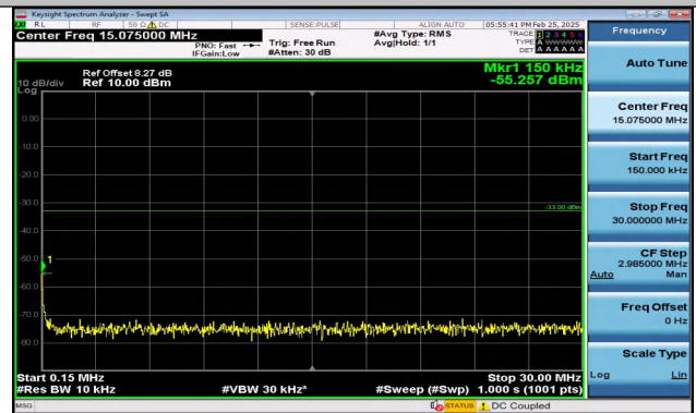
Band66_3MHz_QPSK_132322_1RB#0_0.15~30_0.15~30
