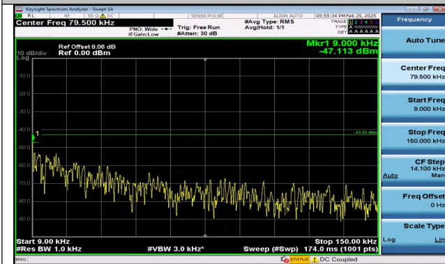
Band66_3MHz_QPSK_132322_1RB#0_0.009~0.15_0.009 ~0.15
