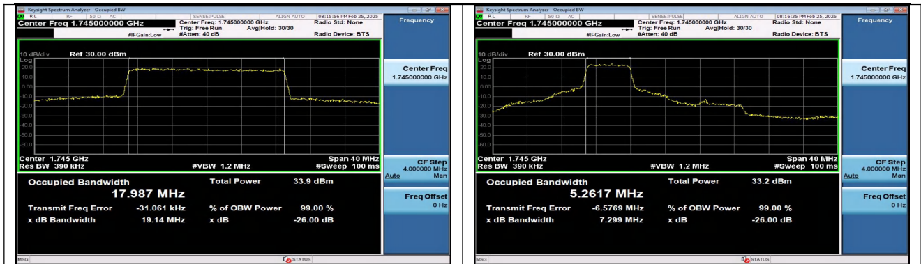
Band66-20MHz-QPSK-132322-100RB#0-PASS
