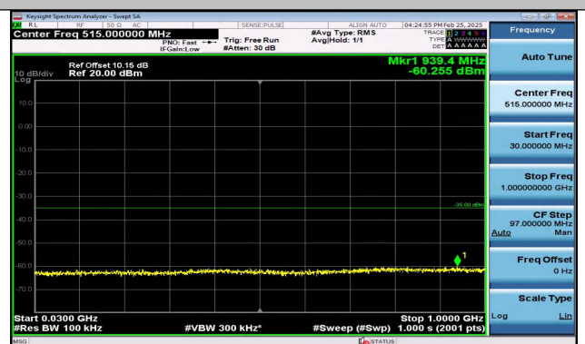
Band41_20MHz_16QAM_39750_1RB#0_30~1000_30~10 00
