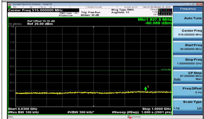
Band41_20MHz_QPSK_39750_100RB#0_30~1000_30~1 000
