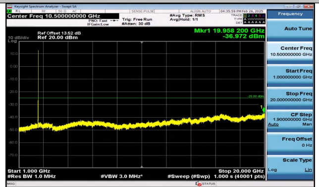
Band41_20MHz_QPSK_39750_100RB#0_1000~20000_1 000~20000
