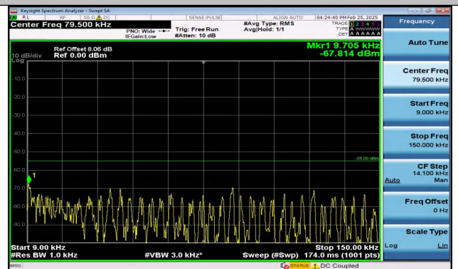
Band41_20MHz_16QAM_39750_1RB#0_0.009~0.15_0.00 9~0.15
