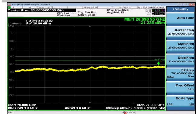
Band41_20MHz_QPSK_39750_100RB#0_20000~27000_20000~27000
