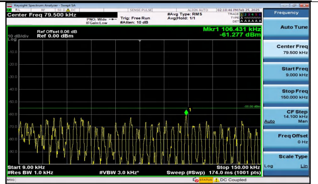
Band41_10MHz_16QAM_41540_1RB#0_0.009~0.15_0.00 9~0.15
