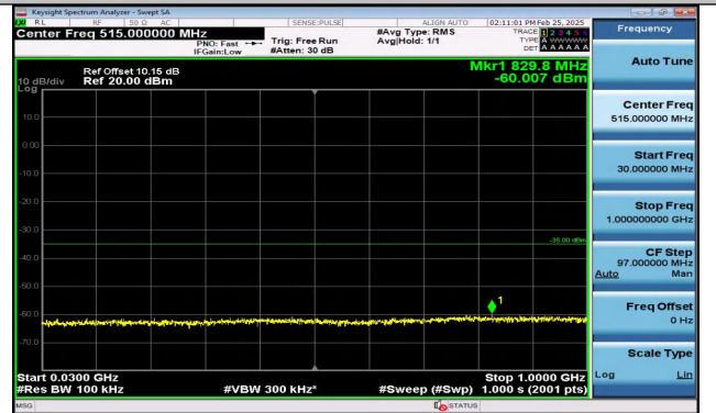
Band41_10MHz_16QAM_41540_1RB#0_30~1000_30~10 00
