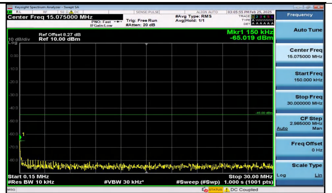
Band41_15MHz_QPSK_39725_1RB#74_0.15~30_0.15~3 0
