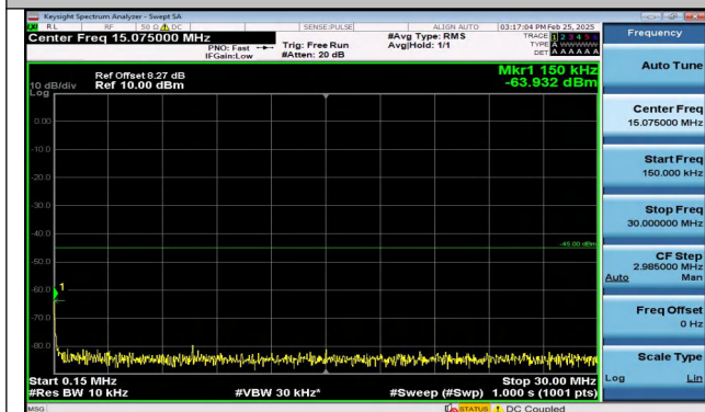
Band41_15MHz_QPSK_39725_75RB#0_0.15~30_0.15~3 0
