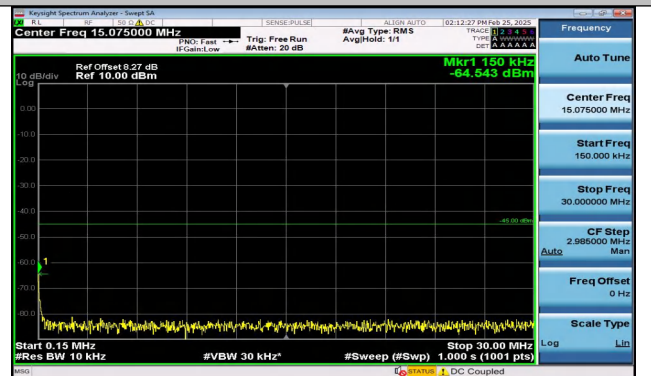
Band41_10MHz_16QAM_41540_1RB#49_0.15~30_0.15~3 30
