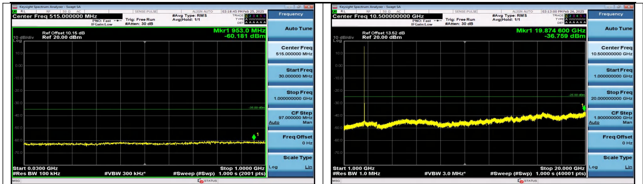
Band41_15MHz_QPSK_40620_75RB#0_30~1000_30~1000
