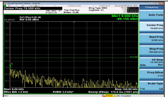
Band41_15MHz_QPSK_39725_75RB#0_0.009~0.15_0.00 9~0.15
