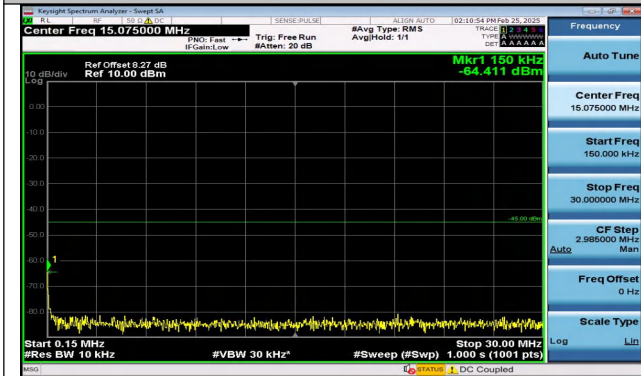
Band41_10MHz_16QAM_41540_1RB#0_0.15~30_0.15~3 0
