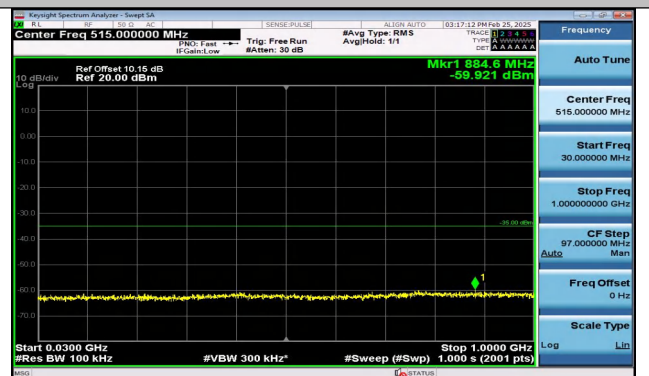
Band41_15MHz_QPSK_39725_75RB#0_30~1000_30~10 00
