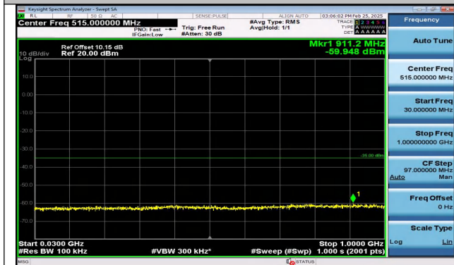
Band41_15MHz_QPSK_39725_1RB#74_30~1000_30~10 00
