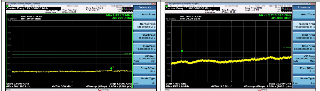
Band41_10MHz_QPSK_41540_50RB#0_30~1000_30~10 00
