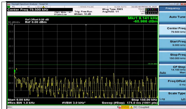
Band41_15MHz_QPSK_39725_1RB#74_0.009~0.15_0.00 9~0.15
