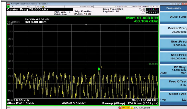
Band41_10MHz_16QAM_41540_1RB#49_0.009~0.15_0.0 09~0.15
