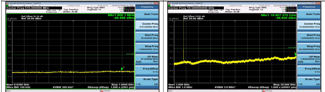
Band41_15MHz_16QAM_39725_1RB#0_30~1000_30~1000
