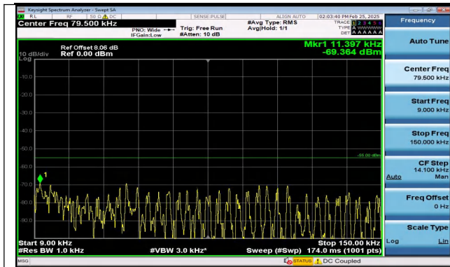
Band41_10MHz_QPSK_39700_1RB#0_0.009~0.15_0.009 ~0.15
