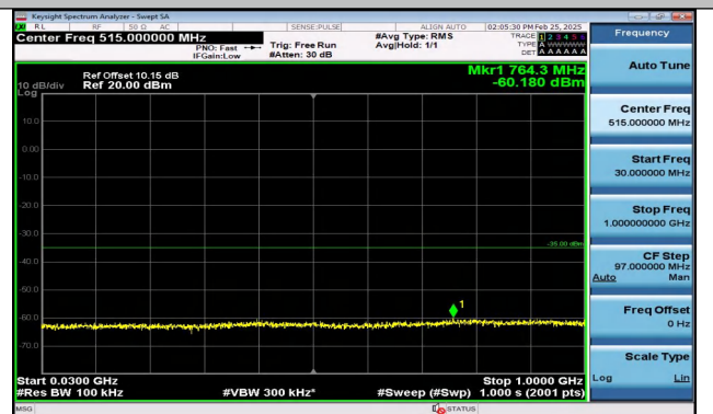
Band41_10MHz_QPSK_39700_1RB#49_30~1000_30~10 00
