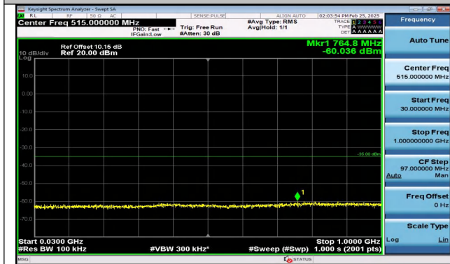
Band41_10MHz_QPSK_39700_1RB#0_30~1000_30~100 0
