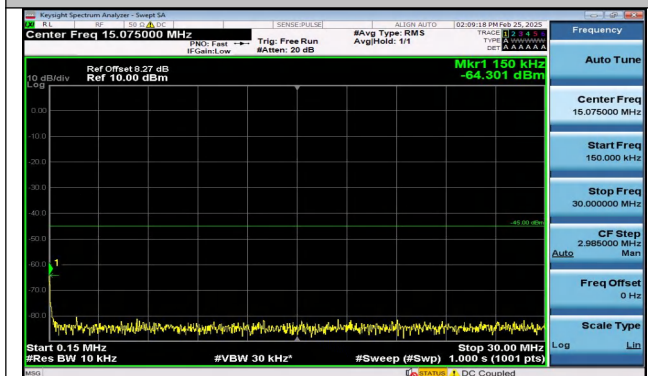
Band41_10MHz_16QAM_40620_1RB#49_0.15~30_0.15~ 30
