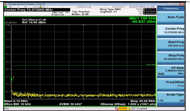
Band41_10MHz_QPSK_39700_1RB#0_0.15~30_0.15~30
