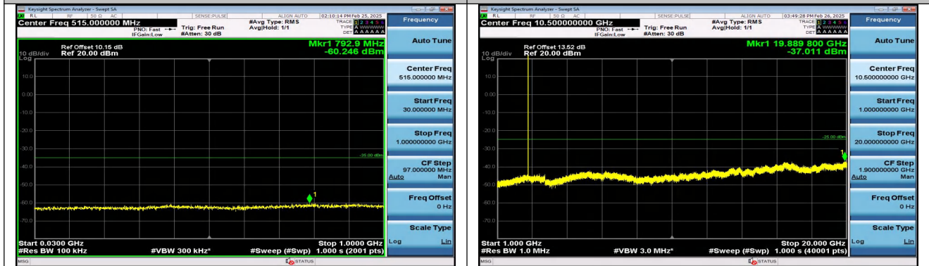
Band41_10MHz_QPSK_41540_1RB#0_30~1000_30~1000
