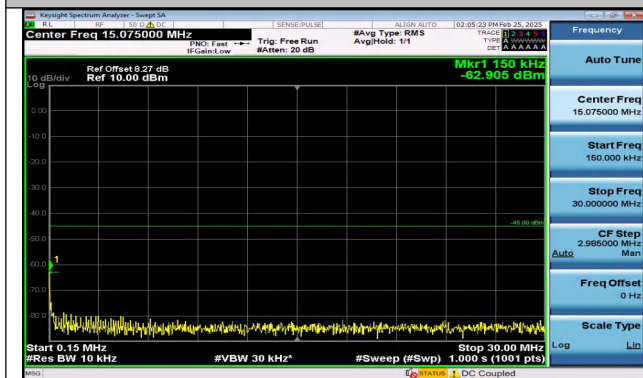
Band41_10MHz_QPSK_39700_1RB#49_0.15~30_0.15~3 0
