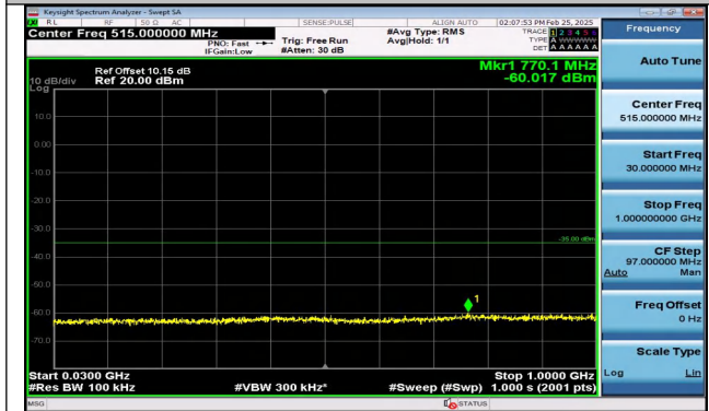
Band41_10MHz_16QAM_40620_1RB#0_30~1000_30~10 00
