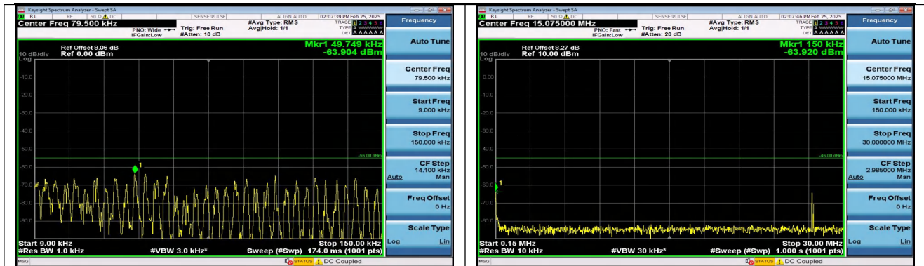
Band41_10MHz_16QAM_40620_1RB#0_0.009~0.15_0.00 9~0.15
