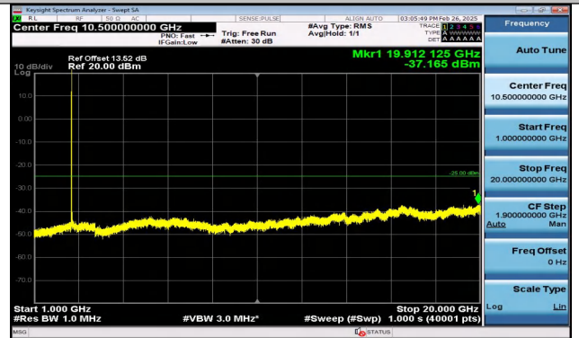
Band41_10MHz_16QAM_40620_1RB#0_1000~20000_10 00~20000
