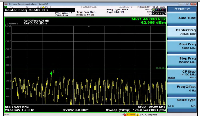
Band41_10MHz_16QAM_40620_1RB#49_0.009~0.15_0.0 09~0.15
