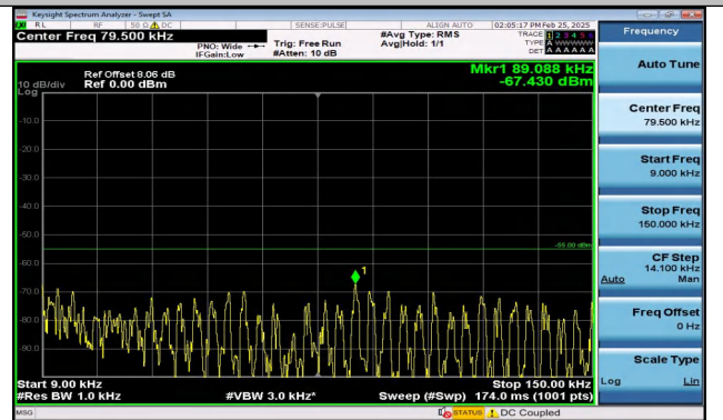
Band41_10MHz_QPSK_39700_1RB#49_0.009~0.15_0.00 9~0.15
