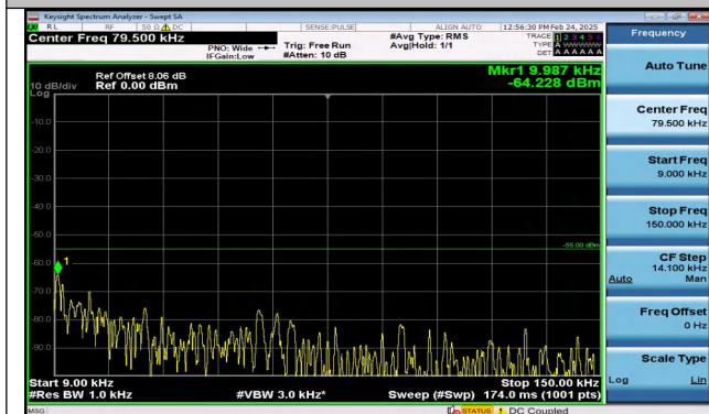
Band38_10MHz_QPSK_38200_50RB#0_0.009~0.15_0.00 9~0.15
