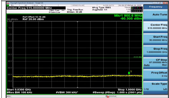
Band38_15MHz_QPSK_37825_1RB#74_30~1000_30~10 00
