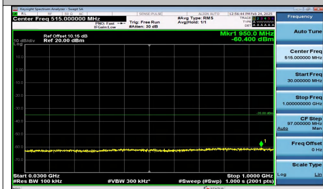
Band38_10MHz_QPSK_38200_50RB#0_30~1000_30~10 00
