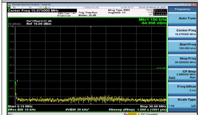
Band38_15MHz_QPSK_37825_75RB#0_0.15~30_0.15~3 0
