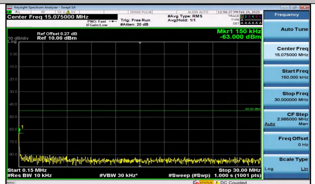
Band38_10MHz_QPSK_38200_50RB#0_0.15~30_0.15~3 0
