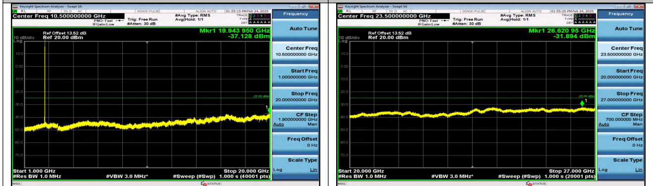
Band38_15MHz_16QAM_38000_1RB#0_1000~20000_1000~20000
