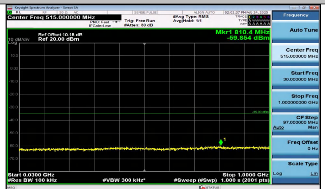
Band38_15MHz_QPSK_37825_75RB#0_30~1000_30~10 00
