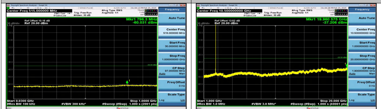
Band38_15MHz_QPSK_38000_1RB#0_30~1000_30~1000
