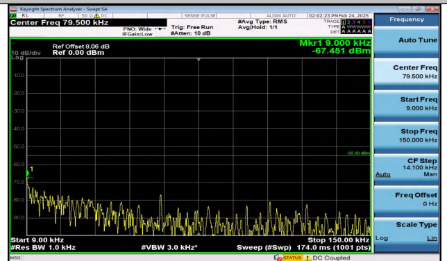
Band38_15MHz_QPSK_37825_75RB#0_0.009~0.15_0.00 9~0.15
