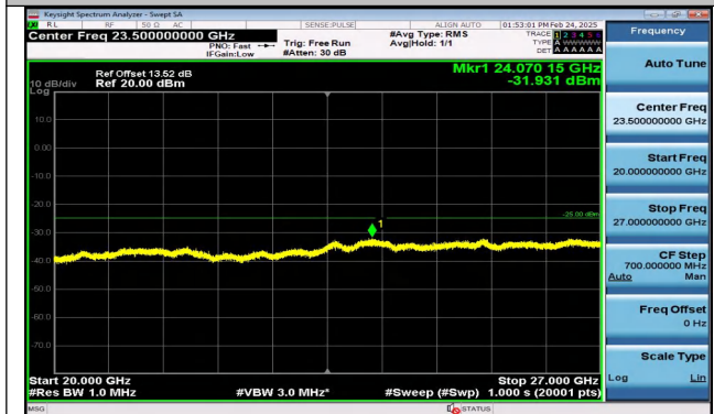
Band38_15MHz_QPSK_37825_1RB#74_20000~27000_2 0000~27000
