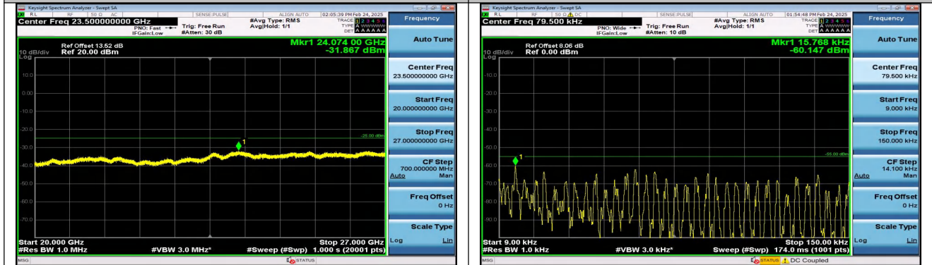
Band38_15MHz_QPSK_38000_75RB#0_20000~27000_20000~27000
