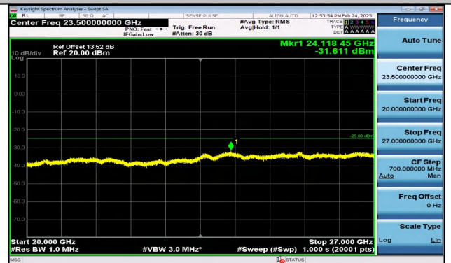
Band38_10MHz_QPSK_38200_1RB#49_20000~27000_2 0000~27000
