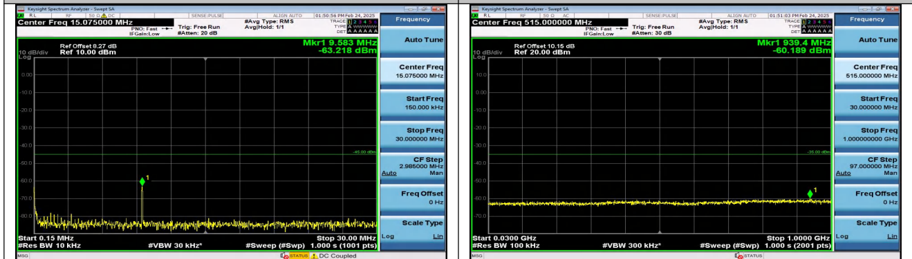
Band38_15MHz_QPSK_37825_1RB#0_0.15~30_0.15~30
