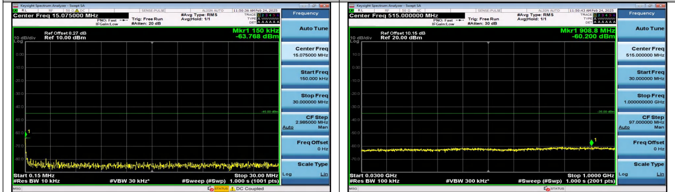
Band38_5MHz_QPSK_38000_1RB#24_30~1000_30~100 0
