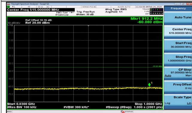
Band38_5MHz_QPSK_38225_1RB#0_30~1000_30~1000
