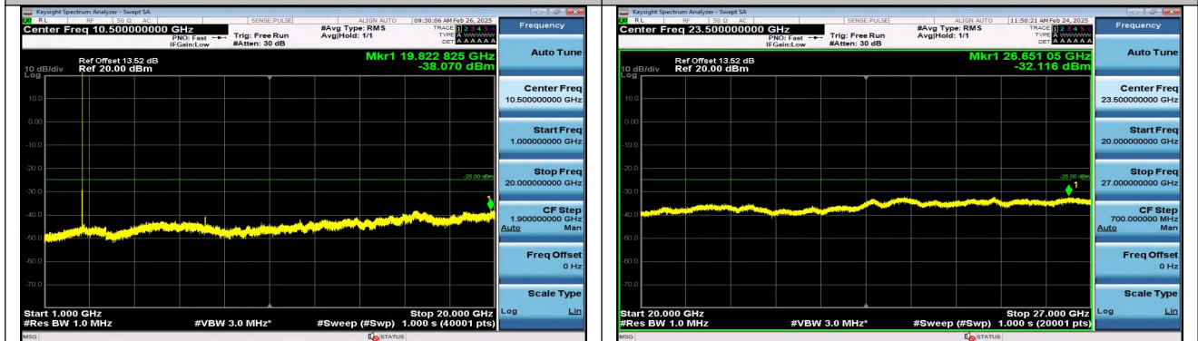
Band38_5MHz_16QAM_38000_1RB#0_1000~20000_1000~20000 0~20000
