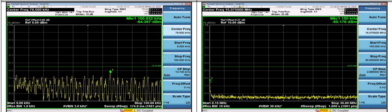
Band38_5MHz_16QAM_38225_1RB#24_0.009~0.15_0.009~0.15
