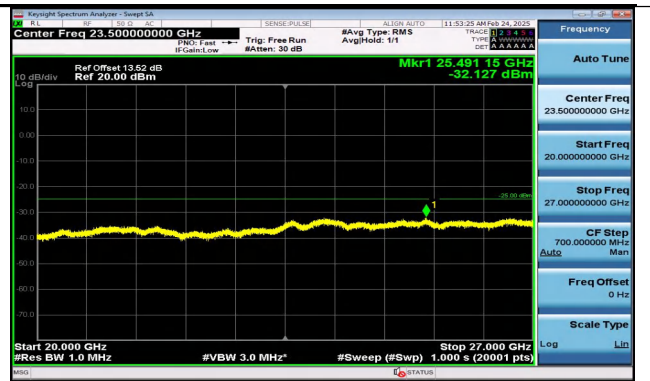
Band38_5MHz_16QAM_38000_25RB#0_20000~27000_20000~27000
