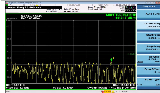
Band38_5MHz_QPSK_38225_1RB#0_0.009~0.15_0.009~0.15
