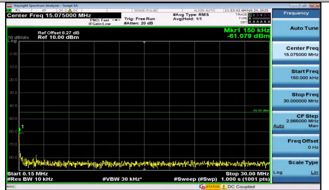
Band38_5MHz_QPSK_38225_1RB#0_0.15~30_0.15~30
