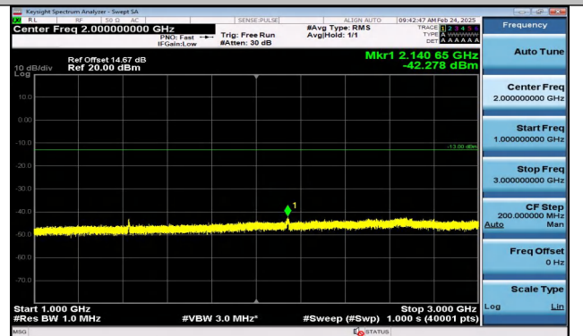
Band17_5MHz_QPSK_23825_25RB#0_1000~3000_1000 ~3000
