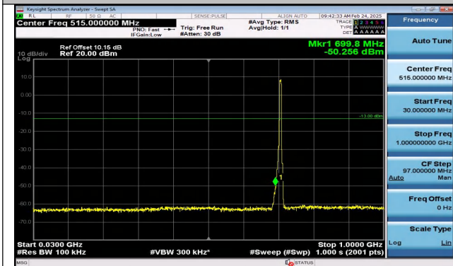
Band17_5MHz_QPSK_23825_25RB#0_30~1000_30~100 0
