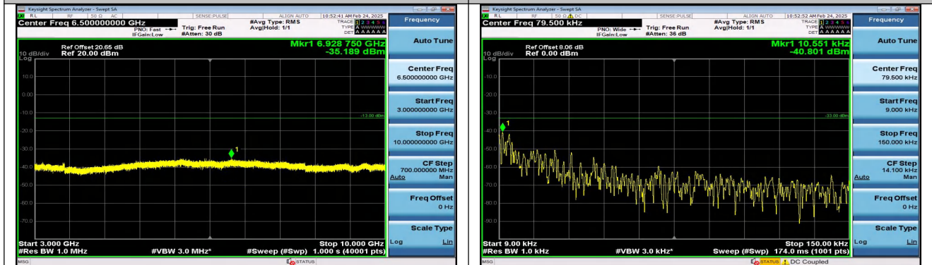
Band17_10MHz_16QAM_23780_1RB#49_3000~10000_3000~10000 000~10000
