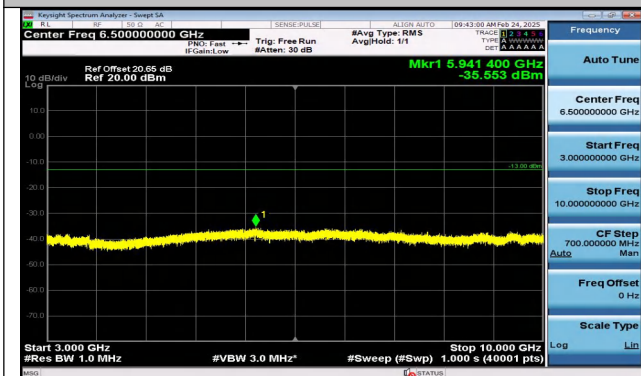
Band17_5MHz_QPSK_23825_25RB#0_3000~10000_300 0~10000
