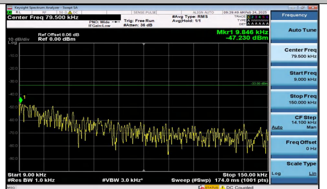
Band17_5MHz_16QAM_23825_1RB#0_0.009~0.15_0.009 ~0.15
