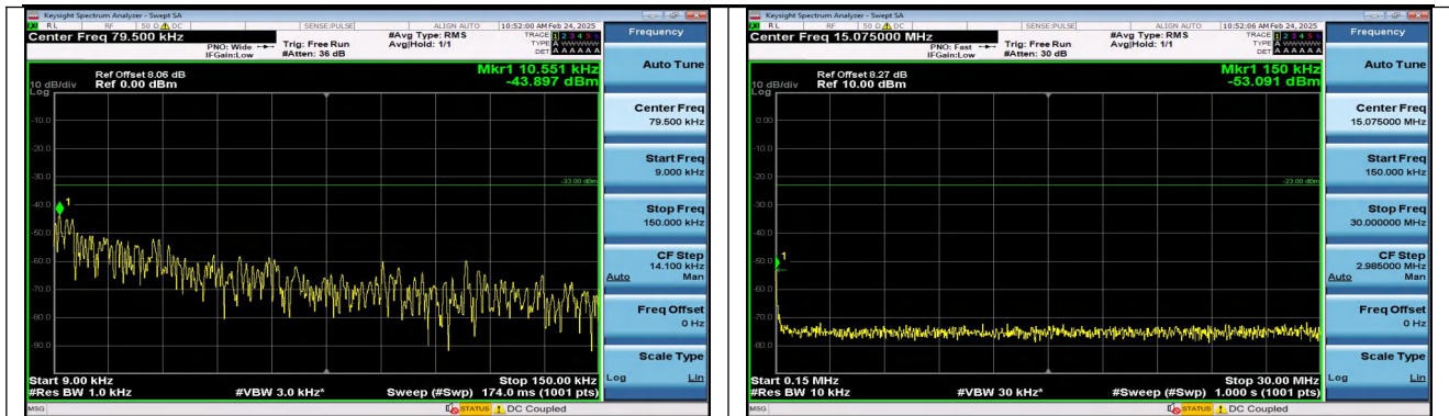
Band17_10MHz_16QAM_23780_1RB#49_0.009~0.15_0.0 09~0.15
