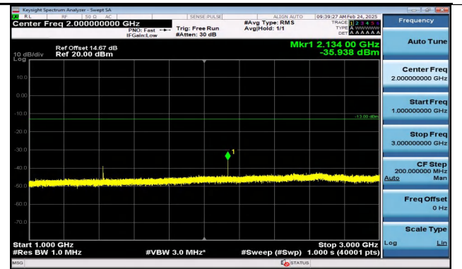
Band17_5MHz_QPSK_23825_1RB#0_1000~3000_1000~3000
