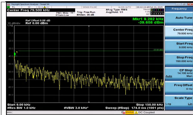
Band17_5MHz_QPSK_23825_25RB#0_0.009~0.15_0.009 ~0.15
