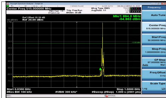
Band17_5MHz_QPSK_23825_1RB#0_30~1000_30~1000
