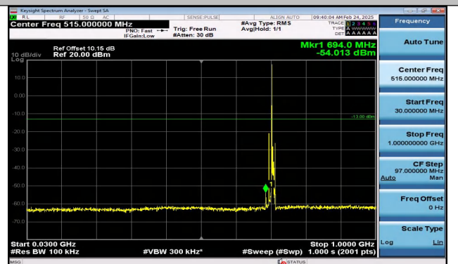
Band17_5MHz_16QAM_23825_1RB#0_30~1000_30~100 0
