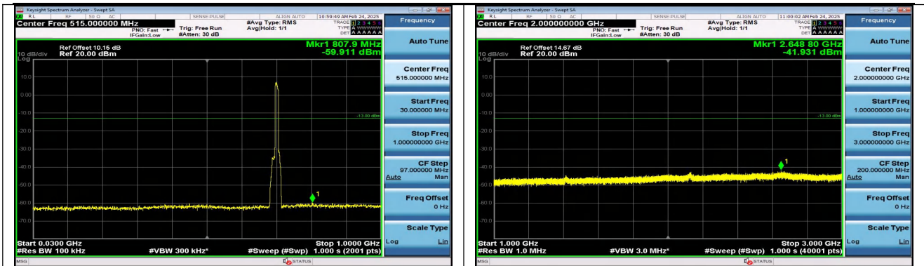
Band17_10MHz_QPSK_23780_50RB#0_30~1000_30~1000
