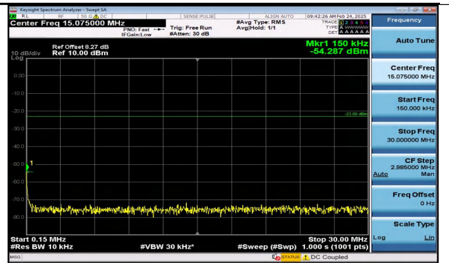
Band17_5MHz_QPSK_23825_25RB#0_0.15~30_0.15~30
