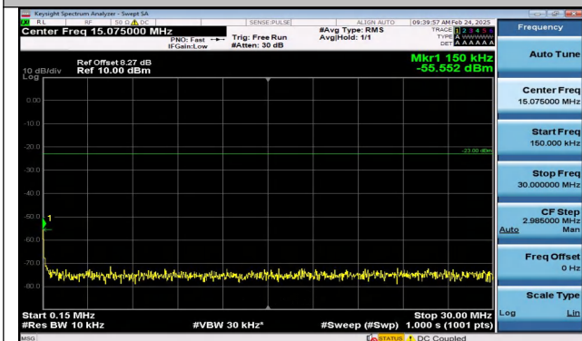
Band17_5MHz_16QAM_23825_1RB#0_0.15~30_0.15~30
