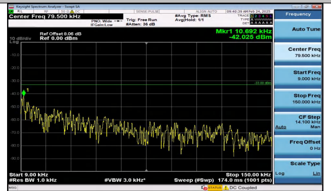
Band17_5MHz_QPSK_23825_1RB#24_0.009~0.15_0.009~0.15
