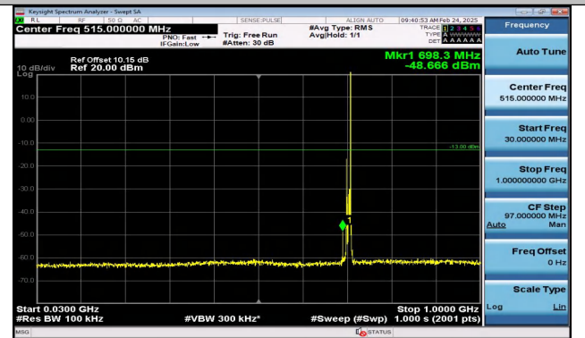
Band17_5MHz_QPSK_23825_1RB#24_30~1000_30~1000
