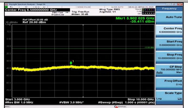
Band17_5MHz_QPSK_23825_1RB#24_3000~10000_3000~10000
