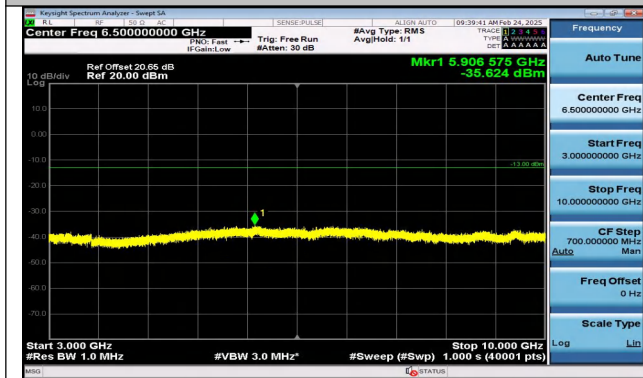
Band17_5MHz_QPSK_23825_1RB#0_3000~10000_3000~10000
