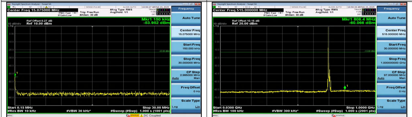
Band17_10MHz_16QAM_23780_1RB#0_0.15~30_0.15~30
