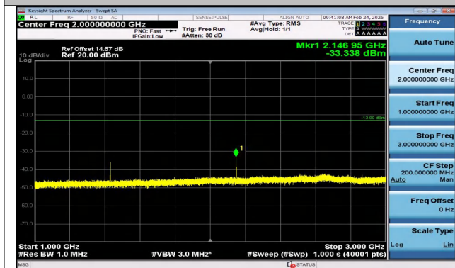
Band17_5MHz_QPSK_23825_1RB#24_1000~3000_1000~3000
