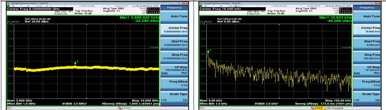
Band17_10MHz_QPSK_23780_50RB#0_3000~10000_3000~10000
