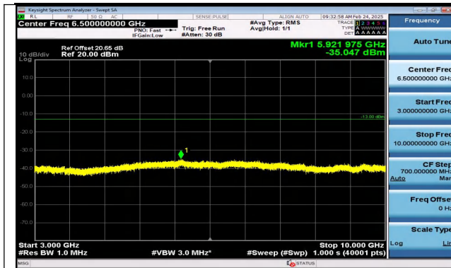
Band17_5MHz_QPSK_23755_25RB#0_3000~10000_300 0~10000
