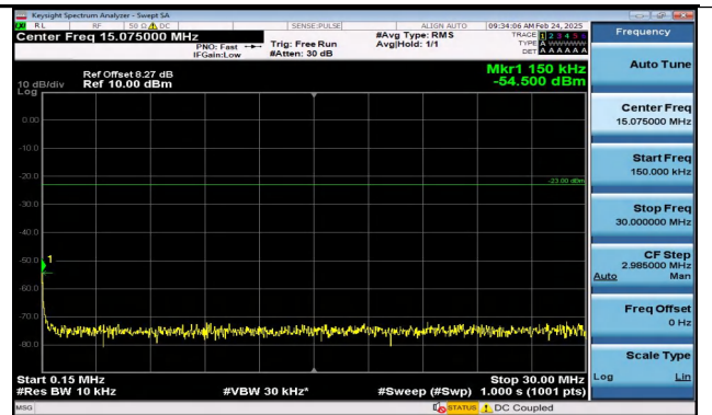
Band17_5MHz_QPSK_23790_1RB#0_0.15~30_0.15~30
