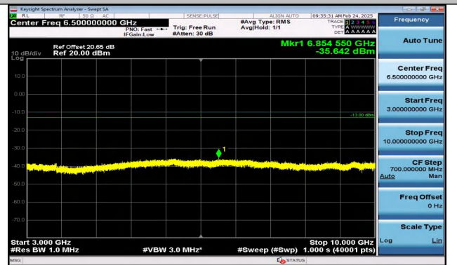
Band17_5MHz_16QAM_23790_1RB#0_3000~10000_3000~10000
