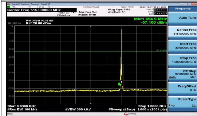
Band17_5MHz_16QAM_23790_1RB#24_30~1000_30~1000
