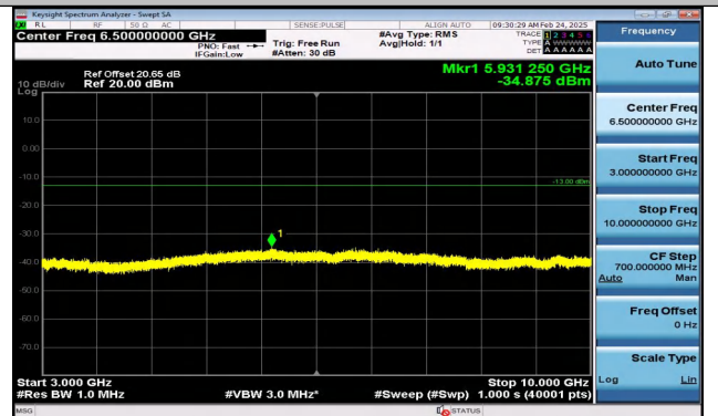
Band17_5MHz_16QAM_23755_1RB#0_3000~10000_300 0~10000
