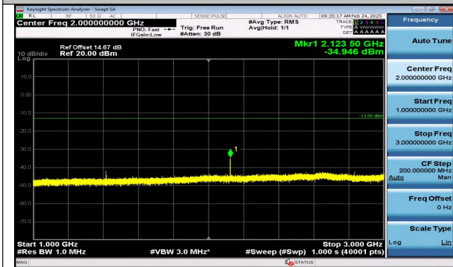
Band17_5MHz_16QAM_23790_1RB#0_1000~3000_1000~3000
