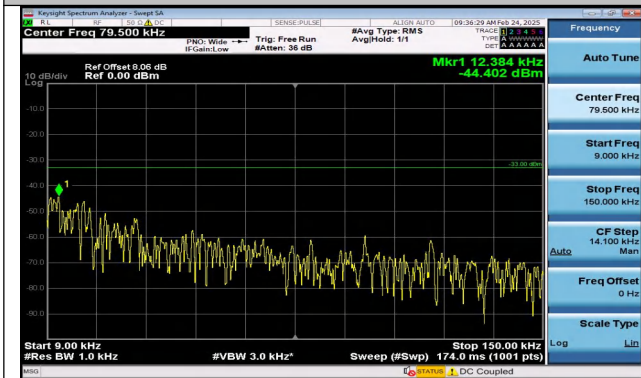
Band17_5MHz_16QAM_23790_1RB#24_0.009~0.15_0.009~0.15
