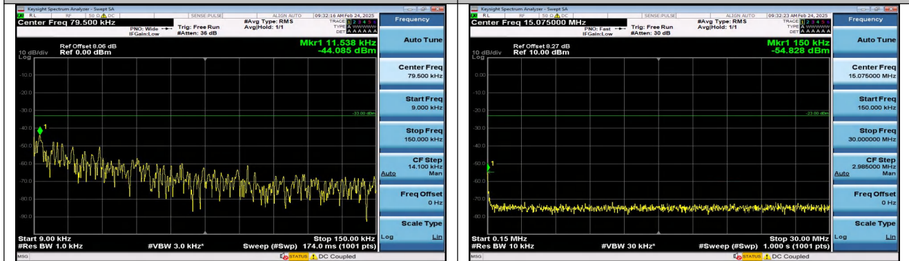
Band17_5MHz_QPSK_23755_25RB#0_0.009~0.15_0.009~0.15 ~0.15
