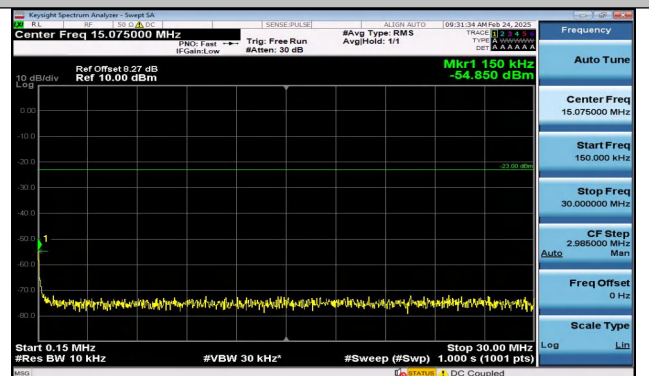
Band17_5MHz_16QAM_23755_1RB#24_0.15~30_0.15~3 0
