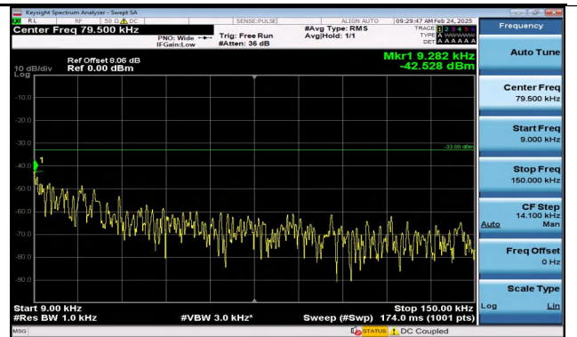
Band17_5MHz_16QAM_23755_1RB#0_0.009~0.15_0.009 ~0.15
