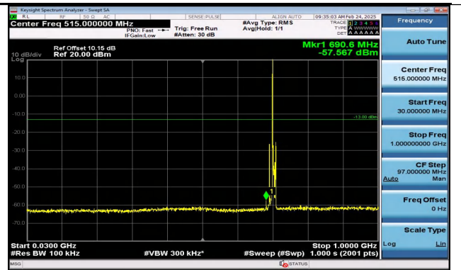
Band17_5MHz_16QAM_23790_1RB#0_30~1000_30~1000
