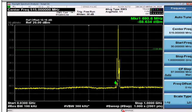
Band17_5MHz_QPSK_23790_1RB#0_30~1000_30~1000
