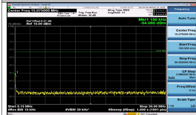
Band17_5MHz_QPSK_23790_1RB#24_0.15~30_0.15~30
