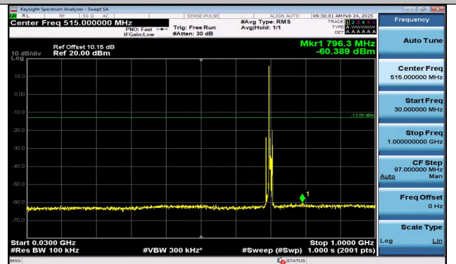
Band17_5MHz_16QAM_23755_1RB#0_30~1000_30~100 0
