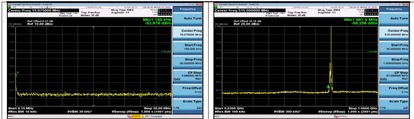
Band17_5MHz_QPSK_23755_1RB#24_30~1000_30~1000 0
