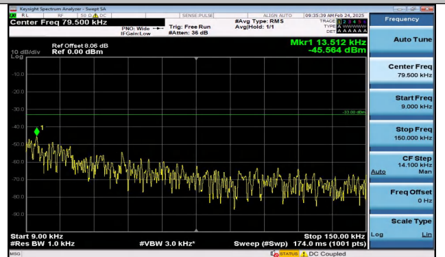
Band17_5MHz_QPSK_23790_1RB#24_0.009~0.15_0.009~0.15
