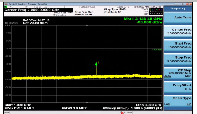
Band17_5MHz_QPSK_23790_1RB#0_1000~3000_1000~3000
