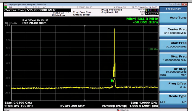
Band17_5MHz_QPSK_23790_1RB#24_30~1000_30~1000
