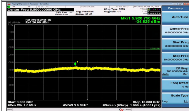
Band17_5MHz_QPSK_23790_1RB#0_3000~10000_3000~10000
