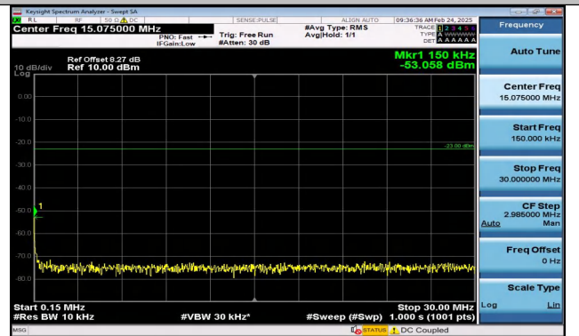
Band17_5MHz_16QAM_23790_1RB#24_0.15~30_0.15~30
