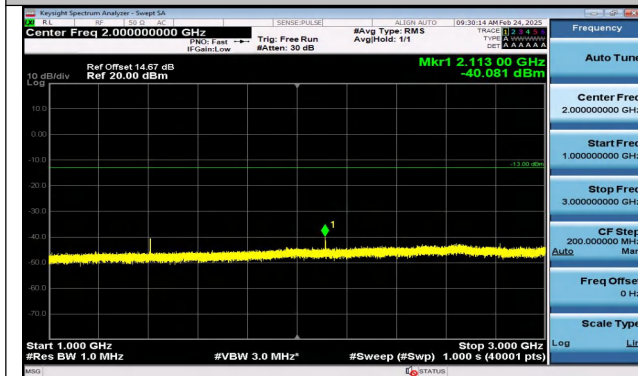
Band17_5MHz_16QAM_23755_1RB#0_1000~3000_1000 ~3000
