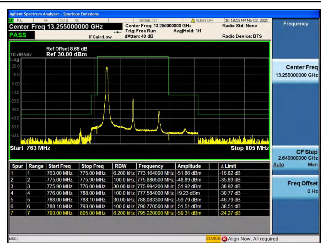
Band13_10MHz_16QAM_23230_1RB#0
