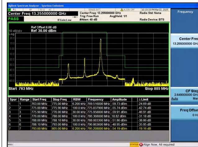
Band13_10MHz_16QAM_23230_1RB#49
