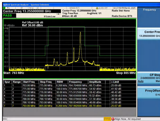
Band13_5MHz_16QAM_23255_1RB#24
