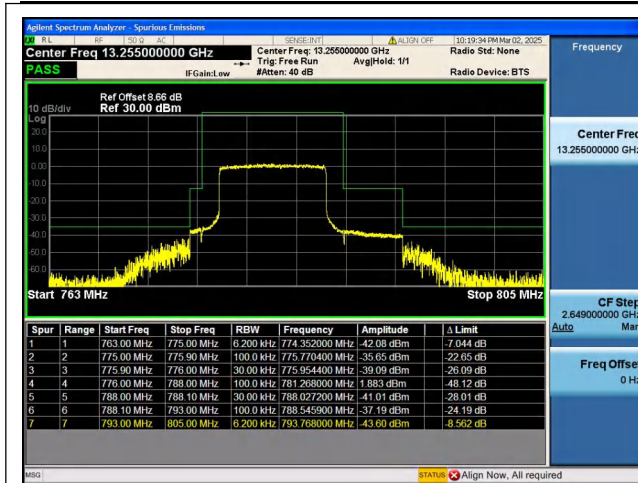
Band13_10MHz_QPSK_23230_50RB#0
