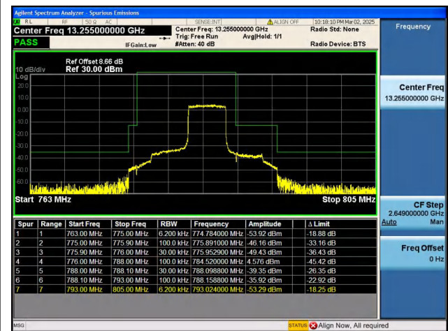
Band13_5MHz_QPSK_23255_25RB#0
