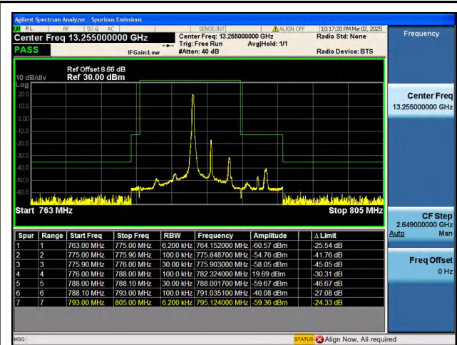
Band13_5MHz_QPSK_23255_1RB#0
