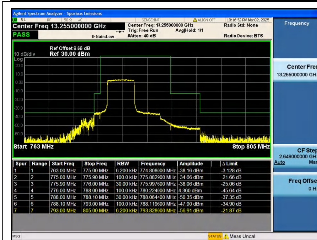
Band13_5MHz_QPSK_23205_25RB#0
