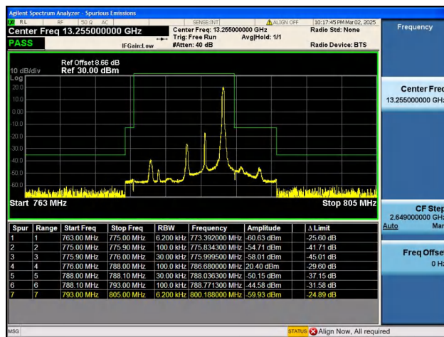
Band13_5MHz_QPSK_23255_1RB#24
