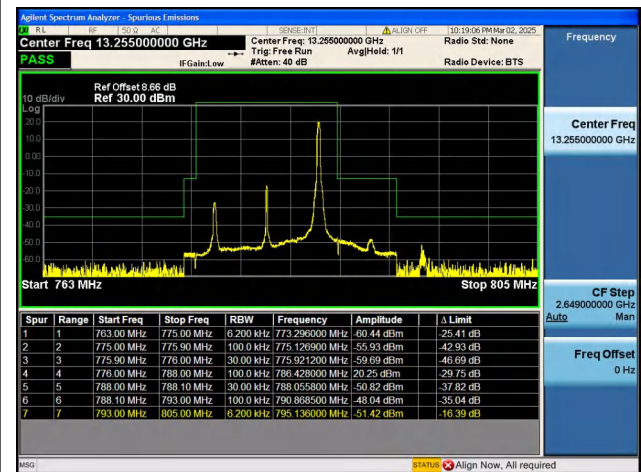
Band13_10MHz_QPSK_23230_1RB#49
