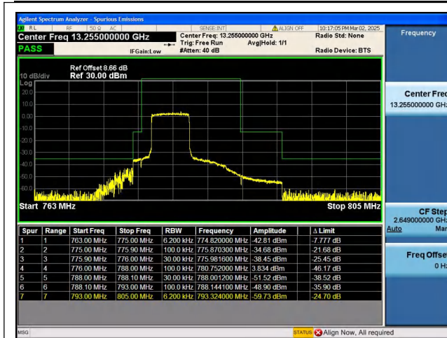
Band13_5MHz_16QAM_23205_25RB#0
