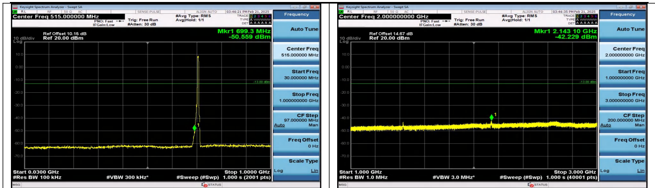
Band12_5MHz_QPSK_23155_25RB#0_30~1000_30~1000 0
