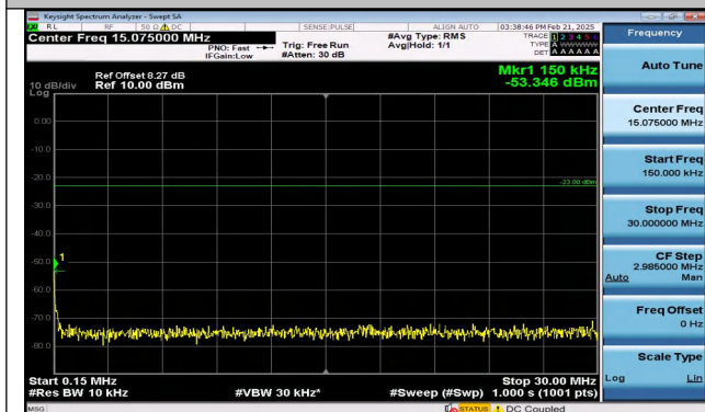
Band12_5MHz_16QAM_23095_1RB#0_0.15~30_0.15~30
