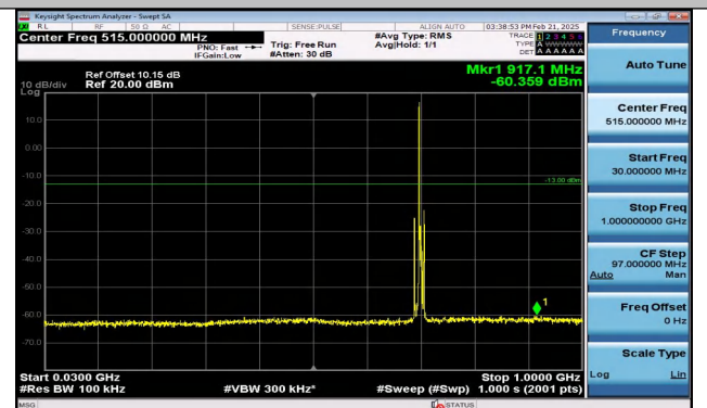
Band12_5MHz_16QAM_23095_1RB#0_30~1000_30~100 0
