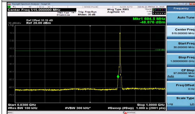
Band12_5MHz_QPSK_23095_25RB#0_30~1000_30~100 0
