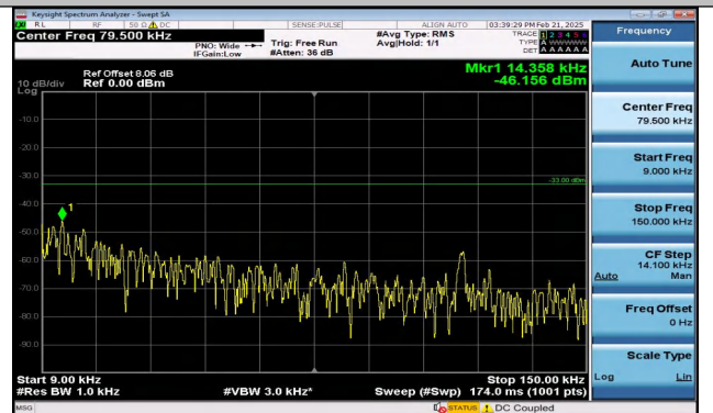
Band12_5MHz_QPSK_23095_1RB#24_0.009~0.15_0.009~0.15
