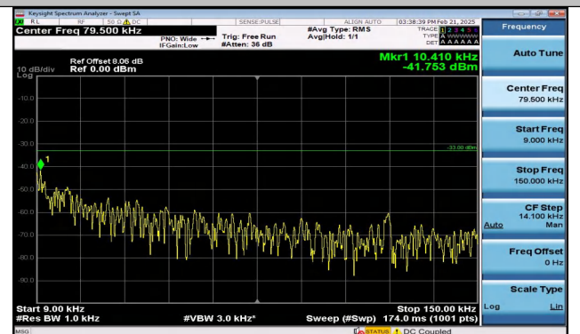
Band12_5MHz_16QAM_23095_1RB#0_0.009~0.15_0.009 ~0.15
