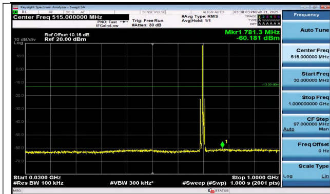
Band12_5MHz_QPSK_23095_1RB#0_30~1000_30~1000
