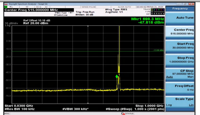
Band12_5MHz_QPSK_23155_1RB#24_30~1000_30~1000 0
