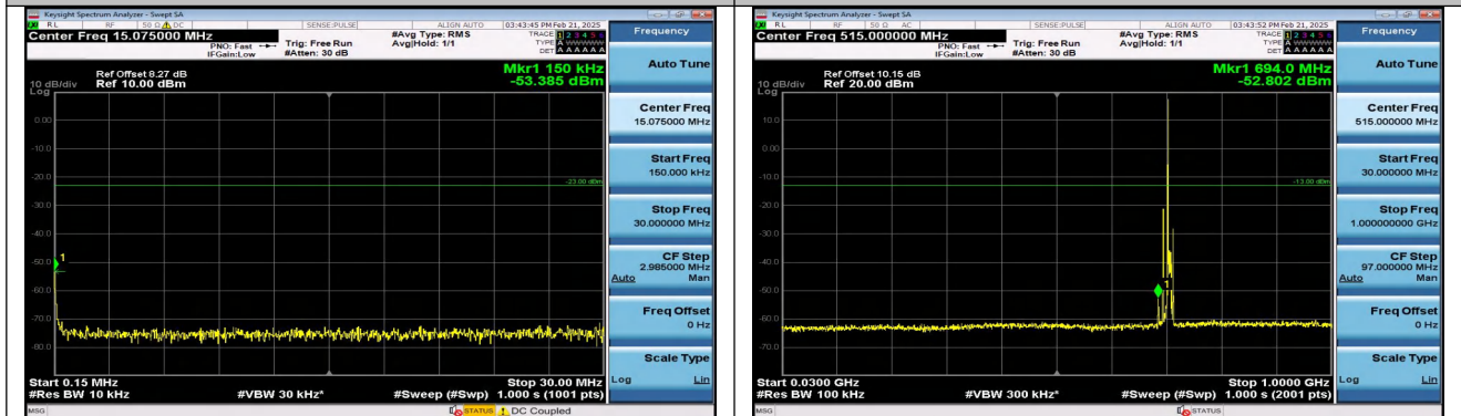
Band12_5MHz_16QAM_23155_1RB#0_0.15~30_0.15~30 0
