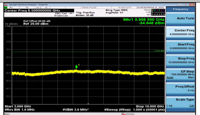
Band12_5MHz_QPSK_23095_1RB#24_3000~10000_3000~10000
