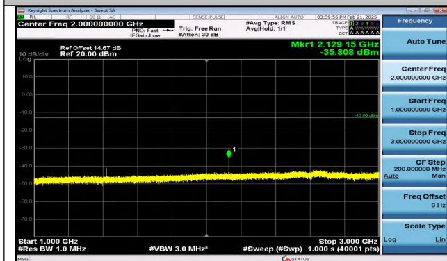
Band12_5MHz_QPSK_23095_1RB#24_1000~3000_1000~3000
