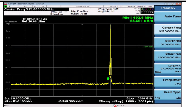
Band12_5MHz_QPSK_23095_1RB#24_30~1000_30~1000
