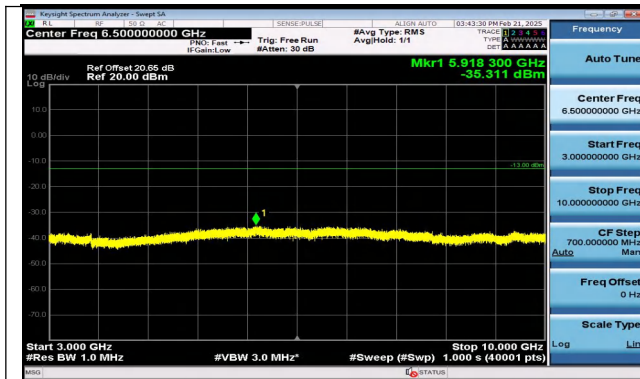
Band12_5MHz_QPSK_23155_1RB#0_3000~10000_3000 ~10000
