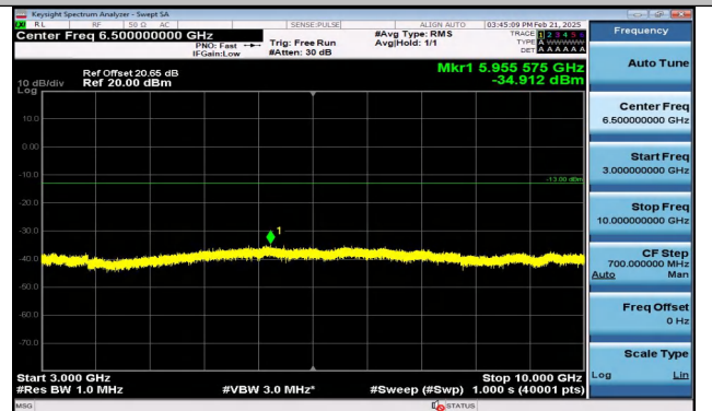
Band12_5MHz_QPSK_23155_1RB#24_3000~10000_300 0~10000
