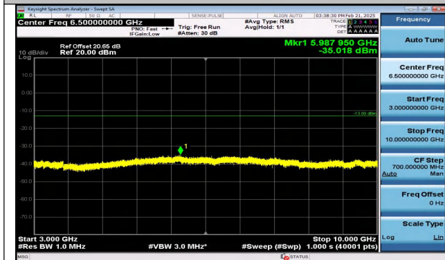
Band12_5MHz_QPSK_23095_1RB#0_3000~10000_3000~10000
