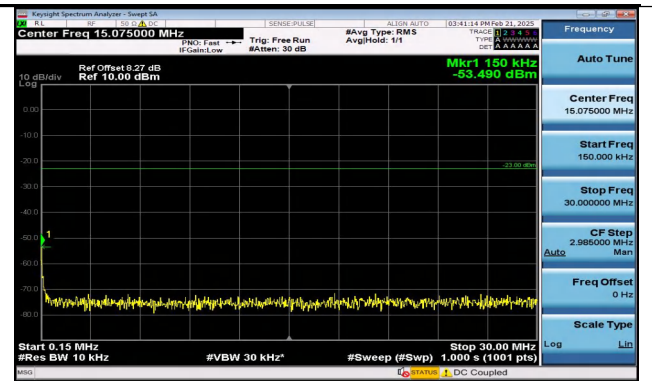
Band12_5MHz_QPSK_23095_25RB#0_0.15~30_0.15~30
