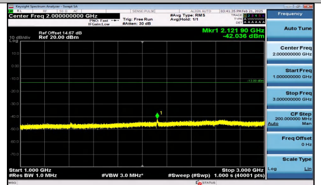
Band12_5MHz_QPSK_23095_25RB#0_1000~3000_1000 ~3000
