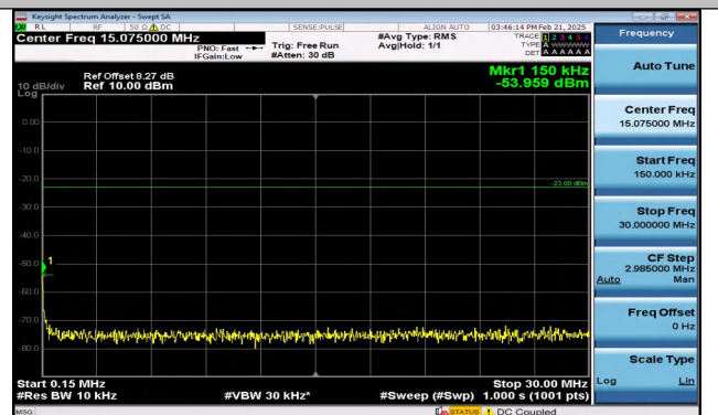
Band12_5MHz_QPSK_23155_25RB#0_0.15~30_0.15~30
