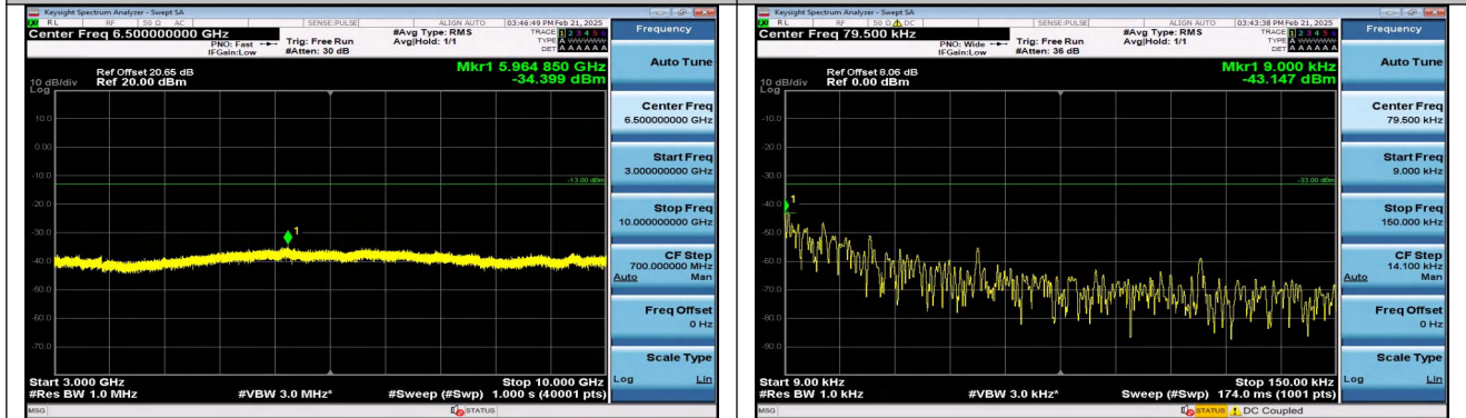
Band12_5MHz_QPSK_23155_25RB#0_3000~10000_3000~10000 0~10000
