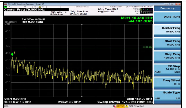
Band12_5MHz_QPSK_23155_1RB#24_0.009~0.15_0.009 ~0.15
