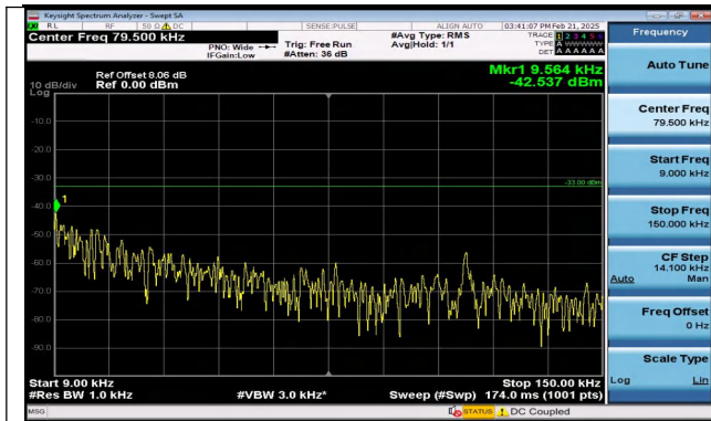
Band12_5MHz_QPSK_23095_25RB#0_0.009~0.15_0.009 ~0.15
