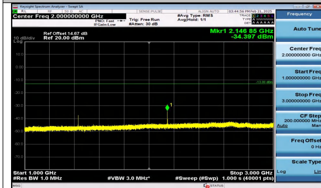
Band12_5MHz_QPSK_23155_1RB#24_1000~3000_1000 ~3000
