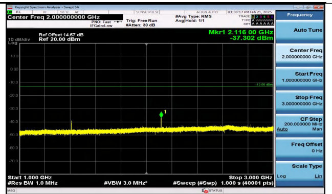
Band12_5MHz_QPSK_23095_1RB#0_1000~3000_1000~3000
