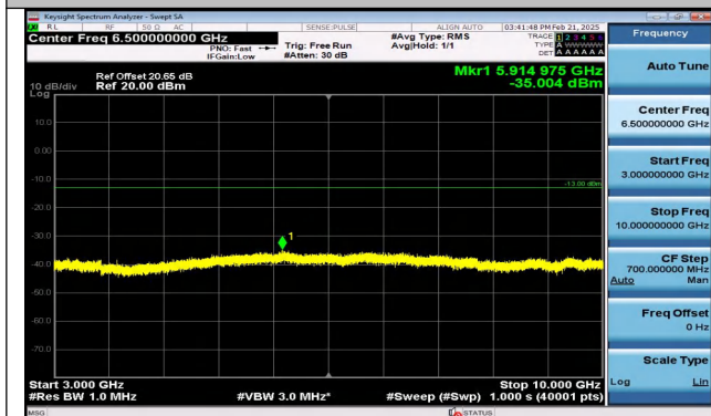
Band12_5MHz_QPSK_23095_25RB#0_3000~10000_300 0~10000
