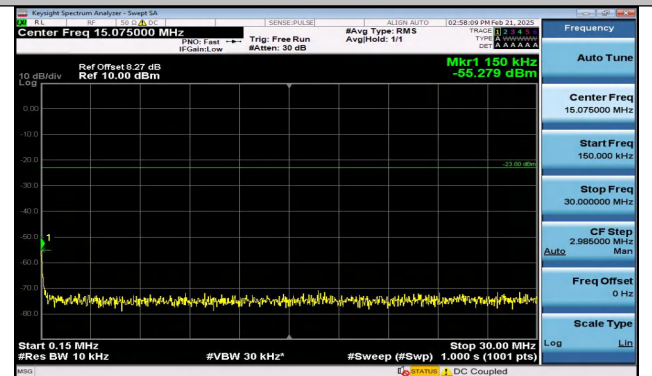
Band12_3MHz_QPSK_23095_15RB#0_0.15~30_0.15~30
