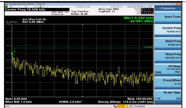
Band12_3MHz_QPSK_23095_1RB#14_0.009~0.15_0.009 ~0.15
