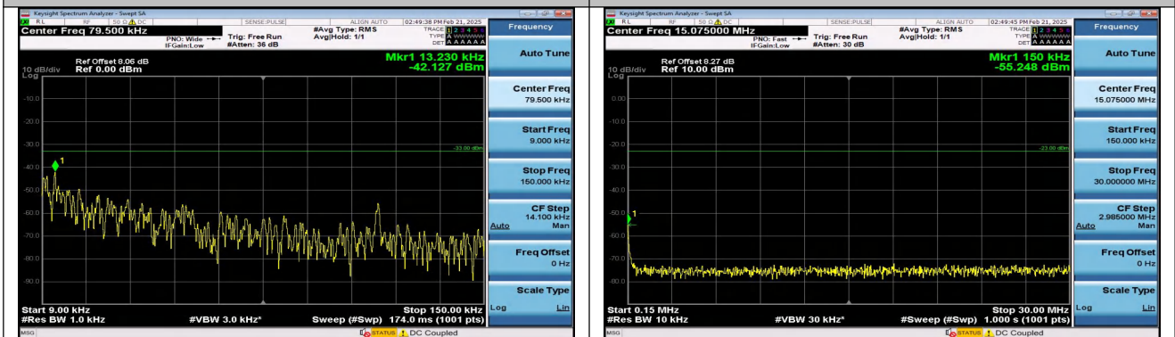
Band12_3MHz_QPSK_23025_1RB#0_0.009~0.15_0.009~0.15 0.15
