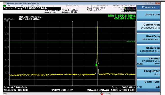
Band12_3MHz_16QAM_23095_15RB#0_30~1000_30~10 00
