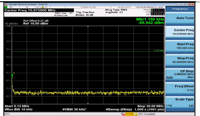
Band12_3MHz_QPSK_23025_15RB#0_0.15~30_0.15~30
