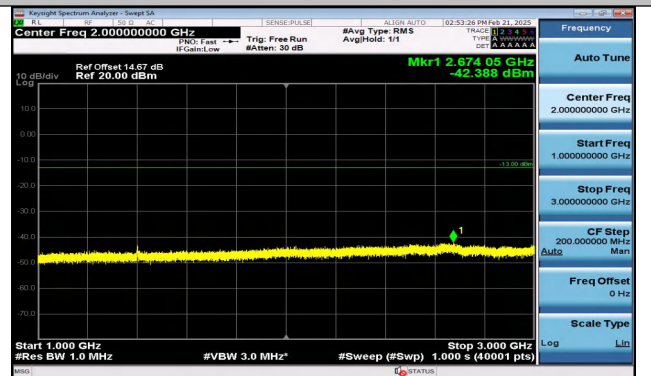
Band12_3MHz_QPSK_23025_15RB#0_1000~3000_1000 ~3000
