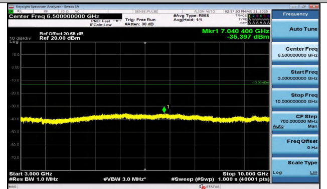
Band12_3MHz_QPSK_23095_1RB#14_3000~10000_300 0~10000
