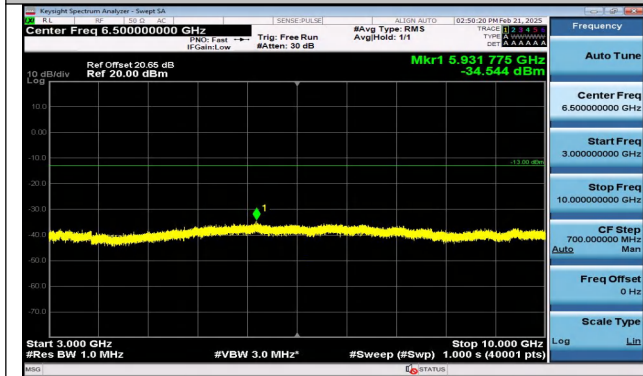
Band12_3MHz_QPSK_23025_1RB#0_3000~10000_3000
