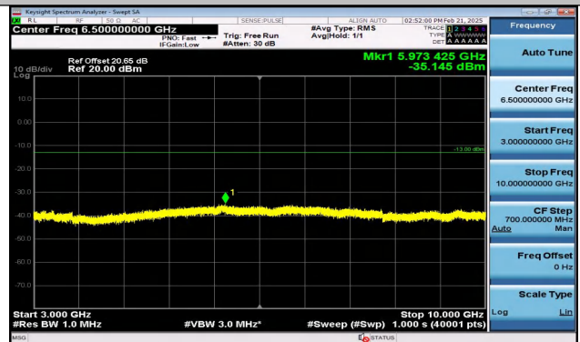
Band12_3MHz_QPSK_23025_1RB#14_3000~10000_3000
