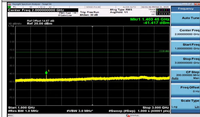
Band12_3MHz_QPSK_23025_1RB#14_1000~3000_1000
