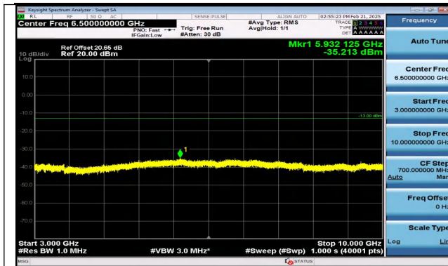
Band12_3MHz_QPSK_23095_1RB#0_3000~10000_3000 ~10000
