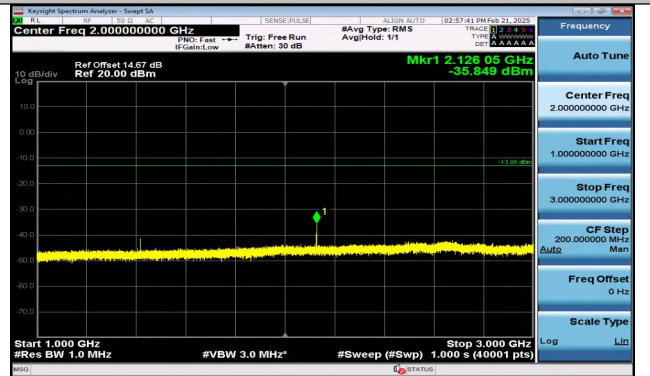
Band12_3MHz_16QAM_23095_1RB#14_1000~3000_100 0~3000
