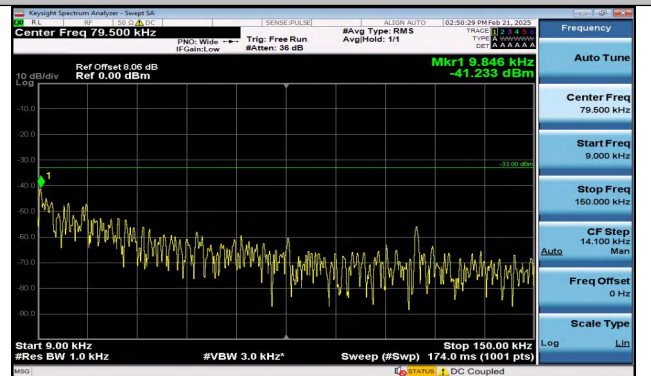
Band12_3MHz_16QAM_23025_1RB#0_0.009~0.15_0.009 ~0.15
