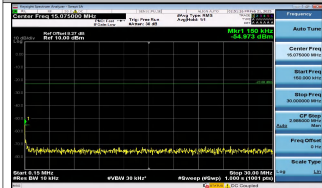
Band12_3MHz_QPSK_23025_1RB#14_0.15~30_0.15~30
