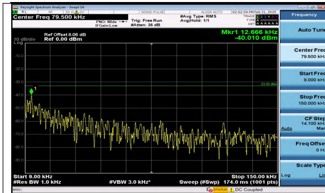
Band12_3MHz_QPSK_23025_15RB#0_0.009~0.15_0.009 ~0.15
