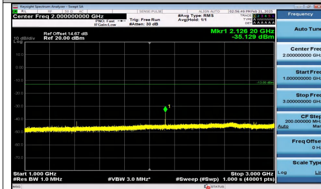
Band12_3MHz_QPSK_23095_1RB#14_1000~3000_1000 ~3000
