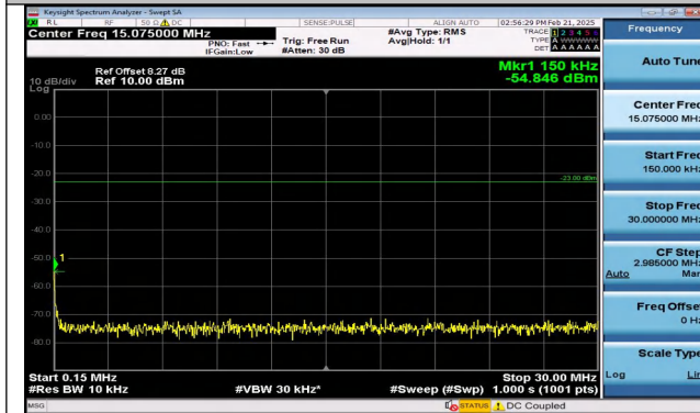
Band12_3MHz_QPSK_23095_1RB#14_0.15~30_0.15~30
