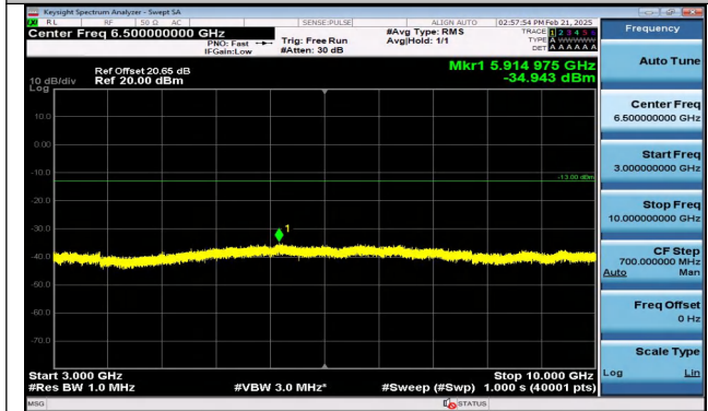
Band12_3MHz_16QAM_23095_1RB#14_3000~10000_30 00~10000
