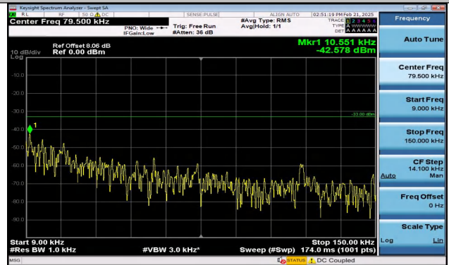
Band12_3MHz_QPSK_23025_1RB#14_0.009~0.15_0.009
