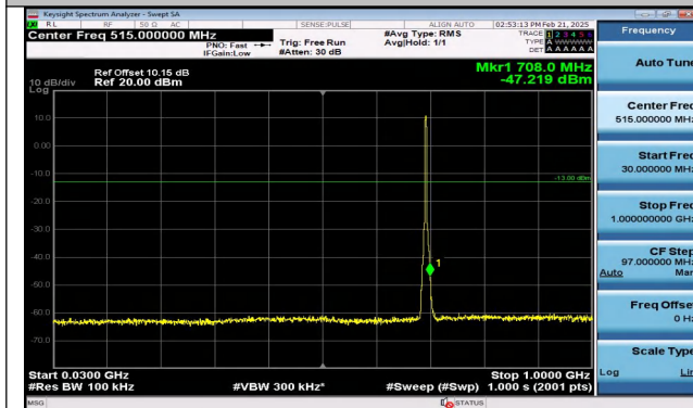
Band12_3MHz_QPSK_23025_15RB#0_30~1000_30~100 0
