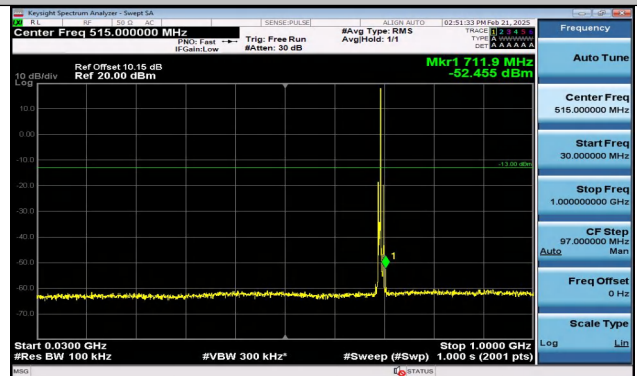
Band12_3MHz_QPSK_23025_1RB#14_30~1000_30~1000
