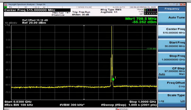
Band12_3MHz_16QAM_23025_1RB#0_30~1000_30~100 0
