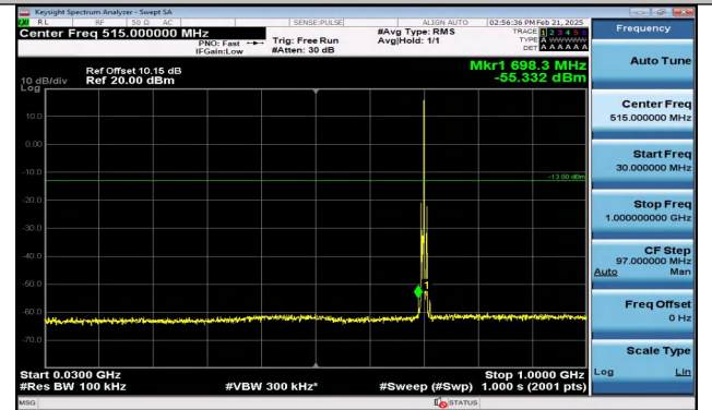
Band12_3MHz_QPSK_23095_1RB#14_30~1000_30~1000 0
