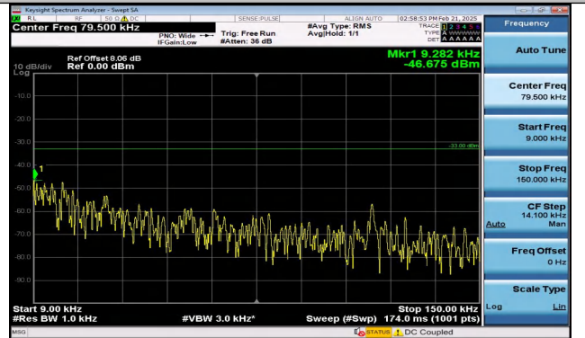
Band12_3MHz_16QAM_23095_15RB#0_0.009~0.15_0.00 9~0.15
