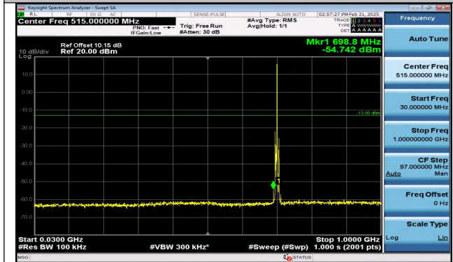
Band12_3MHz_16QAM_23095_1RB#14_30~1000_30~10 00
