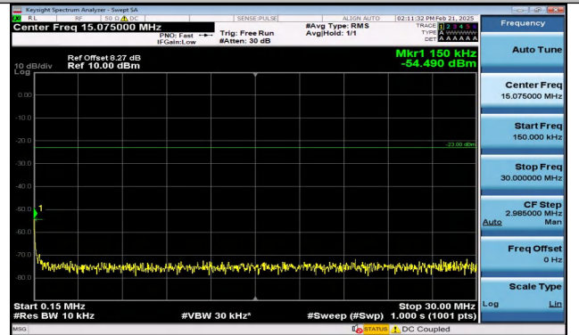
Band12_1.4MHz_QPSK_23095_6RB#0_0.15~30_0.15~30
