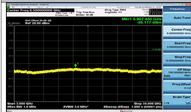
Band12_1.4MHz_QPSK_23095_1RB#0_3000~10000_300 0~10000
