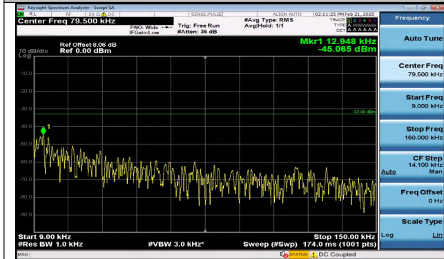
Band12_1.4MHz_QPSK_23095_6RB#0_0.009~0.15_0.009~0.15
