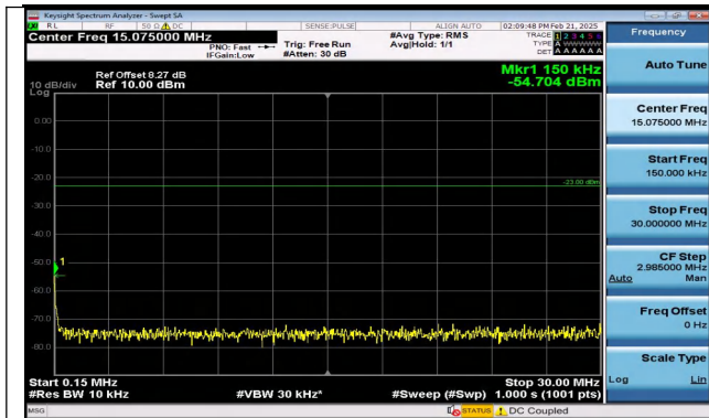
Band12_1.4MHz_QPSK_23095_1RB#5_0.15~30_0.15~30
