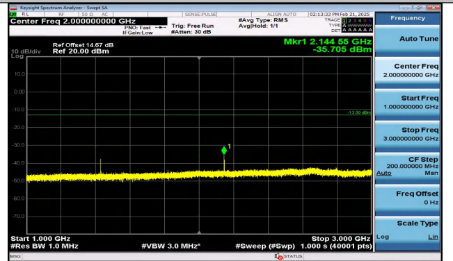
Band12_1.4MHz_QPSK_23173_1RB#0_1000~3000_1000 ~3000
