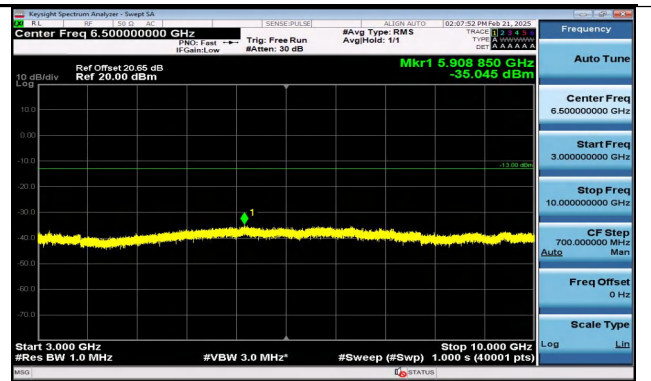
Band12_1.4MHz_16QAM_23017_6RB#0_3000~10000_30 00~10000
