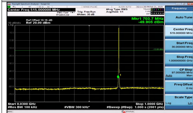
Band12_1.4MHz_QPSK_23095_6RB#0_30~1000_30~1000
