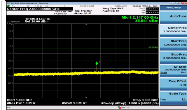
Band12_1.4MHz_QPSK_23173_1RB#5_1000~3000_1000 ~3000
