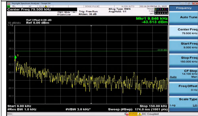
Band12_1.4MHz_QPSK_23173_6RB#0_0.009~0.15_0.00 9~0.15
