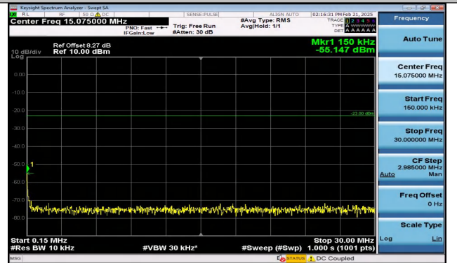
Band12_1.4MHz_QPSK_23173_6RB#0_0.15~30_0.15~30
