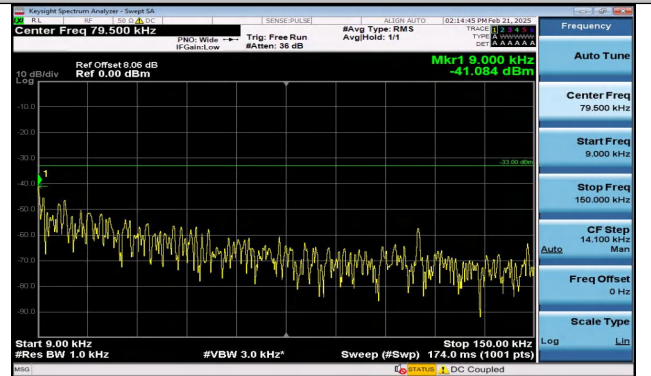
Band12_1.4MHz_QPSK_23173_1RB#5_0.009~0.15_0.00 9~0.15
