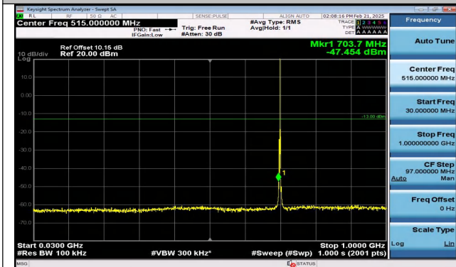
Band12_1.4MHz_QPSK_23095_1RB#0_30~1000_30~100 0
