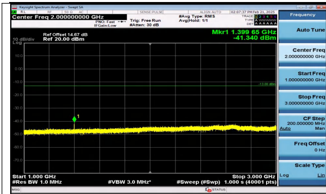
Band12_1.4MHz_16QAM_23017_6RB#0_1000~3000_100 0~3000
