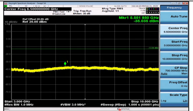
Band12_1.4MHz_QPSK_23095_1RB#5_3000~10000_3000~10000
