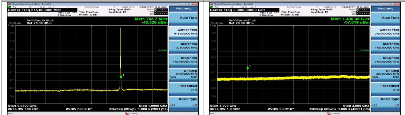
Band12_1.4MHz_16QAM_23017_1RB#5_30~1000_30~1000
