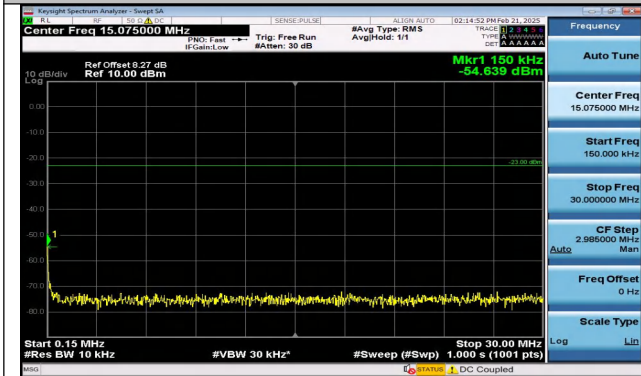
Band12_1.4MHz_QPSK_23173_1RB#5_0.15~30_0.15~30
