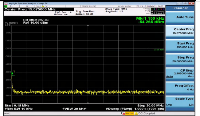
Band12_1.4MHz_QPSK_23173_1RB#0_0.15~30_0.15~30
