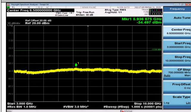
Band12_1.4MHz_QPSK_23173_6RB#0_3000~10000_300 0~10000
