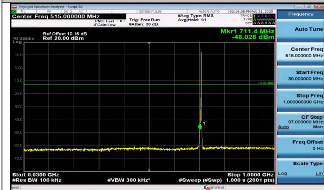
Band12_1.4MHz_QPSK_23173_6RB#0_30~1000_30~100 0
