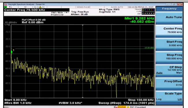
Band12_1.4MHz_16QAM_23173_1RB#0_0.009~0.15_0.0 09~0.15
