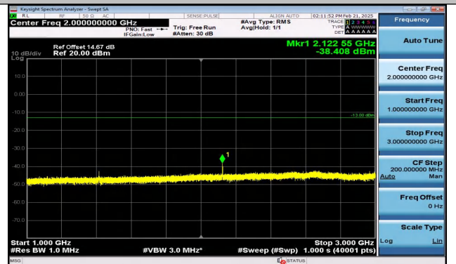
Band12_1.4MHz_QPSK_23095_6RB#0_1000~3000_1000~3000
