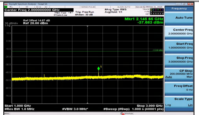
Band12_1.4MHz_QPSK_23173_6RB#0_1000~3000_1000 ~3000
