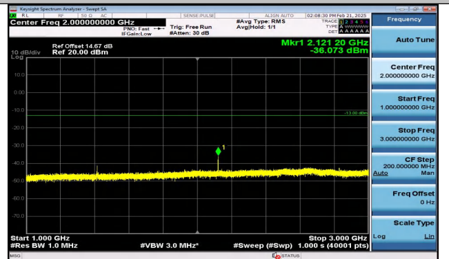
Band12_1.4MHz_QPSK_23095_1RB#0_1000~3000_1000 ~3000
