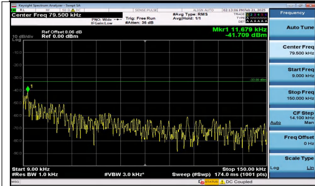
Band12_1.4MHz_QPSK_23173_1RB#0_0.009~0.15_0.00 9~0.15
