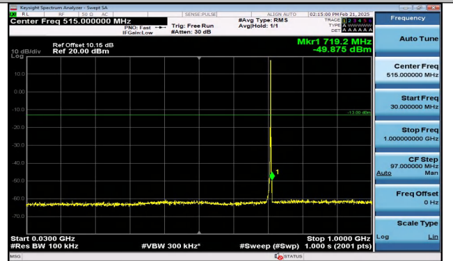
Band12_1.4MHz_QPSK_23173_1RB#5_30~1000_30~100 0
