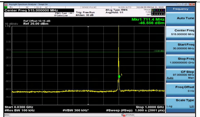
Band12_1.4MHz_QPSK_23095_1RB#5_30~1000_30~1000
