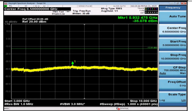
Band12_1.4MHz_QPSK_23173_1RB#5_3000~10000_300 0~10000
