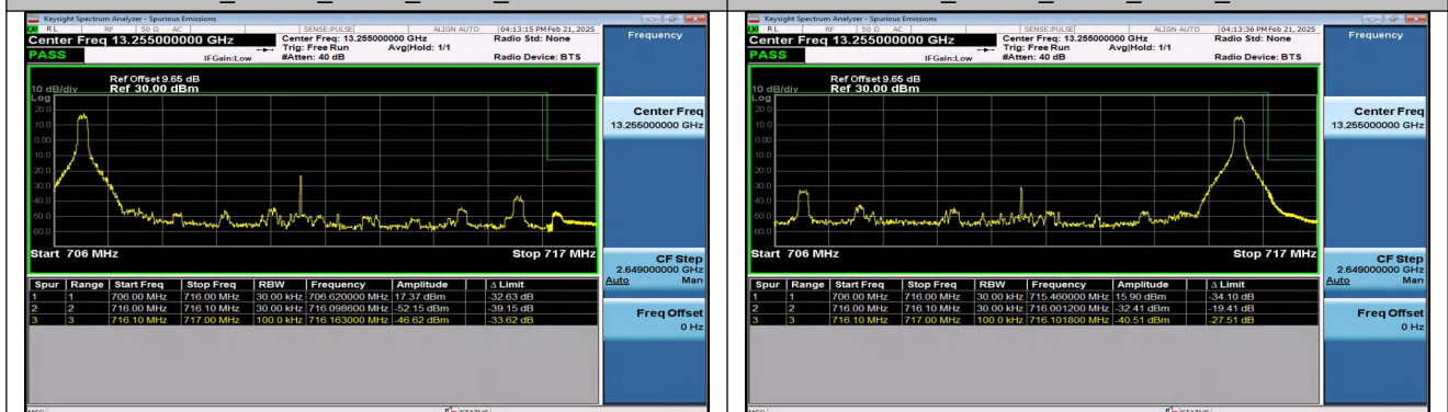
Band12_10MHz_16QAM_23130_1RB#0
