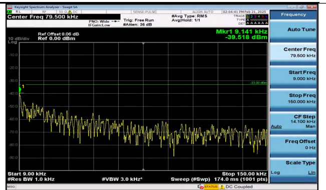
Band12_1.4MHz_QPSK_23017_1RB#5_0.009~0.15_0.00 9~0.15
