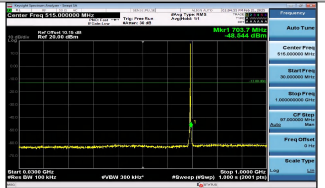
Band12_1.4MHz_QPSK_23017_1RB#5_30~1000_30~100 0
