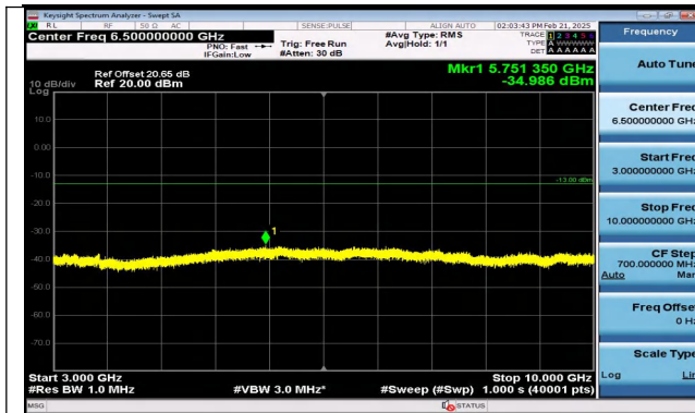
Band12_1.4MHz_QPSK_23017_1RB#0_3000~10000_300 0~10000
