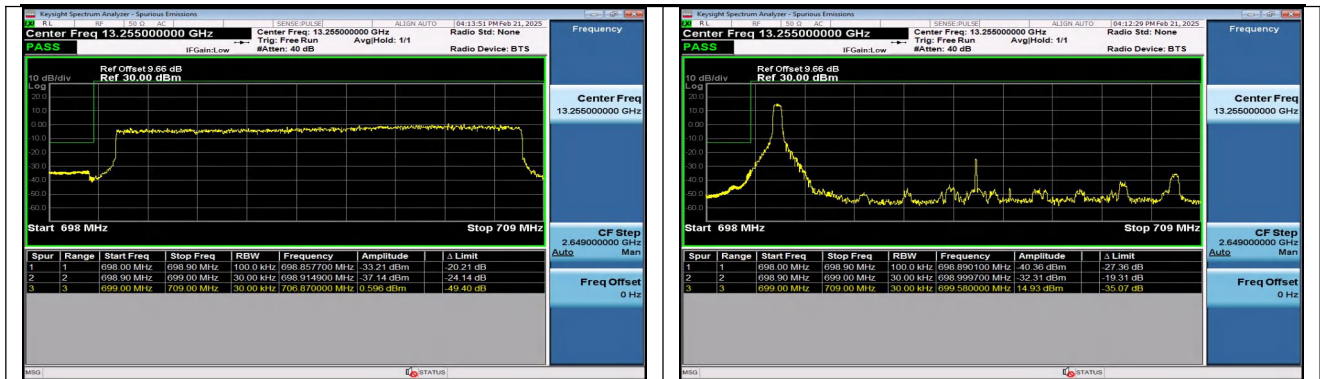
Band12_10MHz_QPSK_23060_50RB#0
