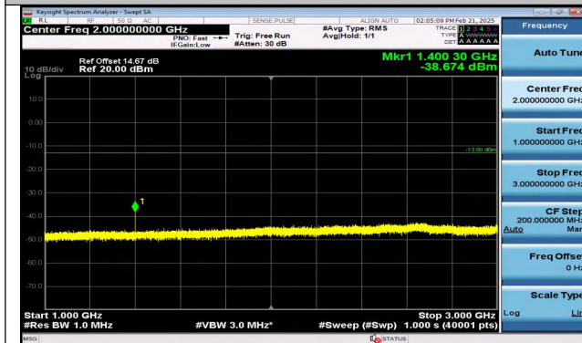
Band12_1.4MHz_QPSK_23017_1RB#5_1000~3000_1000 ~3000
