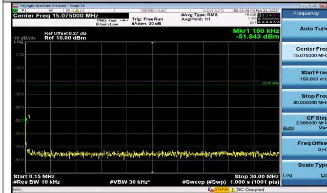
Band12_1.4MHz_QPSK_23017_1RB#5_0.15~30_0.15~30
