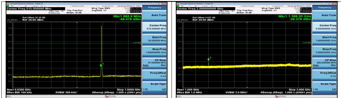
Band12_1.4MHz_QPSK_23017_6RB#0_30~1000_30~1000 0
