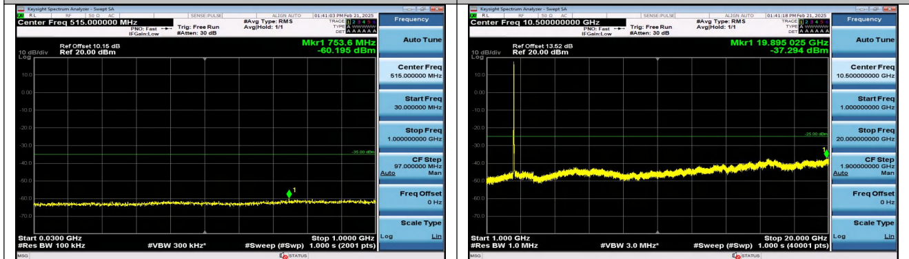
Band7_20MHz_QPSK_20850_100RB#0_30~1000_30~10 00
