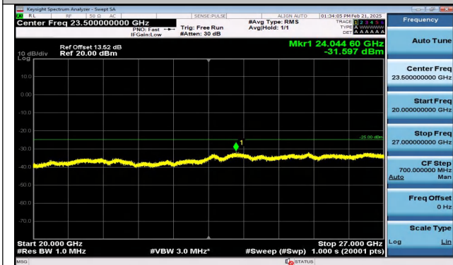
Band7_20MHz_16QAM_20850_1RB#99_20000~27000_2 0000~27000
