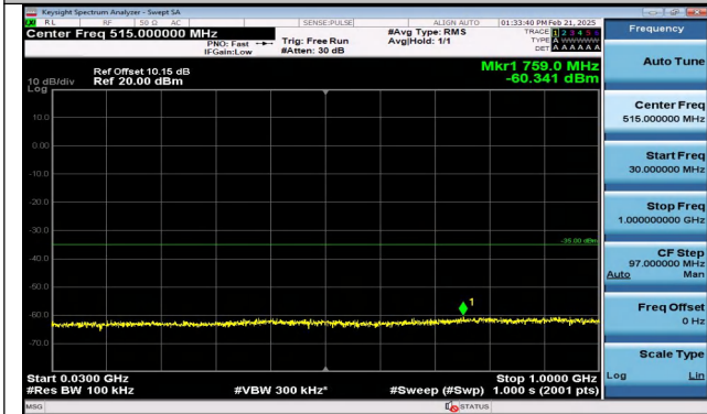
Band7_20MHz_16QAM_20850_1RB#99_30~1000_30~10 00
