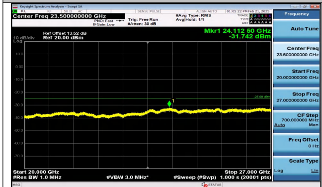
Band7_15MHz_16QAM_21100_1RB#74_20000~27000_2 0000~27000
