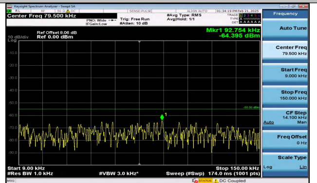
Band7_20MHz_QPSK_21100_1RB#0_0.009~0.15_0.009~ 0.15
