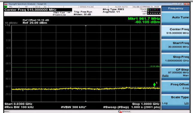
Band7_15MHz_QPSK_21375_1RB#0_30~1000_30~1000
