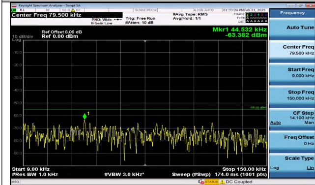
Band7_20MHz_16QAM_20850_1RB#99_0.009~0.15_0.00 9~0.15
