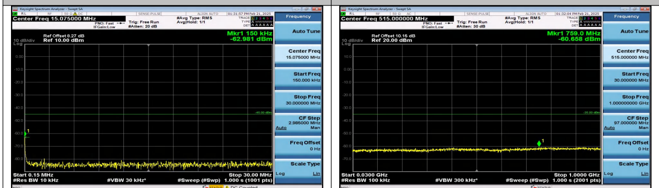
Band7_20MHz_16QAM_20850_1RB#0_0.15~30_0.15~30 0
