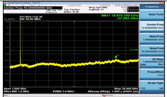
Band7_15MHz_16QAM_21100_1RB#74_1000~20000_10 00~20000
