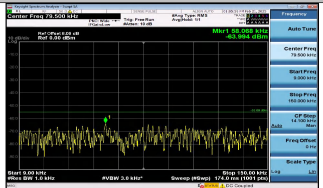
Band7_15MHz_QPSK_21375_1RB#0_0.009~0.15_0.009~ 0.15
