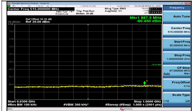
Band7_15MHz_16QAM_21100_1RB#74_30~1000_30~10 00
