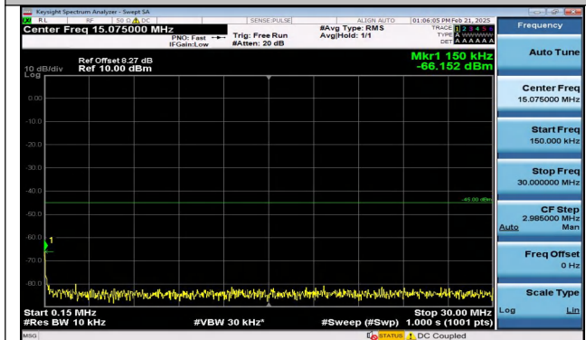
Band7_15MHz_QPSK_21375_1RB#0_0.15~30_0.15~30
