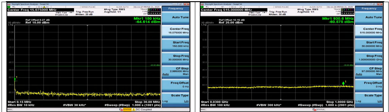
Band7_15MHz_QPSK_21375_75RB#0_30~1000_30~1000
