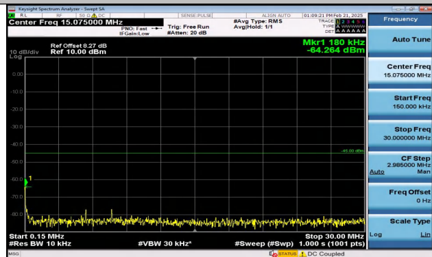
Band7_15MHz_QPSK_20825_75RB#0_0.15~30_0.15~30
