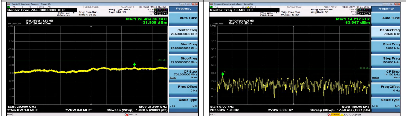
Band7_15MHz_16QAM_20825_1RB#0_20000~27000_20 000~27000
