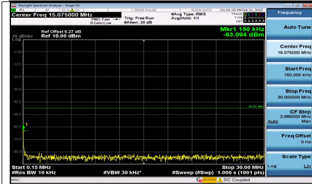
Band7_15MHz_16QAM_20825_1RB#74_0.15~30_0.15~3 0
