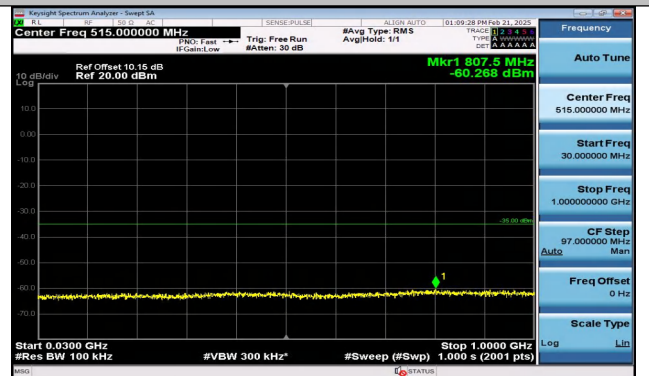
Band7_15MHz_QPSK_20825_75RB#0_30~1000_30~100 0
