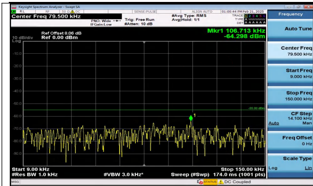
Band7_15MHz_QPSK_20825_1RB#74_0.009~0.15_0.009 ~0.15
