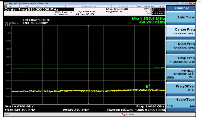
Band7_15MHz_16QAM_20825_1RB#74_30~1000_30~10 00
