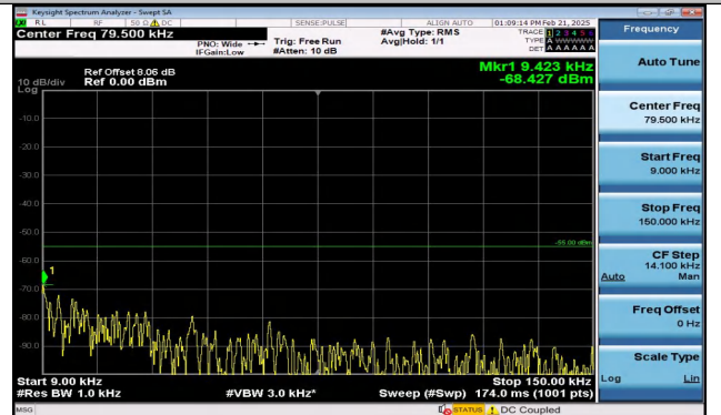
Band7_15MHz_QPSK_20825_75RB#0_0.009~0.15_0.009 ~0.15
