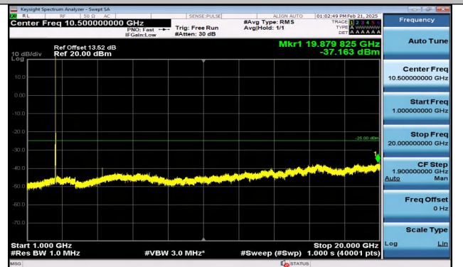
Band7_15MHz_QPSK_21100_1RB#0_1000~20000_1000 ~20000
