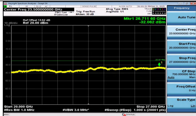
Band7_15MHz_QPSK_20825_1RB#74_20000~27000_20 000~27000
