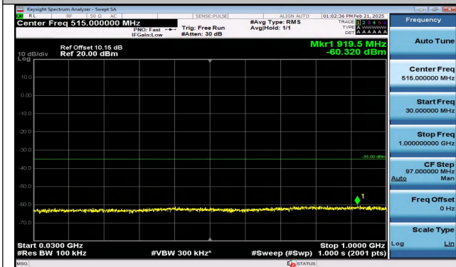
Band7_15MHz_QPSK_21100_1RB#0_30~1000_30~1000
