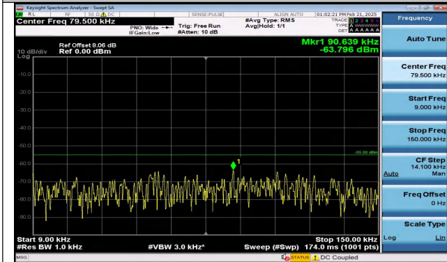
Band7_15MHz_QPSK_21100_1RB#0_0.009~0.15_0.009~ 0.15
