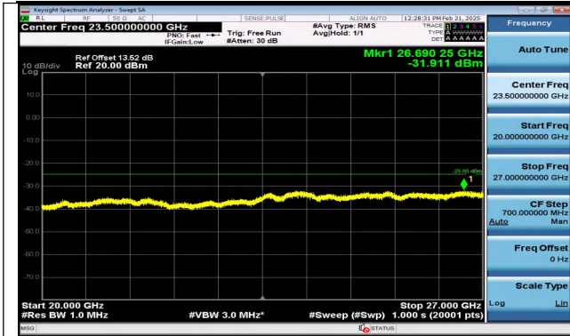
Band7_10MHz_16QAM_20800_1RB#49_20000~27000_20000~27000
