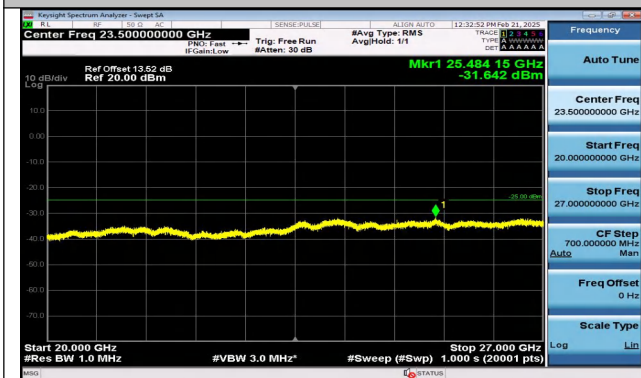
Band7_10MHz_QPSK_21400_1RB#0_20000~27000_20000~27000
