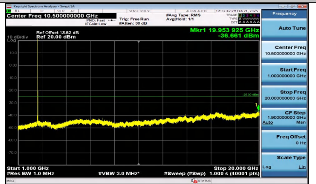
Band7_10MHz_QPSK_21400_1RB#0_1000~20000_1000~20000
