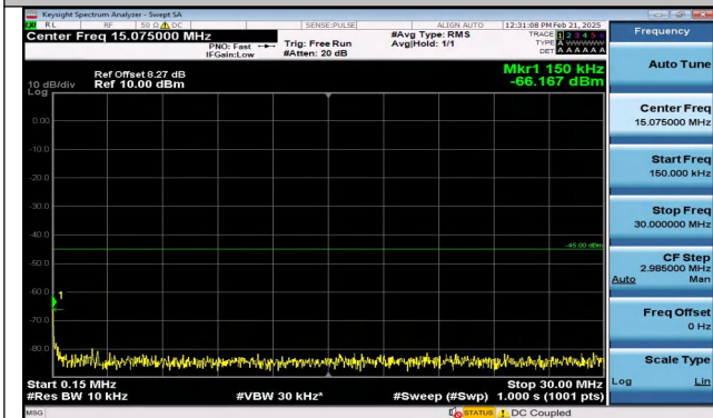
Band7_10MHz_16QAM_21100_1RB#49_0.15~30_0.15~3 0
