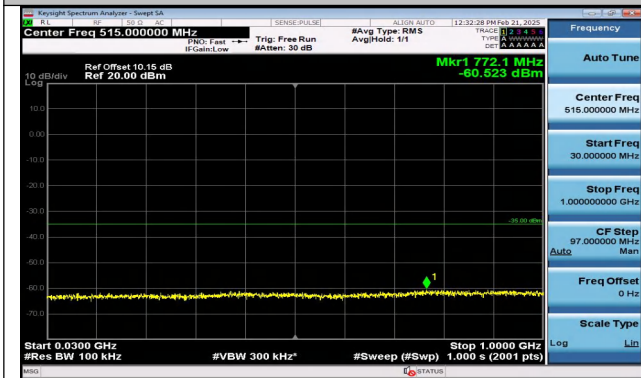
Band7_10MHz_QPSK_21400_1RB#0_30~1000_30~1000
