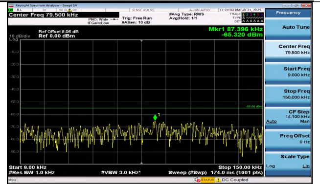
Band7_10MHz_QPSK_21100_1RB#0_0.009~0.15_0.009~0.15
