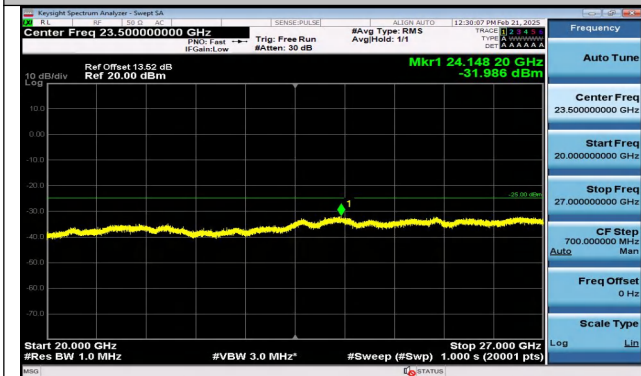
Band7_10MHz_16QAM_21100_1RB#0_20000~27000_20 000~27000
