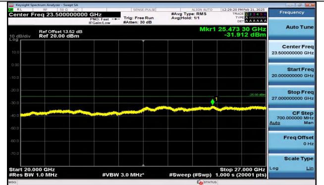
Band7_10MHz_QPSK_21100_1RB#0_20000~27000_20000~27000
