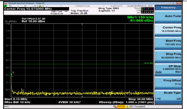
Band7_10MHz_16QAM_21100_1RB#0_0.15~30_0.15~30
