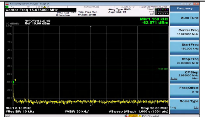
Band7_10MHz_QPSK_21100_1RB#49_0.15~30_0.15~30
