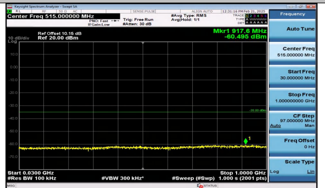
Band7_10MHz_16QAM_21100_1RB#49_30~1000_30~10 00
