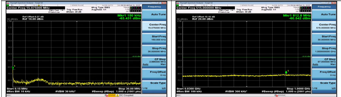
Band7_5MHz_16QAM_21425_25RB#0_0.15~30_0.15~30 0
