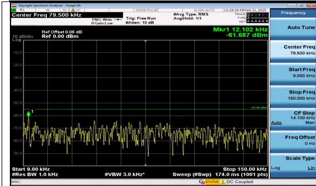
Band7_10MHz_16QAM_21100_1RB#0_0.009~0.15_0.009 ~0.15
