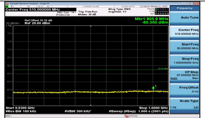
Band7_10MHz_QPSK_21100_1RB#0_30~1000_30~1000
