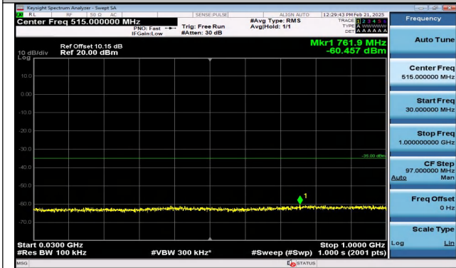
Band7_10MHz_16QAM_21100_1RB#0_30~1000_30~100 0
