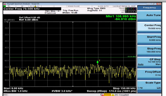
Band7_10MHz_QPSK_21400_1RB#49_0.009~0.15_0.009~0.15
