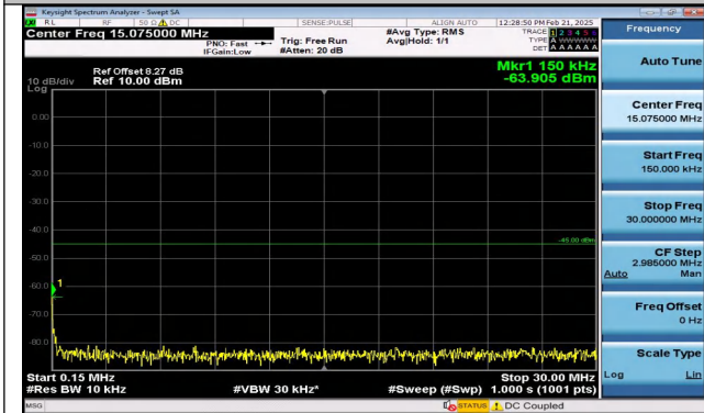
Band7_10MHz_QPSK_21100_1RB#0_0.15~30_0.15~30
