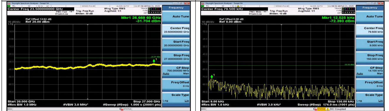
Band7_5MHz_16QAM_21425_1RB#24_20000~27000_20000~27000 000~27000
