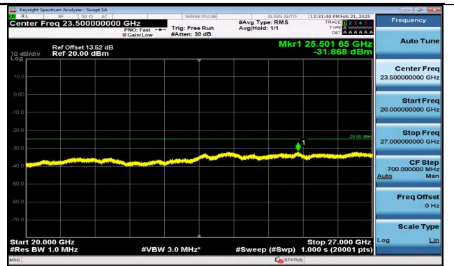
Band7_10MHz_16QAM_21100_1RB#49_20000~27000_20000~27000
