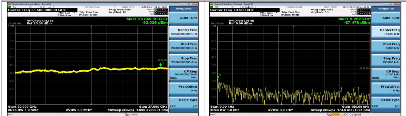
Band7_5MHz_16QAM_20775_1RB#24_20000~27000_20 000~27000
