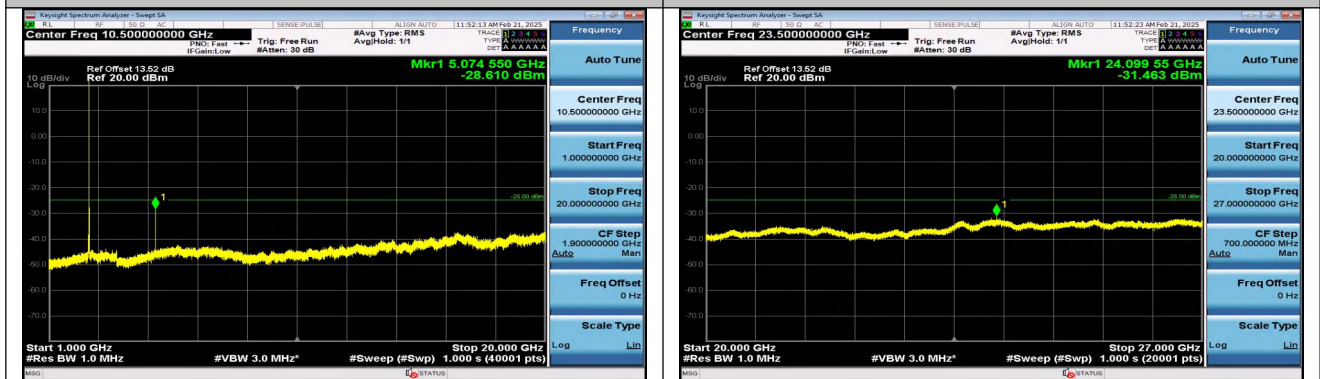
Band7_5MHz_QPSK_21100_1RB#24_1000~20000_1000 ~20000
