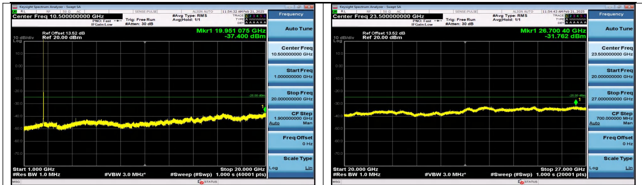
Band7_5MHz_16QAM_21100_25RB#0_1000~20000_100 0~20000
