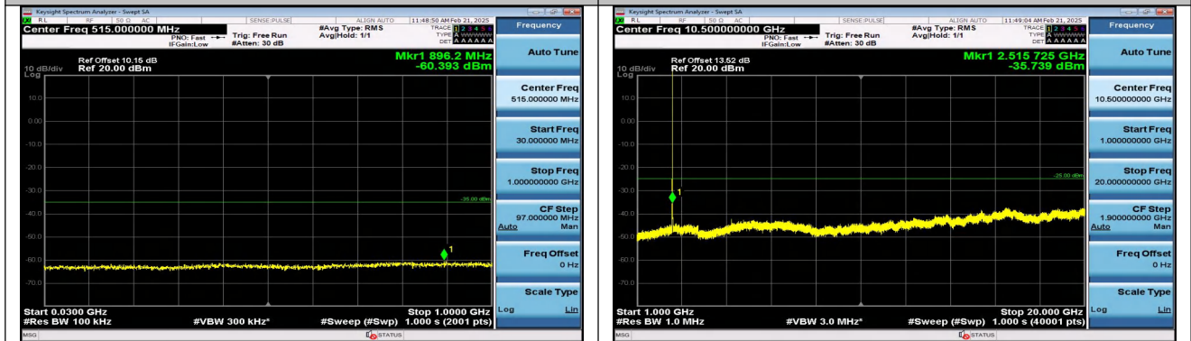
Band7_5MHz_QPSK_20775_25RB#0_1000~20000_1000~20000
