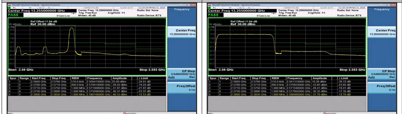
Band7_10MHz_QPSK_21400_1RB#49
