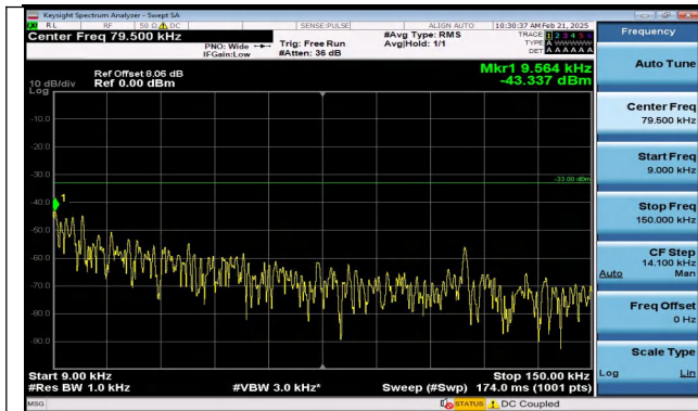
Band5_5MHz_QPSK_20425_1RB#0_0.009~0.15_0.009~0.15
