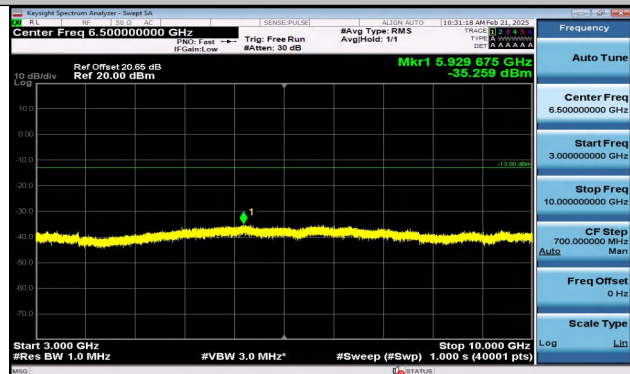
Band5_5MHz_QPSK_20425_1RB#0_3000~10000_3000~10000
