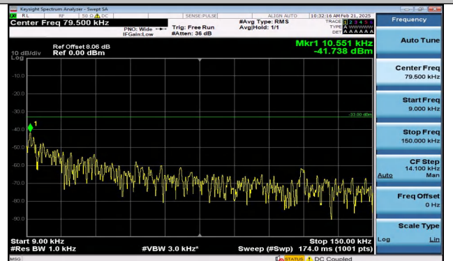
Band5_5MHz_QPSK_20425_1RB#24_0.009~0.15_0.009~0.15
