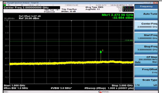
Band5_5MHz_QPSK_20425_1RB#0_1000~3000_1000~3000
