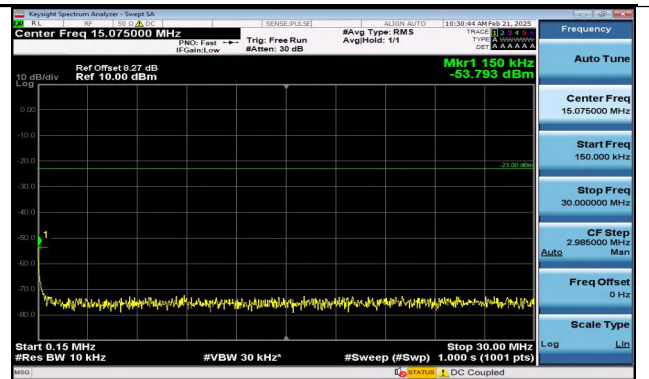
Band5_5MHz_QPSK_20425_1RB#0_0.15~30_0.15~30
