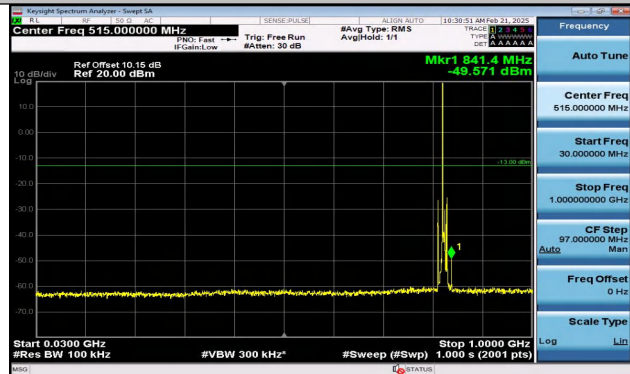
Band5_5MHz_QPSK_20425_1RB#0_30~1000_30~1000
