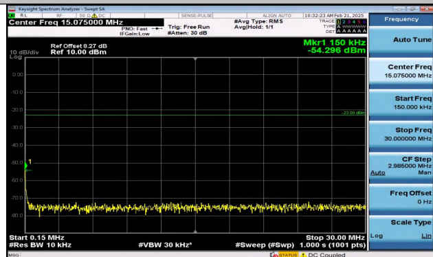
Band5_5MHz_QPSK_20425_1RB#24_0.15~30_0.15~30
