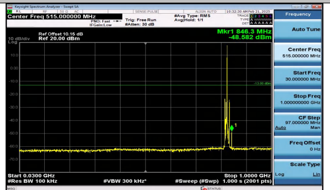
Band5_5MHz_QPSK_20425_1RB#24_30~1000_30~1000
