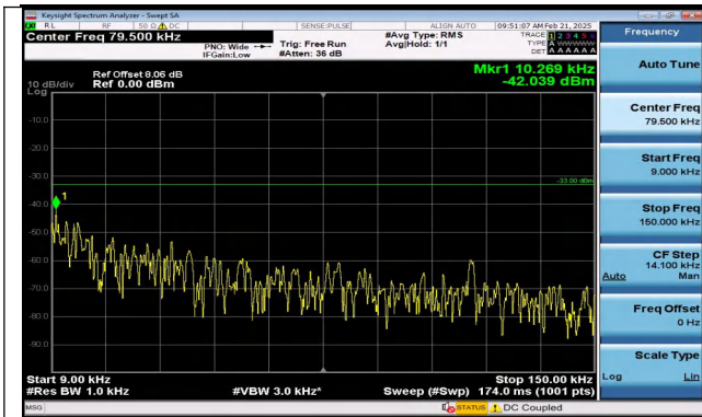
Band5_3MHz_QPSK_20415_15RB#0_0.009~0.15_0.009~0.15
