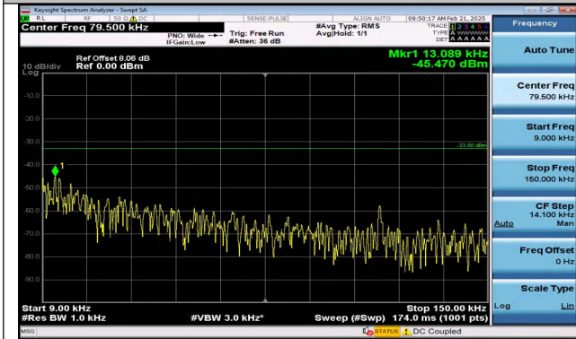
Band5_3MHz_16QAM_20415_1RB#14_0.009~0.15_0.009~0.15
