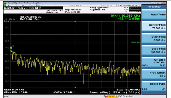
Band5_3MHz_QPSK_20415_1RB#14_0.009~0.15_0.009~0.15
