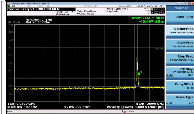
Band5_3MHz_QPSK_20415_1RB#0_30~1000_30~1000
