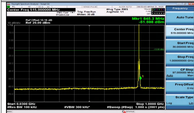
Band5_3MHz_QPSK_20525_1RB#0_30~1000_30~1000
