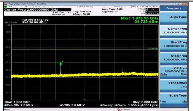
Band5_3MHz_QPSK_20525_1RB#0_1000~3000_1000~3000
