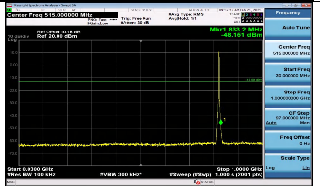
Band5_3MHz_16QAM_20415_15RB#0_30~1000_30~1000
