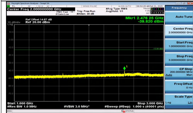
Band5_3MHz_16QAM_20415_15RB#0_1000~3000_1000~3000
