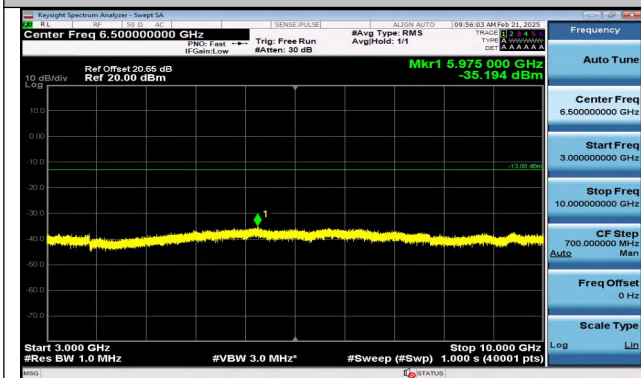
Band5_3MHz_16QAM_20525_1RB#14_3000~10000_300 0~10000
