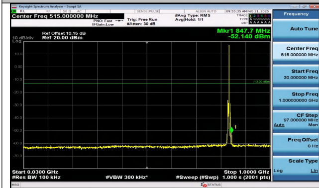
Band5_3MHz_16QAM_20525_1RB#14_30~1000_30~100 0
