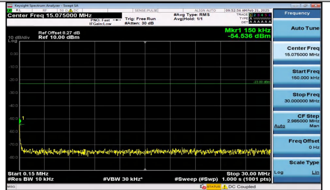
Band5_3MHz_QPSK_20525_1RB#0_0.15~30_0.15~30
