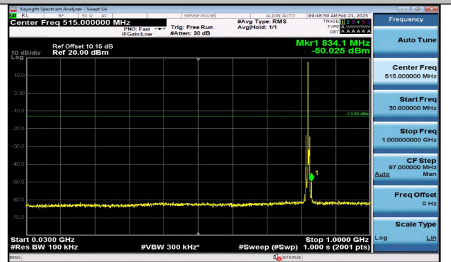
Band5_3MHz_16QAM_20415_1RB#0_30~1000_30~1000
