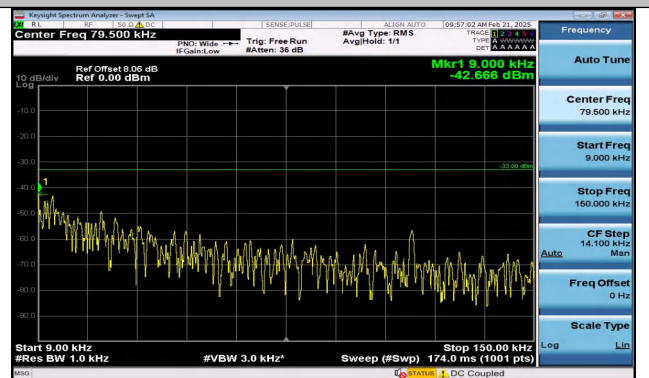
Band5_3MHz_16QAM_20525_15RB#0_0.009~0.15_0.009 ~0.15
