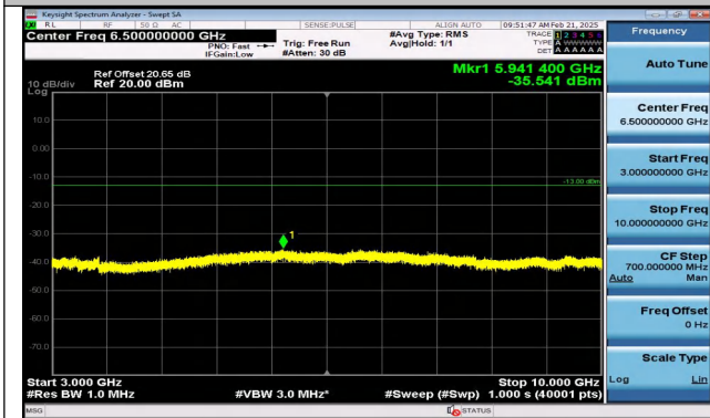
Band5_3MHz_QPSK_20415_15RB#0_3000~10000_3000~10000
