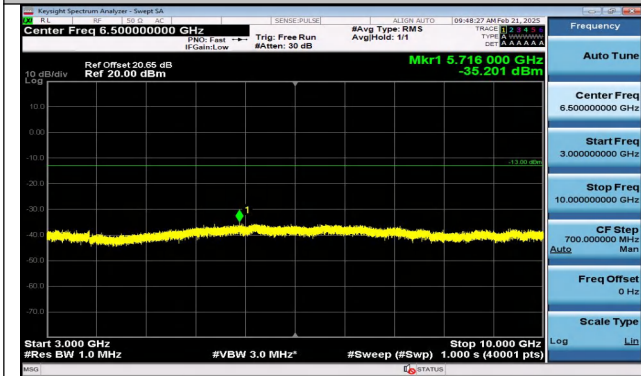
Band5_3MHz_QPSK_20415_1RB#0_3000~10000_3000~10000
