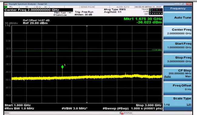
Band5_3MHz_16QAM_20525_1RB#14_1000~3000_1000 ~3000
