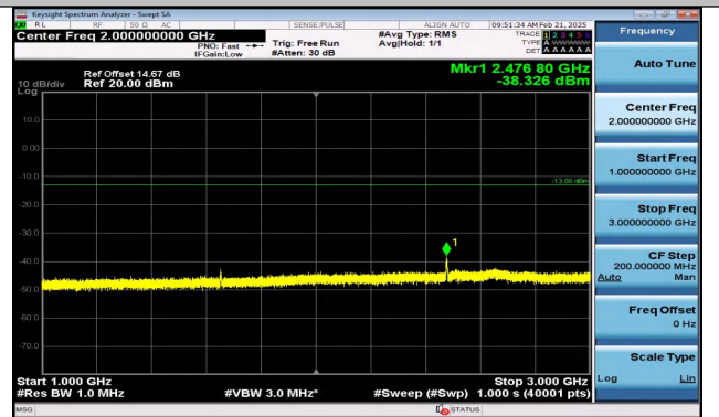
Band5_3MHz_QPSK_20415_15RB#0_1000~3000_1000~3000
