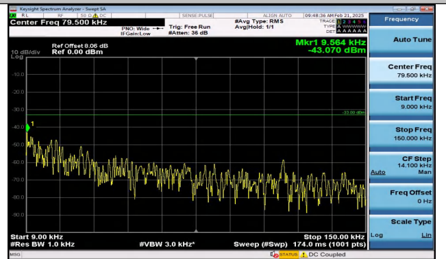
Band5_3MHz_16QAM_20415_1RB#0_0.009~0.15_0.009~0.15
