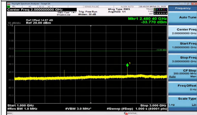
Band5_3MHz_QPSK_20415_1RB#14_1000~3000_1000~3000
