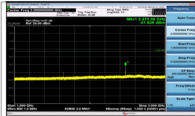
Band5_3MHz_16QAM_20415_1RB#0_1000~3000_1000~3000
