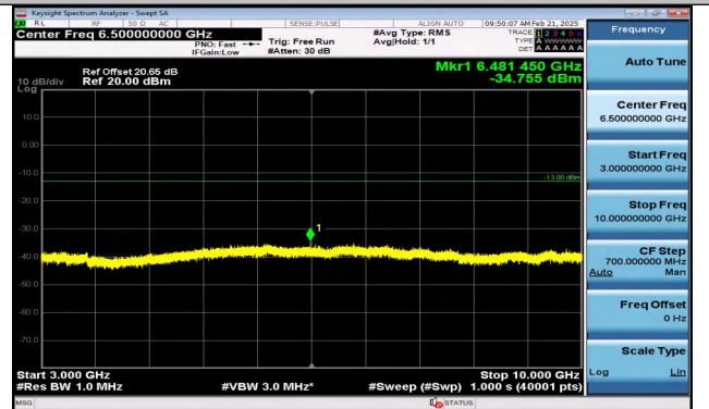
Band5_3MHz_QPSK_20415_1RB#14_3000~10000_3000~10000
