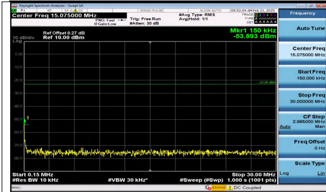
Band5_3MHz_16QAM_20415_15RB#0_0.15~30_0.15~30
