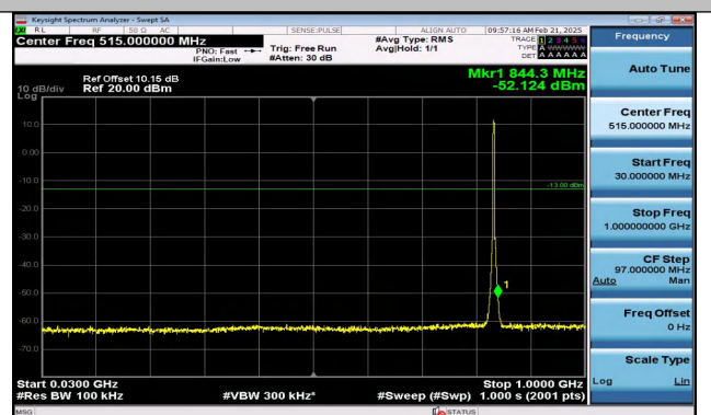
Band5_3MHz_16QAM_20525_15RB#0_30~1000_30~100 0
