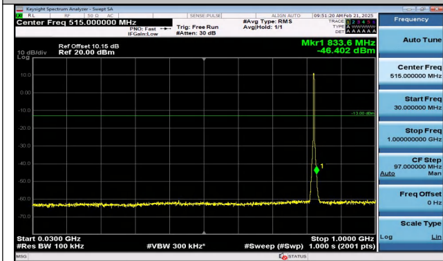
Band5_3MHz_QPSK_20415_15RB#0_30~1000_30~1000
