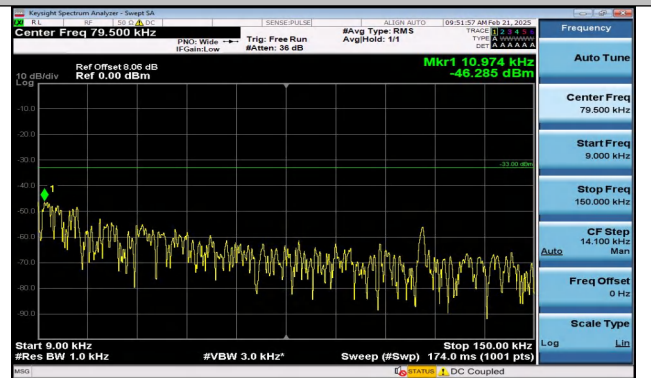
Band5_3MHz_16QAM_20415_15RB#0_0.009~0.15_0.009~0.15
