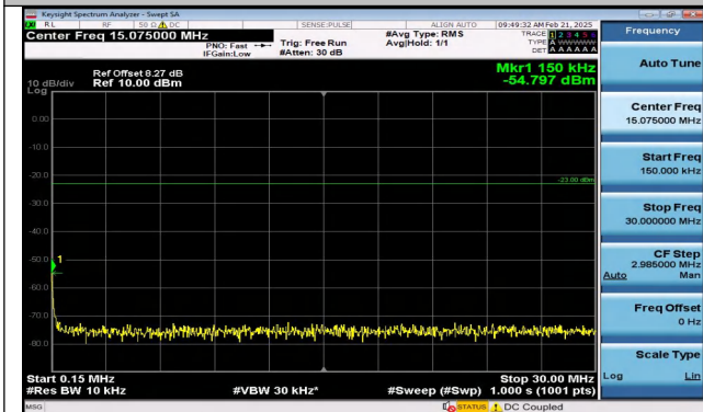
Band5_3MHz_QPSK_20415_1RB#14_0.15~30_0.15~30
