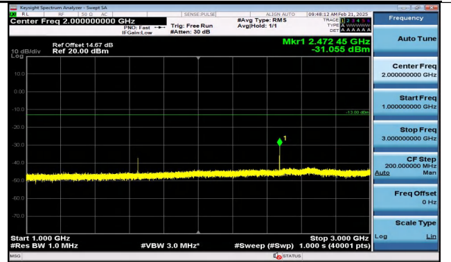
Band5_3MHz_QPSK_20415_1RB#0_1000~3000_1000~3000
