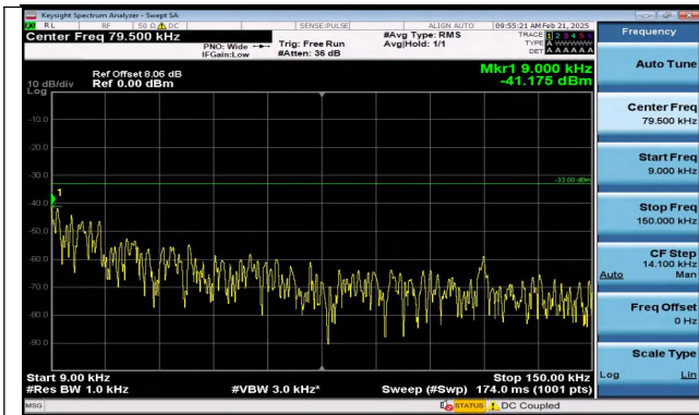
Band5_3MHz_16QAM_20525_1RB#14_0.009~0.15_0.009 ~0.15
