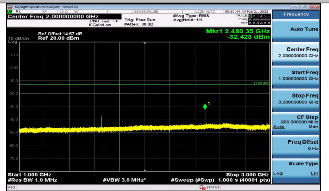
Band5_3MHz_16QAM_20415_1RB#14_1000~3000_1000~3000
