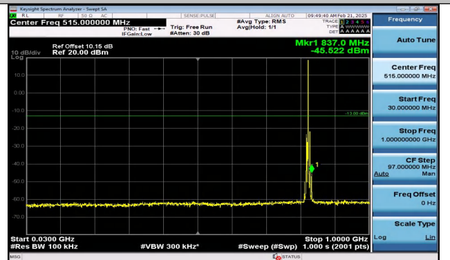
Band5_3MHz_QPSK_20415_1RB#14_30~1000_30~1000
