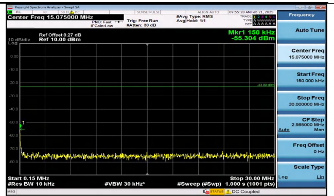
Band5_3MHz_16QAM_20525_1RB#14_0.15~30_0.15~30
