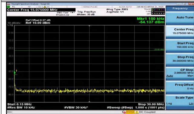
Band5_3MHz_16QAM_20415_1RB#0_0.15~30_0.15~30
