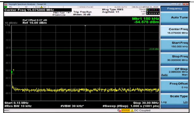
Band5_3MHz_QPSK_20415_15RB#0_0.15~30_0.15~30
