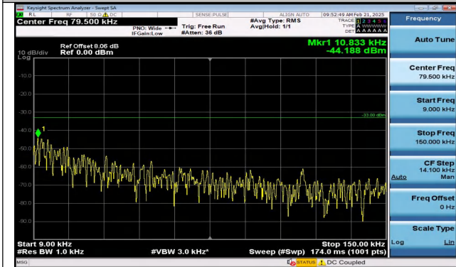
Band5_3MHz_QPSK_20525_1RB#0_0.009~0.15_0.009~0.15
