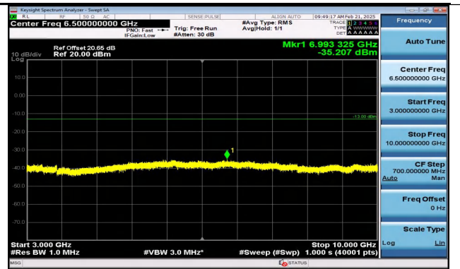
Band5_3MHz_16QAM_20415_1RB#0_3000~10000_3000~10000
